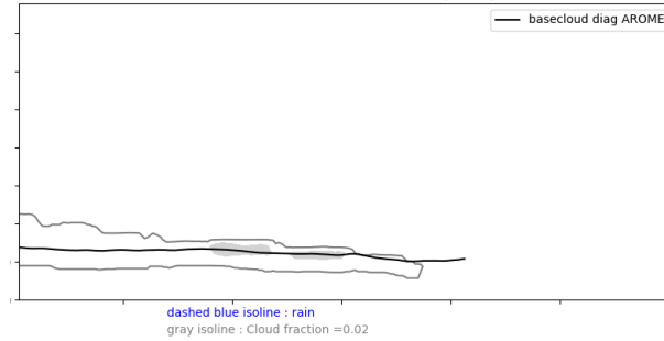
Cross section E/W @ 19.5N 20240618-12-UTC ech(36h)
