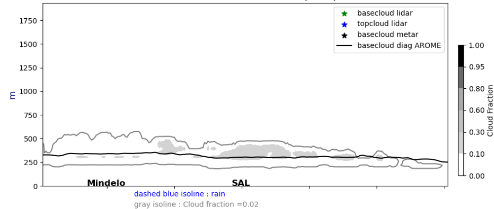
Cross section E/W @ 17.5N 20240617-12-UTC ech(12h)
