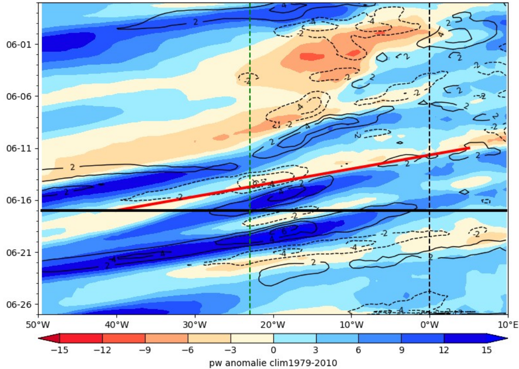
ECMWF PW (color) AND V at 925 hPa 2024-06-17
