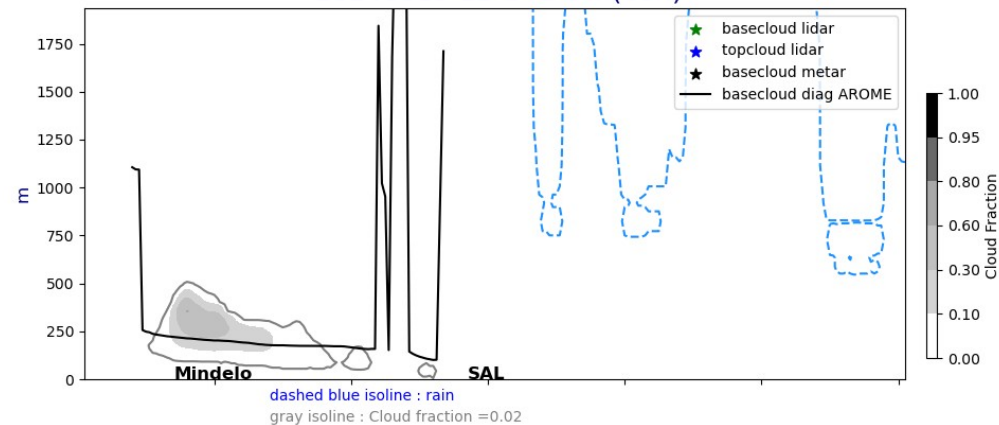
Cross section E/W @ 17.5N 20240619-12-UTC ech(60h)
