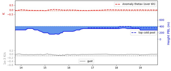
Cross section S/N @ -26W 20240617-12-UTC ech(12h)
