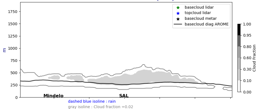
Cross section E/W @ 17.5N 20240618-12-UTC ech(36h)
