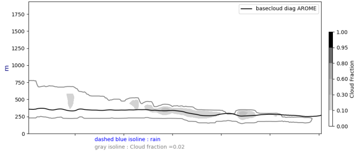
Cross section E/W @ 19.5N 20240617-12-UTC ech(12h)
