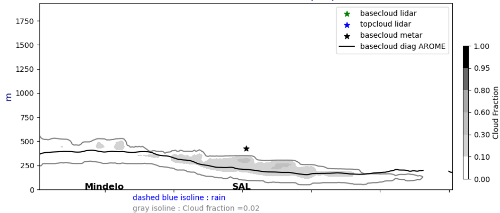
Cross section E/W @ 17.5N 20240617-01-UTC ech(1h)
