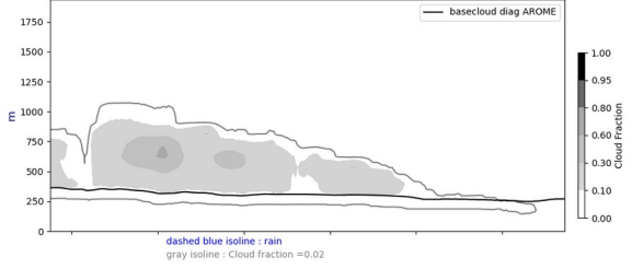
Cross section S/N @ -22W 20240618-12-UTC ech(36h)
