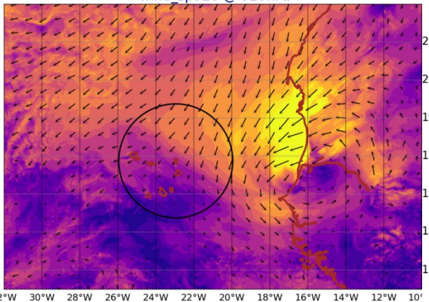
AROME25 20240617-12-UTC -ech(12h) wind_sp920 @ 920hPa
