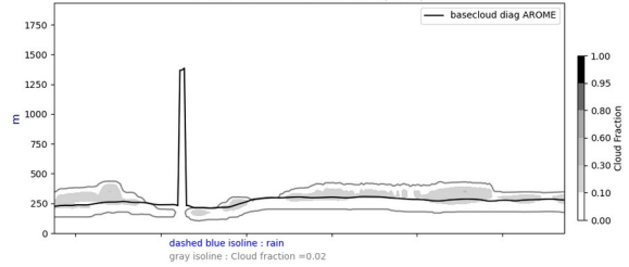
Cross section S/N @ -22W 20240617-12-UTC ech(12h)
