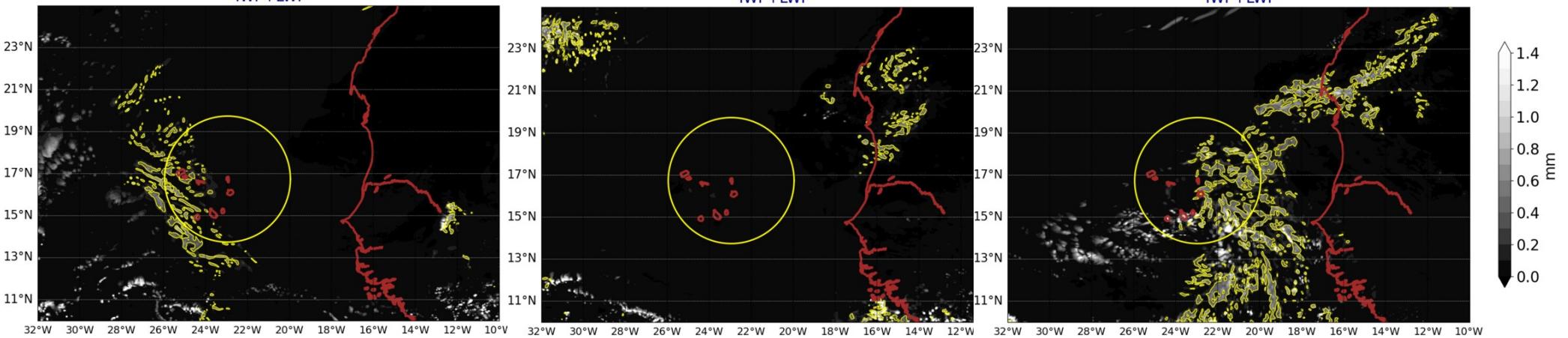
AROME25 20240617-12-UTC -ech(12h) IWP+LWP
