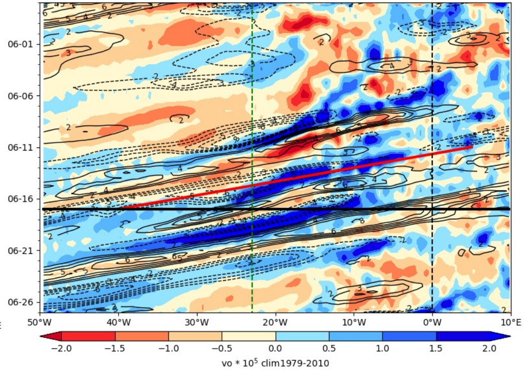
ECMWF Vorticity 850 hPa (color), V-700 hPa 2024-06-17
