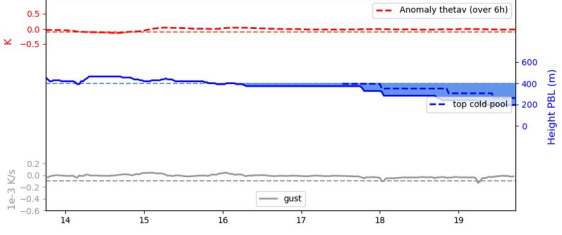
Cross section S/N @ -26W 20240618-12-UTC ech(36h)
