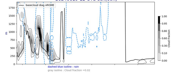
Cross section S/N @ -22W 20240619-12-UTC ech(60h)
