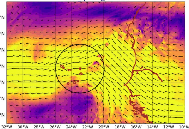
AROME25 20240619-12-UTC -ech(60h) wind_sp920 @ 920hPa
