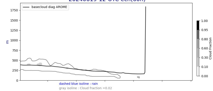
Cross section E/W @ 19.5N 20240619-12-UTC ech(60h)
