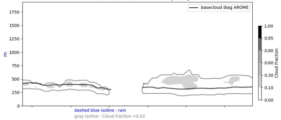
Cross section S/N @ -26W 20240618-12-UTC ech(36h)
