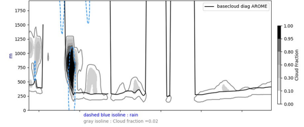
Cross section S/N @ -26W 20240619-12-UTC ech(60h)
