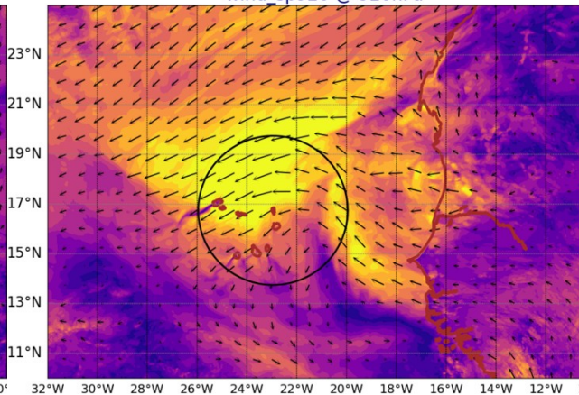
AROME25 20240618-12-UTC -ech(36h) wind_sp920 @ 920hPa
