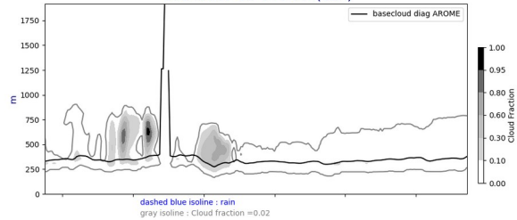
Cross section S/N @ -26W 20240617-12-UTC ech(12h)
