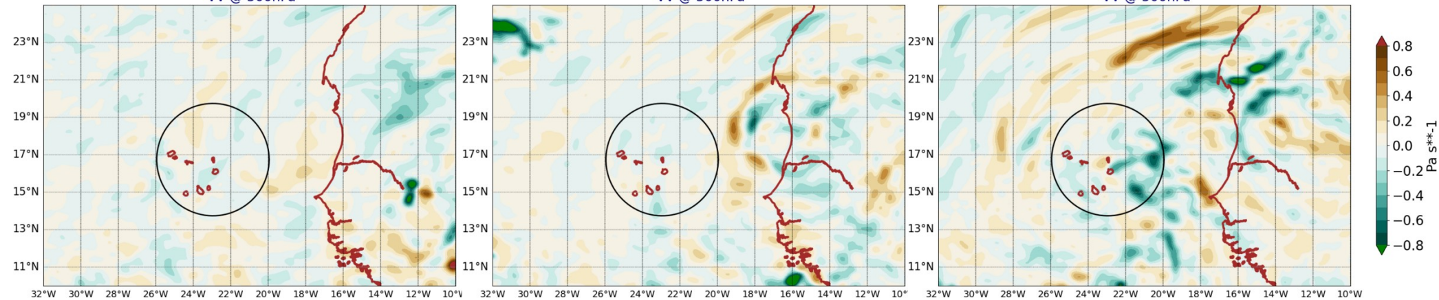
AROME25 20240617-12-UTC -ech(12h) VV @ 500hPa
