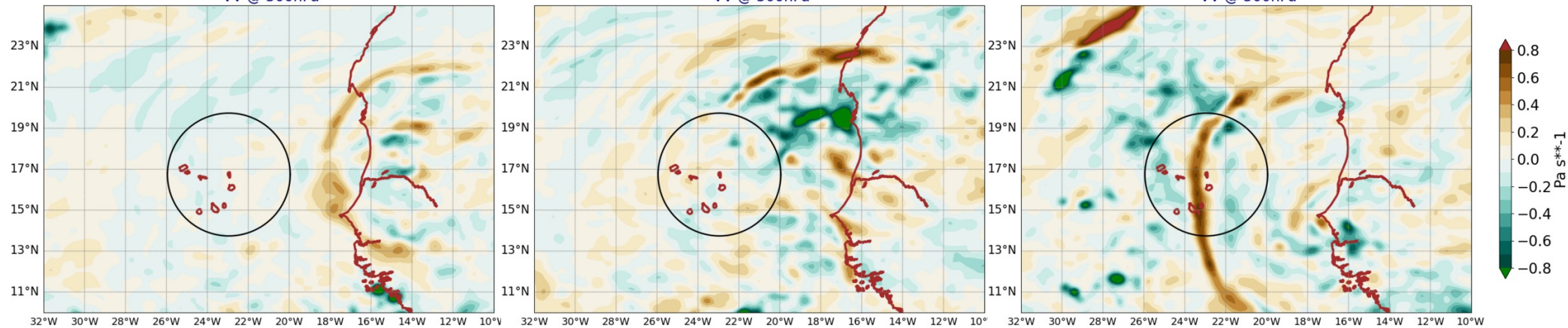
AROME25 20240618-12-UTC -ech(12h) VV @ 500hPa
