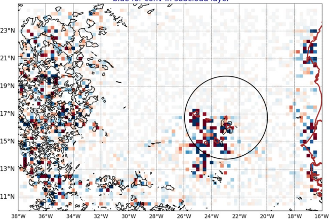
AROME25 regrid 0.25 20240618-12-UTC -ech(12h) blue for conv in subcloud layer
