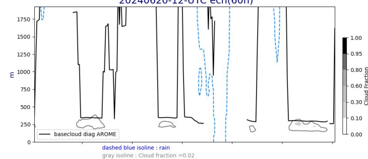
Cross section E/W @ 19.5N 20240620-12-UTC ech(60h)
