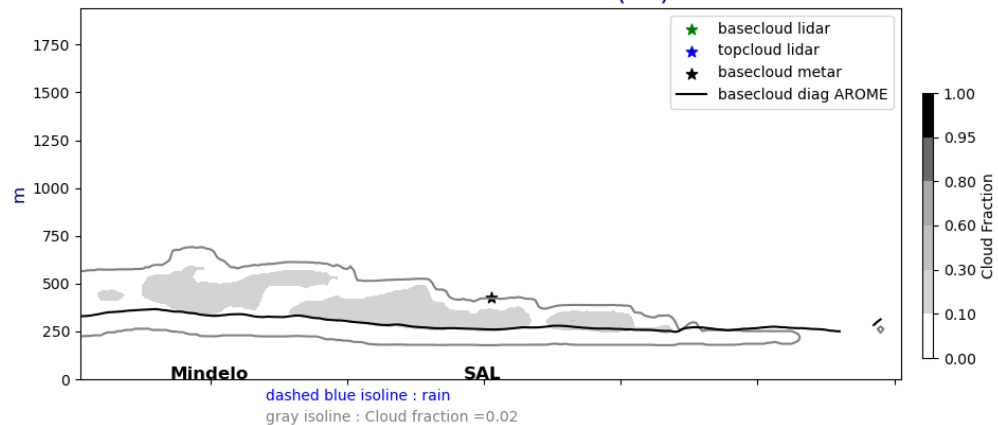
Cross section E/W @ 17.5N 20240618-01-UTC ech(1h)
