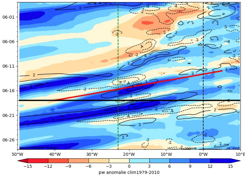
ECMWF PW (color) AND V at 925 hPa 2024-06-18
