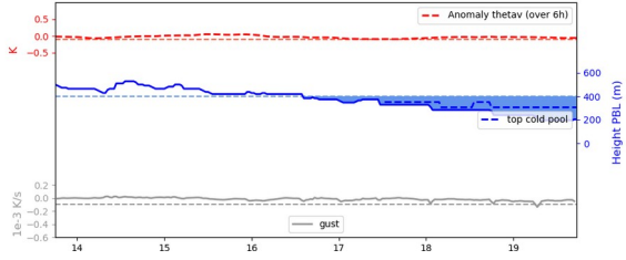
Cross section S/N @ -26W 20240618-12-UTC ech(12h)
