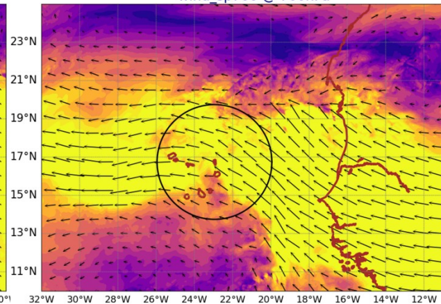
AROME25 20240619-12-UTC -ech(36h) wind_sp920 @ 920hPa
