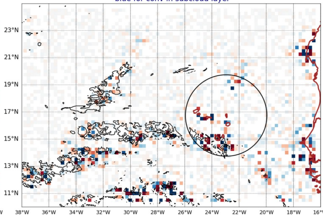
AROME25 regrid 0.25 20240620-12-UTC -ech(60h) blue for conv in subcloud layer
