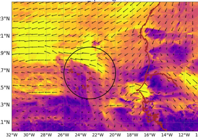
AROME25 20240620-12-UTC -ech(60h) wind_sp920 @ 920hPa
