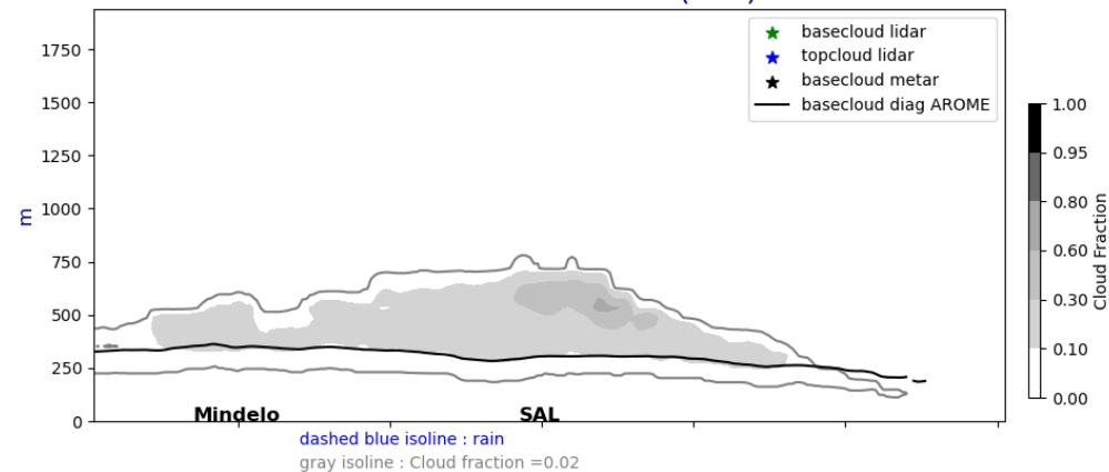
Cross section E/W @ 17.5N 20240618-12-UTC ech(12h)
