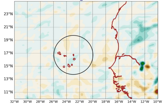
AROME25 20240617-12-UTC -ech(12h) VV @ 500hPa
