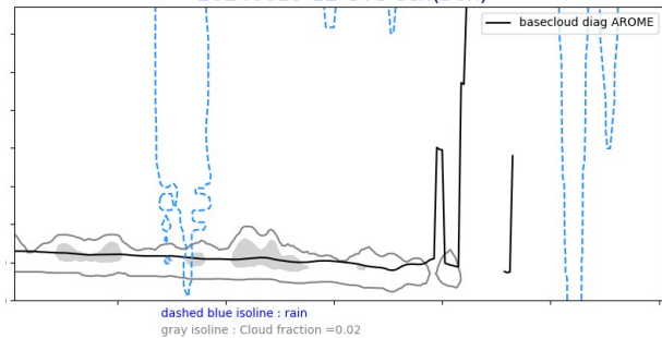
Cross section E/W @ 19.5N 20240619-12-UTC ech(36h)
