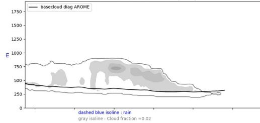
Cross section S/N @ -22W 20240618-12-UTC ech(12h)
