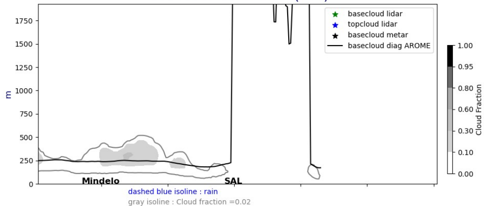
Cross section E/W @ 17.5N 20240619-12-UTC ech(36h)
