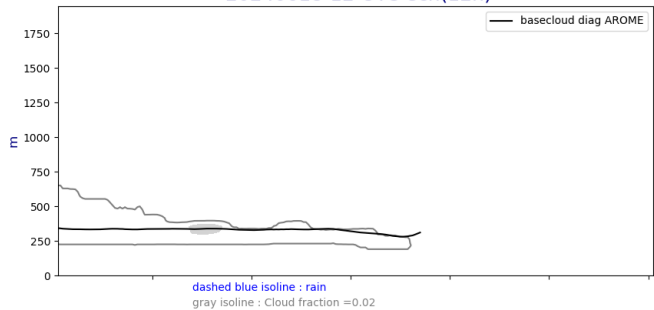
Cross section E/W @ 19.5N 20240618-12-UTC ech(12h)
