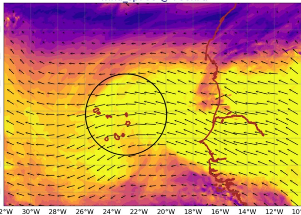
AROME25 20240618-12-UTC -ech(12h) wind_sp920 @ 920hPa
