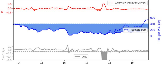
Cross section S/N @ -26W 20240619-12-UTC ech(36h)
