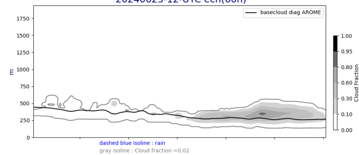
Cross section E/W @ 19.5N 20240623-12-UTC ech(60h)
