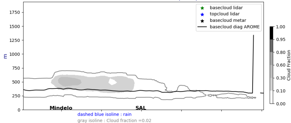
Cross section E/W @ 17.5N 20240623-12-UTC ech(60h)
