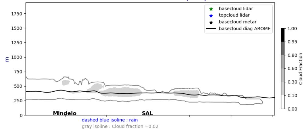
Cross section E/W @ 17.5N 20240621-12-UTC ech(12h)
