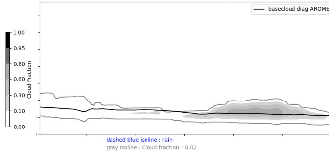
Cross section E/W @ 19.5N 20240622-12-UTC ech(36h)
