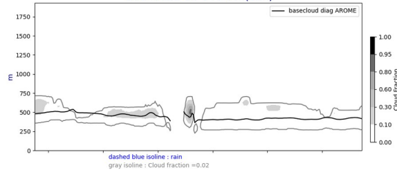
Cross section S/N @ -26W 20240621-12-UTC ech(12h)
