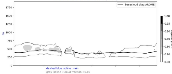
Cross section S/N @ -26W 20240622-12-UTC ech(36h)
