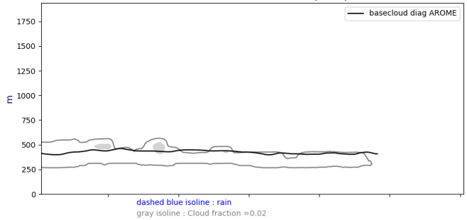
Cross section E/W @ 19.5N 20240621-12-UTC ech(12h)
