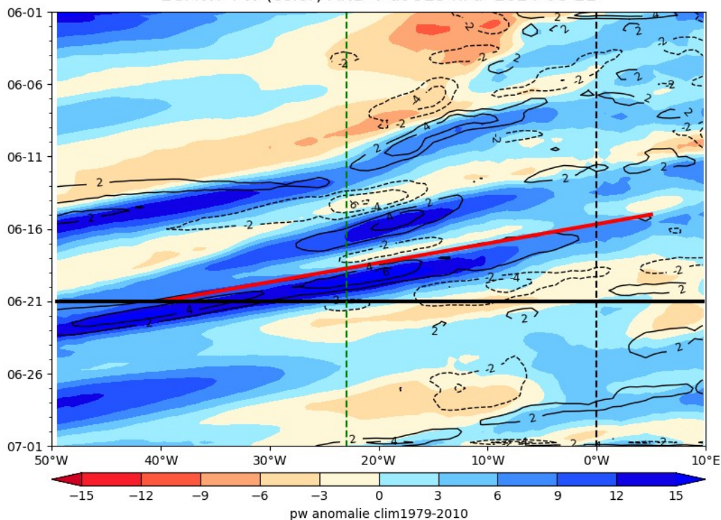
ECMWF PW (color) AND V at 925 hPa 2024-06-21
