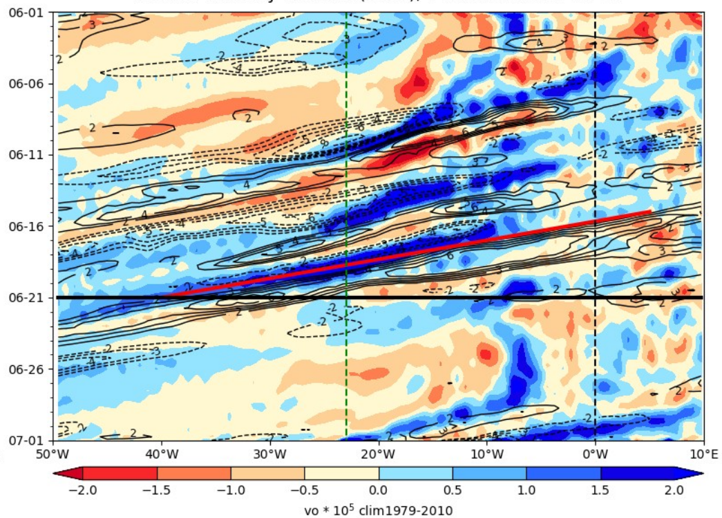
ECMWF Vorticity 850 hPa (color), V-700 hPa 2024-06-21
