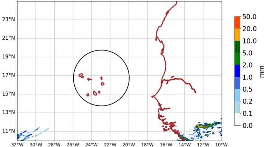
AROME25 20240621-15-UTC -ech(15h) RR cumulated over 6h
