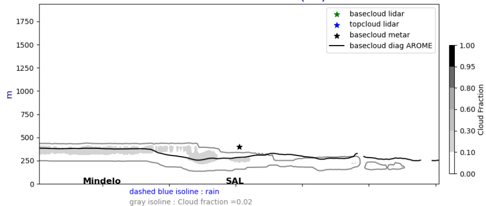
Cross section E/W @ 17.5N 20240621-01-UTC ech(1h)
