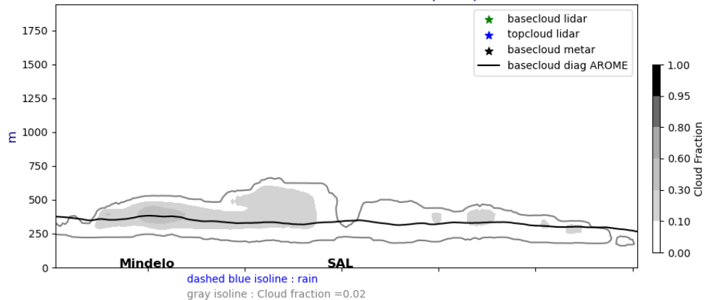
Cross section E/W @ 17.5N 20240622-12-UTC ech(36h)
