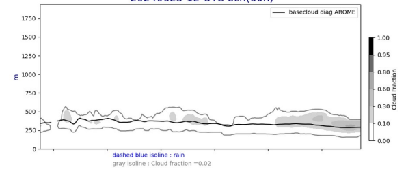
Cross section S/N @ -22W 20240623-12-UTC ech(60h)
