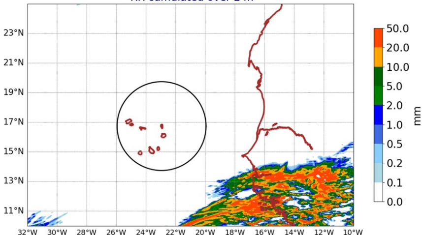
AROME25 20240623-12-UTC -ech(60h) RR cumulated over 24h
