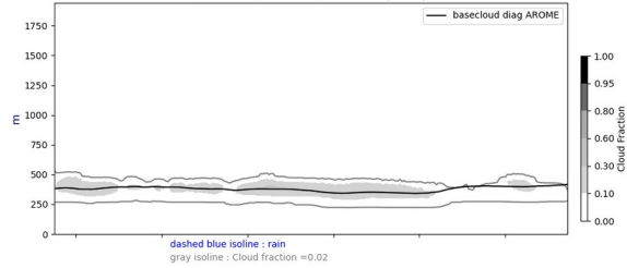
Cross section S/N @ -22W 20240621-12-UTC ech(12h)
