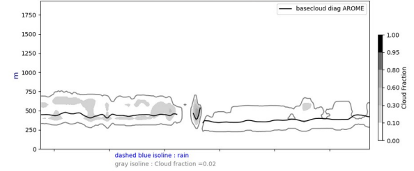
Cross section S/N @ -26W 20240623-12-UTC ech(60h)
