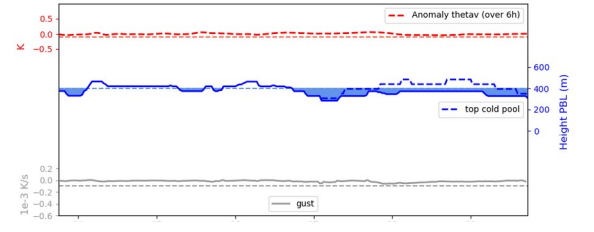
Cross section S/N @ -26W 20240623-12-UTC ech(60h)
