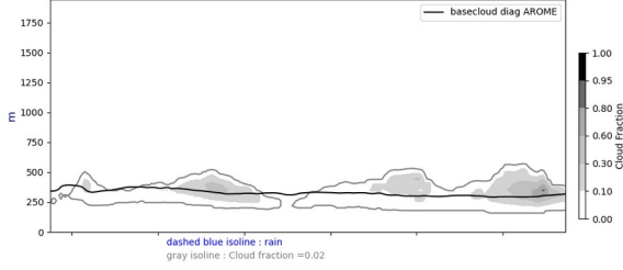
Cross section S/N @ -22W 20240622-12-UTC ech(36h)
