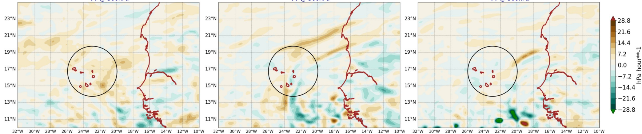
AROME25 20240623-12-UTC -ech(12h) VV @ 500hPa
