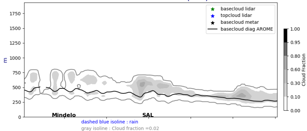
Cross section E/W @ 17.5N 20240624-12-UTC ech(36h)
