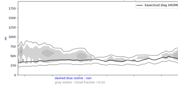
Cross section S/N @ -22W 20240624-12-UTC ech(36h)
