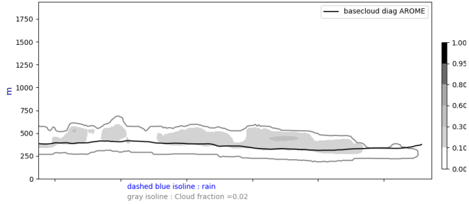
Cross section S/N @ -22W 20240623-12-UTC ech(12h)
