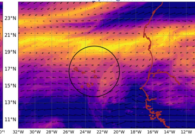
AROME25 20240624-12-UTC -ech(36h) wind_sp920 @ 920hPa
