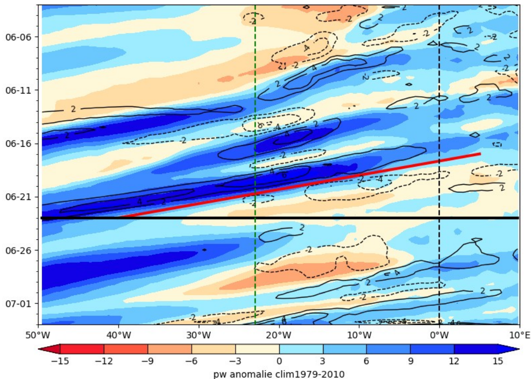
ECMWF PW (color) AND V at 925 hPa 2024-06-23
