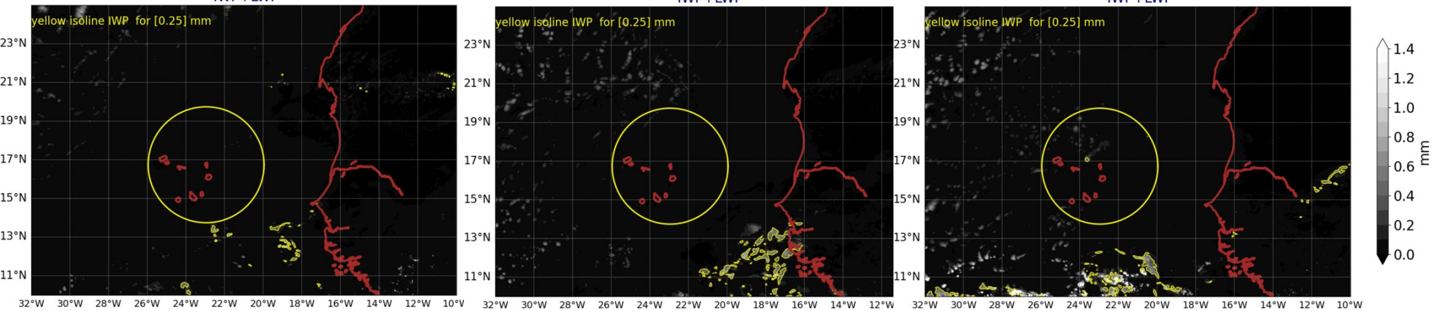
AROME25 20240623-12-UTC -ech(12h) IWP+LWP
