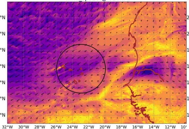
AROME25 20240623-12-UTC -ech(12h) wind_sp920 @ 920hPa
