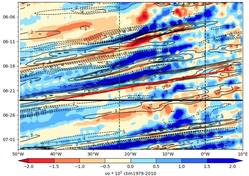
ECMWF Vorticity 850 hPa (color), V-700 hPa 2024-06-23
