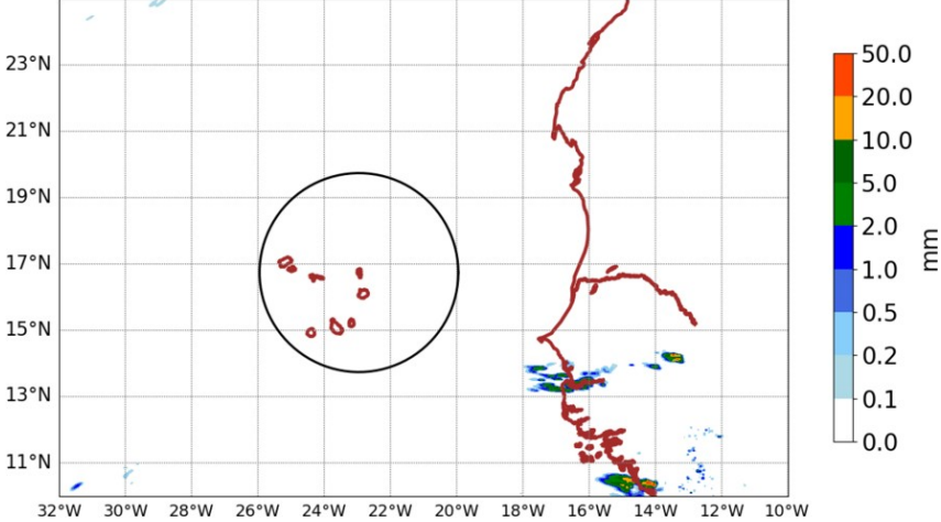
AROME25 20240623-15-UTC -ech(15h) RR cumulated over 6h
