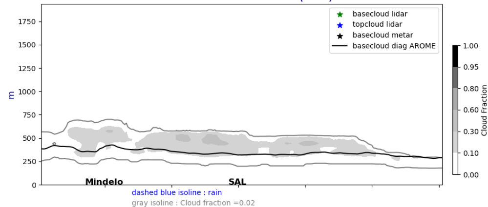
Cross section E/W @ 17.5N 20240623-12-UTC ech(12h)
