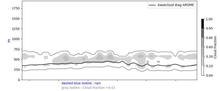
Cross section S/N @ -22W 20240625-12-UTC ech(60h)
