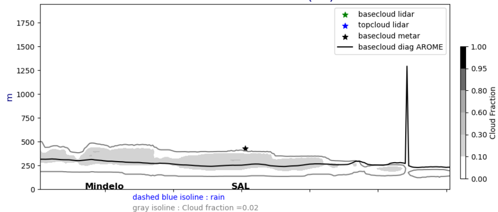
Cross section E/W @ 17.5N 20240623-01-UTC ech(1h)
