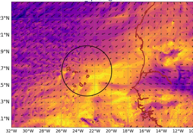
AROME25 20240625-12-UTC -ech(60h) wind_sp920 @ 920hPa
