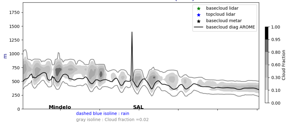
Cross section E/W @ 17.5N 20240625-12-UTC ech(60h)
