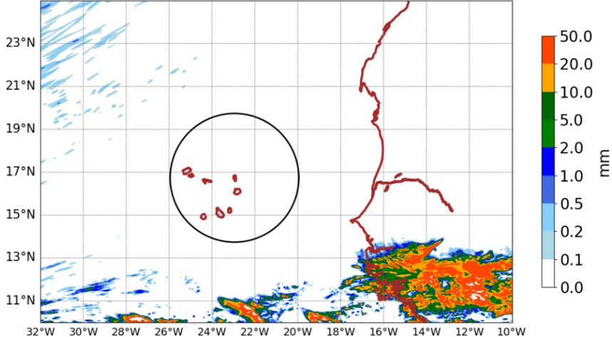
AROME25 20240625-12-UTC -ech(60h) RR cumulated over 24h
