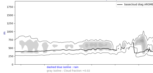
Cross section S/N @ -22W 20240625-12-UTC ech(36h)
