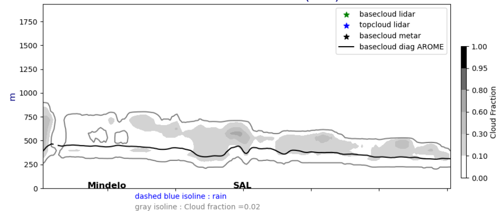
Cross section E/W @ 17.5N 20240624-12-UTC ech(12h)
