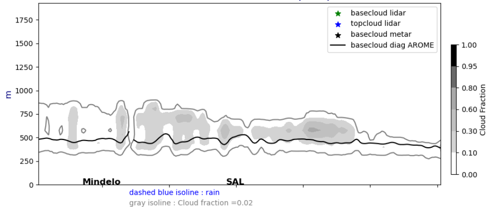
Cross section E/W @ 17.5N 20240625-12-UTC ech(36h)
