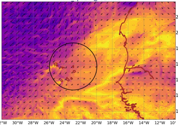
AROME25 20240624-12-UTC -ech(12h) wind_sp920 @ 920hPa
