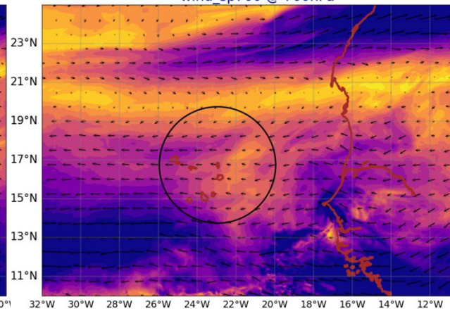
AROME25 20240625-12-UTC -ech(36h) wind_sp920 @ 920hPa
