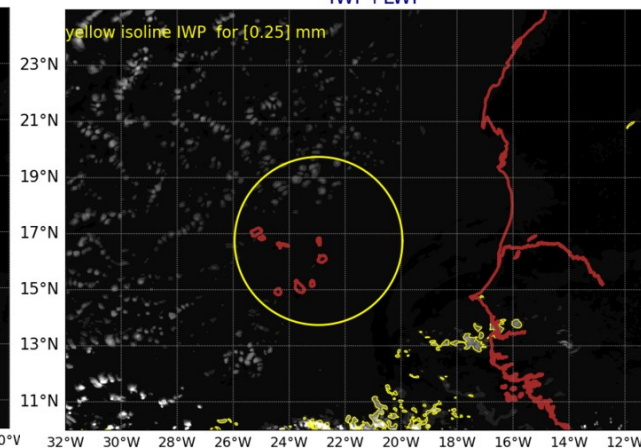
AROME25 20240625-12-UTC -ech(36h) IWP+LWP
