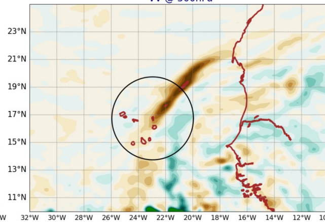
AROME25 20240625-12-UTC -ech(36h) VV @ 500hPa
