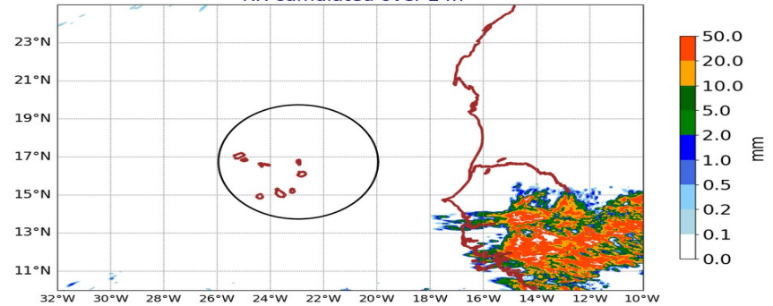
AROME25 20240624-00-UTC -ech(24h) RR cumulated over 24h
