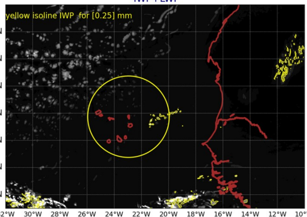
AROME25 20240626-12-UTC -ech(60h) IWP+LWP
