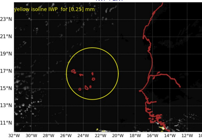
AROME25 20240624-12-UTC -ech(12h) IWP+LWP
