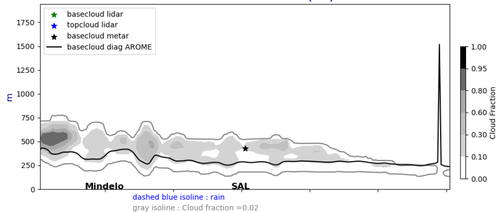
Cross section E/W @ 17.5N 20240624-01-UTC ech(1h)
