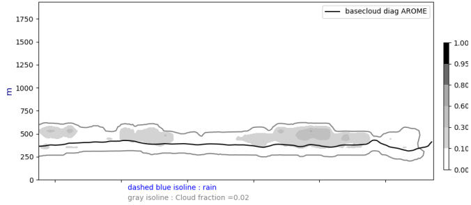
Cross section S/N @ -22W 20240624-12-UTC ech(12h)
