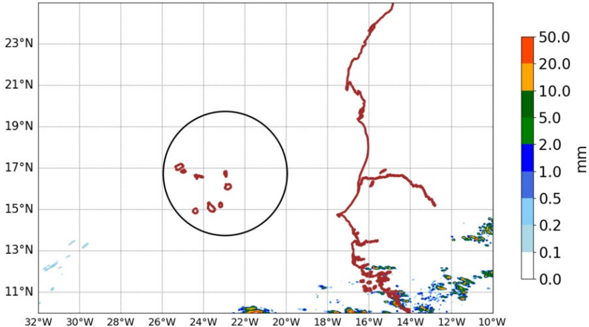
AROME25 20240624-15-UTC -ech(15h) RR cumulated over 6h
