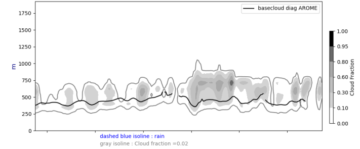
Cross section S/N @ -22W 20240626-12-UTC ech(60h)
