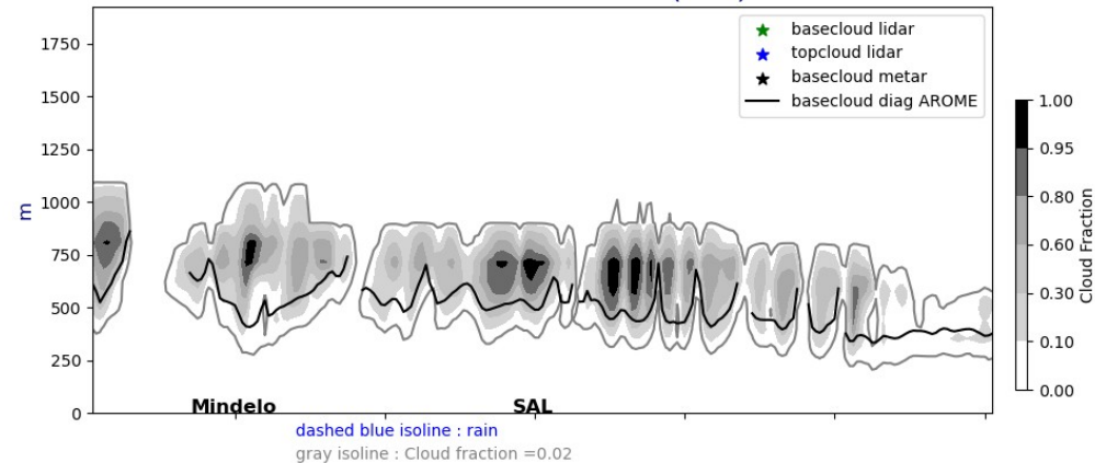
Cross section E/W @ 17.5N 20240626-12-UTC ech(60h)
