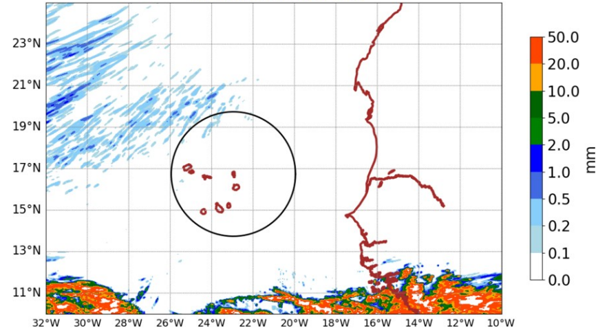
AROME25 20240626-12-UTC -ech(60h) RR cumulated over 24h
