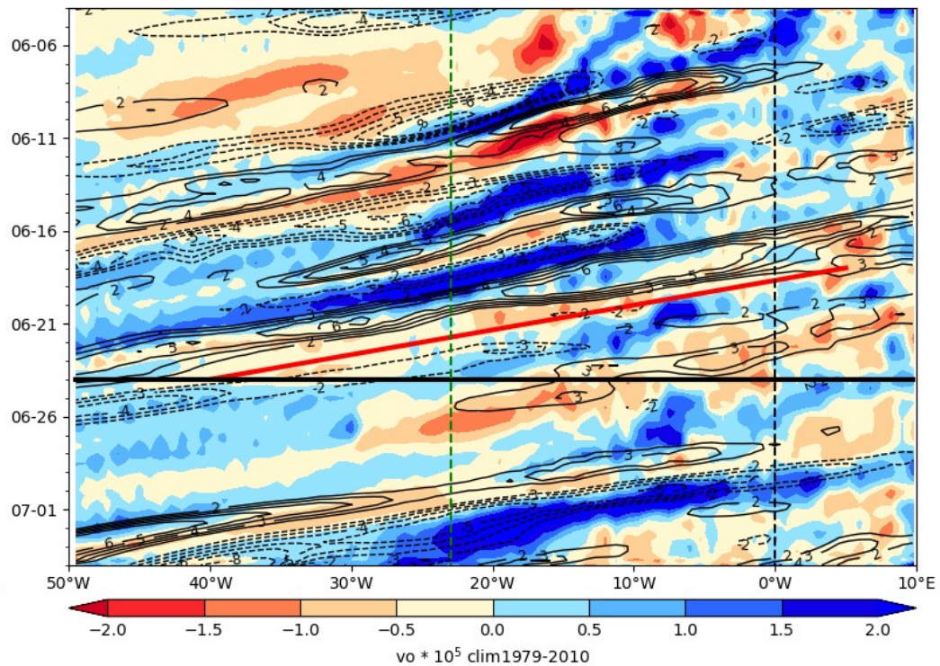
ECMWF Vorticity 850 hPa (color), V-700 hPa 2024-06-24
