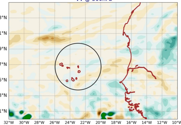
AROME25 20240626-12-UTC -ech(60h) VV @ 500hPa
