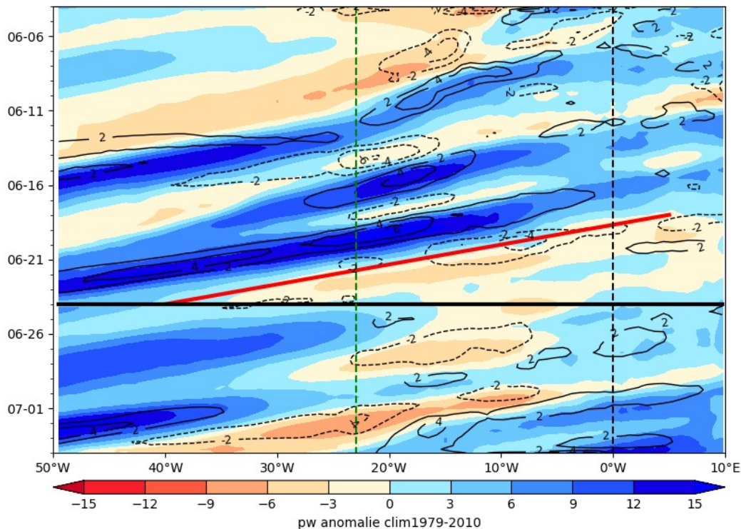
ECMWF PW (color) AND V at 925 hPa 2024-06-24
