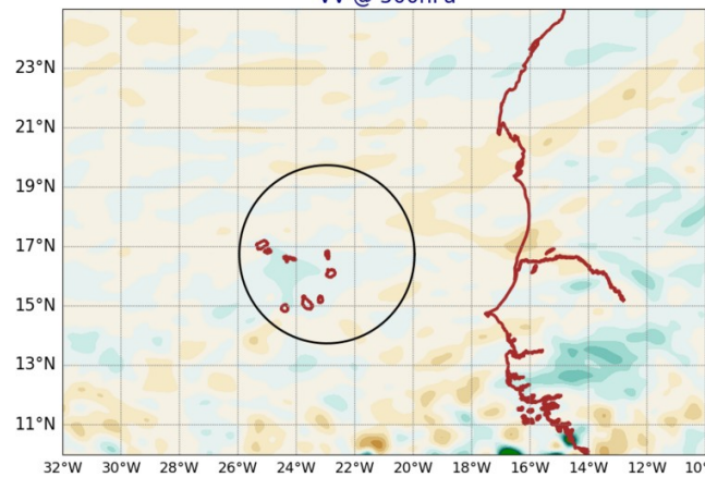
AROME25 20240624-12-UTC -ech(12h) VV @ 500hPa
