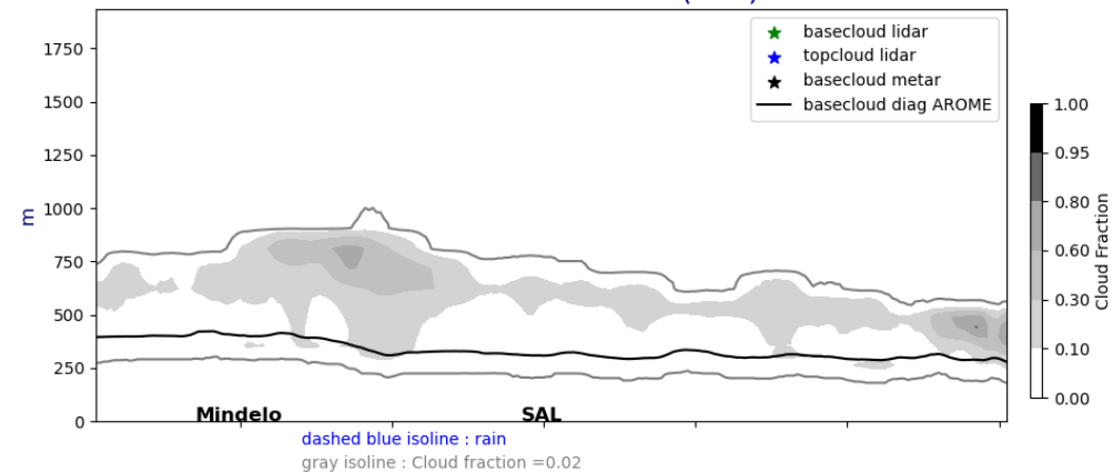
Cross section E/W @ 17.5N 20240702-12-UTC ech(12h)
