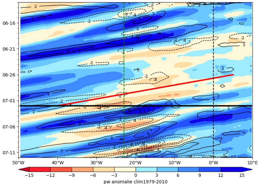
ECMWF PW (color) AND V at 925 hPa 2024-07-02
