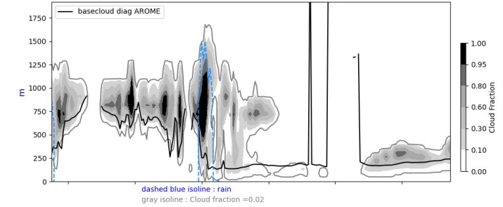
Cross section S/N @ -22W 20240704-12-UTC ech(60h)
