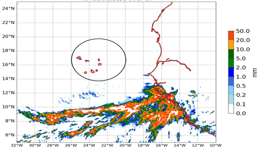
AROME25 20240702-15-UTC -ech(15h) RR cumulated over 6h
