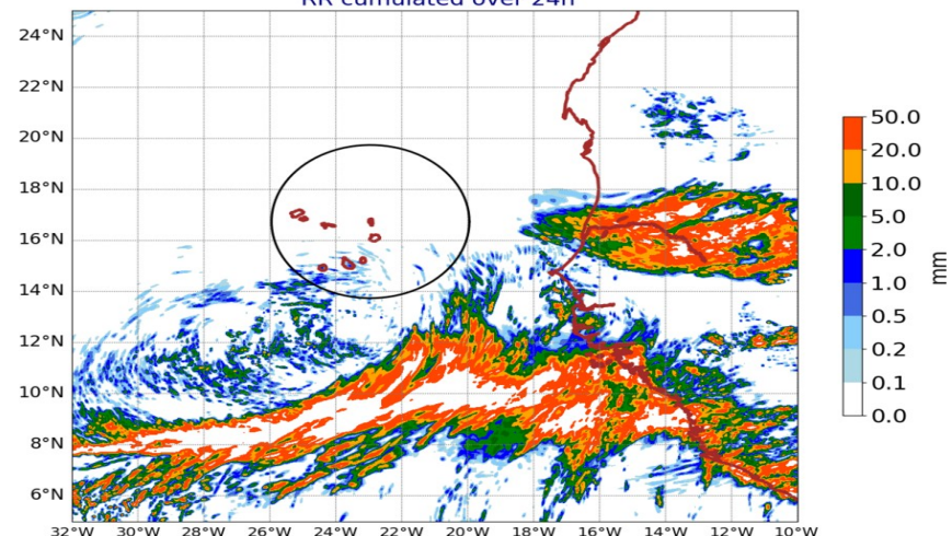
AROME25 20240704-12-UTC -ech(60h) RR cumulated over 24h
