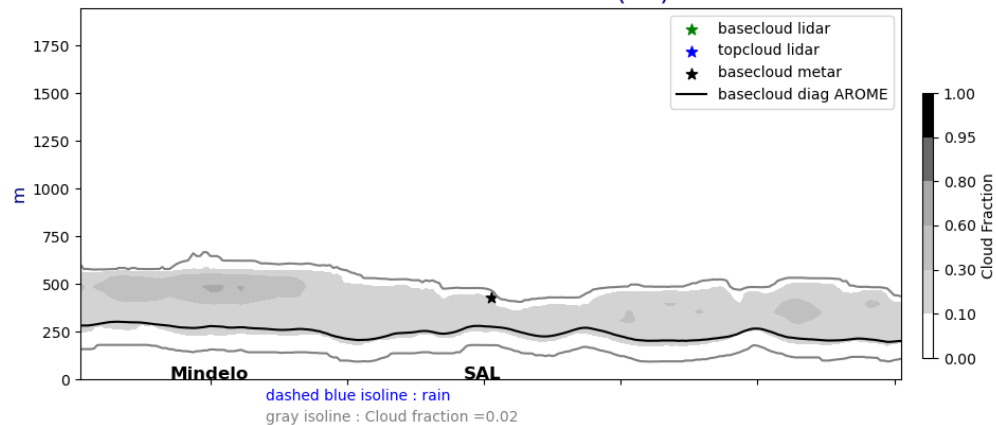
Cross section E/W @ 17.5N 20240702-01-UTC ech(1h)
