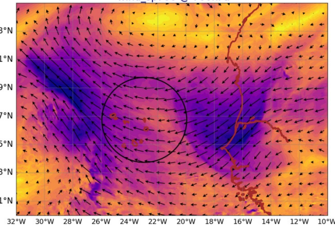
AROME25 20240704-12-UTC -ech(60h) wind_sp920 @ 920hPa
