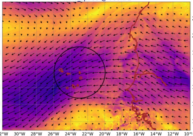
AROME25 20240702-12-UTC -ech(12h) wind_sp920 @ 920hPa
