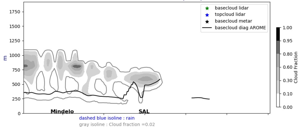
Cross section E/W @ 17.5N 20240703-12-UTC ech(36h)
