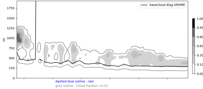
Cross section S/N @ -22W 20240702-12-UTC ech(12h)
