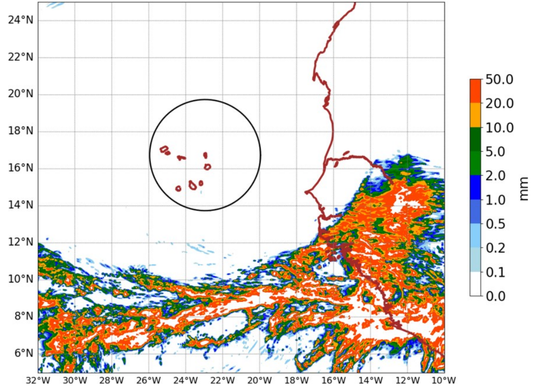
AROME25 20240702-00-UTC -ech(24h)
