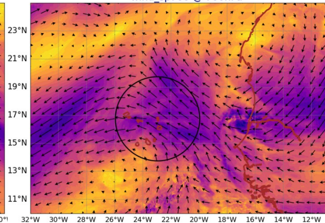
AROME25 20240703-12-UTC -ech(36h) wind_sp920 @ 920hPa
