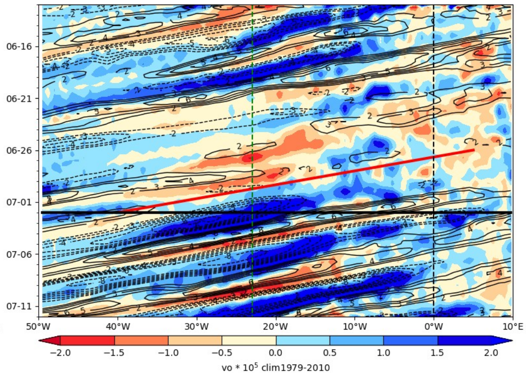
ECMWF Vorticity 850 hPa (color), V-700 hPa 2024-07-02
