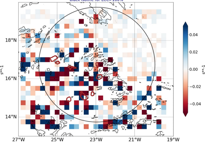
AROME25 regrid 0.25 20240704-12-UTC -ech(60h) blue for conv in subcloud layer black isoline for LCC>100%
