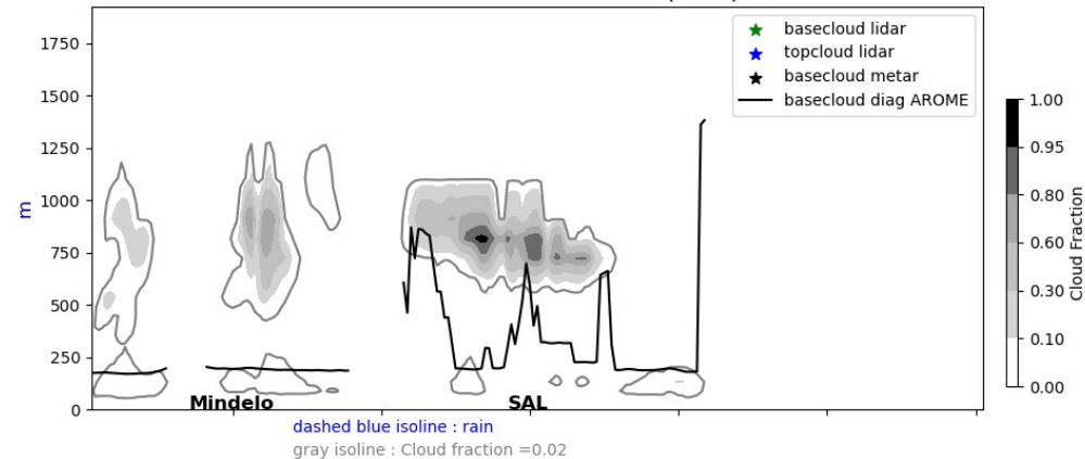
Cross section E/W @ 17.5N 20240704-12-UTC ech(60h)
