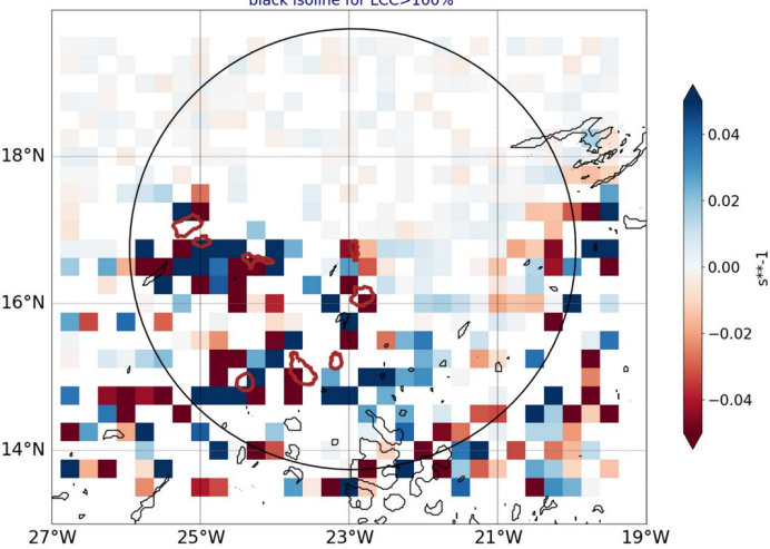
AROME25 regrid 0.25 20240702-12-UTC -ech(12h) blue for conv in subcloud layer black isoline for LCC>100%
