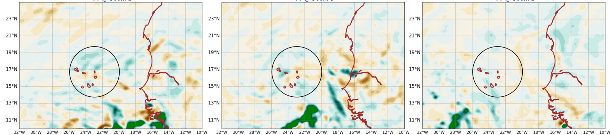
AROME25 20240702-12-UTC -ech(12h) VV @ 500hPa
