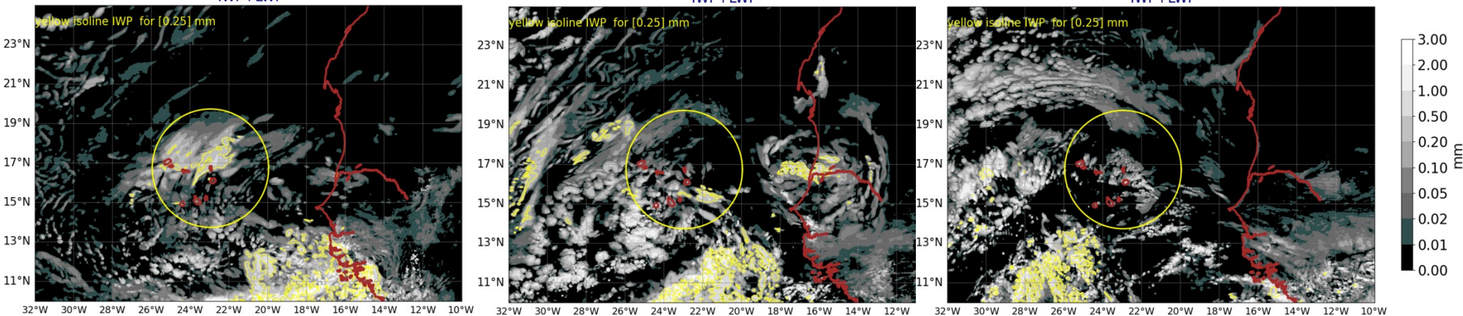
AROME25 20240702-12-UTC -ech(12h) IWP+LWP
