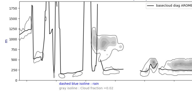
Cross section S/N @ -22W 20240703-12-UTC ech(36h)
