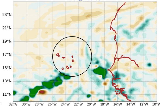
AROME25 20240708-12-UTC -ech(36h) VV @ 500hPa
