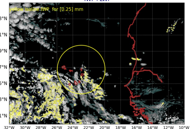
AROME25 20240709-12-UTC -ech(60h) IWP+LWP
