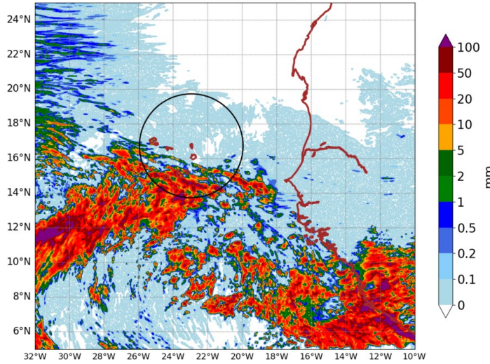
AROME25 20240709-12-UTC -ech(60h) RR cumulated over 24h
