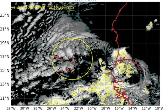
AROME25 20240707-12-UTC -ech(12h) IWP+LWP
