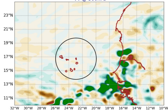
AROME25 20240707-12-UTC -ech(12h) VV @ 500hPa
