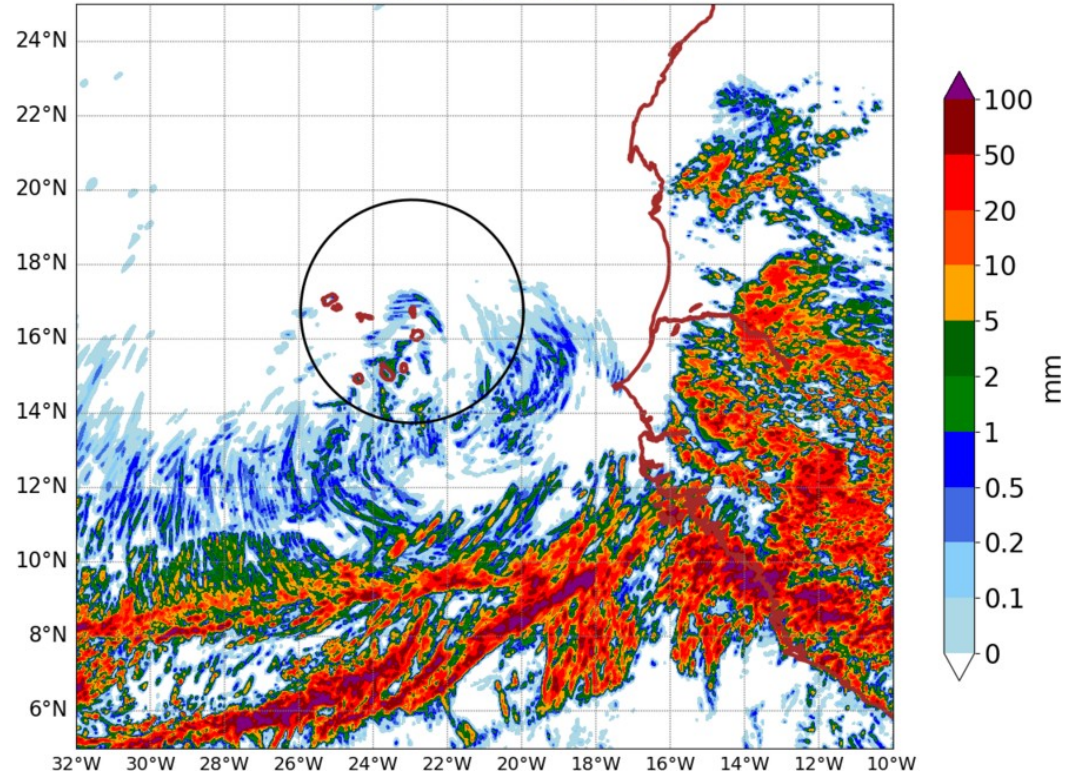
AROME25 20240707-00-UTC -ech(24h)
