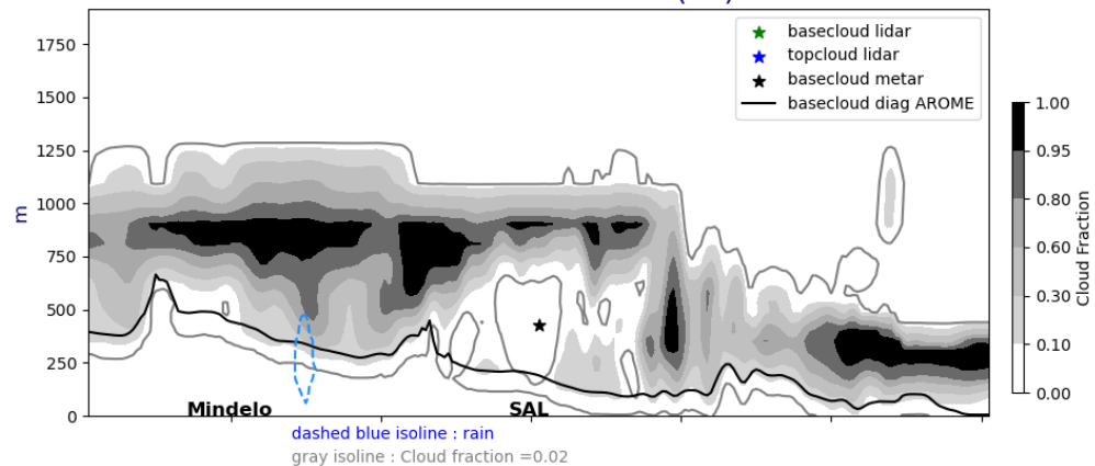
Cross section E/W @ 17.5N 20240707-01-UTC ech(1h)
