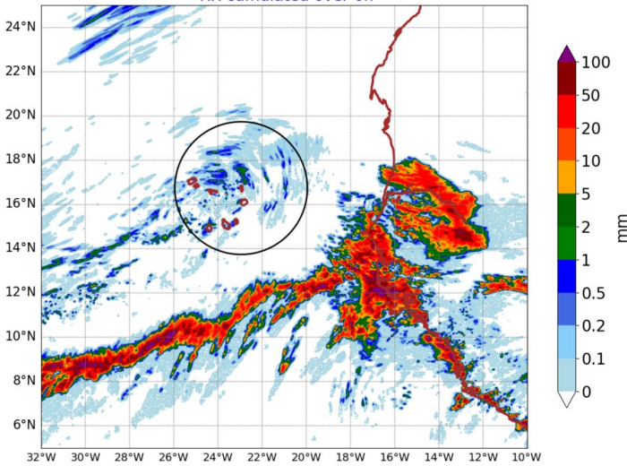
AROME25 20240707-15-UTC -ech(15h) RR cumulated over 6h
