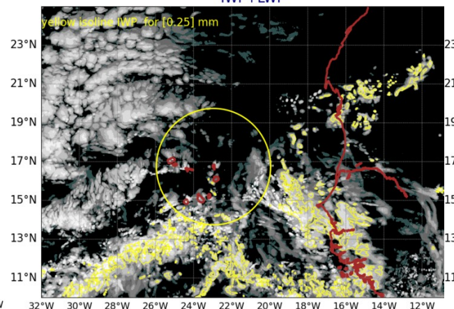
AROME25 20240708-12-UTC -ech(36h) IWP+LWP
