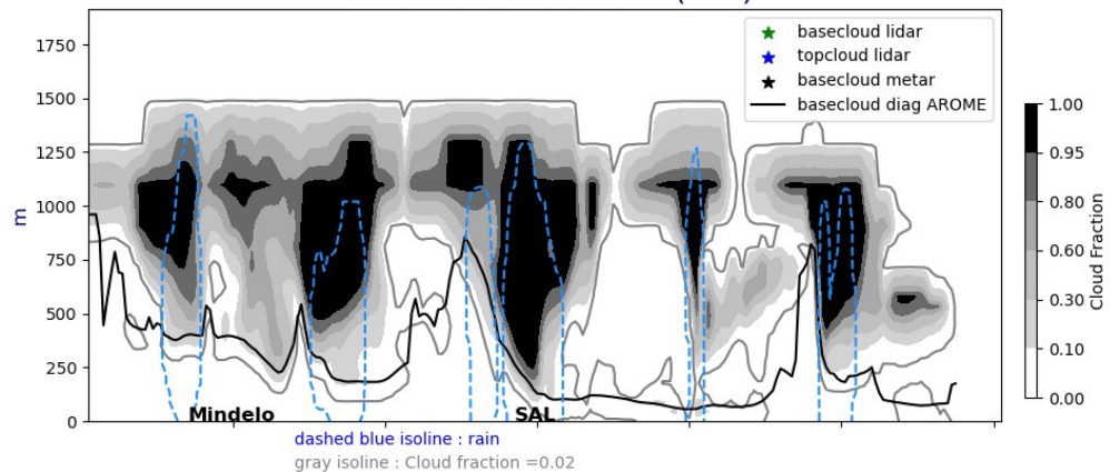
Cross section E/W @ 17.5N 20240707-12-UTC ech(12h)
