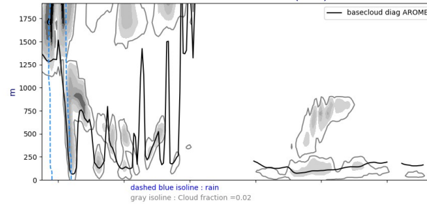
Cross section S/N @ -22W 20240708-12-UTC ech(36h)
