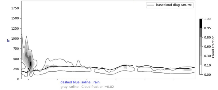
Cross section S/N @ -22W 20240709-12-UTC ech(60h)
