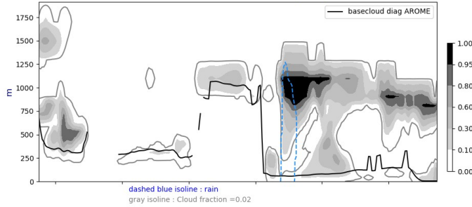
Cross section S/N @ -22W 20240707-12-UTC ech(12h)
