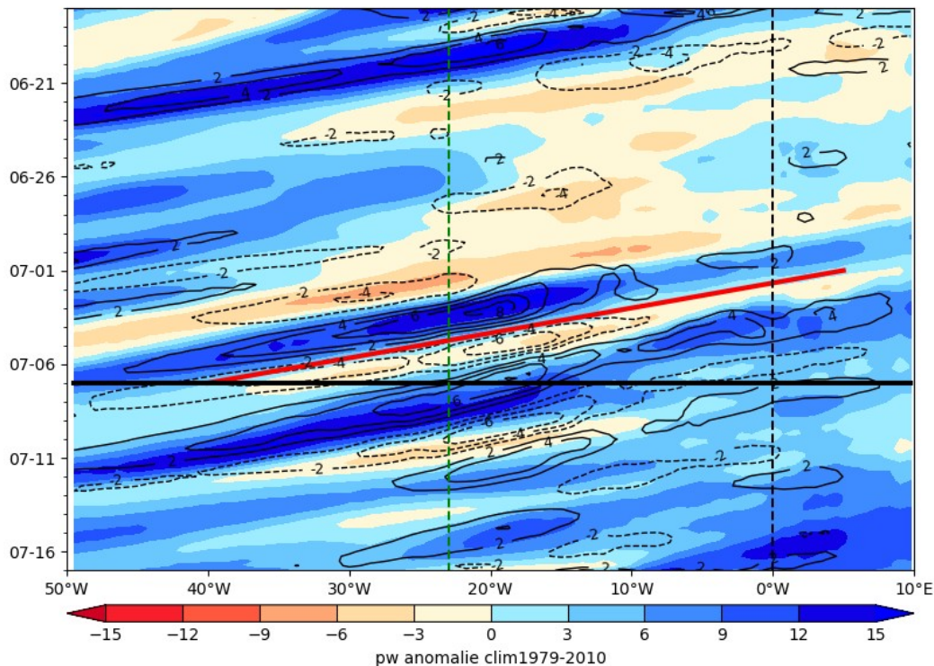
ECMWF PW (color) AND V at 925 hPa 2024-07-07
