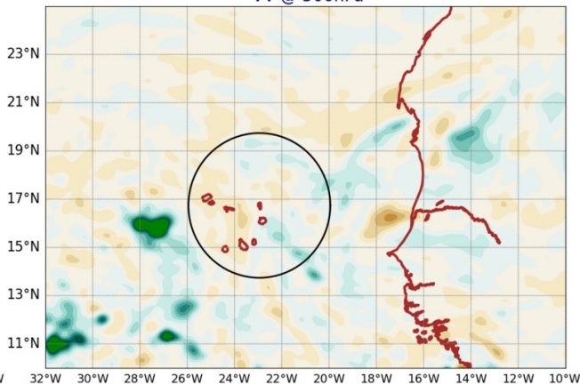
AROME25 20240709-12-UTC -ech(60h) VV @ 500hPa
