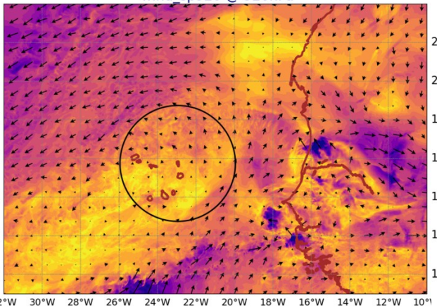
AROME25 20240707-12-UTC -ech(12h) wind_sp920 @ 920hPa
