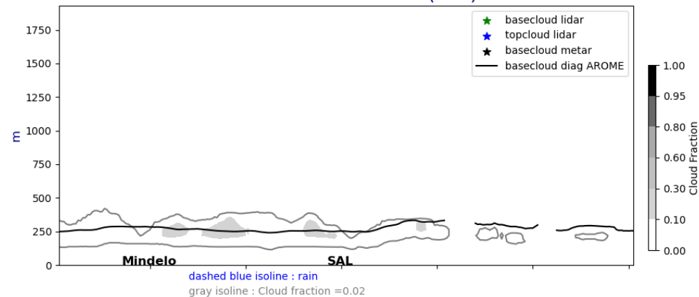
Cross section E/W @ 17.5N 20240709-12-UTC ech(60h)
