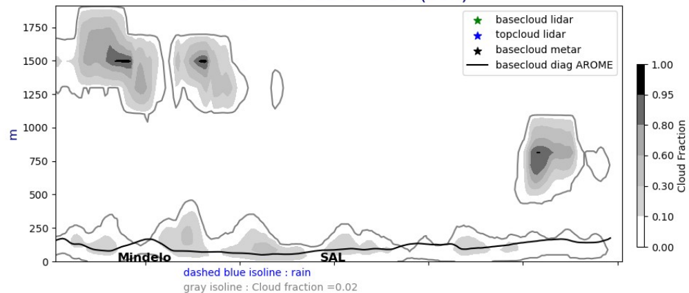
Cross section E/W @ 17.5N 20240708-12-UTC ech(36h)
