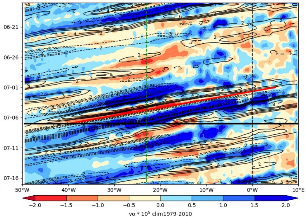
ECMWF Vorticity 850 hPa (color), V-700 hPa 2024-07-07
