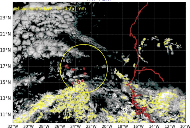
AROME25 20240708-12-UTC -ech(12h) IWP+LWP
