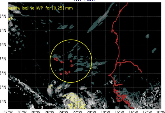
AROME25 20240710-12-UTC -ech(60h) IWP+LWP
