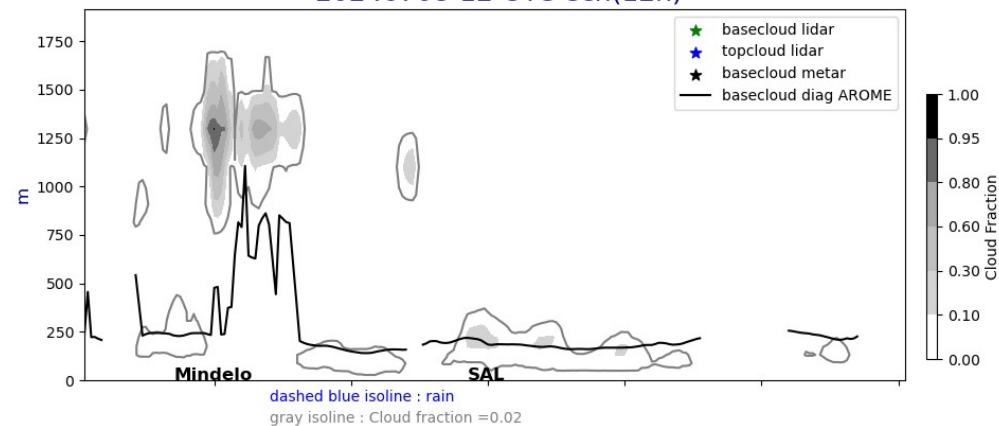
Cross section E/W @ 17.5N 20240708-12-UTC ech(12h)
