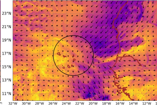
AROME25 20240709-12-UTC -ech(36h) wind_sp920 @ 920hPa
