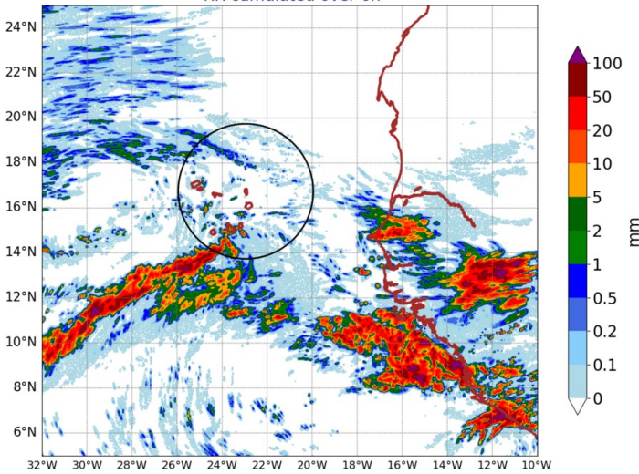
AROME25 20240708-15-UTC -ech(15h) RR cumulated over 6h
