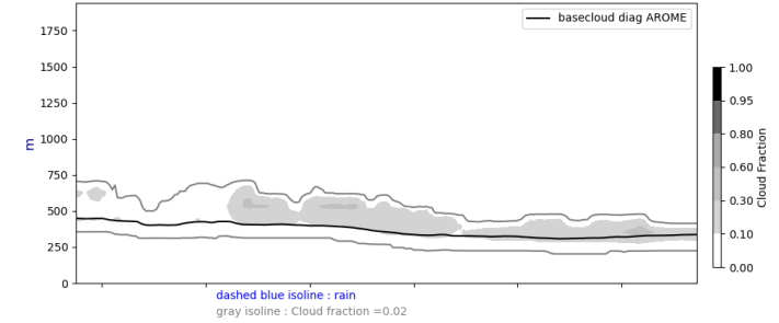
Cross section S/N @ -22W 20240710-12-UTC ech(60h)
