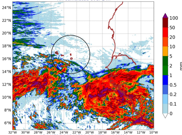
AROME25 20240710-12-UTC -ech(60h) RR cumulated over 24h
