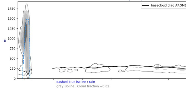
Cross section S/N @ -22W 20240709-12-UTC ech(36h)
