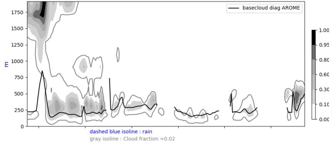
Cross section S/N @ -22W 20240708-12-UTC ech(12h)
