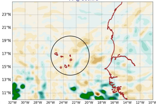
AROME25 20240709-12-UTC -ech(36h) VV @ 500hPa
