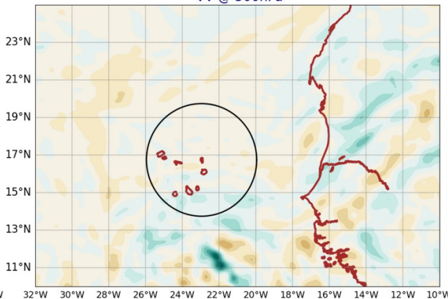
AROME25 20240710-12-UTC -ech(60h) VV @ 500hPa
