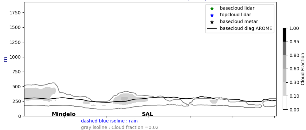
Cross section E/W @ 17.5N 20240709-12-UTC ech(36h)
