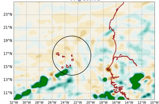
AROME25 20240708-12-UTC -ech(12h) VV @ 500hPa
