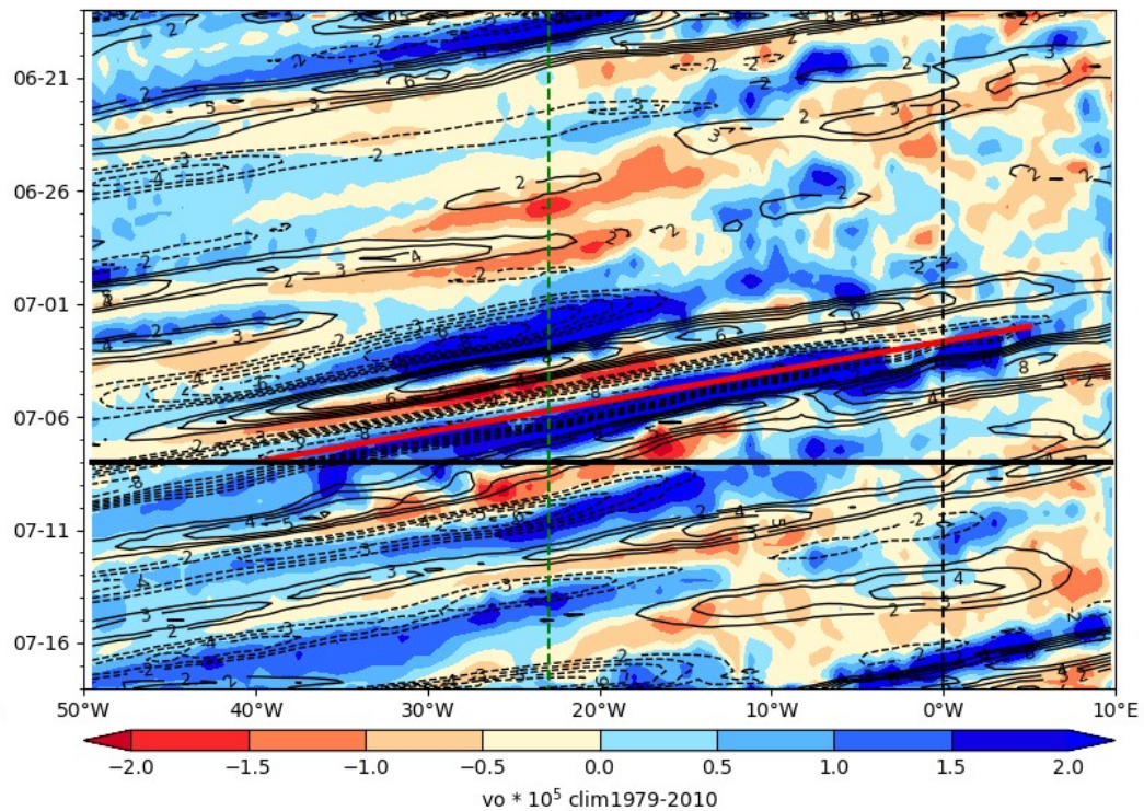
ECMWF Vorticity 850 hPa (color), V-700 hPa 2024-07-08
