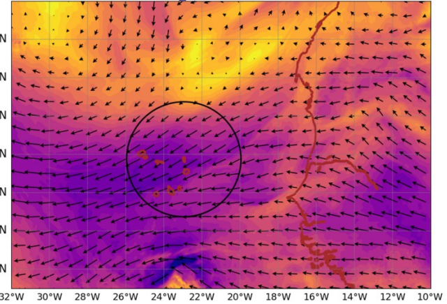
AROME25 20240710-12-UTC -ech(60h) wind_sp920 @ 920hPa
