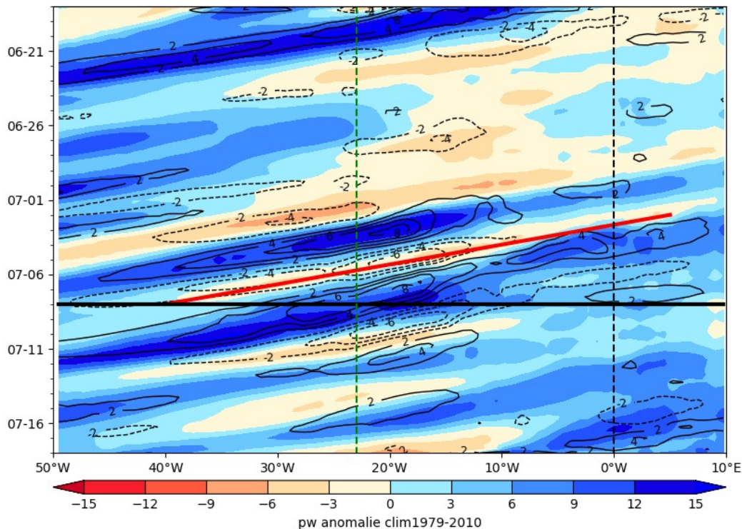
ECMWF PW (color) AND V at 925 hPa 2024-07-08
