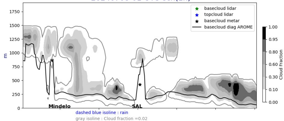
Cross section E/W @ 17.5N 20240708-01-UTC ech(1h)
