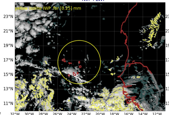
AROME25 20240709-12-UTC -ech(36h) IWP+LWP
