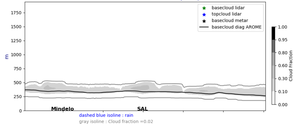
Cross section E/W @ 17.5N 20240710-12-UTC ech(60h)
