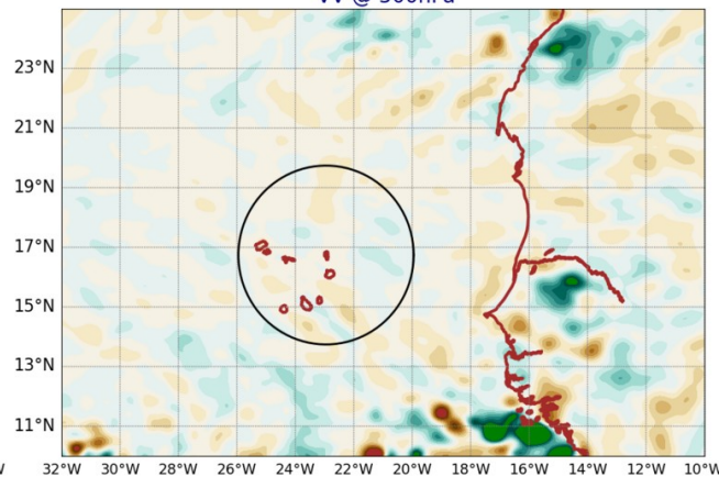
AROME25 20240715-12-UTC -ech(36h) VV @ 500hPa
