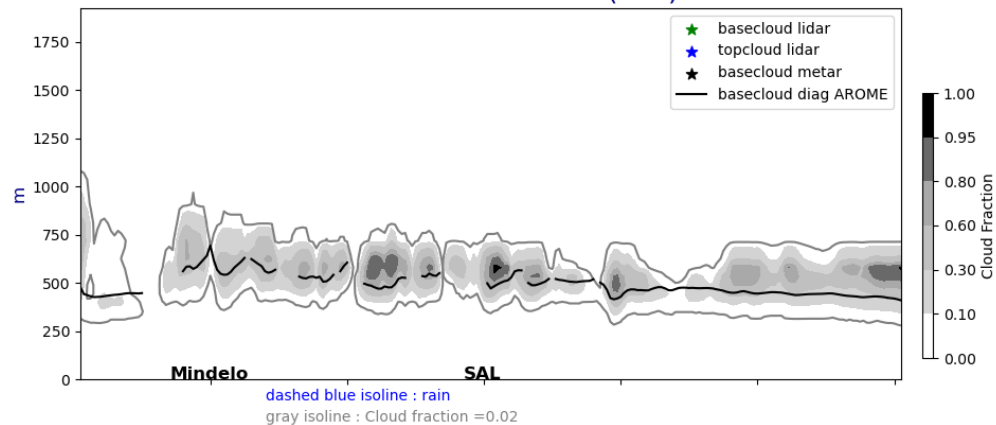
Cross section E/W @ 17.5N 20240715-12-UTC ech(36h)
