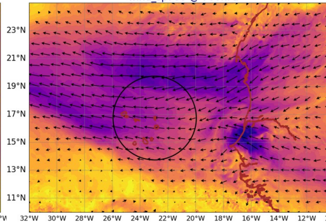
AROME25 20240715-12-UTC -ech(36h) wind_sp920 @ 920hPa
