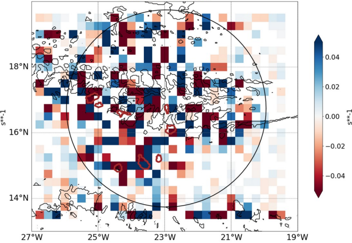
AROME25 regrid 0.25 20240716-12-UTC -ech(60h) blue for conv in subcloud layer black isoline for LCC>100%
