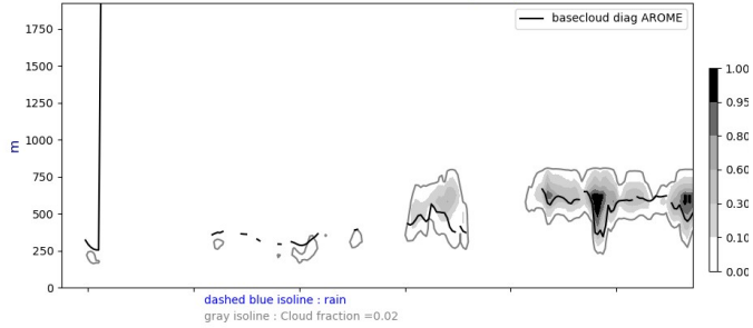
Cross section S/N @ -22W 20240714-12-UTC ech(12h)
