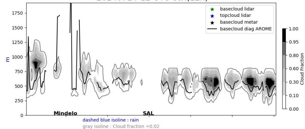
Cross section E/W @ 17.5N 20240714-12-UTC ech(12h)
