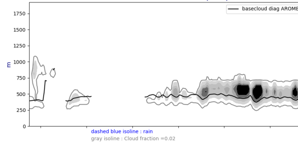
Cross section S/N @ -22W 20240715-12-UTC ech(36h)
