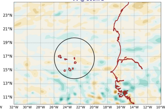
AROME25 20240716-12-UTC -ech(60h) VV @ 500hPa
