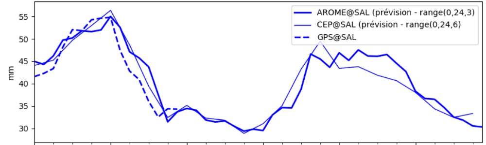
PW AROME & CEP (fct 0-23h) vs GPS 20240708 -20240713
