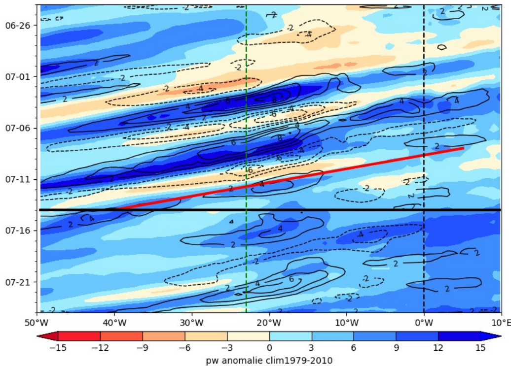
ECMWF PW (color) AND V at 925 hPa 2024-07-14
