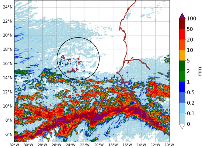
AROME25 20240716-12-UTC -ech(60h) RR cumulated over 24h
