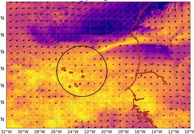
AROME25 20240716-12-UTC -ech(60h) wind_sp920 @ 920hPa
