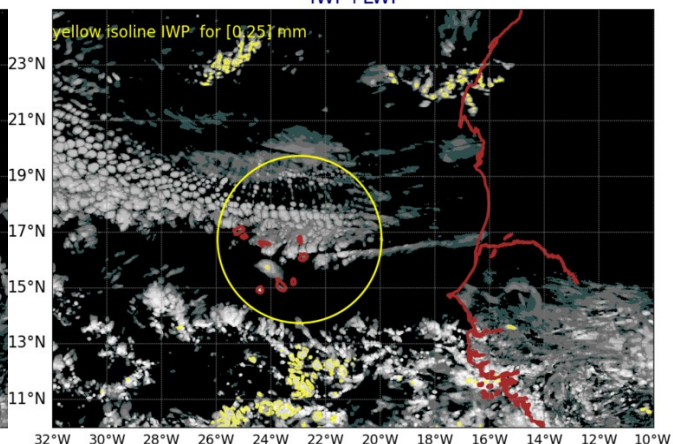
AROME25 20240716-12-UTC -ech(60h) IWP+LWP
