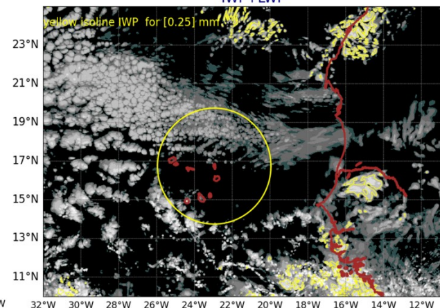
AROME25 20240715-12-UTC -ech(36h) IWP+LWP
