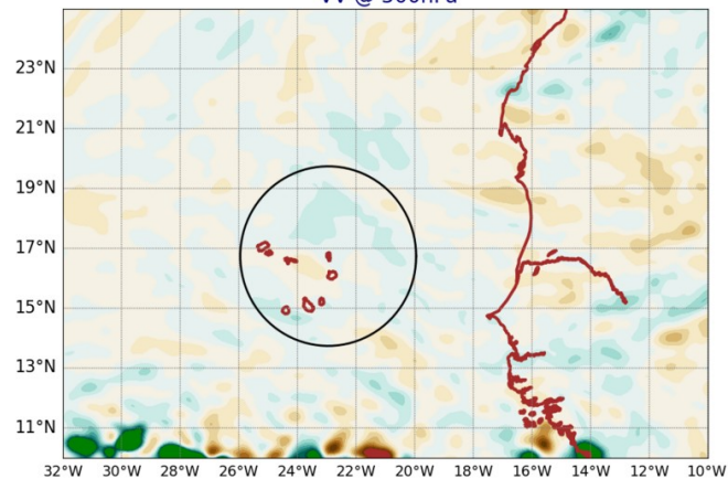
AROME25 20240714-12-UTC -ech(12h) VV @ 500hPa
