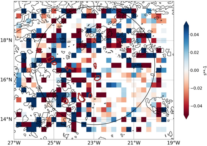
AROME25 regrid 0.25 20240714-12-UTC -ech(12h) blue for conv in subcloud layer black isoline for LCC>100%
