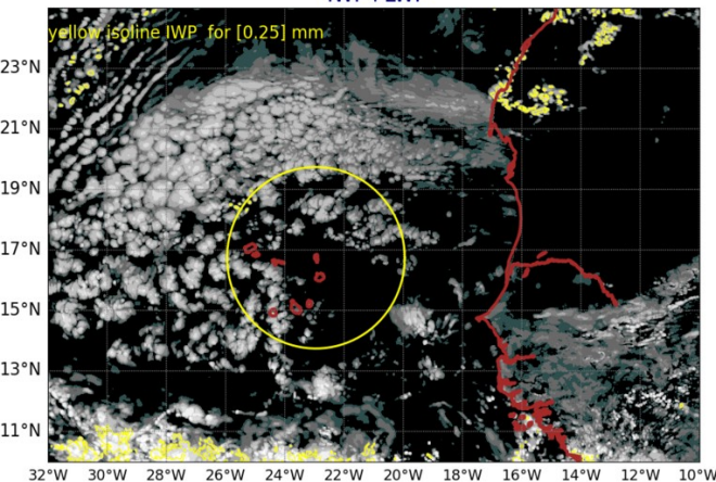
AROME25 20240714-12-UTC -ech(12h) IWP+LWP
