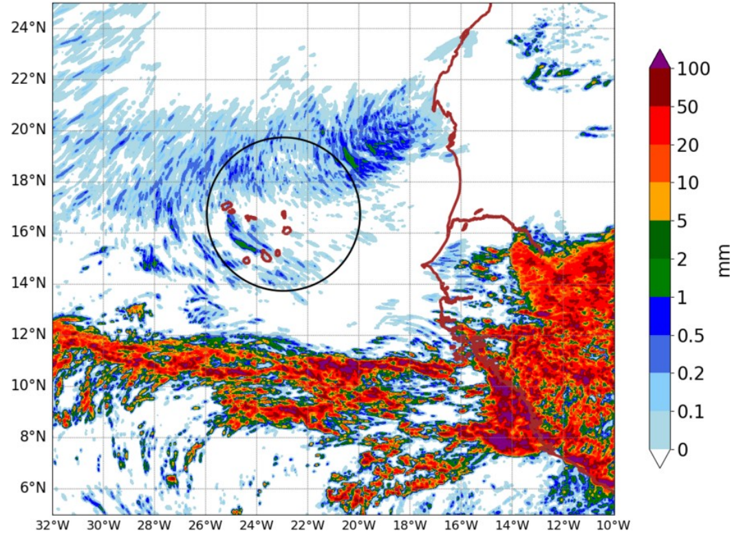
AROME25 20240714-00-UTC -ech(24h)
