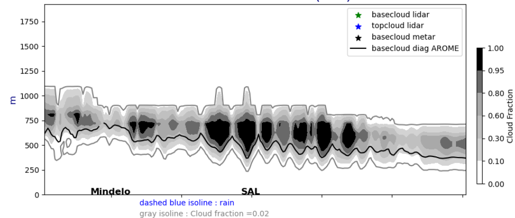
Cross section E/W @ 17.5N 20240716-12-UTC ech(60h)
