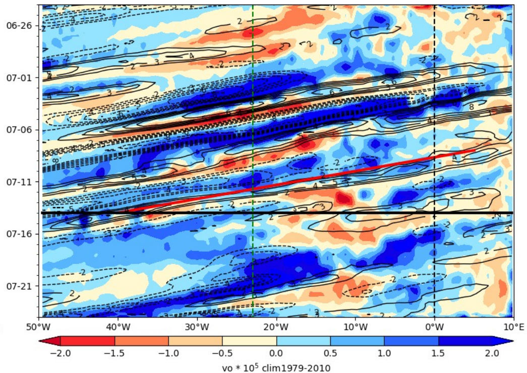
ECMWF Vorticity 850 hPa (color), V-700 hPa 2024-07-14
