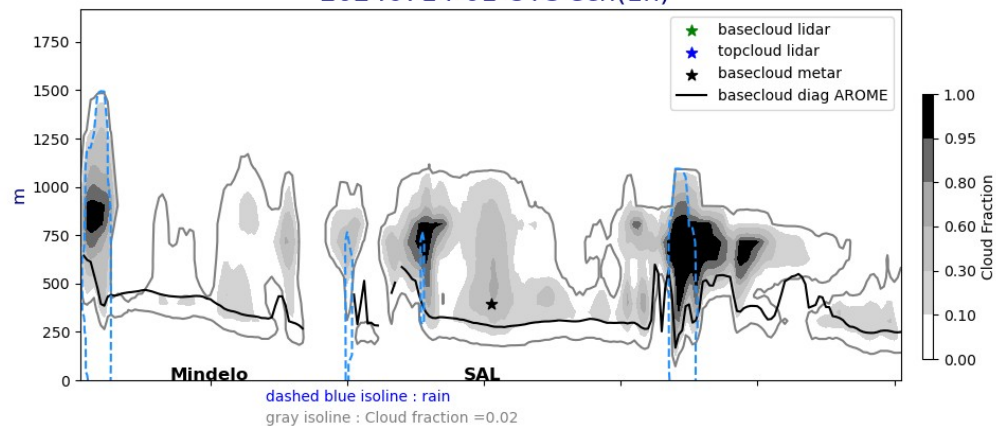
Cross section E/W @ 17.5N 20240714-01-UTC ech(1h)
