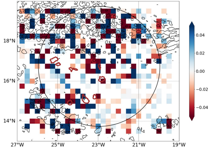
AROME25 regrid 0.25 20240715-12-UTC -ech(36h) blue for conv in subcloud layer black isoline for LCC>100%
