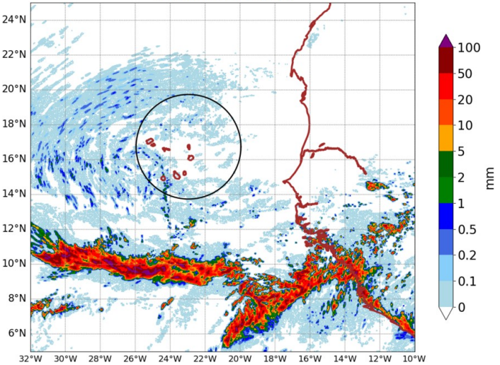
AROME25 20240714-15-UTC -ech(15h) RR cumulated over 6h
