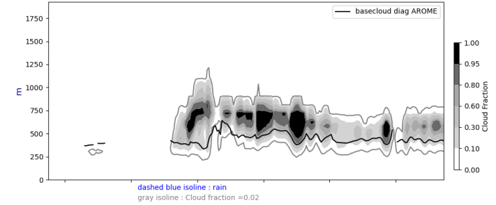
Cross section S/N @ -22W 20240716-12-UTC ech(60h)
