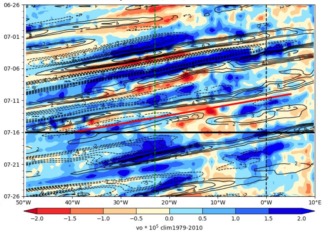
ECMWF Vorticity 850 hPa (color), V-700 hPa 2024-07-16
