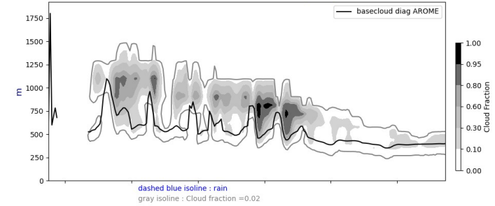
Cross section S/N @ -22W 20240718-12-UTC ech(60h)
