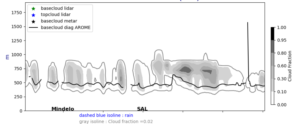
Cross section E/W @ 17.5N 20240718-12-UTC ech(60h)
