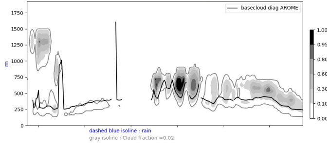
Cross section S/N @ -22W 20240716-12-UTC ech(12h)
