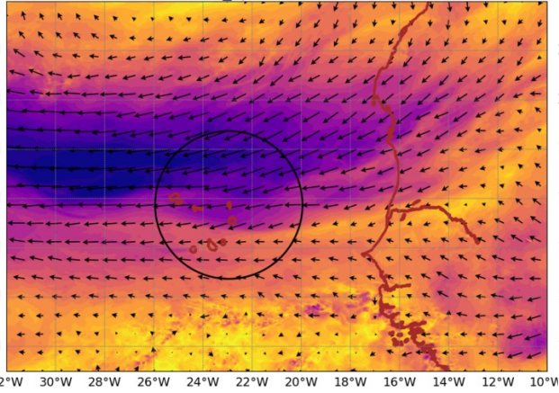
AROME25 20240716-12-UTC -ech(12h) wind_sp920 @ 920hPa
