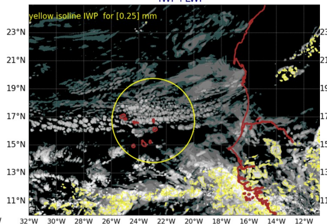
AROME25 20240717-12-UTC -ech(36h) IWP+LWP
