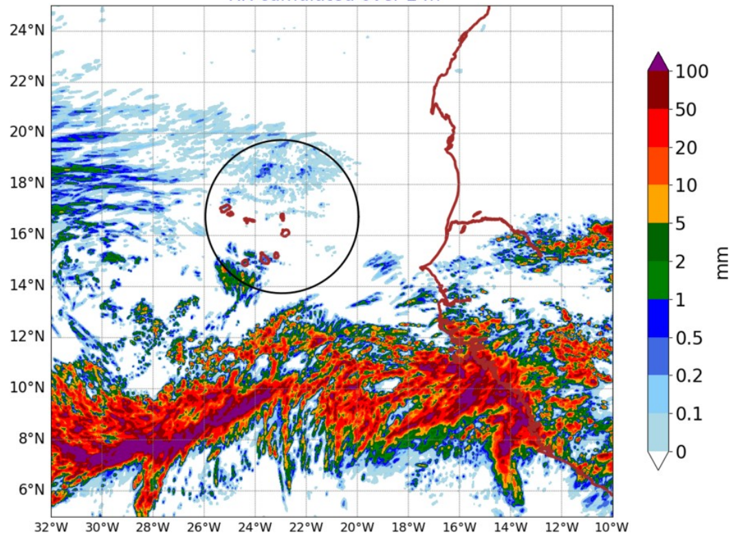
AROME25 20240716-00-UTC -ech(24h) RR cumulated over 24h
