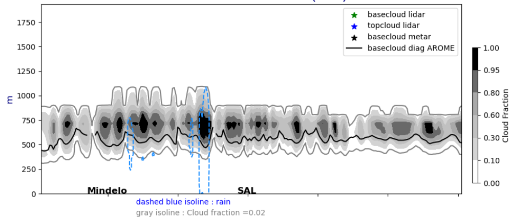
Cross section E/W @ 17.5N 20240717-12-UTC ech(36h)
