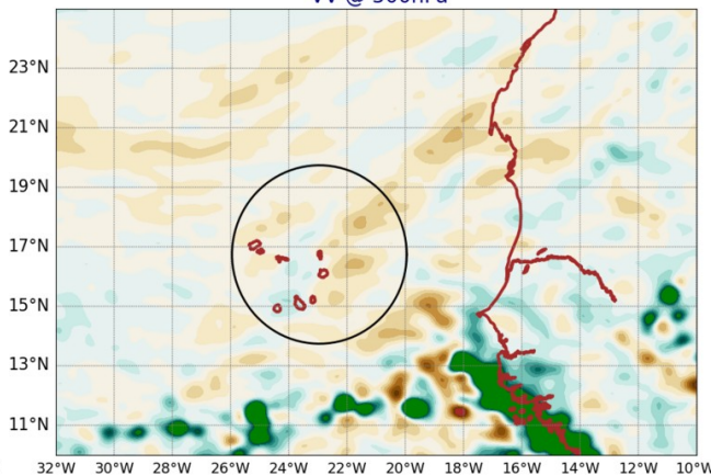
AROME25 20240717-12-UTC -ech(36h) VV @ 500hPa
