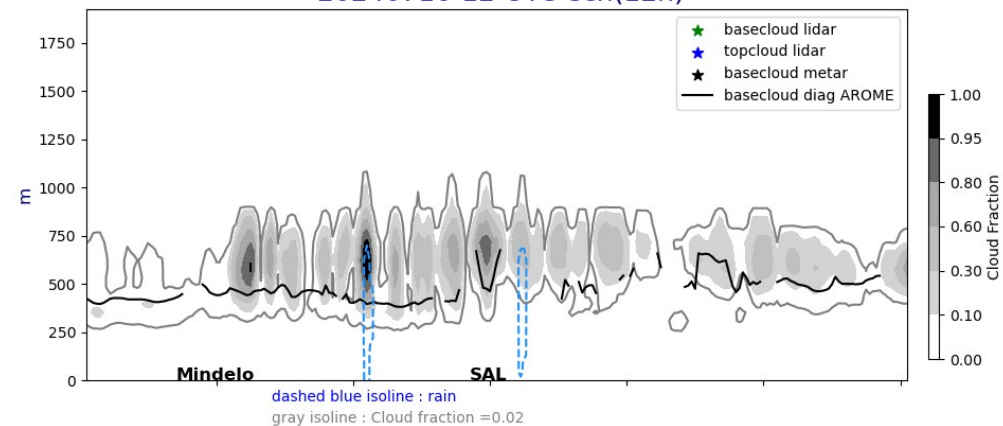
Cross section E/W @ 17.5N 20240716-12-UTC ech(12h)
