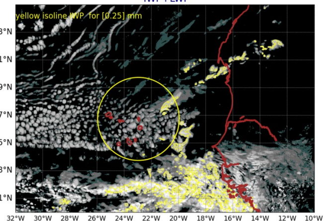
AROME25 20240718-12-UTC -ech(60h) IWP+LWP
