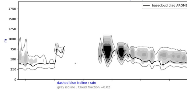
Cross section S/N @ -22W 20240717-12-UTC ech(36h)
