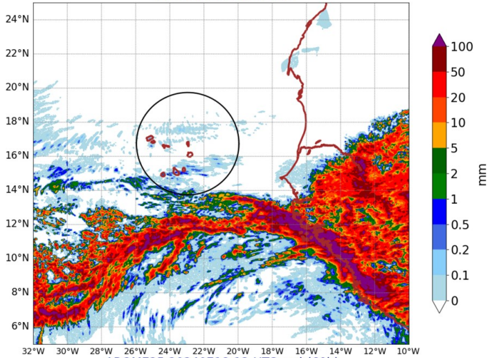
AROME25 20240718-12-UTC -ech(60h) RR cumulated over 24h
