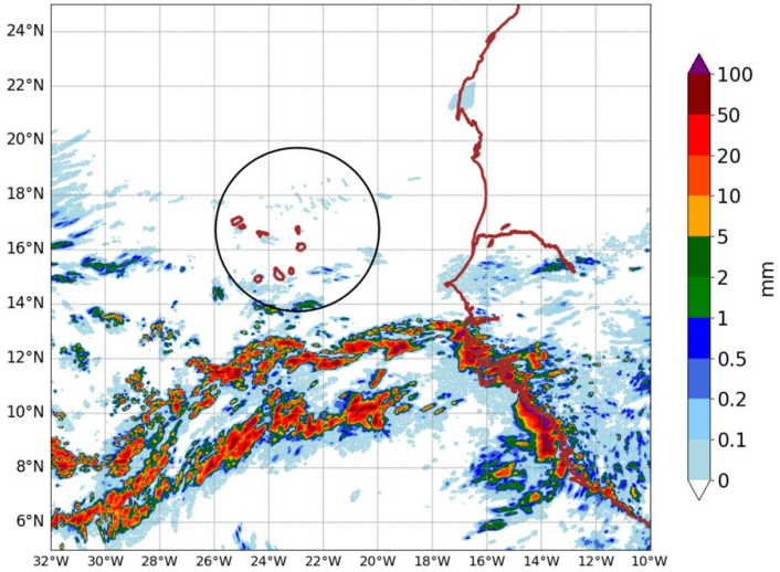
AROME25 20240716-15-UTC -ech(15h) RR cumulated over 6h
