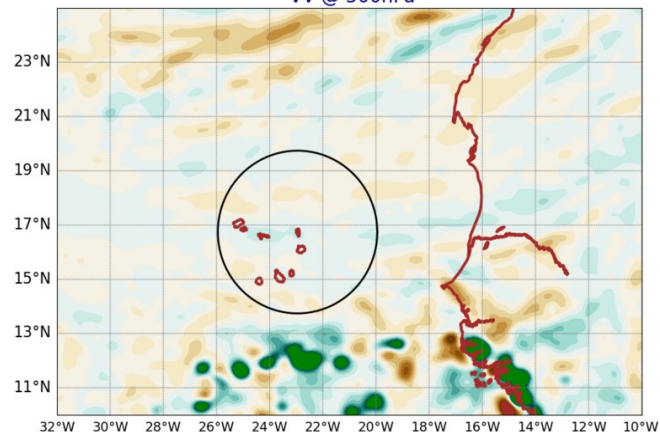
AROME25 20240716-12-UTC -ech(12h) VV @ 500hPa
