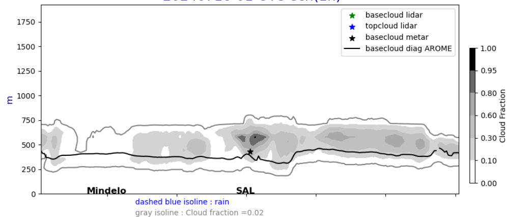
Cross section E/W @ 17.5N 20240716-01-UTC ech(1h)
