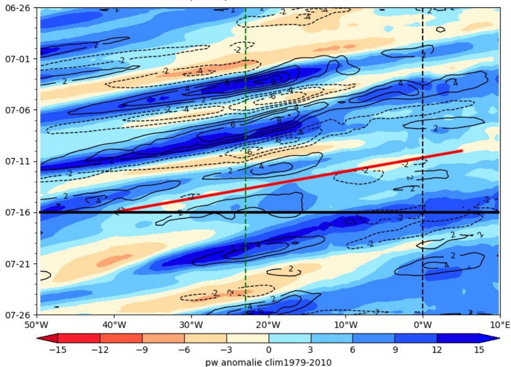
ECMWF PW (color) AND V at 925 hPa 2024-07-16
