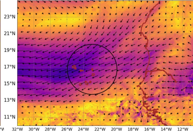
AROME25 20240717-12-UTC -ech(36h) wind_sp920 @ 920hPa
