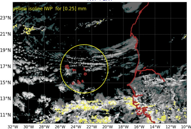
AROME25 20240716-12-UTC -ech(12h) IWP+LWP
