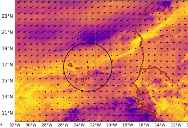
AROME25 20240717-12-UTC -ech(36h) wind_sp920 @ 920hPa
