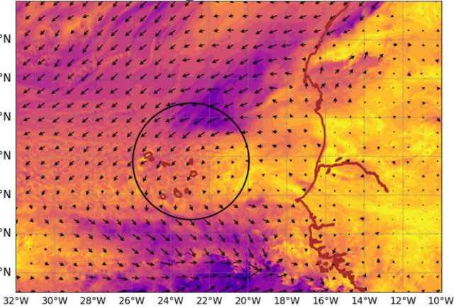
AROME25 20240718-12-UTC -ech(60h) wind_sp920 @ 920hPa
