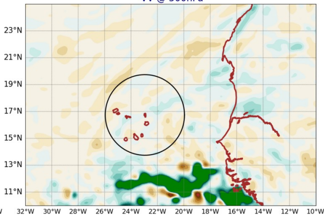
AROME25 20240718-12-UTC -ech(60h) VV @ 500hPa
