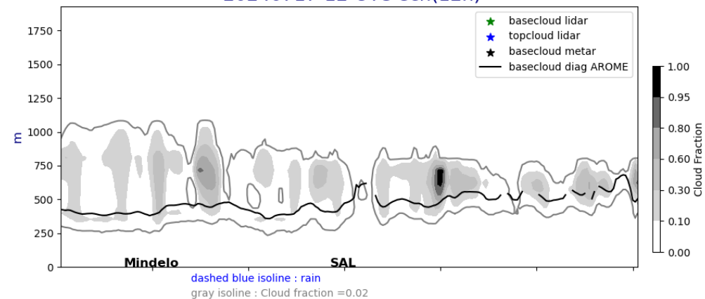
Cross section E/W @ 17.5N 20240717-12-UTC ech(12h)
