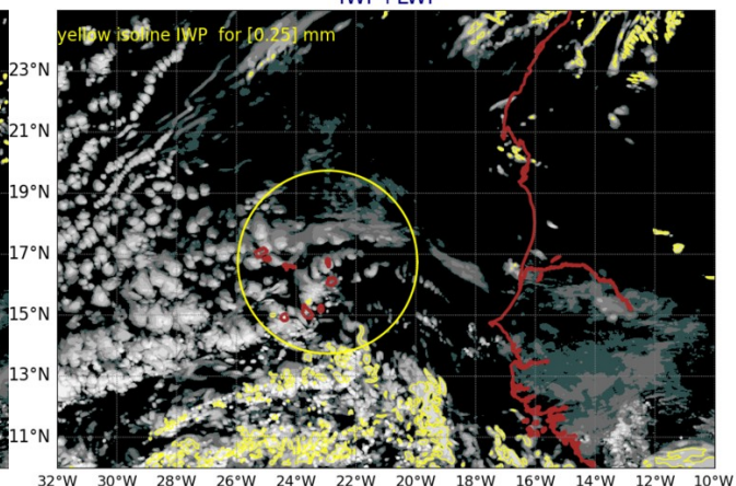
AROME25 20240719-12-UTC -ech(60h) IWP+LWP
