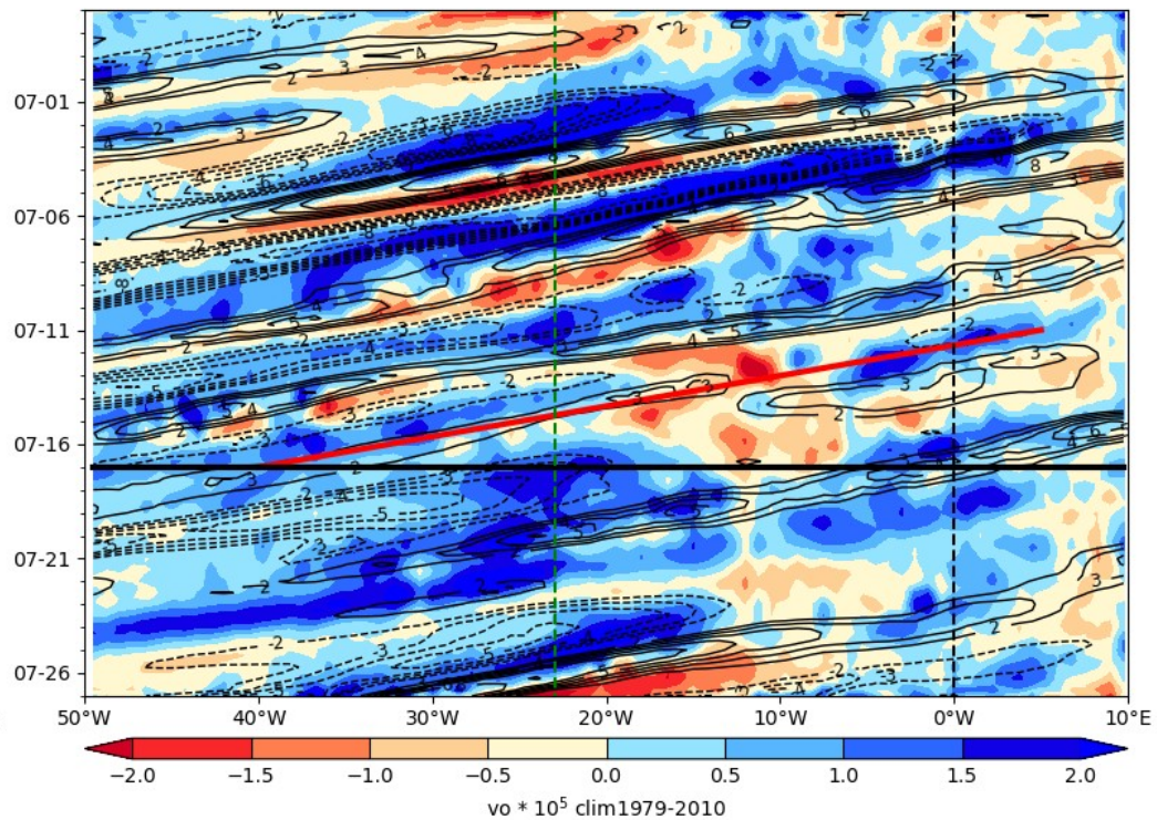
ECMWF Vorticity 850 hPa (color), V-700 hPa 2024-07-17
