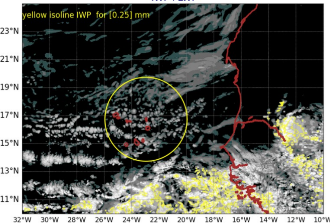
AROME25 20240717-12-UTC -ech(12h) IWP+LWP
