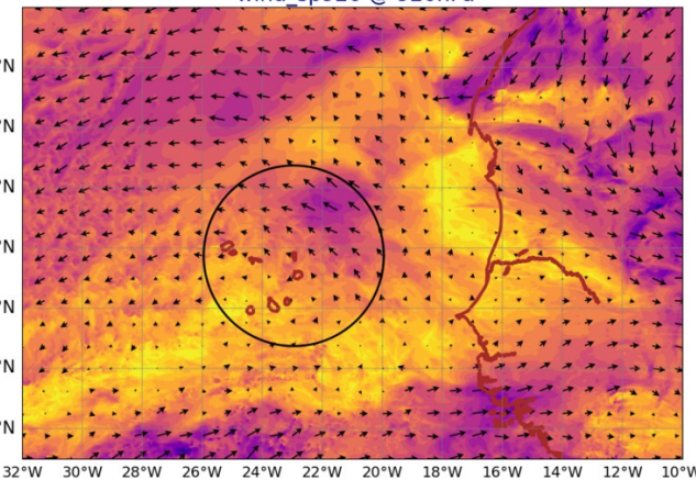
AROME25 20240719-12-UTC -ech(60h) wind_sp920 @ 920hPa
