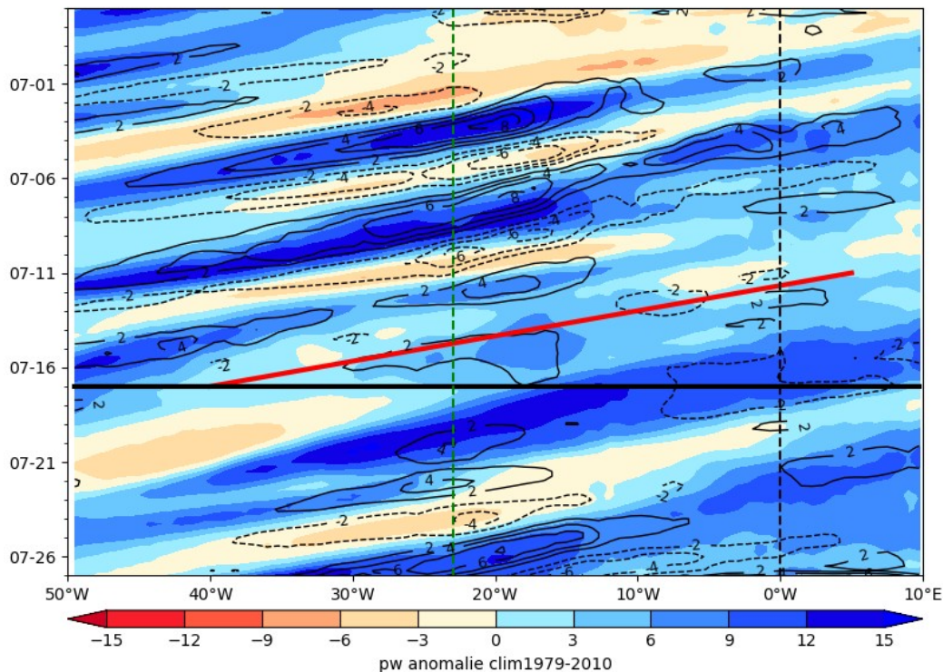
ECMWF PW (color) AND V at 925 hPa 2024-07-17
