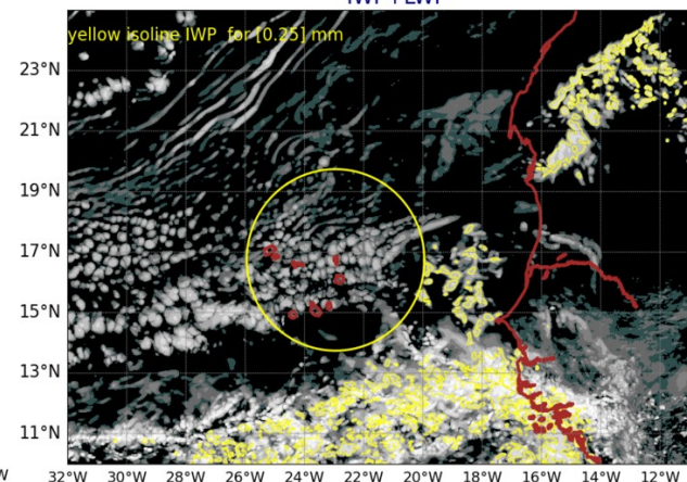
AROME25 20240718-12-UTC -ech(36h) IWP+LWP
