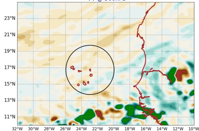
AROME25 20240717-12-UTC -ech(12h) VV @ 500hPa
