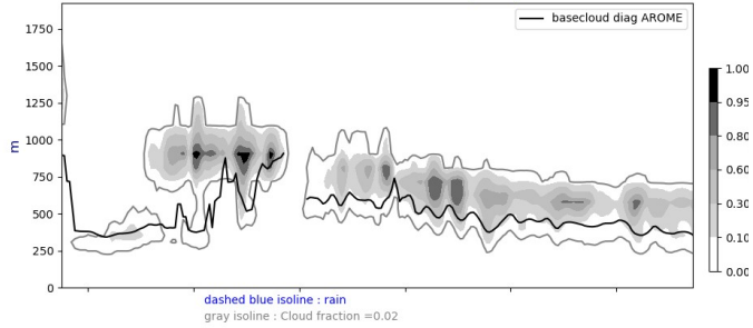
Cross section S/N @ -22W 20240717-12-UTC ech(12h)
