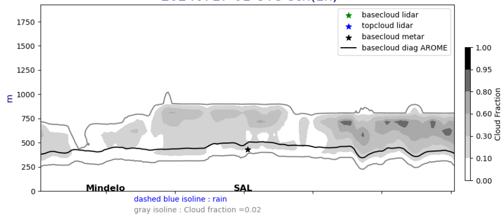
Cross section E/W @ 17.5N 20240717-01-UTC ech(1h)
