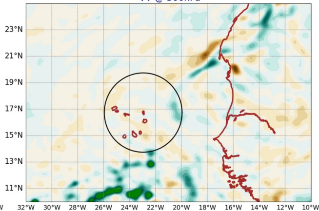
AROME25 20240719-12-UTC -ech(60h) VV @ 500hPa
