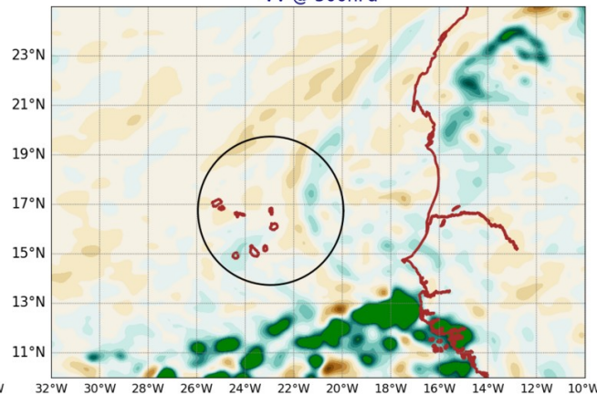
AROME25 20240718-12-UTC -ech(36h) VV @ 500hPa
