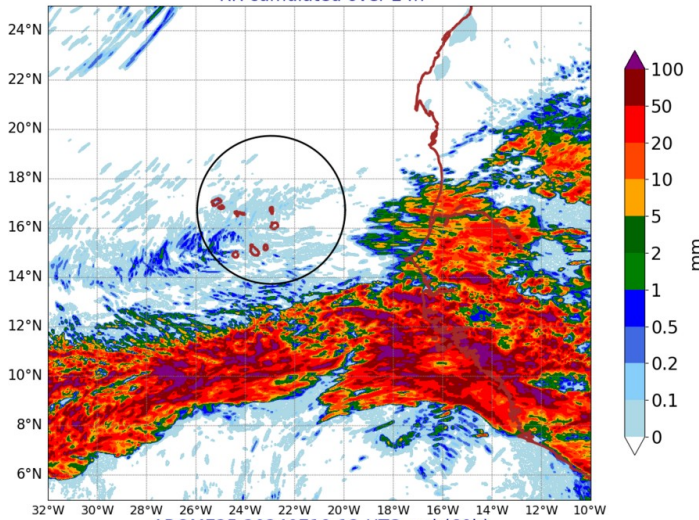
AROME25 20240719-12-UTC -ech(60h) RR cumulated over 24h
