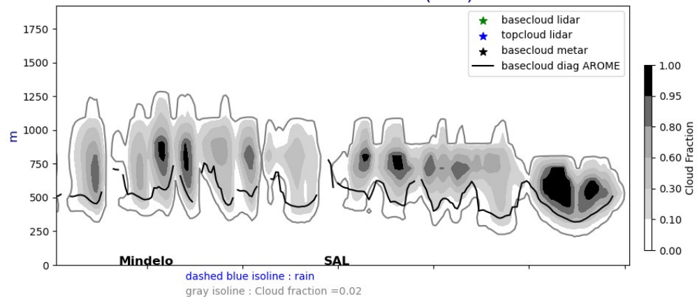
Cross section E/W @ 17.5N 20240718-12-UTC ech(36h)
