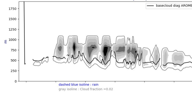
Cross section S/N @ -22W 20240718-12-UTC ech(36h)
