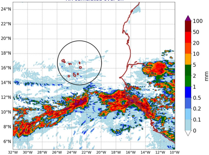
AROME25 20240717-15-UTC -ech(15h) RR cumulated over 6h
