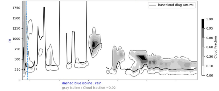
Cross section S/N @ -22W 20240719-12-UTC ech(60h)
