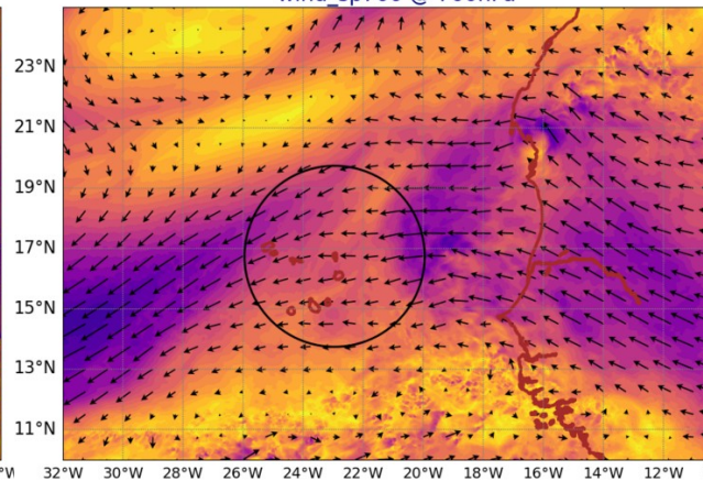
AROME25 20240718-12-UTC -ech(36h) wind_sp920 @ 920hPa
