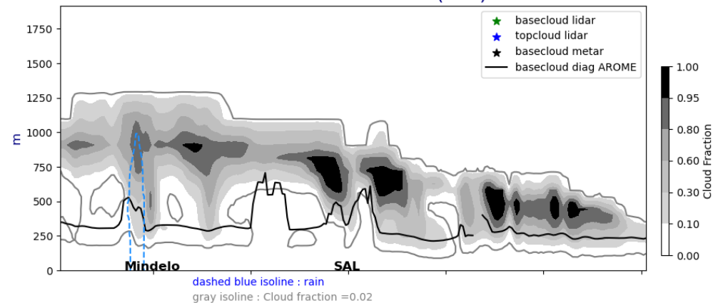
Cross section E/W @ 17.5N 20240719-12-UTC ech(60h)
