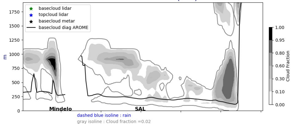
Cross section E/W @ 17.5N 20240719-12-UTC ech(36h)
