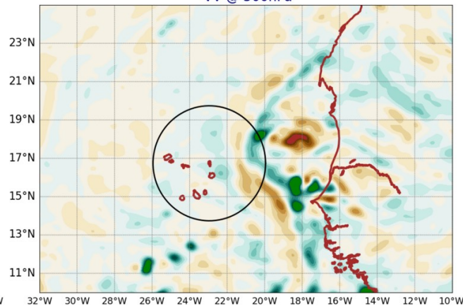
AROME25 20240719-12-UTC -ech(36h) VV @ 500hPa
