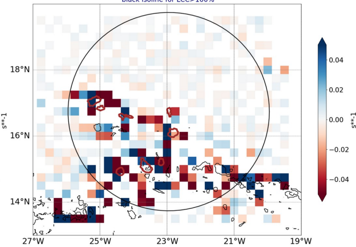
AROME25 regrid 0.25 20240720-12-UTC -ech(60h) blue for conv in subcloud layer black isoline for LCC>100%
