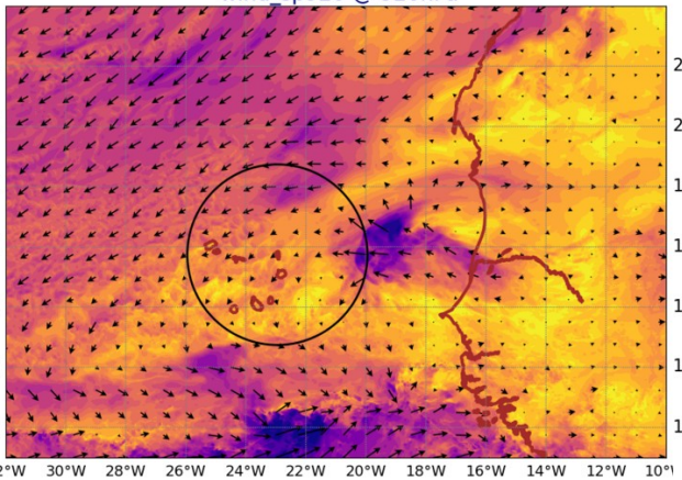
AROME25 20240718-12-UTC -ech(12h) wind_sp920 @ 920hPa
