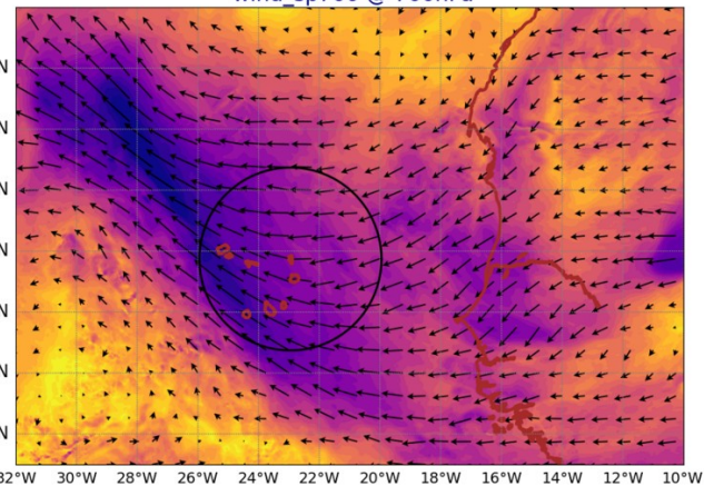
AROME25 20240720-12-UTC -ech(60h) wind_sp920 @ 920hPa
