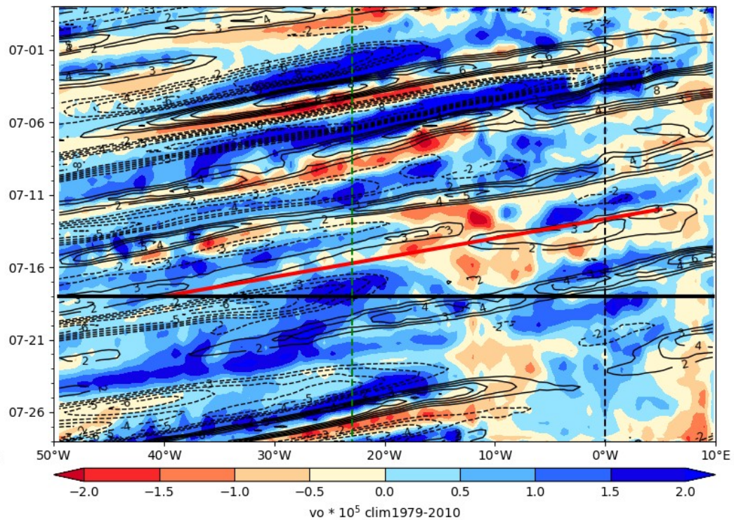
ECMWF Vorticity 850 hPa (color), V-700 hPa 2024-07-18
