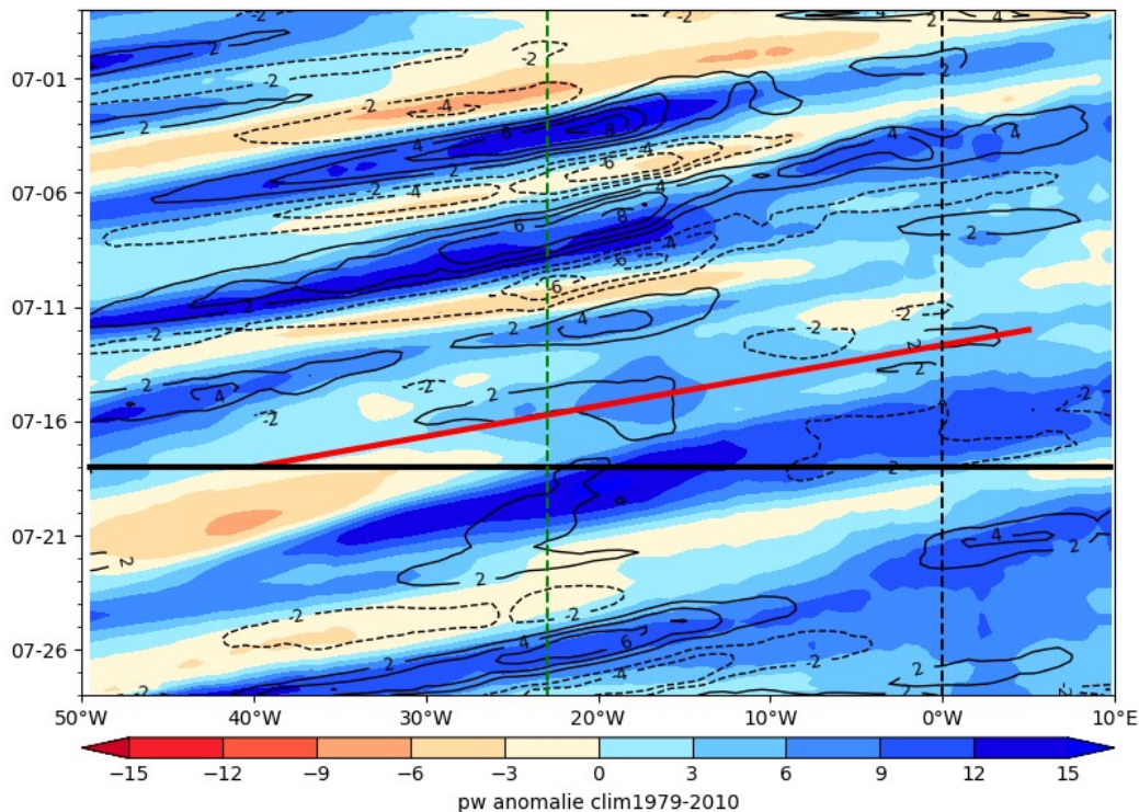
ECMWF PW (color) AND V at 925 hPa 2024-07-18
