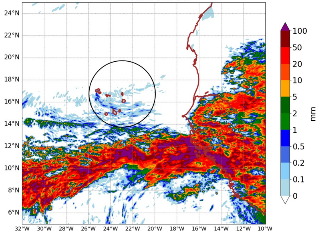
AROME25 20240718-00-UTC -ech(24h) RR cumulated over 24h
