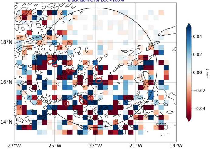
AROME25 regrid 0.25 20240718-12-UTC -ech(12h) blue for conv in subcloud layer black isoline for LCC>100%
