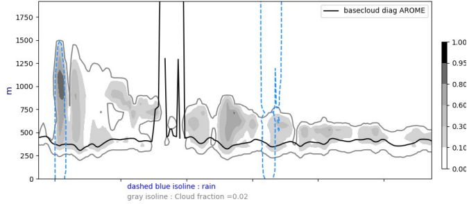
Cross section S/N @ -22W 20240718-12-UTC ech(12h)
