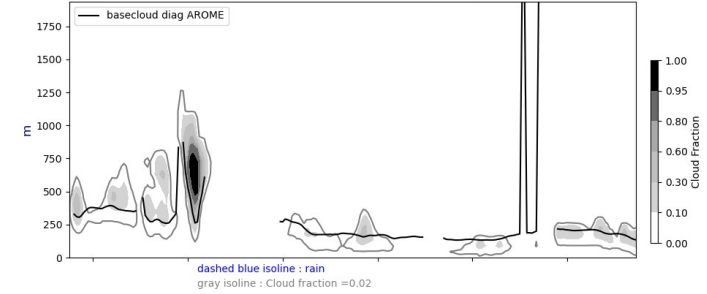
Cross section S/N @ -22W 20240720-12-UTC ech(60h)
