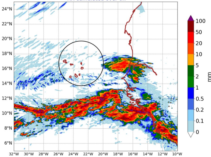
AROME25 20240718-15-UTC -ech(15h) RR cumulated over 6h
