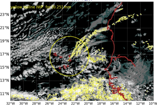
AROME25 20240718-12-UTC -ech(12h) IWP+LWP
