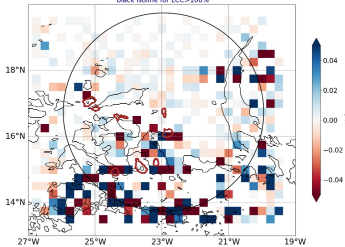
AROME25 regrid 0.25 20240719-12-UTC -ech(36h) blue for conv in subcloud layer black isoline for LCC>100%
