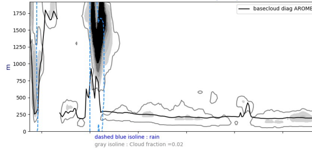
Cross section S/N @ -22W 20240719-12-UTC ech(36h)
