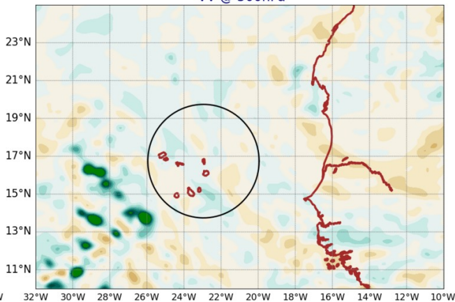
AROME25 20240720-12-UTC -ech(60h) VV @ 500hPa
