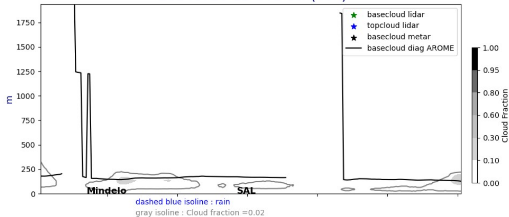
Cross section E/W @ 17.5N 20240720-12-UTC ech(60h)
