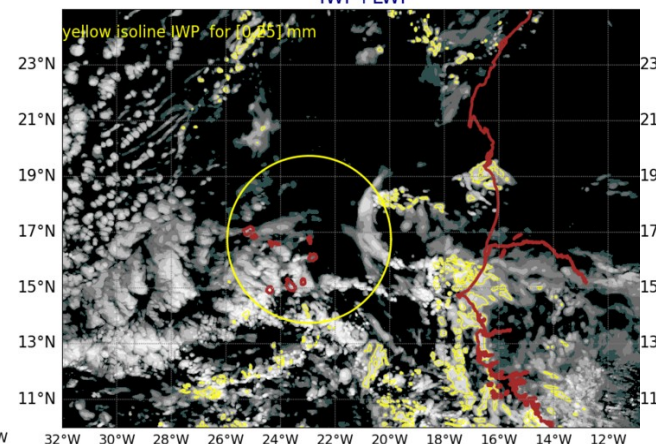
AROME25 20240719-12-UTC -ech(36h) IWP+LWP
