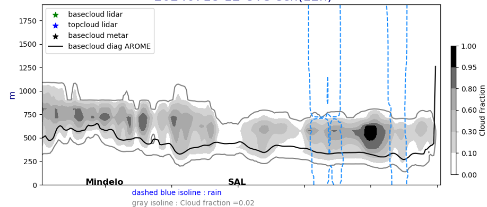
Cross section E/W @ 17.5N 20240718-12-UTC ech(12h)
