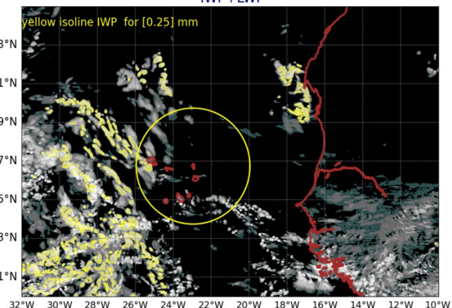
AROME25 20240720-12-UTC -ech(60h) IWP+LWP
