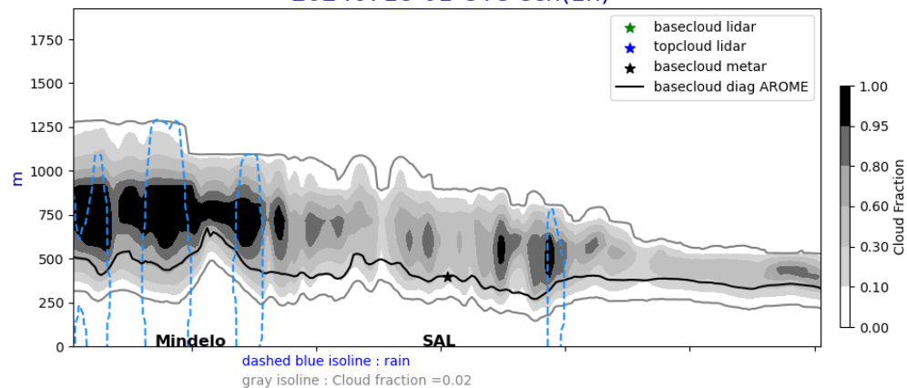
Cross section E/W @ 17.5N 20240718-01-UTC ech(1h)
