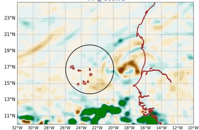
AROME25 20240718-12-UTC -ech(12h) VV @ 500hPa
