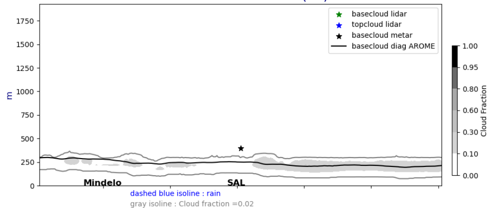
Cross section E/W @ 17.5N 20240720-01-UTC ech(1h)
