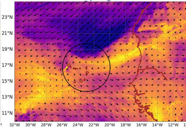
AROME25 20240721-12-UTC -ech(36h) wind_sp920 @ 920hPa
