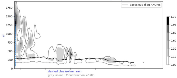
Cross section S/N @ -22W 20240720-12-UTC ech(12h)
