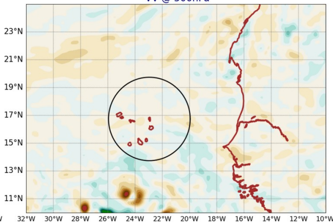
AROME25 20240722-12-UTC -ech(60h) VV @ 500hPa
