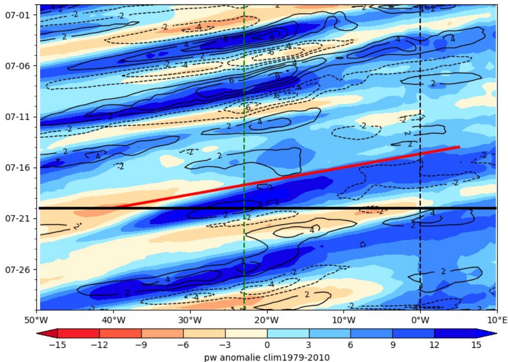
ECMWF PW (color) AND V at 925 hPa 2024-07-20
