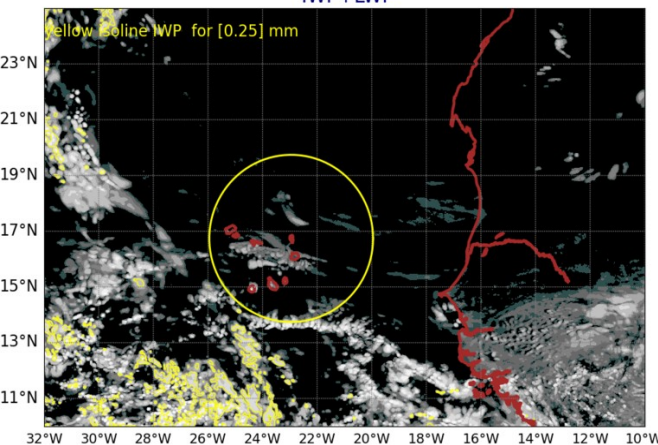
AROME25 20240720-12-UTC -ech(12h) IWP+LWP
