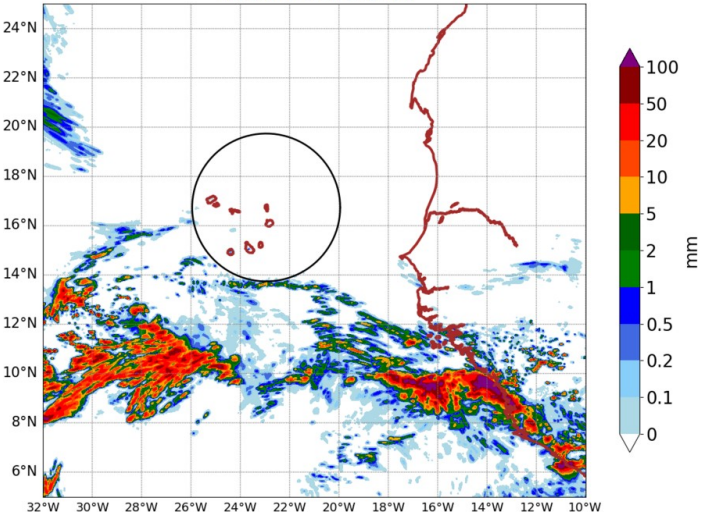
AROME25 20240720-15-UTC -ech(15h) RR cumulated over 6h
