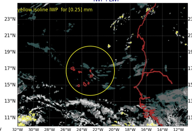
AROME25 20240721-12-UTC -ech(36h) IWP+LWP
