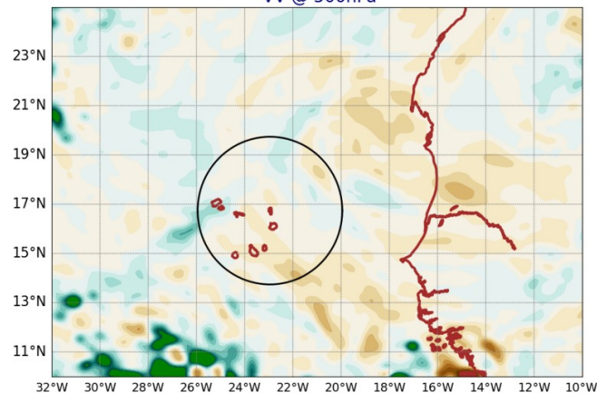
AROME25 20240720-12-UTC -ech(12h) VV @ 500hPa
