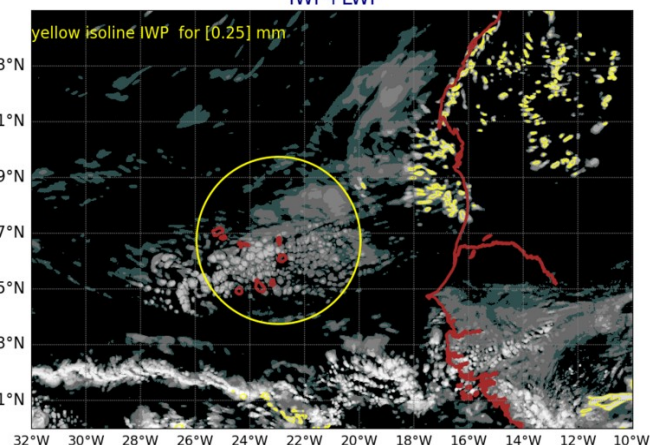
AROME25 20240722-12-UTC -ech(60h) IWP+LWP
