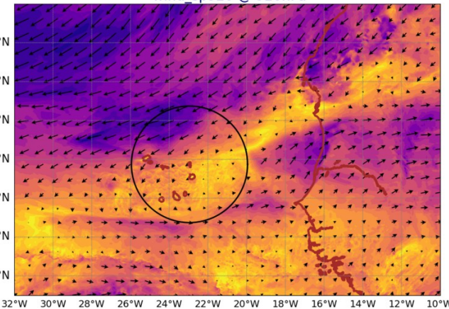
AROME25 20240722-12-UTC -ech(60h) wind_sp920 @ 920hPa
