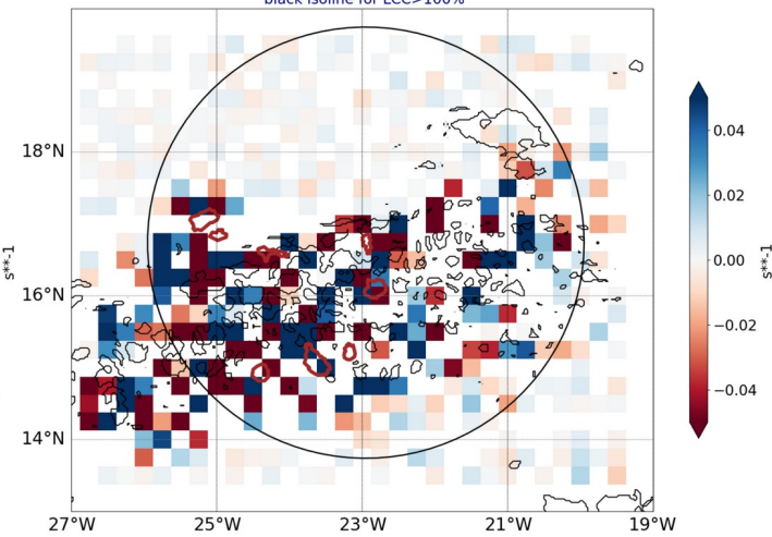
AROME25 regrid 0.25 20240722-12-UTC -ech(60h) blue for conv in subcloud layer black isoline for LCC>100%
