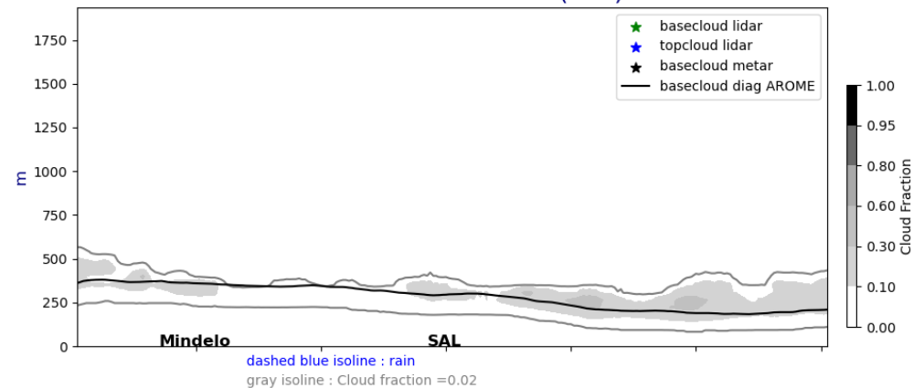
Cross section E/W @ 17.5N 20240720-12-UTC ech(12h)
