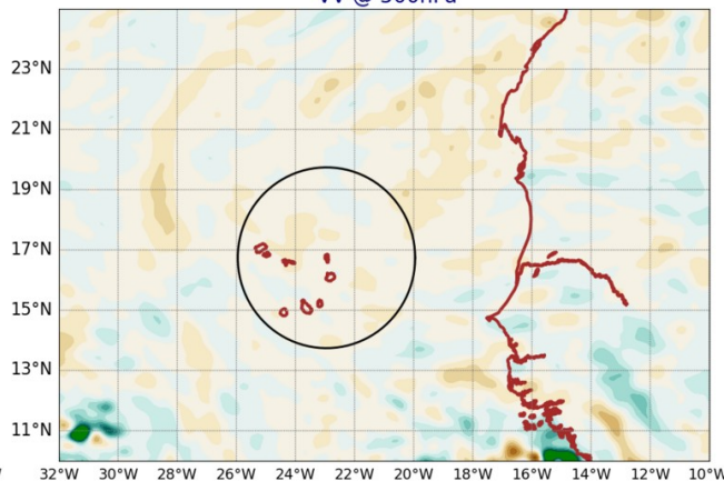
AROME25 20240721-12-UTC -ech(36h) VV @ 500hPa
