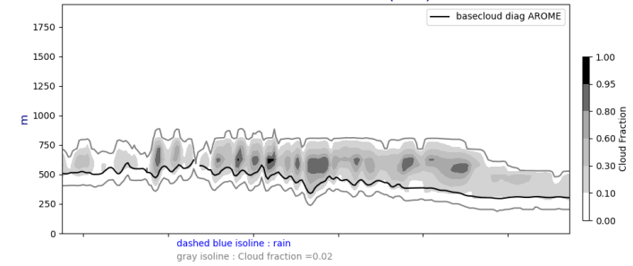
Cross section S/N @ -22W 20240722-12-UTC ech(60h)
