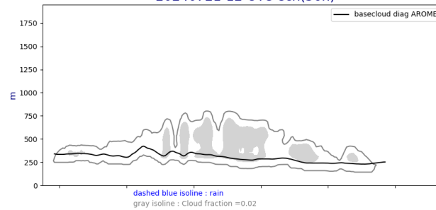
Cross section S/N @ -22W 20240721-12-UTC ech(36h)
