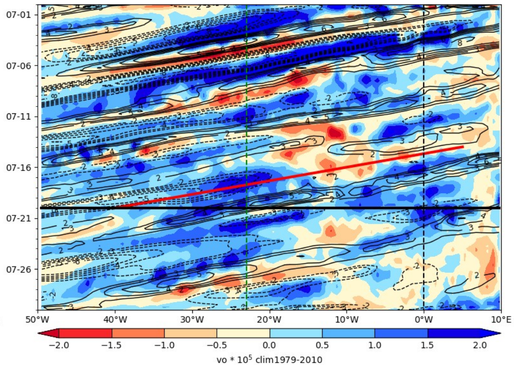
ECMWF Vorticity 850 hPa (color), V-700 hPa 2024-07-20
