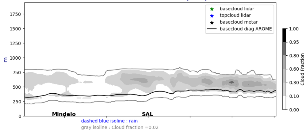
Cross section E/W @ 17.5N 20240722-12-UTC ech(60h)
