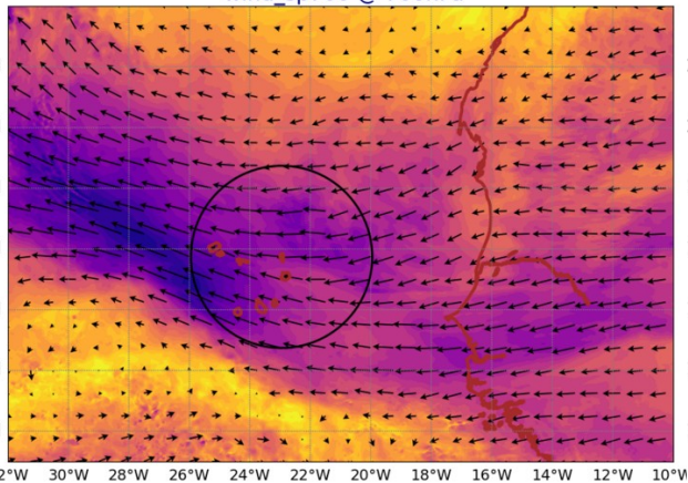
AROME25 20240720-12-UTC -ech(12h) wind_sp920 @ 920hPa
