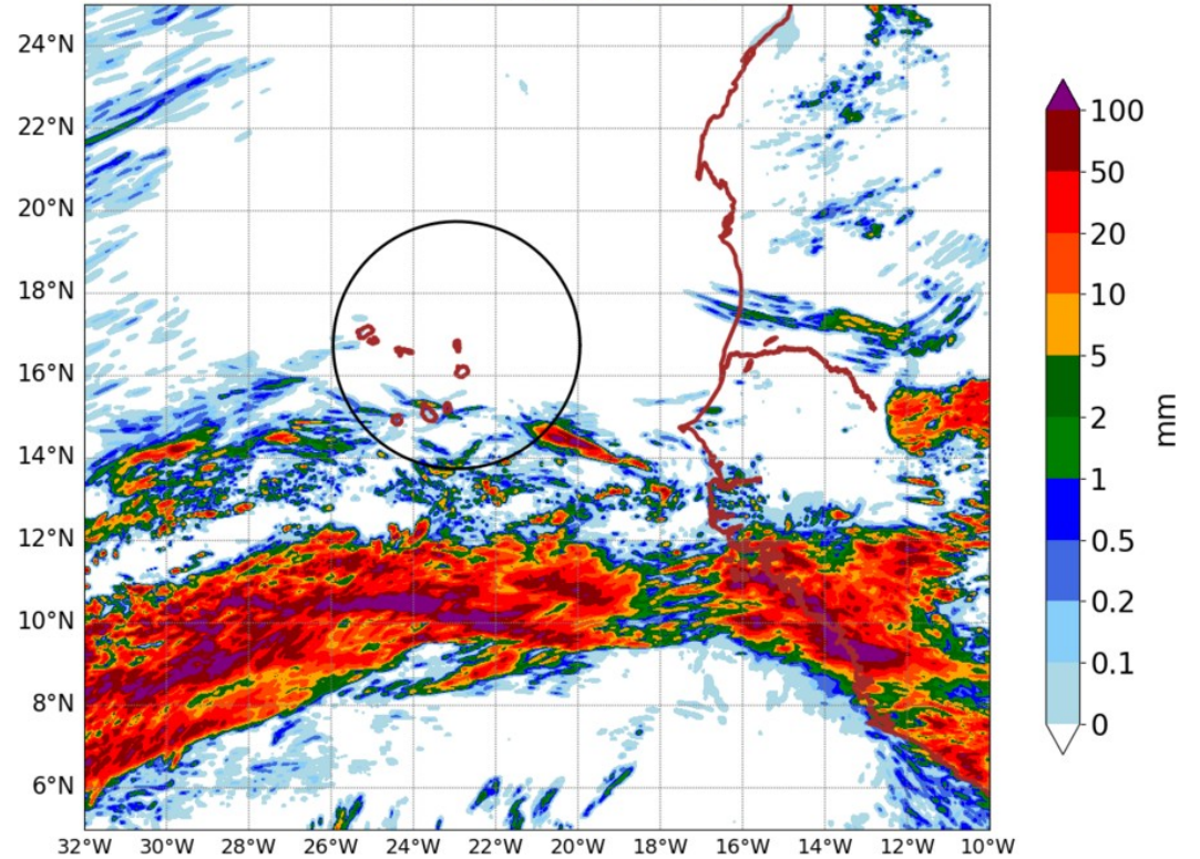
AROME25 20240720-00-UTC -ech(24h)
