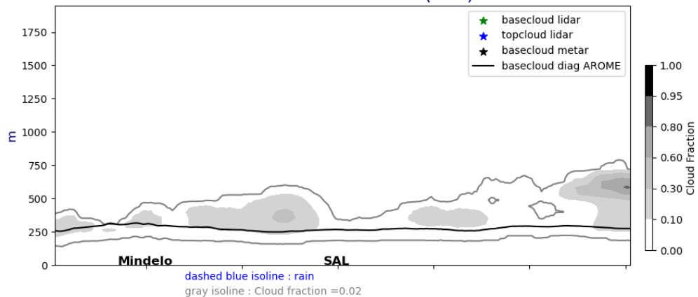
Cross section E/W @ 17.5N 20240721-12-UTC ech(36h)
