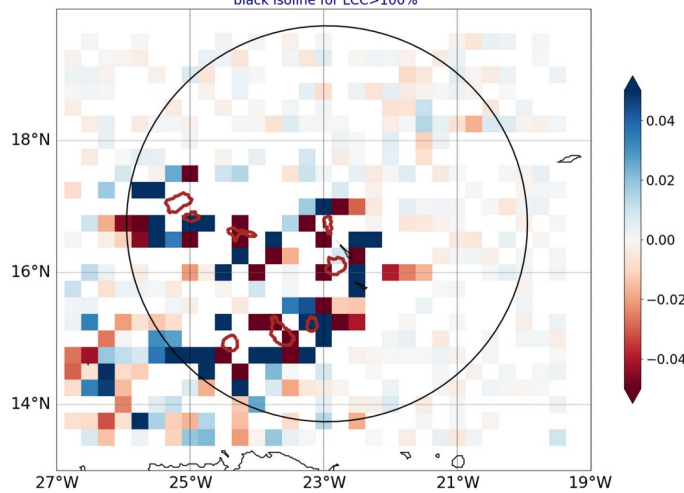
AROME25 regrid 0.25 20240721-12-UTC -ech(36h) blue for conv in subcloud layer black isoline for LCC>100%
