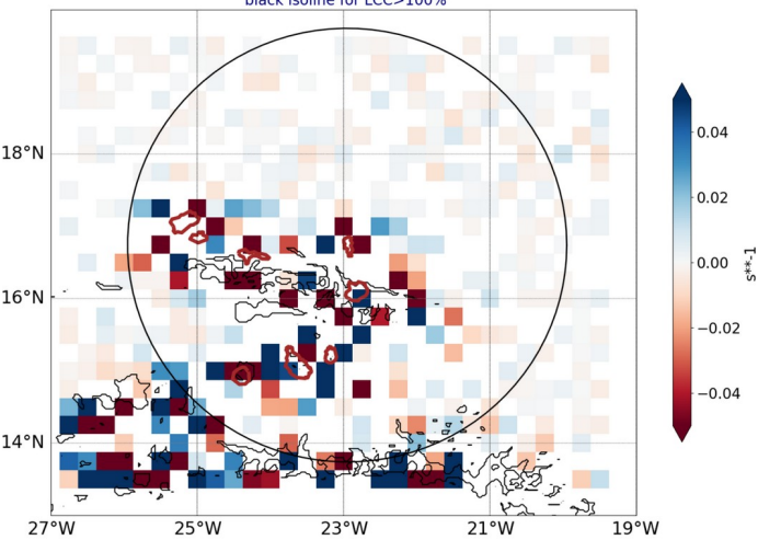
AROME25 regrid 0.25 20240720-12-UTC -ech(12h) blue for conv in subcloud layer black isoline for LCC>100%
