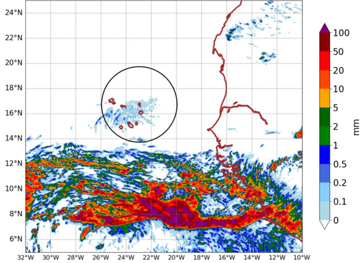
AROME25 20240722-12-UTC -ech(60h) RR cumulated over 24h
