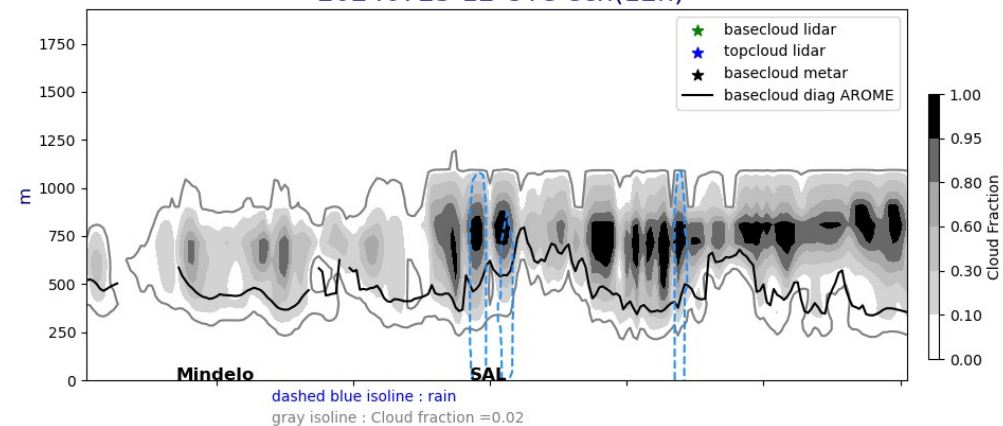
Cross section E/W @ 17.5N 20240723-12-UTC ech(12h)
