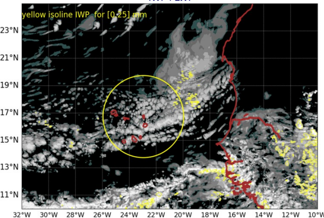
AROME25 20240723-12-UTC -ech(12h) IWP+LWP
