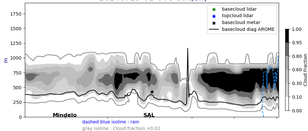
Cross section E/W @ 17.5N 20240723-01-UTC ech(1h)
