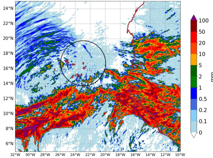
AROME25 20240725-12-UTC -ech(60h) RR cumulated over 24h
