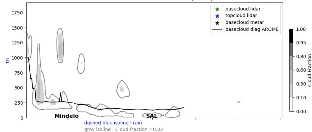
Cross section E/W @ 17.5N 20240725-12-UTC ech(60h)
