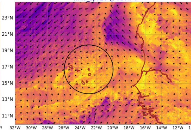
AROME25 20240724-12-UTC -ech(36h) wind_sp920 @ 920hPa
