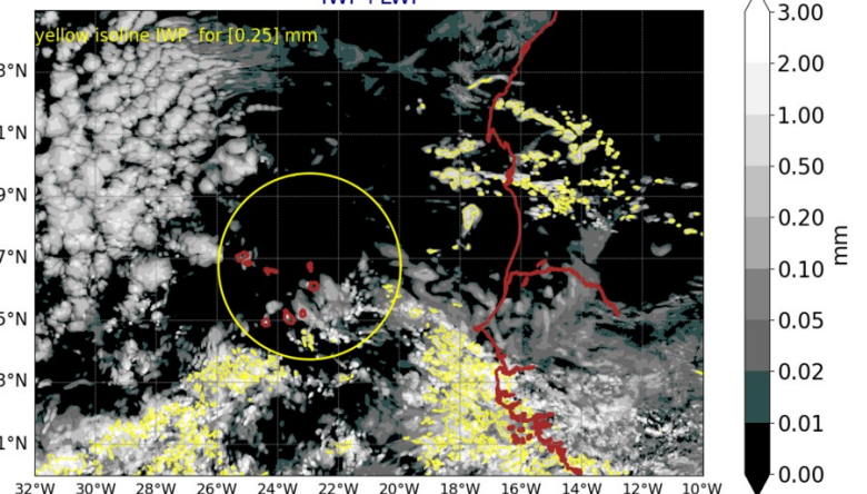
AROME25 20240725-12-UTC -ech(60h) IWP+LWP
