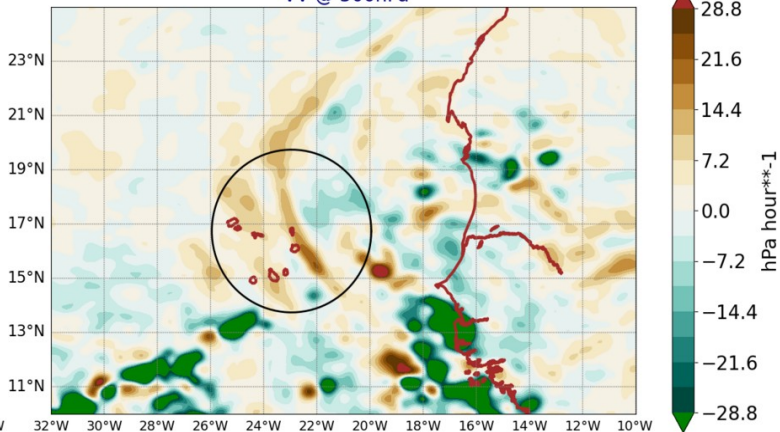
AROME25 20240725-12-UTC -ech(60h) VV @ 500hPa
