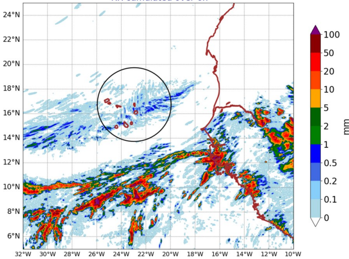
AROME25 20240723-15-UTC -ech(15h) RR cumulated over 6h
