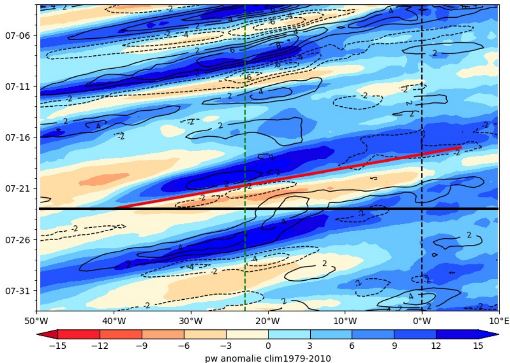
ECMWF PW (color) AND V at 925 hPa 2024-07-23
