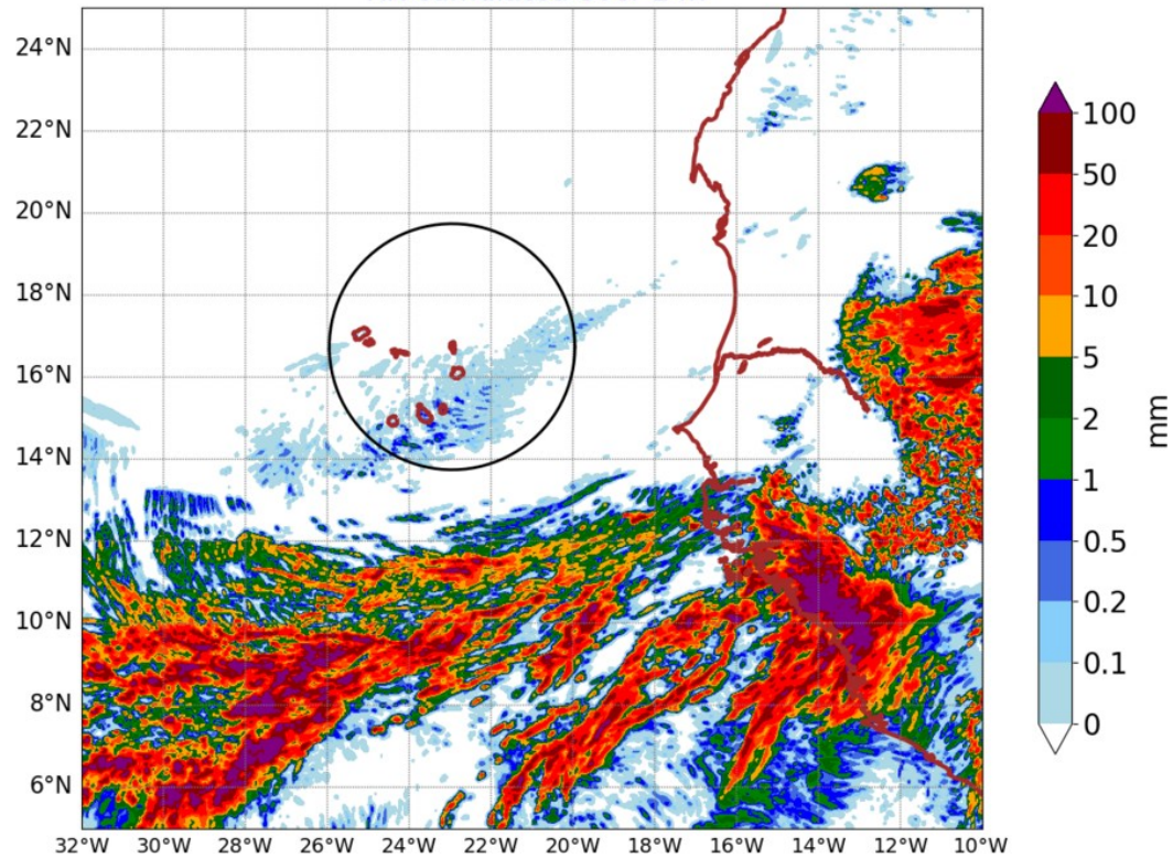
AROME25 20240723-00-UTC -ech(24h) RR cumulated over 24h
