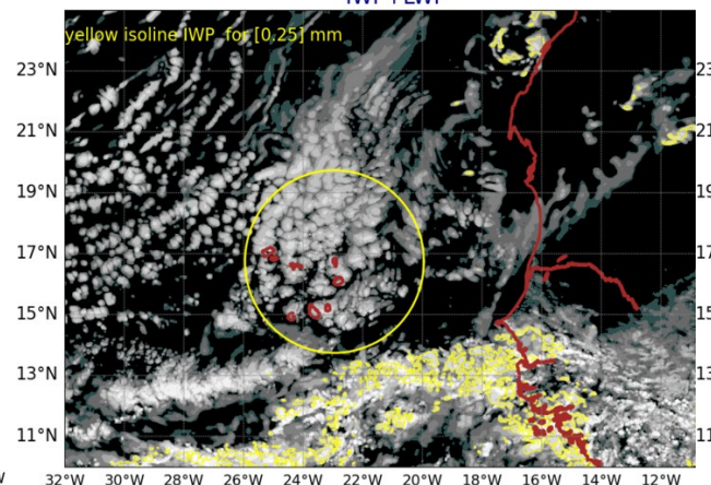
AROME25 20240724-12-UTC -ech(36h) IWP+LWP
