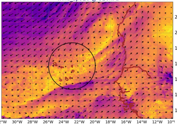
AROME25 20240723-12-UTC -ech(12h) wind_sp920 @ 920hPa
