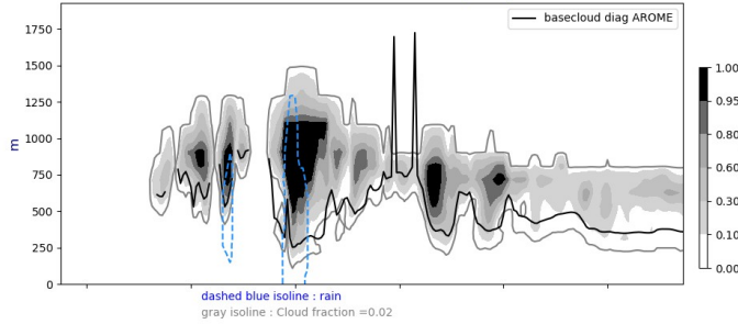
Cross section S/N @ -22W 20240723-12-UTC ech(12h)
