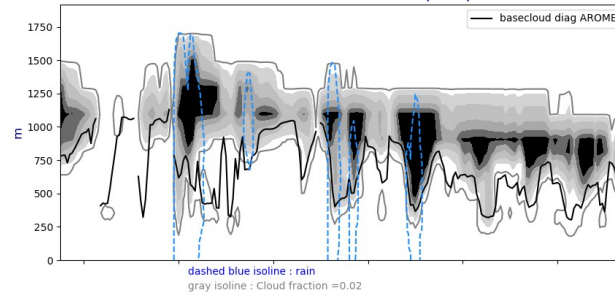
Cross section S/N @ -22W 20240724-12-UTC ech(36h)
