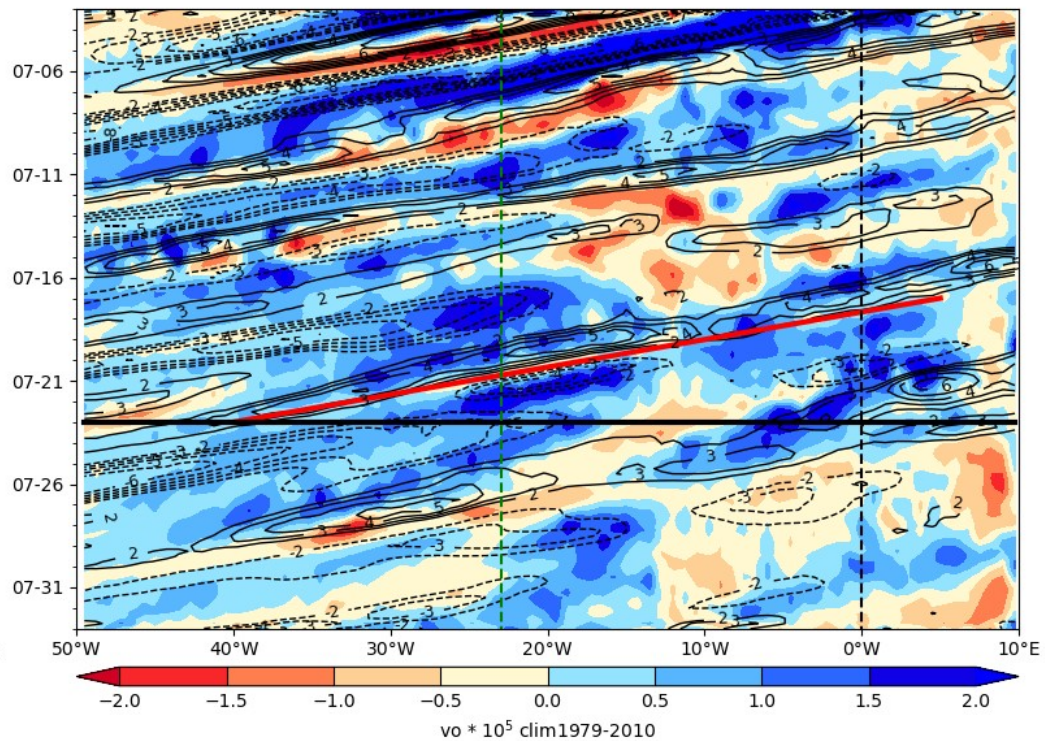
ECMWF Vorticity 850 hPa (color), V-700 hPa 2024-07-23
