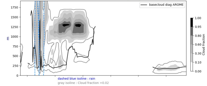
Cross section S/N @ -22W 20240725-12-UTC ech(60h)
