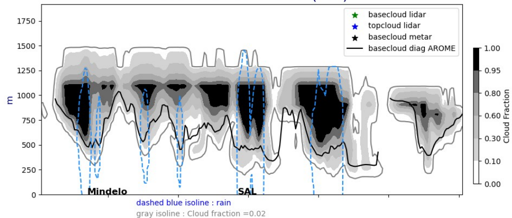
Cross section E/W @ 17.5N 20240724-12-UTC ech(36h)
