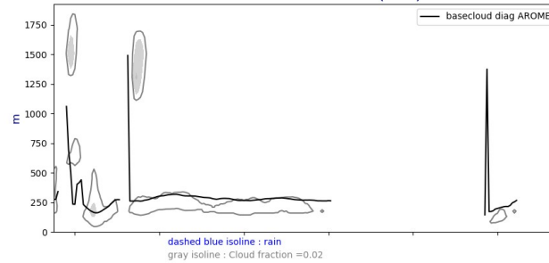
Cross section S/N @ -22W 20240725-12-UTC ech(36h)
