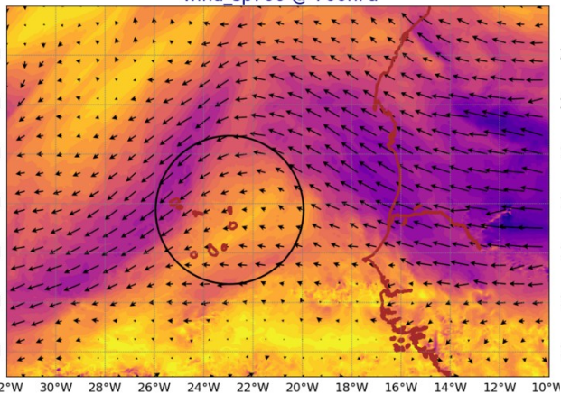
AROME25 20240724-12-UTC -ech(12h) wind_sp920 @ 920hPa
