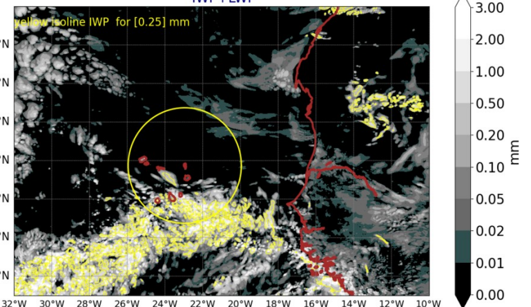
AROME25 20240726-12-UTC -ech(60h) IWP+LWP
