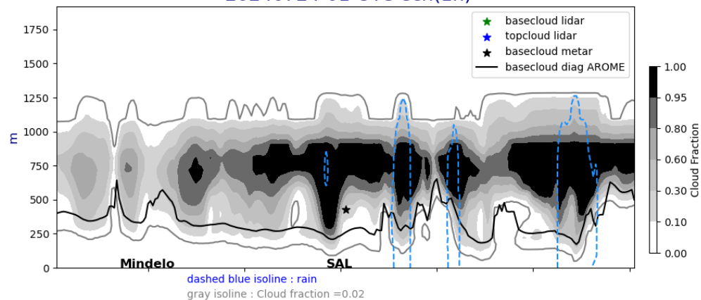
Cross section E/W @ 17.5N 20240724-01-UTC ech(1h)
