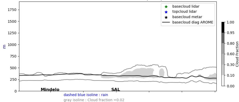
Cross section E/W @ 17.5N 20240726-12-UTC ech(60h)
