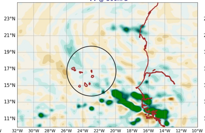
AROME25 20240725-12-UTC -ech(36h) VV @ 500hPa
