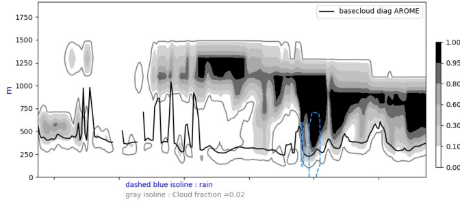
Cross section S/N @ -22W 20240724-12-UTC ech(12h)
