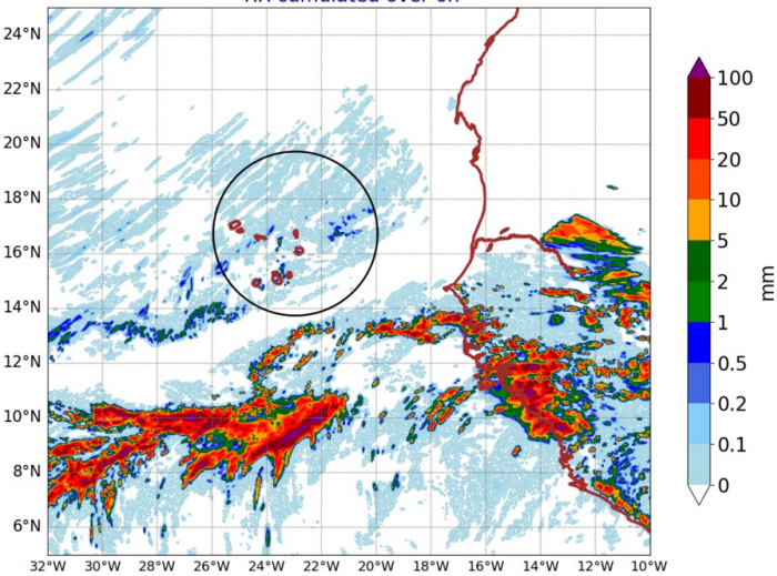
AROME25 20240724-15-UTC -ech(15h) RR cumulated over 6h
