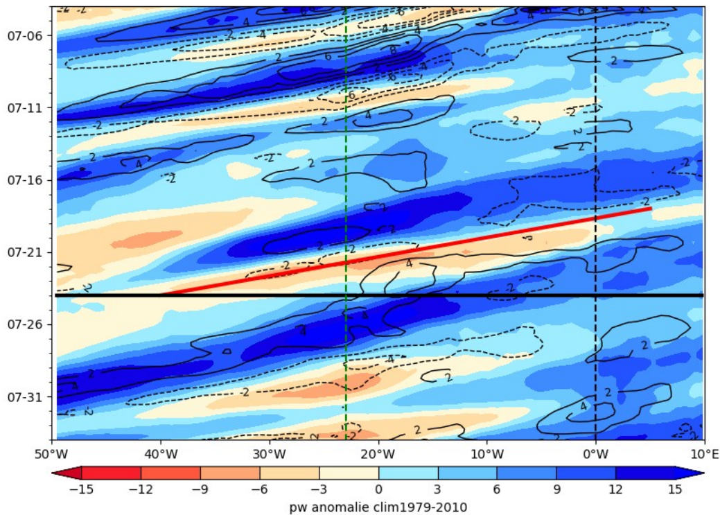
ECMWF PW (color) AND V at 925 hPa 2024-07-24
