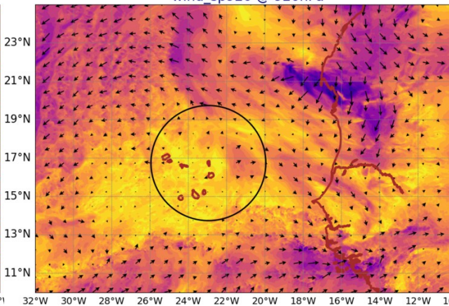
AROME25 20240725-12-UTC -ech(36h) wind_sp920 @ 920hPa
