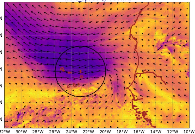
AROME25 20240726-12-UTC -ech(60h) wind_sp920 @ 920hPa
