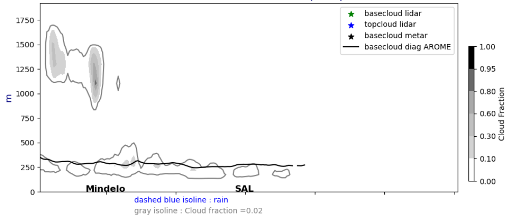
Cross section E/W @ 17.5N 20240725-12-UTC ech(36h)
