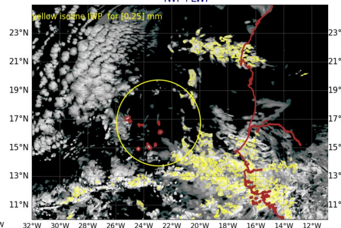
AROME25 20240725-12-UTC -ech(36h) IWP+LWP
