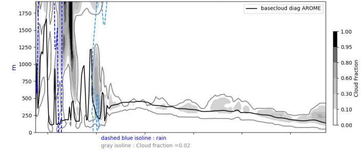
Cross section S/N @ -22W 20240726-12-UTC ech(60h)
