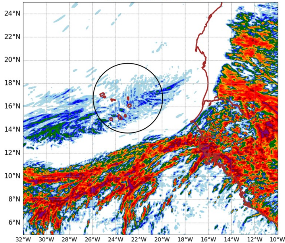
AROME25 20240724-00-UTC -ech(24h) RR cumulated over 24h
