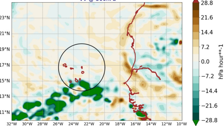
AROME25 20240726-12-UTC -ech(60h) VV @ 500hPa
