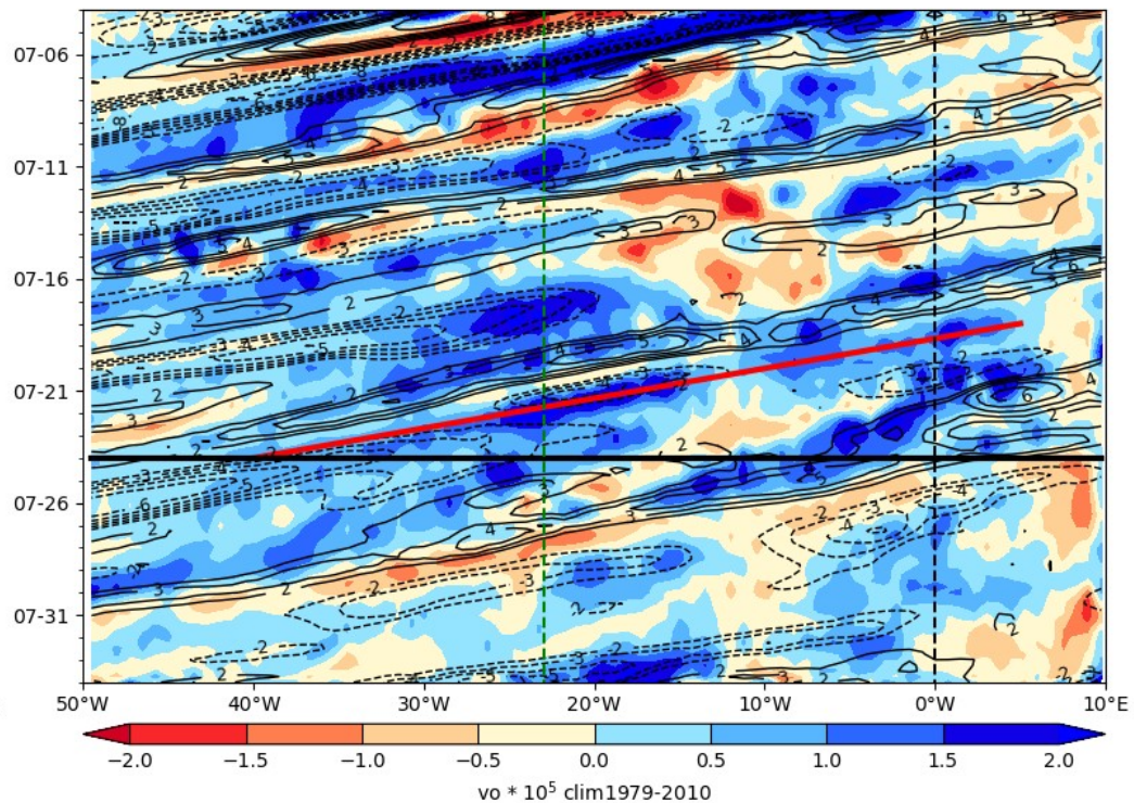
ECMWF Vorticity 850 hPa (color), V-700 hPa 2024-07-24
