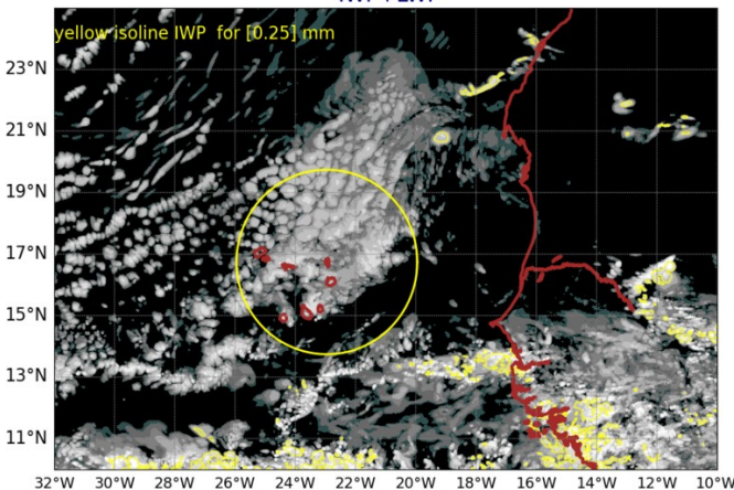
AROME25 20240724-12-UTC -ech(12h) IWP+LWP
