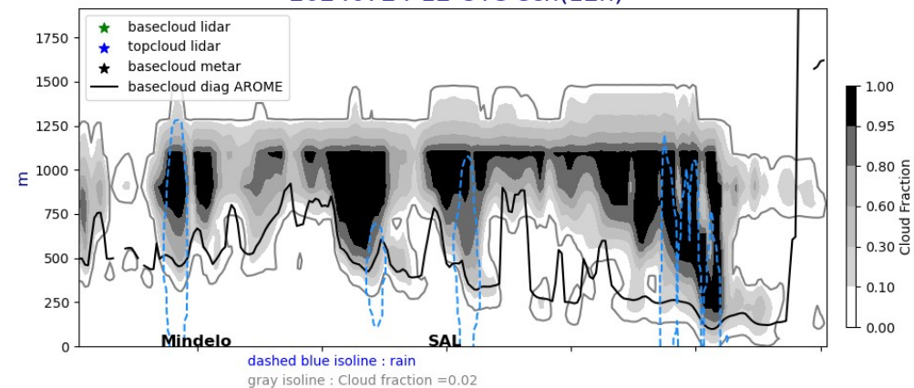
Cross section E/W @ 17.5N 20240724-12-UTC ech(12h)
