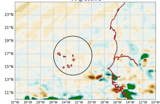
AROME25 20240724-12-UTC -ech(12h) VV @ 500hPa
