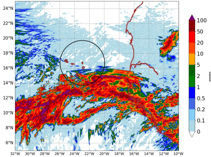
AROME25 20240726-12-UTC -ech(60h) RR cumulated over 24h
