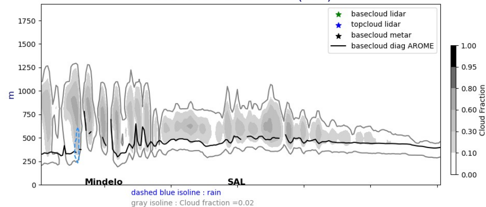
Cross section E/W @ 17.5N 20240727-12-UTC ech(60h)
