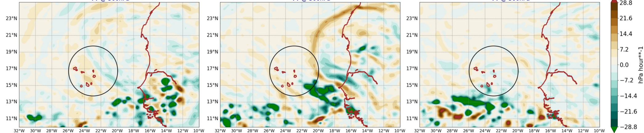
AROME25 20240725-12-UTC -ech(12h) VV @ 500hPa
