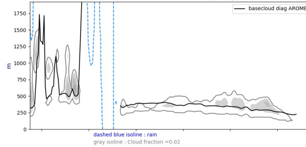
Cross section S/N @ -22W 20240726-12-UTC ech(36h)
