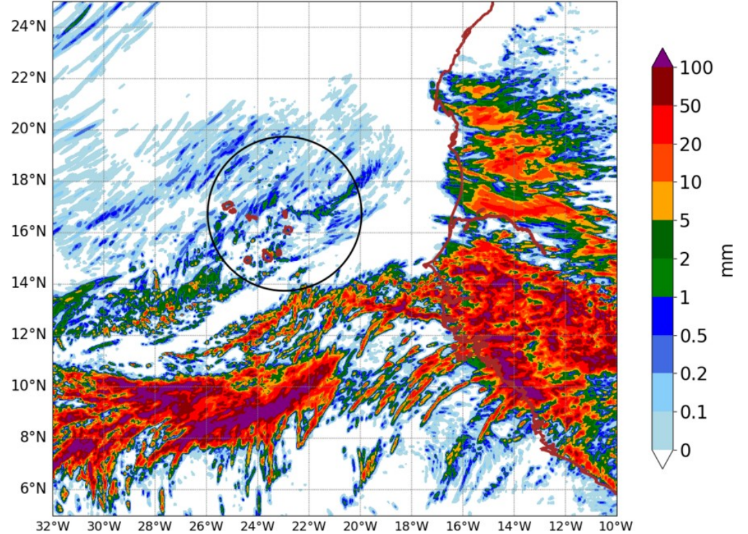
AROME25 20240725-00-UTC -ech(24h)
