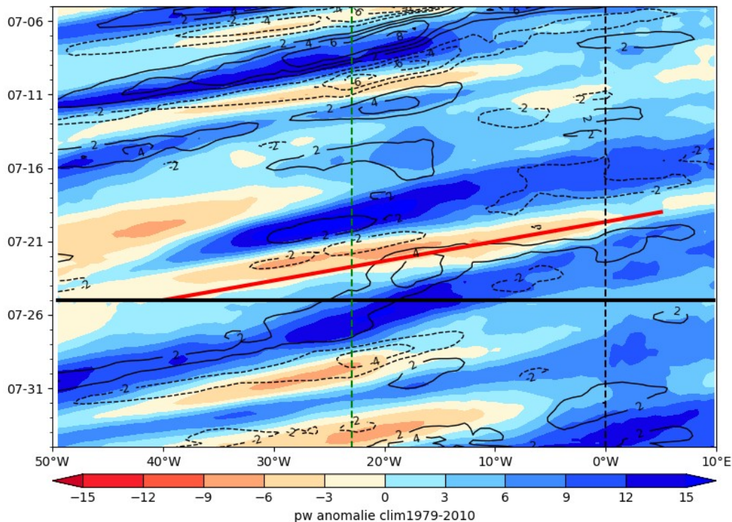
ECMWF PW (color) AND V at 925 hPa 2024-07-25
