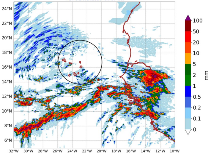
AROME25 20240725-15-UTC -ech(15h) RR cumulated over 6h
