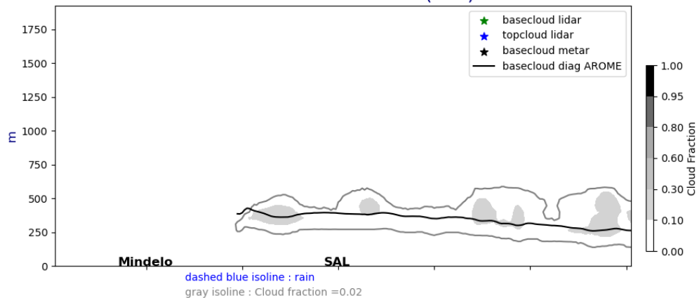
Cross section E/W @ 17.5N 20240726-12-UTC ech(36h)
