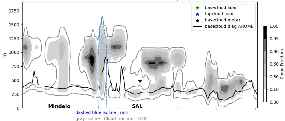
Cross section E/W @ 17.5N 20240725-01-UTC ech(1h)
