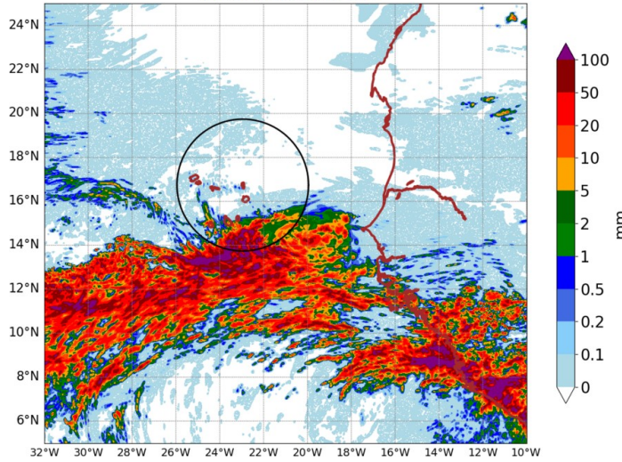
AROME25 20240727-12-UTC -ech(60h) RR cumulated over 24h
