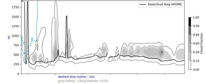
Cross section S/N @ -22W 20240727-12-UTC ech(60h)
