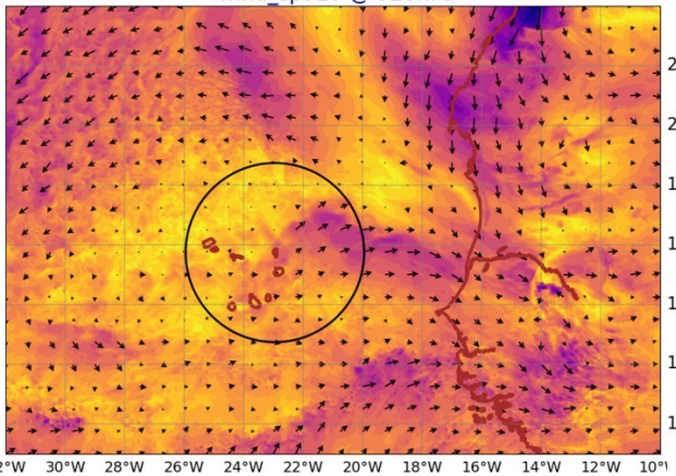
AROME25 20240725-12-UTC -ech(12h) wind_sp920 @ 920hPa
