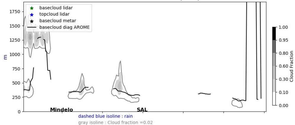
Cross section E/W @ 17.5N 20240725-12-UTC ech(12h)
