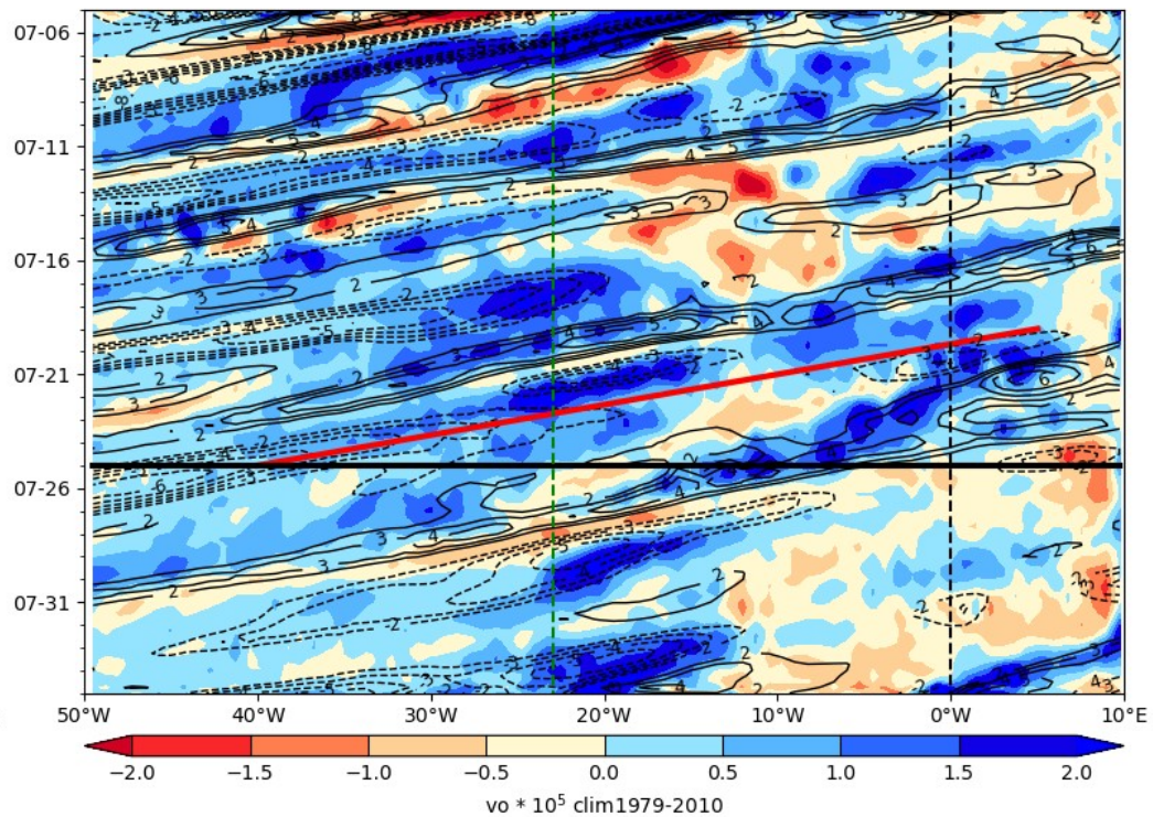
ECMWF Vorticity 850 hPa (color), V-700 hPa 2024-07-25
