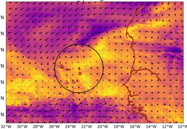
AROME25 20240727-12-UTC -ech(60h) wind_sp920 @ 920hPa
