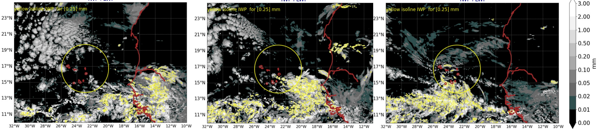
AROME25 20240725-12-UTC -ech(12h) IWP+LWP
