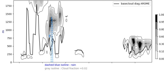
Cross section S/N @ -22W 20240725-12-UTC ech(12h)
