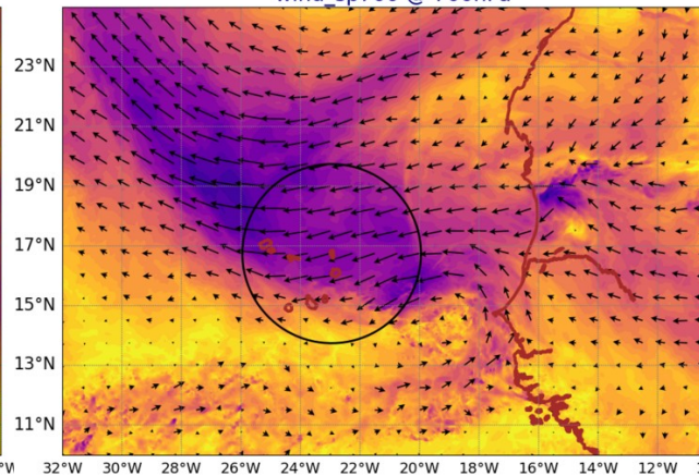
AROME25 20240726-12-UTC -ech(36h) wind_sp920 @ 920hPa
