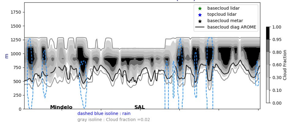
Cross section E/W @ 17.5N 20240803-12-UTC ech(60h)
