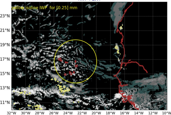
AROME25 20240801-12-UTC -ech(12h) IWP+LWP
