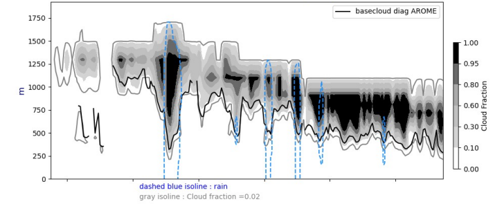
Cross section S/N @ -22W 20240803-12-UTC ech(60h)
