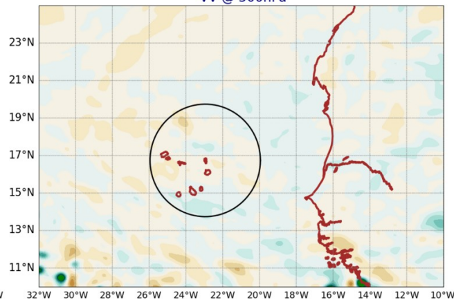
AROME25 20240802-12-UTC -ech(36h) VV @ 500hPa
