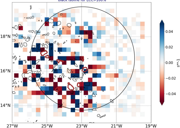
AROME25 regrid 0.25 20240801-12-UTC -ech(12h) blue for conv in subcloud layer black isoline for LCC>100%
