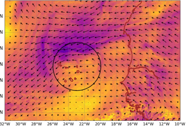
AROME25 20240803-12-UTC -ech(60h) wind_sp920 @ 920hPa
