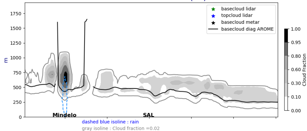
Cross section E/W @ 17.5N 20240801-01-UTC ech(1h)
