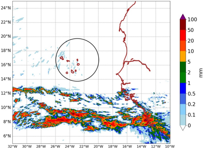
AROME25 20240801-15-UTC -ech(15h) RR cumulated over 6h
