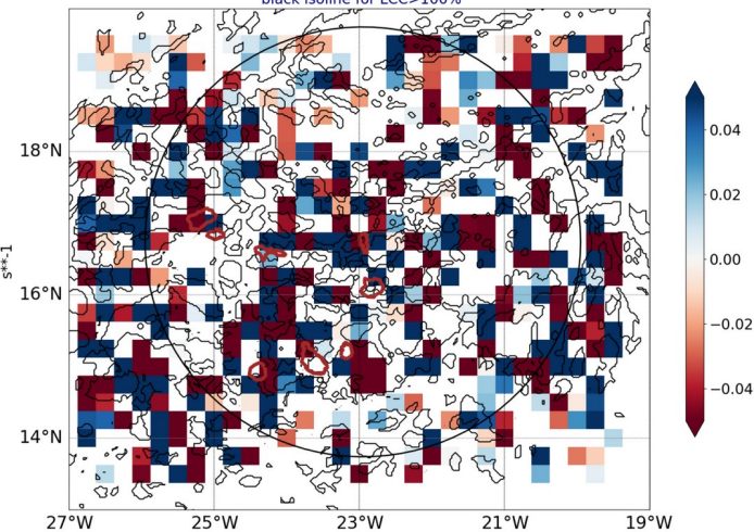
AROME25 regrid 0.25 20240803-12-UTC -ech(60h) blue for conv in subcloud layer black isoline for LCC>100%
