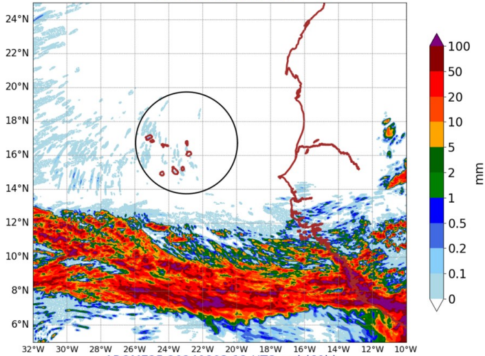
AROME25 20240803-12-UTC -ech(60h) RR cumulated over 24h
