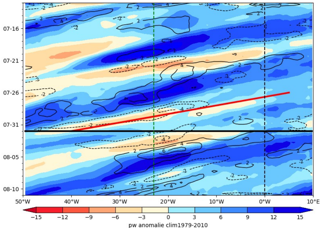
ECMWF PW (color) AND V at 925 hPa 2024-08-01
