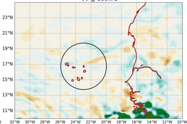
AROME25 20240803-12-UTC -ech(60h) VV @ 500hPa
