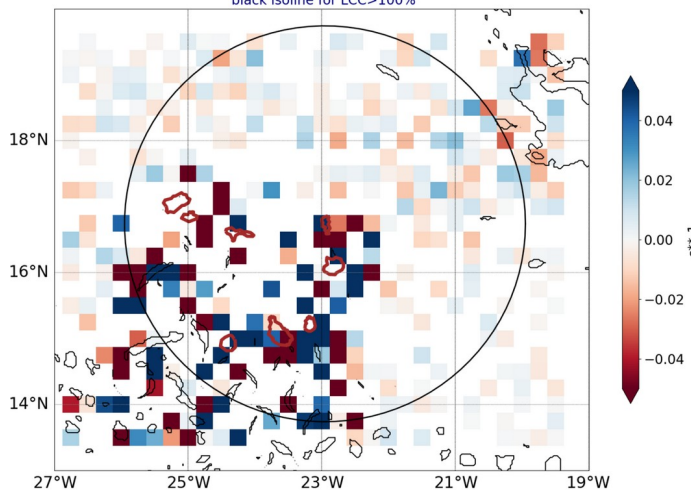
AROME25 regrid 0.25 20240802-12-UTC -ech(36h) blue for conv in subcloud layer black isoline for LCC>100%
