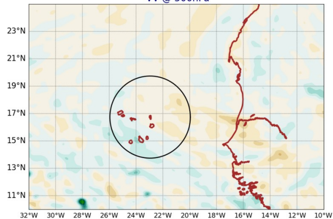
AROME25 20240801-12-UTC -ech(12h) VV @ 500hPa
