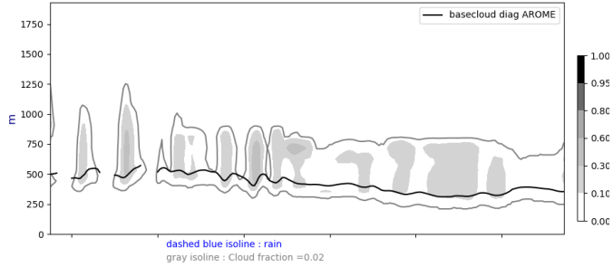
Cross section S/N @ -22W 20240801-12-UTC ech(12h)
