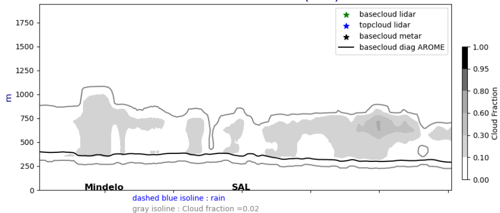
Cross section E/W @ 17.5N 20240802-12-UTC ech(36h)
