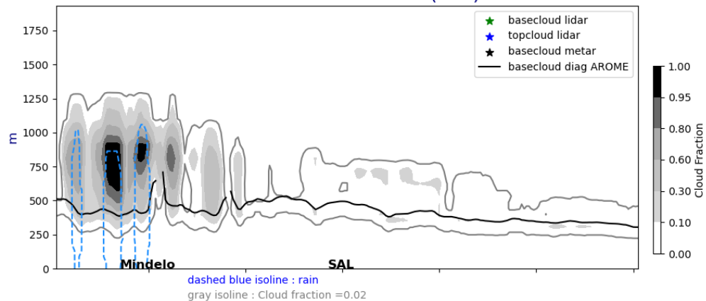
Cross section E/W @ 17.5N 20240801-12-UTC ech(12h)
