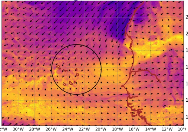
AROME25 20240801-12-UTC -ech(12h) wind_sp920 @ 920hPa
