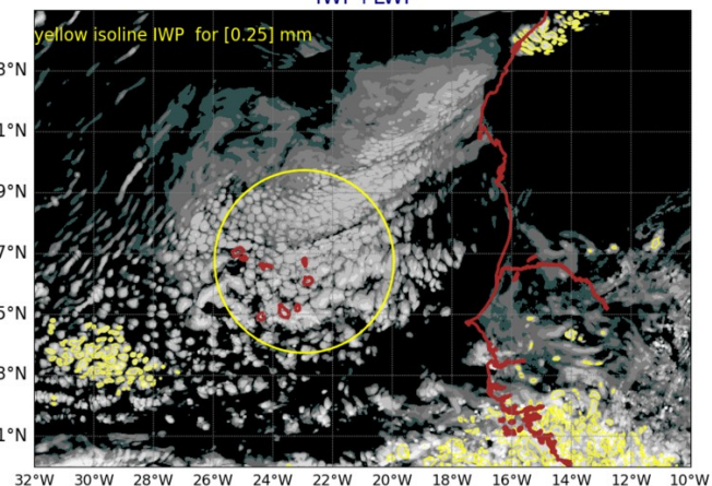
AROME25 20240803-12-UTC -ech(60h) IWP+LWP
