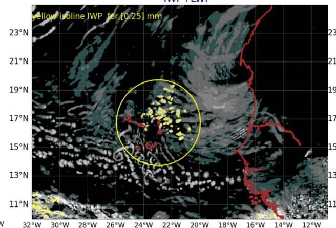
AROME25 20240802-12-UTC -ech(36h) IWP+LWP
