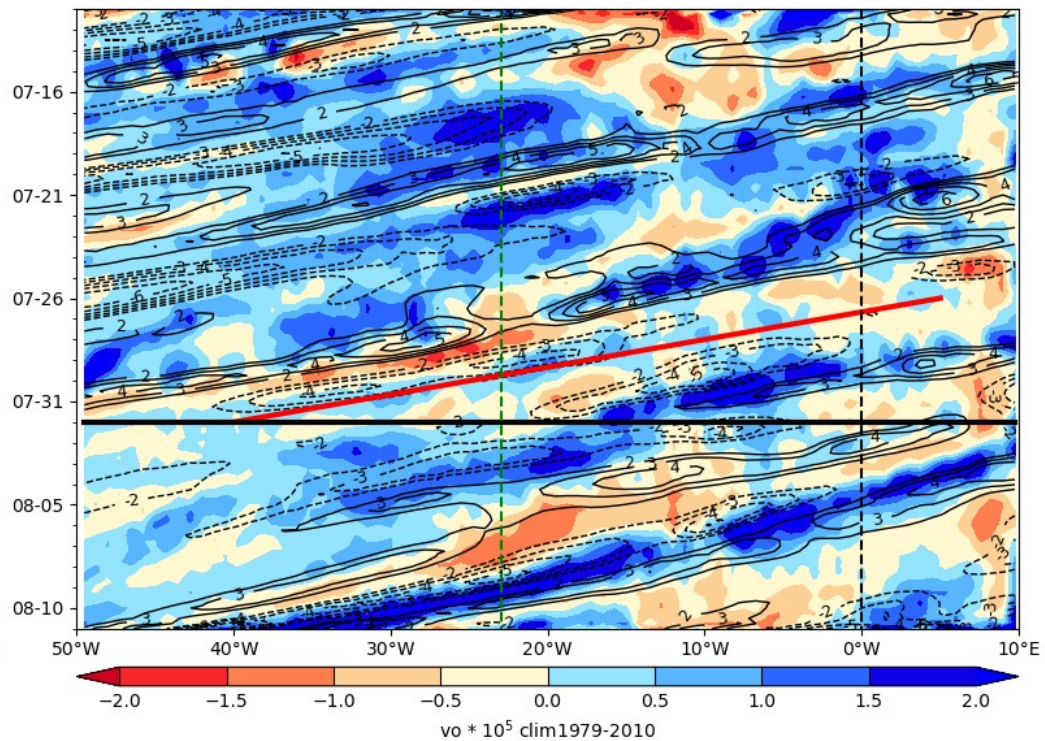
ECMWF Vorticity 850 hPa (color), V-700 hPa 2024-08-01
