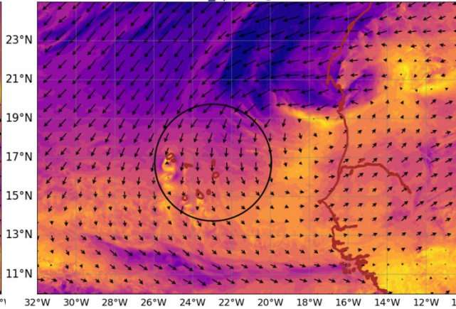
AROME25 20240802-12-UTC -ech(36h) wind_sp920 @ 920hPa
