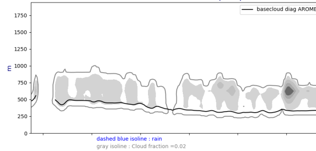
Cross section S/N @ -22W 20240802-12-UTC ech(36h)
