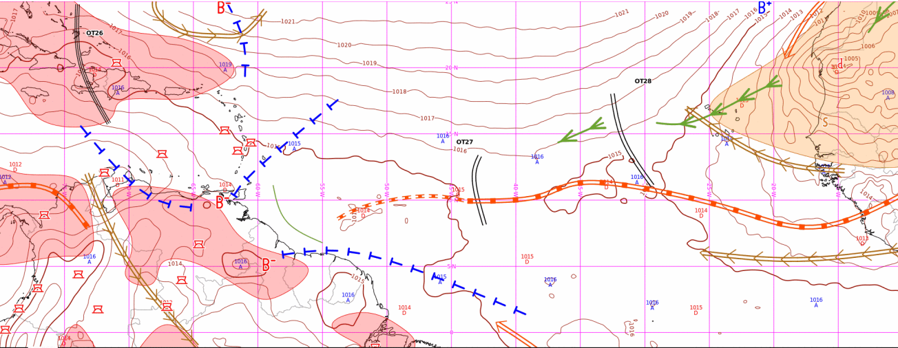
ANASYG du ven. 02/08/2024 - 00 UTC
