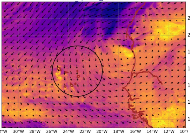
AROME25 20240802-12-UTC -ech(12h) wind_sp920 @ 920hPa
