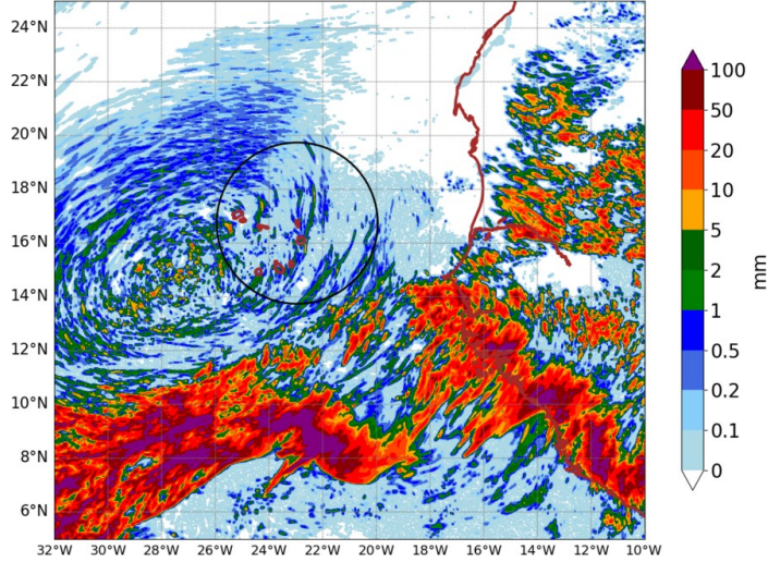
AROME25 20240804-12-UTC -ech(60h) RR cumulated over 24h
