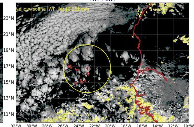
AROME25 20240804-12-UTC -ech(60h) IWP+LWP
