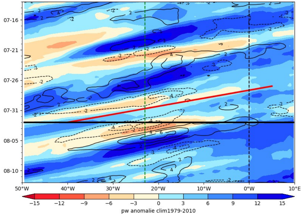
ECMWF PW (color) AND V at 925 hPa 2024-08-02
