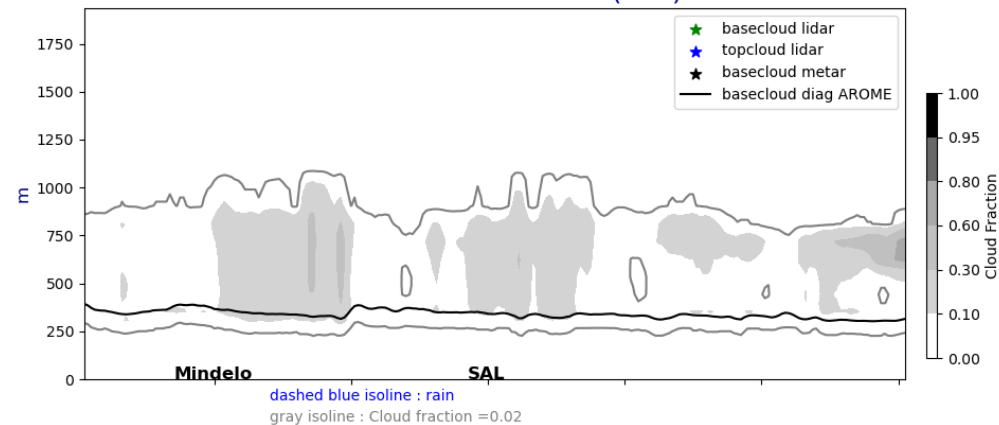
Cross section E/W @ 17.5N 20240802-12-UTC ech(12h)
