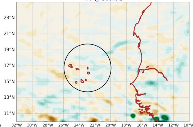
AROME25 20240803-12-UTC -ech(36h) VV @ 500hPa
