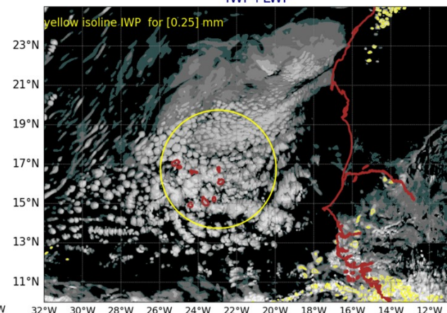
AROME25 20240803-12-UTC -ech(36h) IWP+LWP
