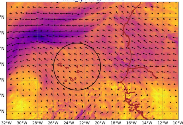
AROME25 20240804-12-UTC -ech(60h) wind_sp920 @ 920hPa
