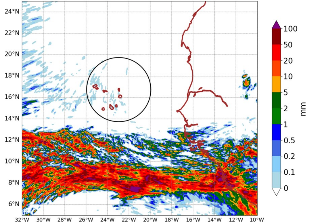
AROME25 20240802-00-UTC -ech(24h)
