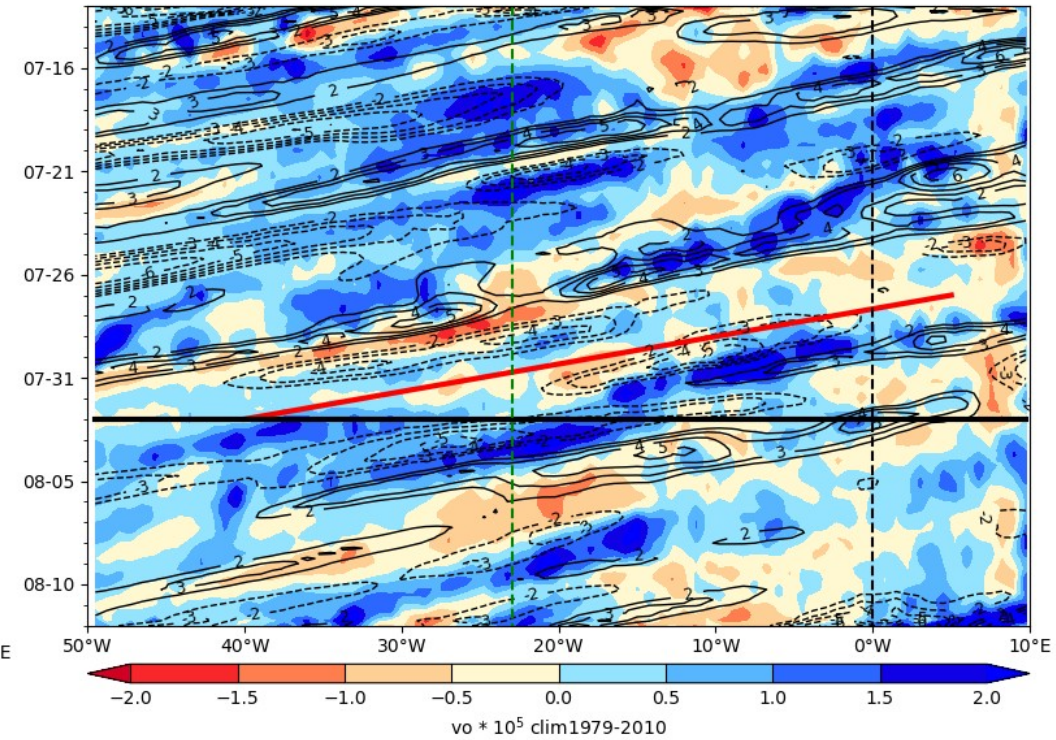
ECMWF Vorticity 850 hPa (color), V-700 hPa 2024-08-02
