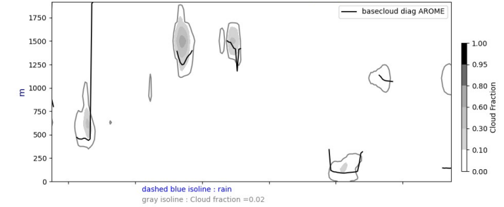
Cross section S/N @ -22W 20240804-12-UTC ech(60h)
