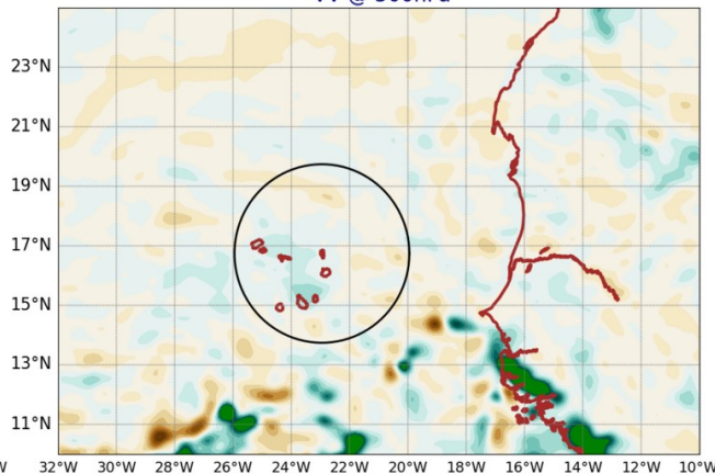
AROME25 20240804-12-UTC -ech(60h) VV @ 500hPa
