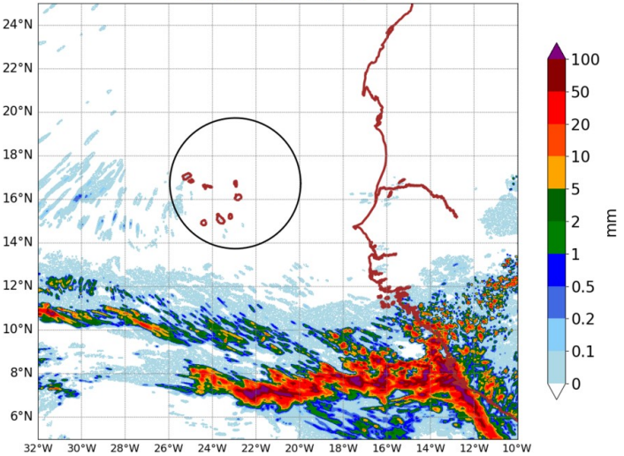
AROME25 20240802-15-UTC -ech(15h) RR cumulated over 6h
