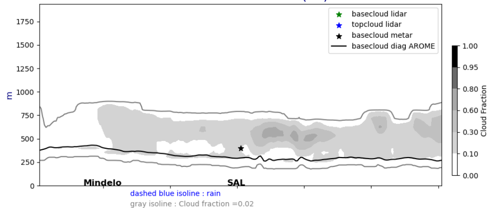
Cross section E/W @ 17.5N 20240802-01-UTC ech(1h)
