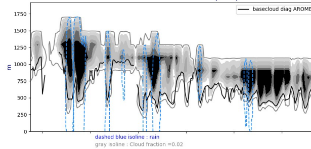
Cross section S/N @ -22W 20240803-12-UTC ech(36h)
