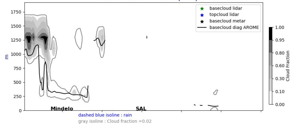
Cross section E/W @ 17.5N 20240804-12-UTC ech(60h)
