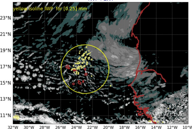
AROME25 20240802-12-UTC -ech(12h) IWP+LWP
