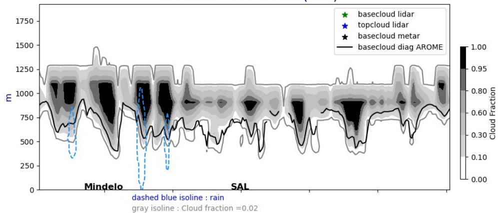
Cross section E/W @ 17.5N 20240803-12-UTC ech(36h)
