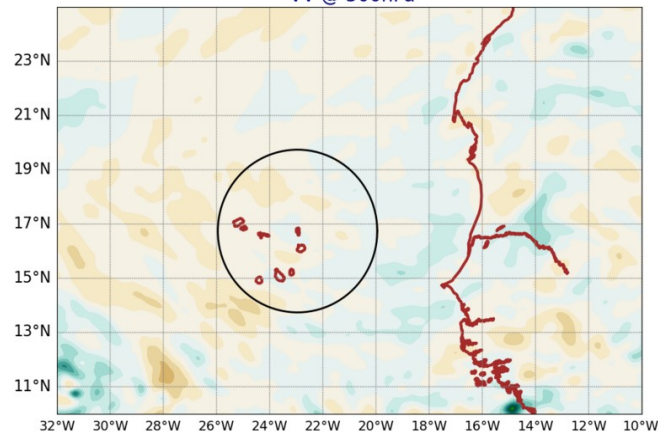
AROME25 20240802-12-UTC -ech(12h) VV @ 500hPa
