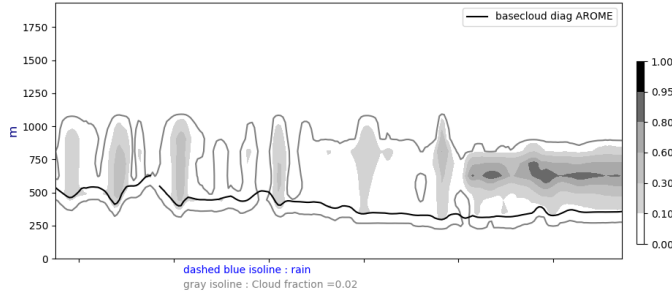
Cross section S/N @ -22W 20240802-12-UTC ech(12h)
