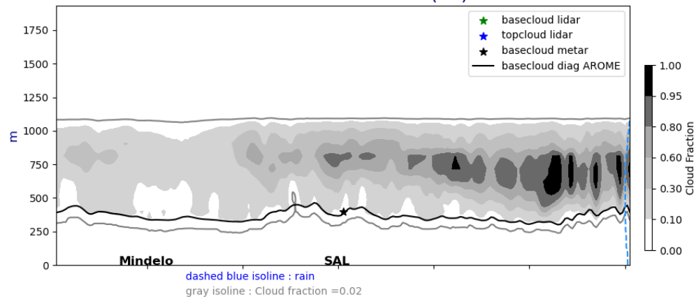
Cross section E/W @ 17.5N 20240803-01-UTC ech(1h)
