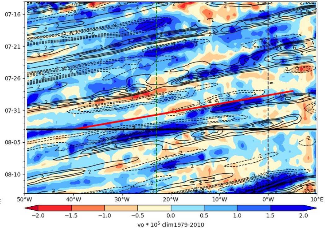
ECMWF Vorticity 850 hPa (color), V-700 hPa 2024-08-03
