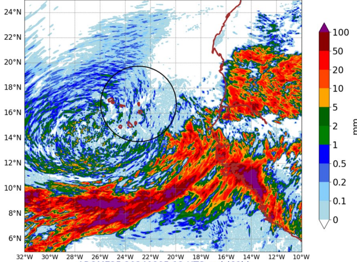
AROME25 20240805-12-UTC -ech(60h) RR cumulated over 24h
