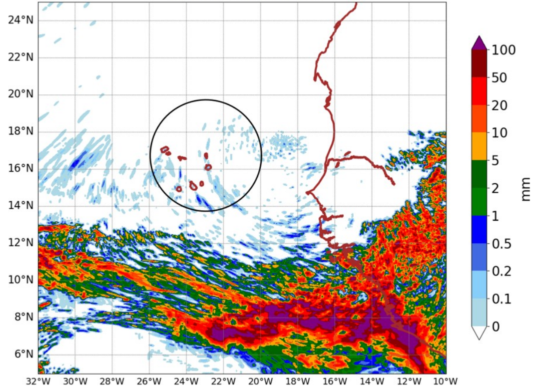
AROME25 20240803-00-UTC -ech(24h)
