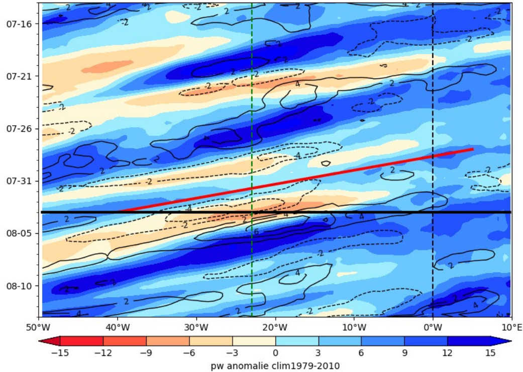
ECMWF PW (color) AND V at 925 hPa 2024-08-03
