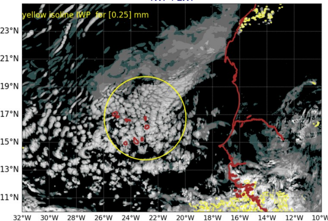
AROME25 20240803-12-UTC -ech(12h) IWP+LWP
