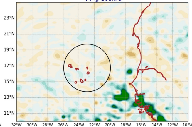
AROME25 20240804-12-UTC -ech(36h) VV @ 500hPa
