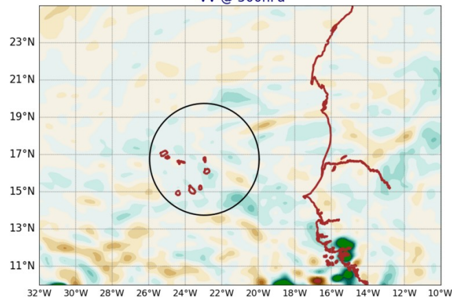
AROME25 20240803-12-UTC -ech(12h) VV @ 500hPa
