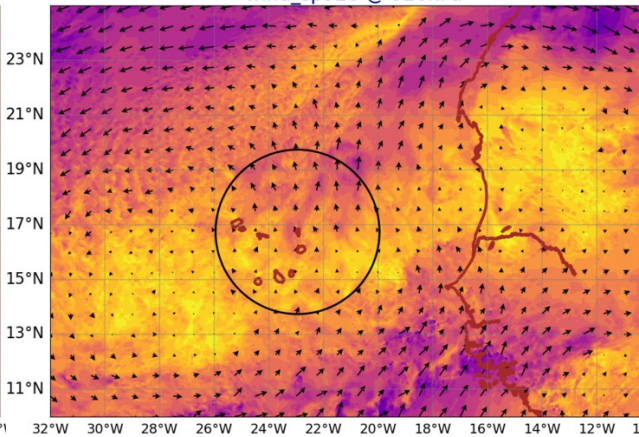
AROME25 20240804-12-UTC -ech(36h) wind_sp920 @ 920hPa
