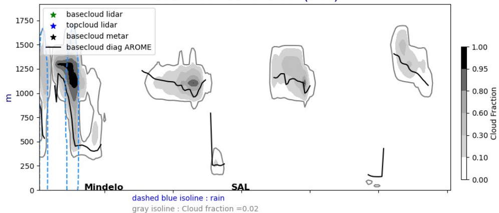
Cross section E/W @ 17.5N 20240804-12-UTC ech(36h)
