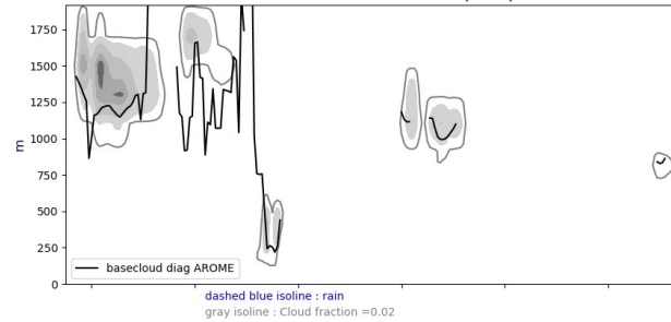
Cross section S/N @ -22W 20240804-12-UTC ech(36h)
