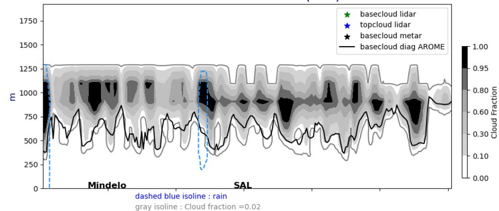
Cross section E/W @ 17.5N 20240803-12-UTC ech(12h)
