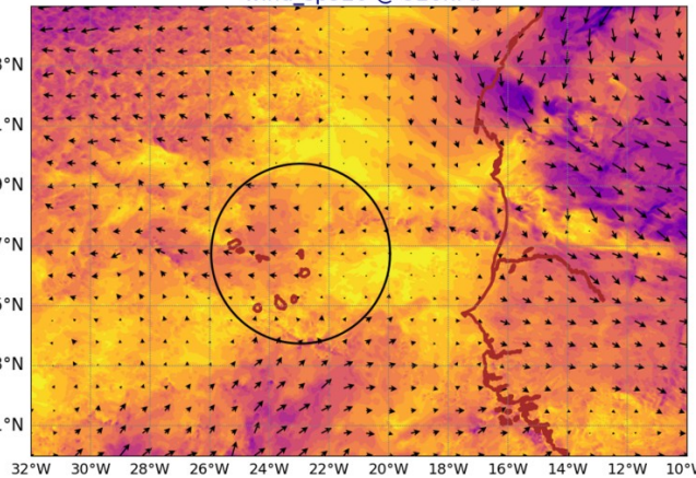
AROME25 20240805-12-UTC -ech(60h) wind_sp920 @ 920hPa
