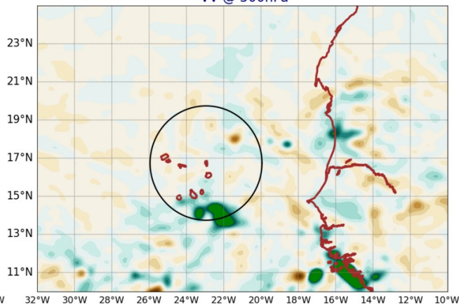
AROME25 20240805-12-UTC -ech(60h) VV @ 500hPa
