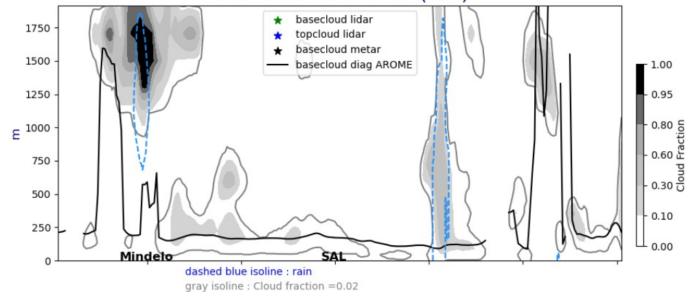
Cross section E/W @ 17.5N 20240805-12-UTC ech(60h)
