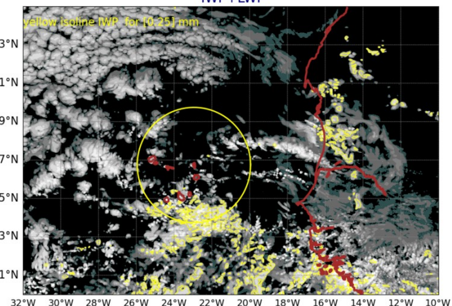
AROME25 20240805-12-UTC -ech(60h) IWP+LWP
