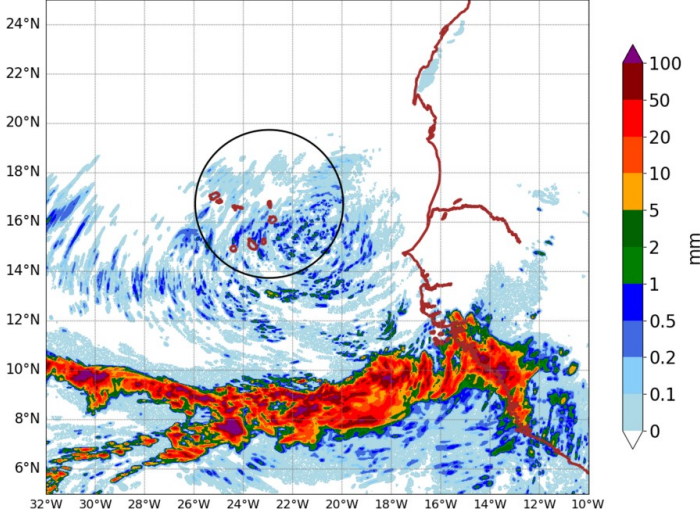
AROME25 20240803-15-UTC -ech(15h) RR cumulated over 6h
