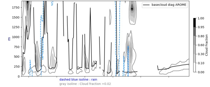
Cross section S/N @ -22W 20240805-12-UTC ech(60h)
