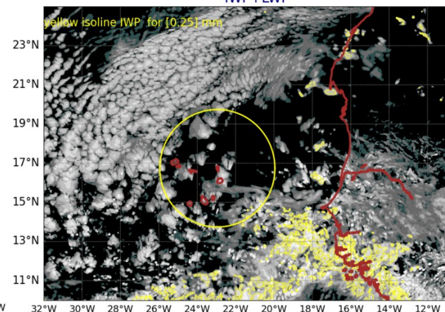
AROME25 20240804-12-UTC -ech(36h) IWP+LWP
