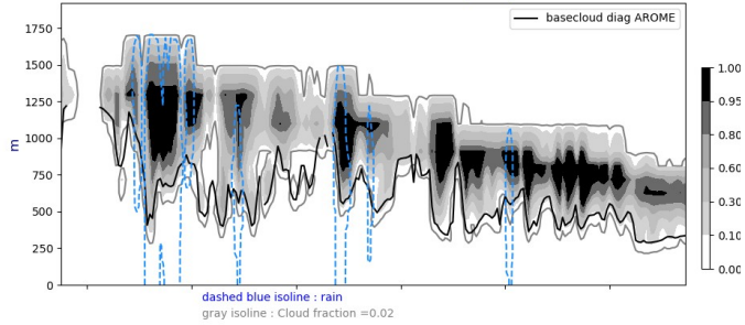
Cross section S/N @ -22W 20240803-12-UTC ech(12h)
