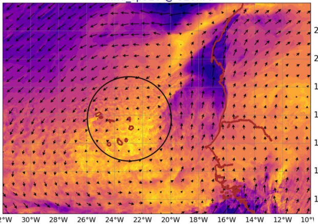
AROME25 20240803-12-UTC -ech(12h) wind_sp920 @ 920hPa
