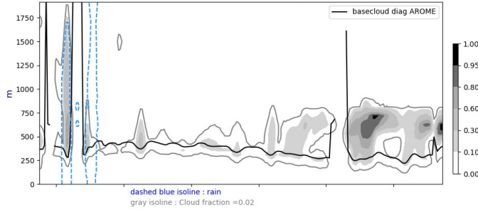
Cross section S/N @ -22W 20240806-12-UTC ech(12h)
