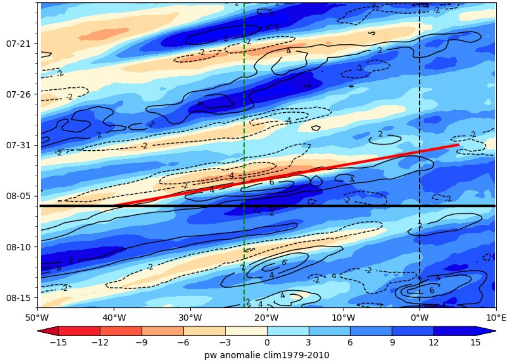
ECMWF PW (color) AND V at 925 hPa 2024-08-06
