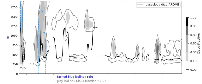
Cross section S/N @ -22W 20240808-12-UTC ech(60h)
