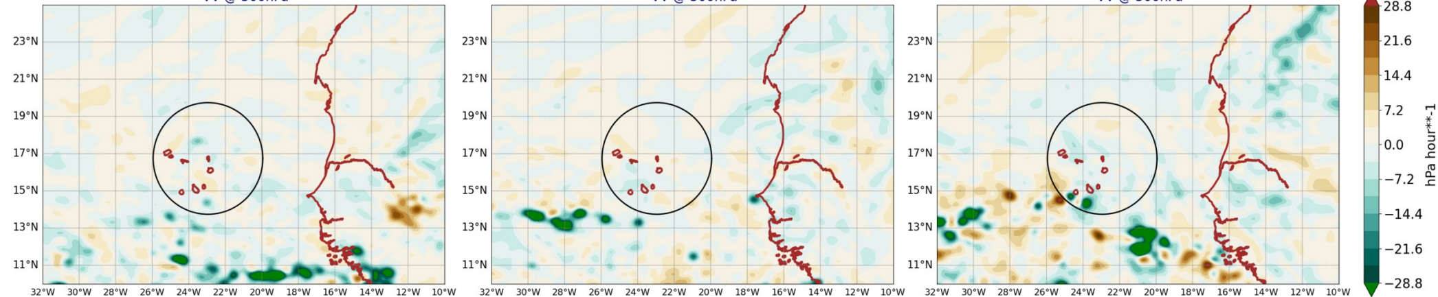
AROME25 20240806-12-UTC -ech(12h) VV @ 500hPa
