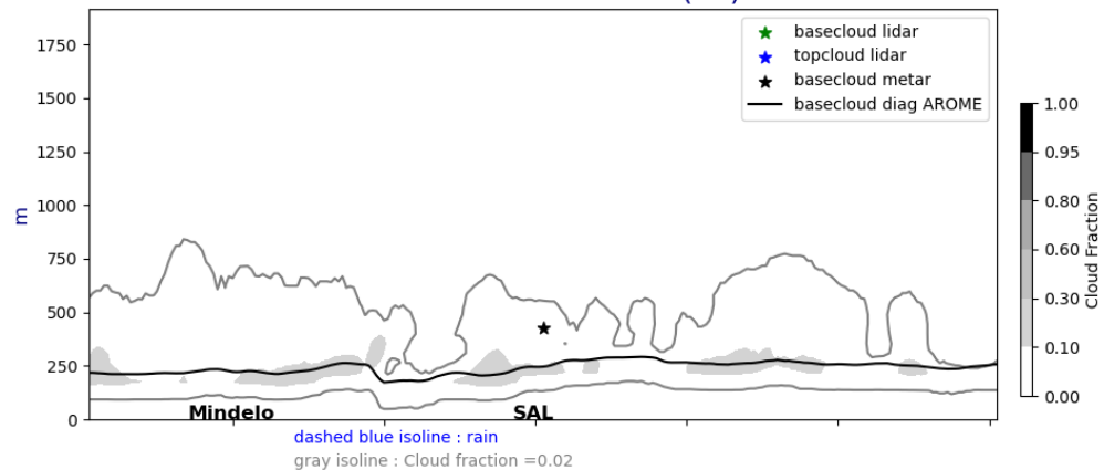
Cross section E/W @ 17.5N 20240806-01-UTC ech(1h)
