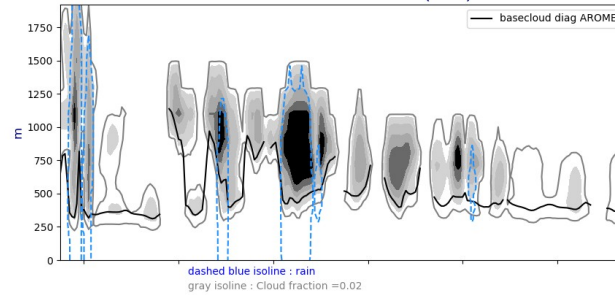
Cross section S/N @ -22W 20240807-12-UTC ech(36h)
