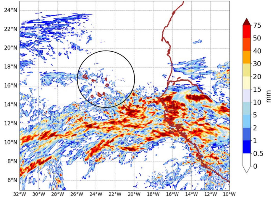
AROME25 20240806-00-UTC -ech(24h)
