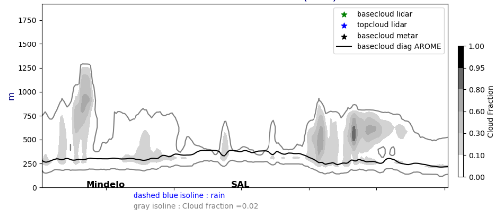
Cross section E/W @ 17.5N 20240806-12-UTC ech(12h)
