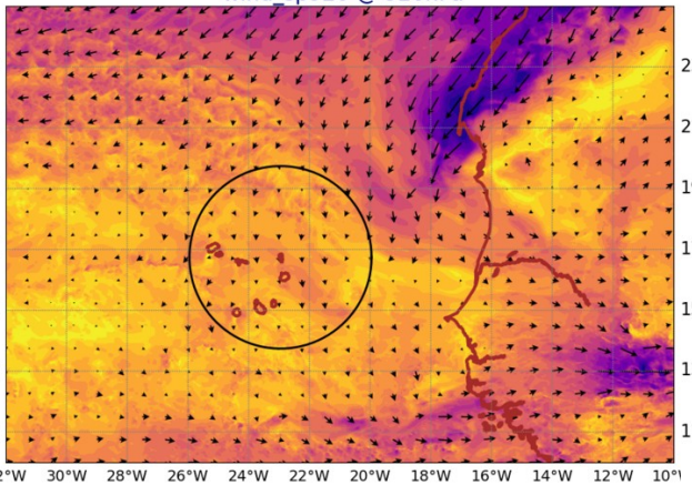
AROME25 20240806-12-UTC -ech(12h) wind_sp920 @ 920hPa
