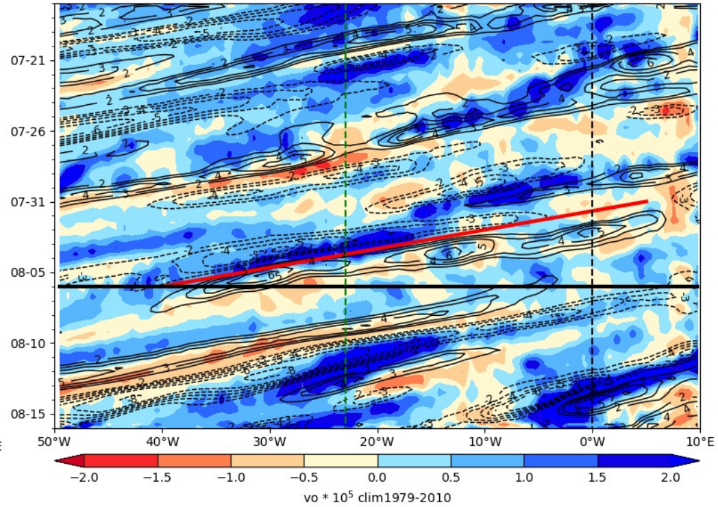
ECMWF Vorticity 850 hPa (color), V-700 hPa 2024-08-06
