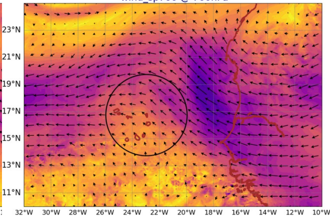
AROME25 20240808-12-UTC -ech(60h) wind_sp920 @ 920hPa
