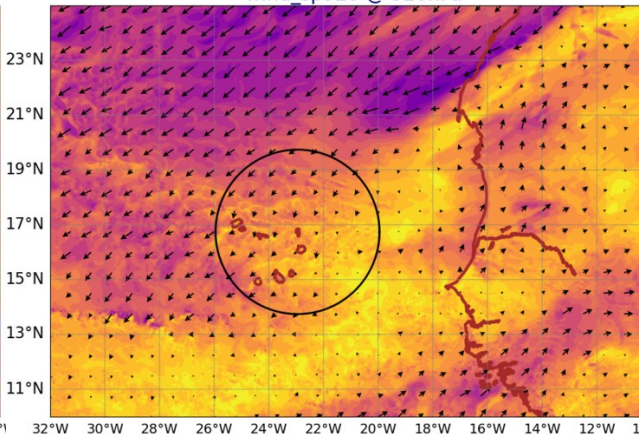
AROME25 20240807-12-UTC -ech(36h) wind_sp920 @ 920hPa
