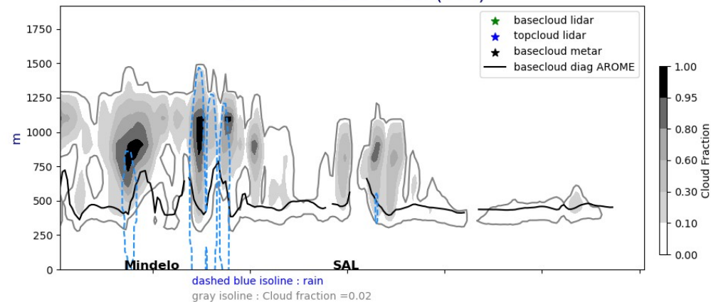
Cross section E/W @ 17.5N 20240808-12-UTC ech(60h)
