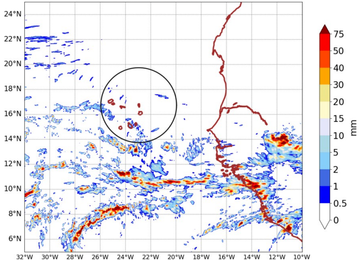
AROME25 20240806-15-UTC -ech(15h) RR cumulated over 6h
