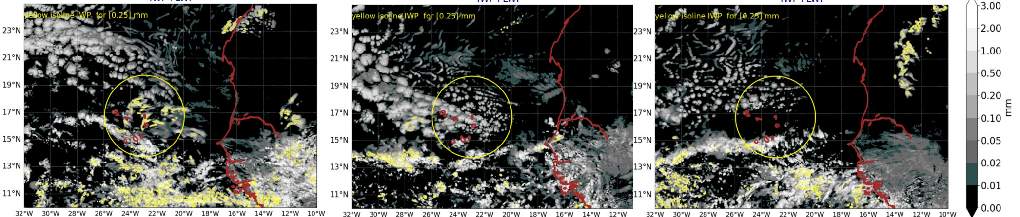
AROME25 20240806-12-UTC -ech(12h) IWP+LWP
