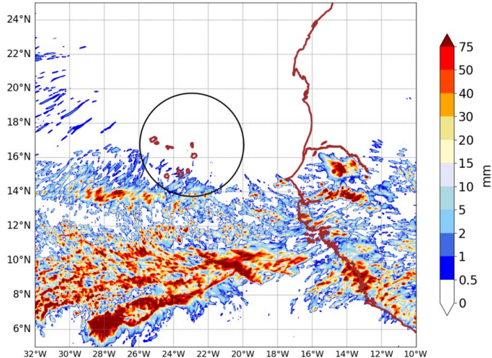
AROME25 20240808-12-UTC -ech(60h) RR cumulated over 24h
