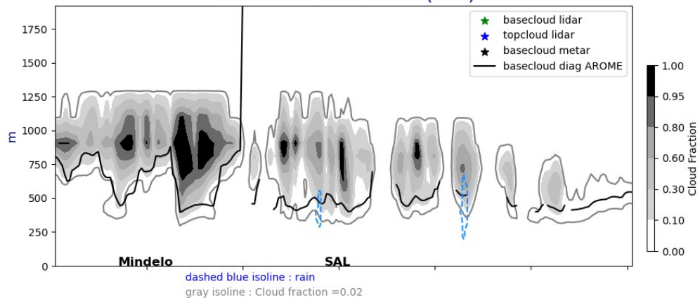
Cross section E/W @ 17.5N 20240807-12-UTC ech(36h)
