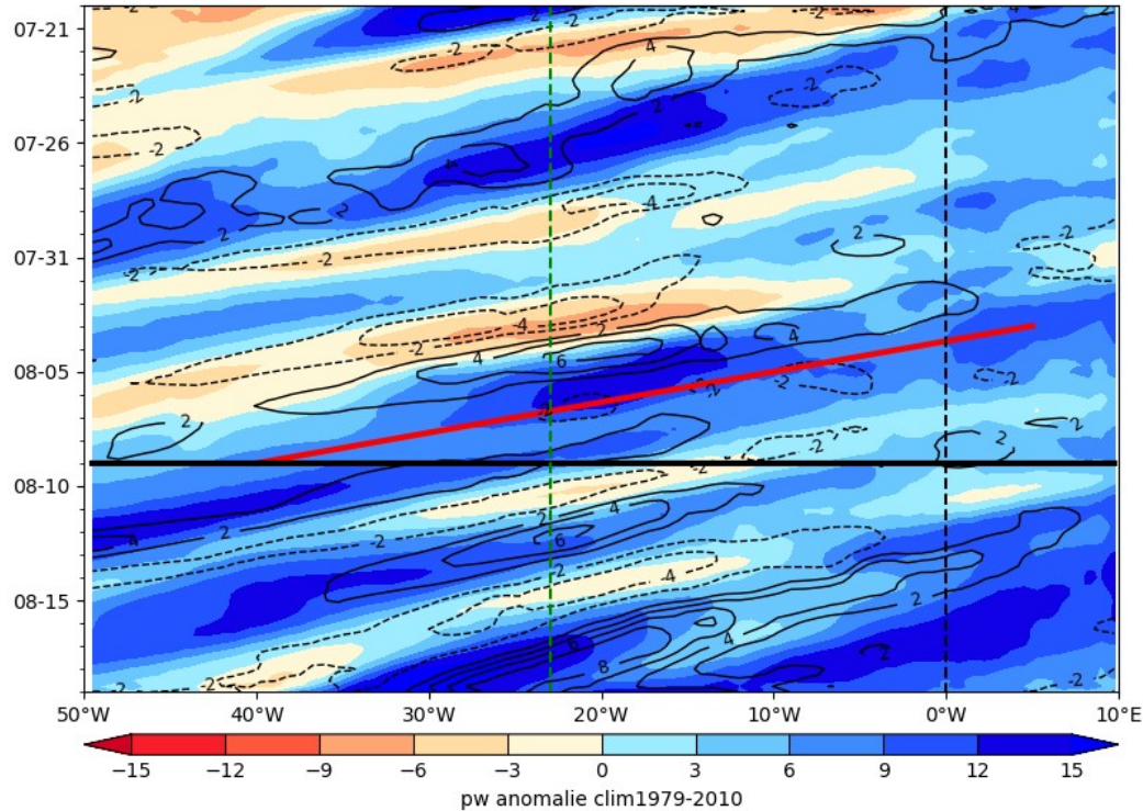
ECMWF PW (color) AND V at 925 hPa 2024-08-09
