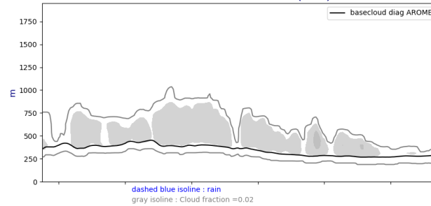
Cross section S/N @ -22W 20240810-12-UTC ech(36h)
