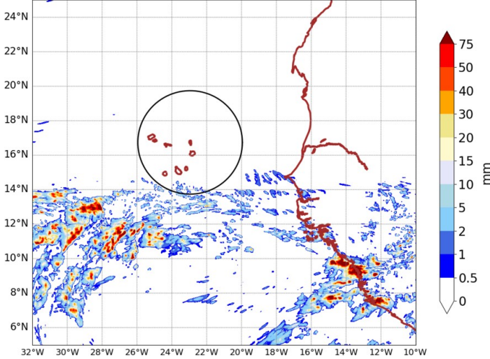
AROME25 20240809-15-UTC -ech(15h) RR cumulated over 6h
