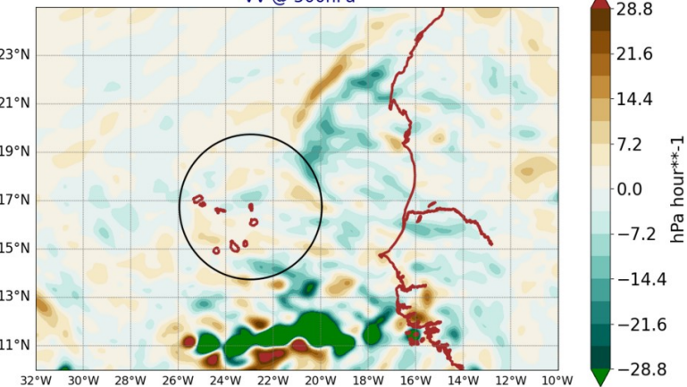
AROME25 20240811-12-UTC -ech(60h) VV @ 500hPa
