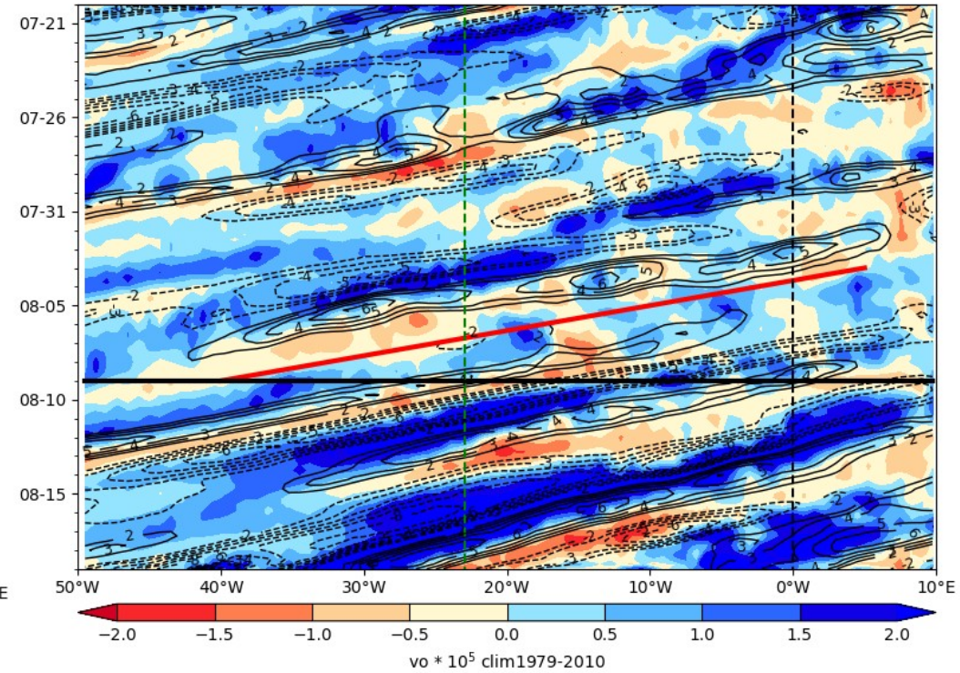
ECMWF Vorticity 850 hPa (color), V-700 hPa 2024-08-09
