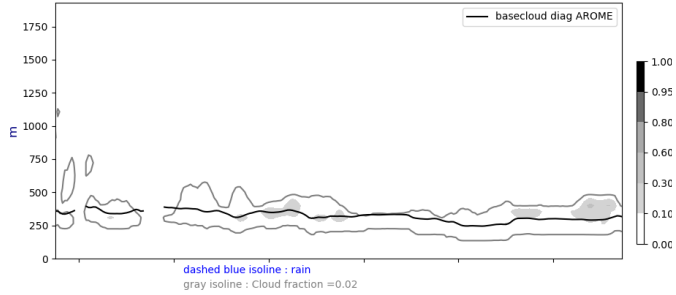
Cross section S/N @ -22W 20240809-12-UTC ech(12h)
