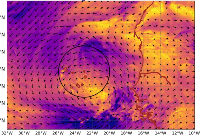
AROME25 20240811-12-UTC -ech(60h) wind_sp920 @ 920hPa
