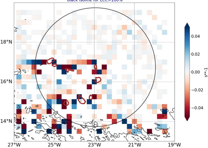
AROME25 regrid 0.25 20240809-12-UTC -ech(12h) blue for conv in subcloud layer black isoline for LCC>100%
