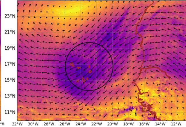
AROME25 20240810-12-UTC -ech(36h) wind_sp920 @ 920hPa
