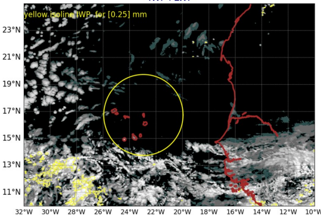
AROME25 20240809-12-UTC -ech(12h) IWP+LWP
