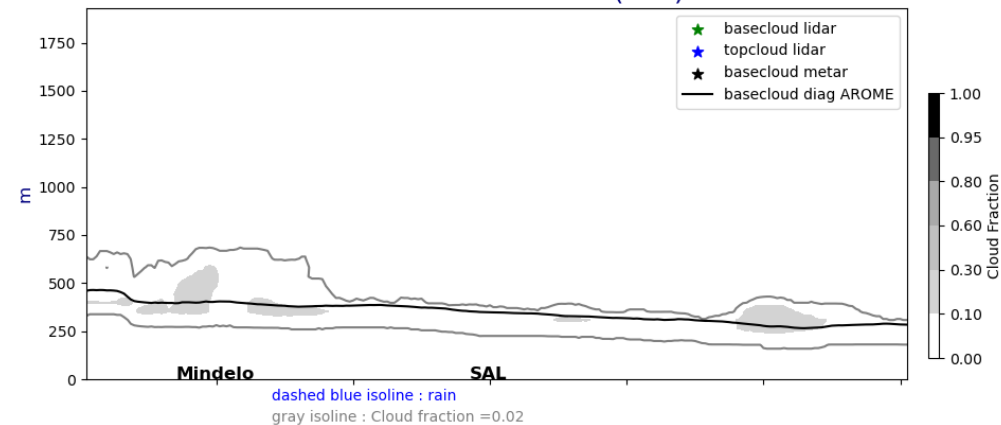
Cross section E/W @ 17.5N 20240809-12-UTC ech(12h)
