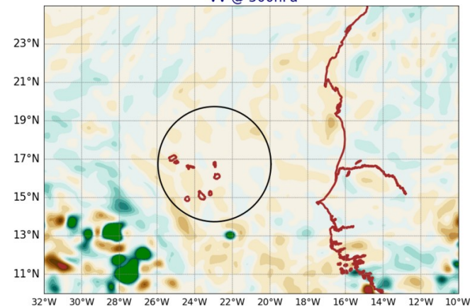
AROME25 20240809-12-UTC -ech(12h) VV @ 500hPa
