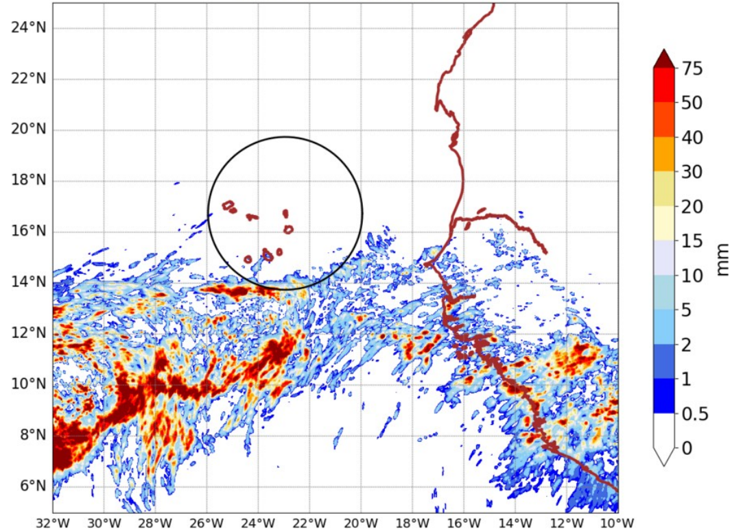
AROME25 20240809-00-UTC -ech(24h)
