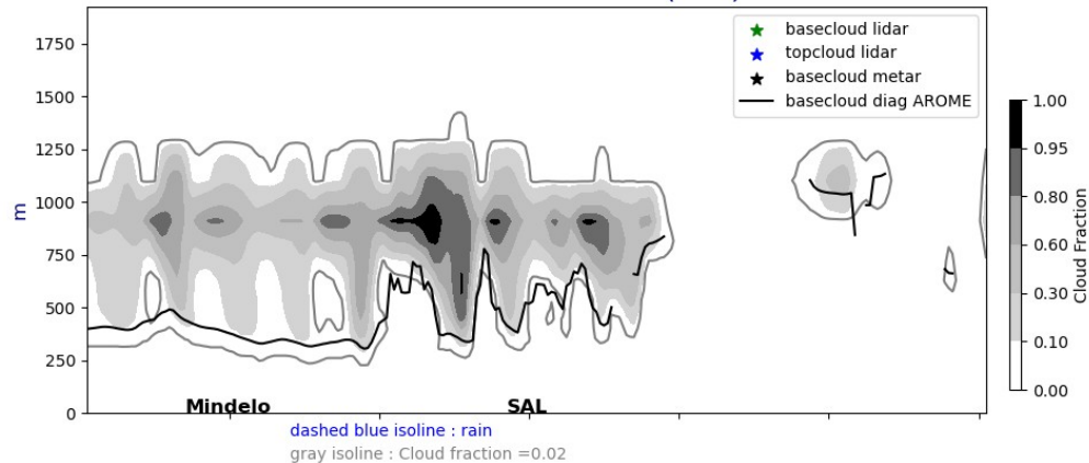
Cross section E/W @ 17.5N 20240811-12-UTC ech(60h)
