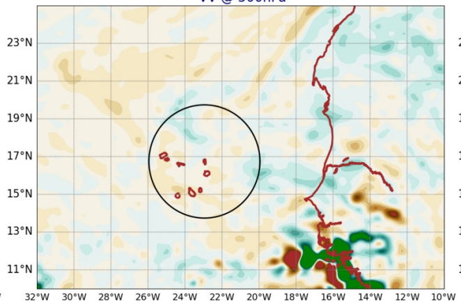
AROME25 20240810-12-UTC -ech(36h) VV @ 500hPa
