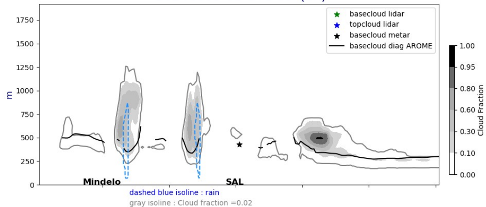
Cross section E/W @ 17.5N 20240809-01-UTC ech(1h)
