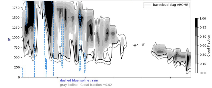
Cross section S/N @ -22W 20240811-12-UTC ech(60h)
