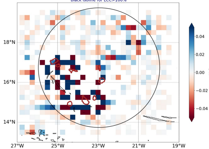
AROME25 regrid 0.25 20240810-12-UTC -ech(36h) blue for conv in subcloud layer black isoline for LCC>100%
