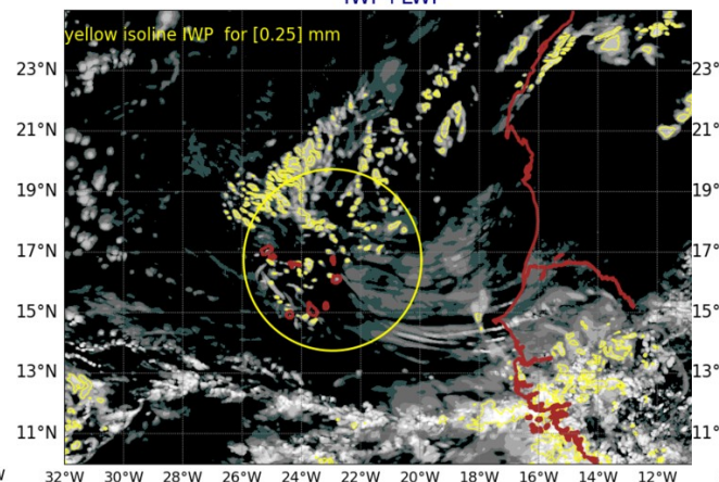
AROME25 20240810-12-UTC -ech(36h) IWP+LWP
