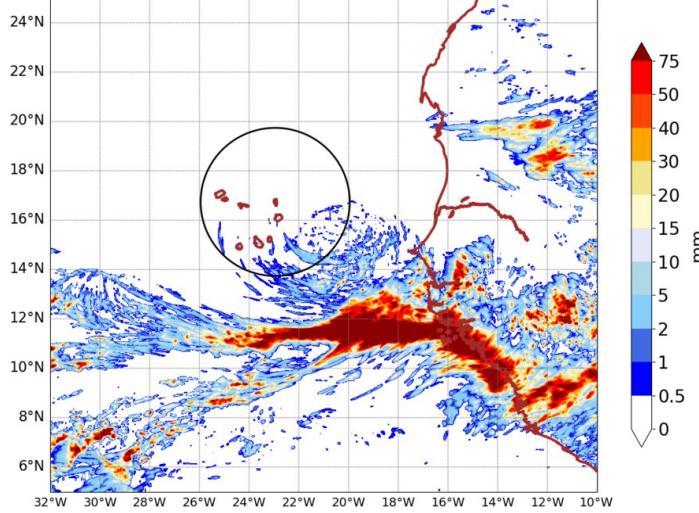
AROME25 20240811-12-UTC -ech(60h) RR cumulated over 24h
