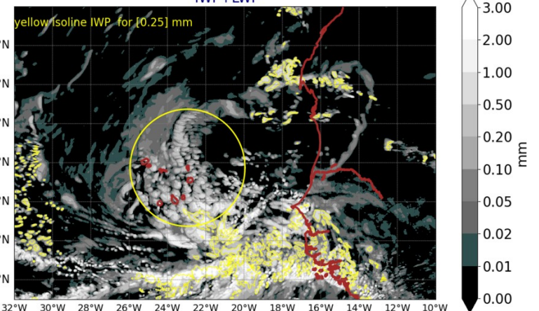
AROME25 20240811-12-UTC -ech(60h) IWP+LWP
