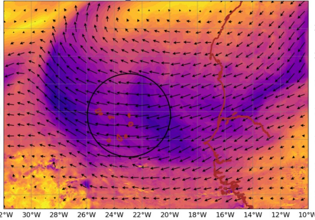
AROME25 20240809-12-UTC -ech(12h) wind_sp920 @ 920hPa
