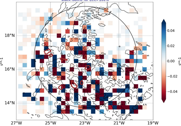
AROME25 regrid 0.25 20240811-12-UTC -ech(60h) blue for conv in subcloud layer black isoline for LCC>100%
