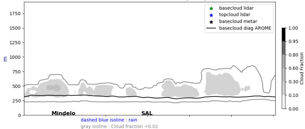
Cross section E/W @ 17.5N 20240810-12-UTC ech(36h)
