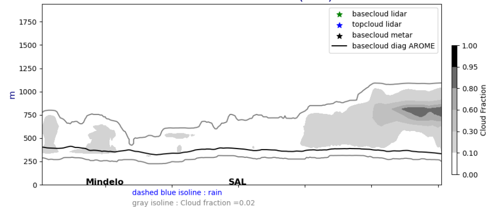
Cross section E/W @ 17.5N 20240810-12-UTC ech(12h)
