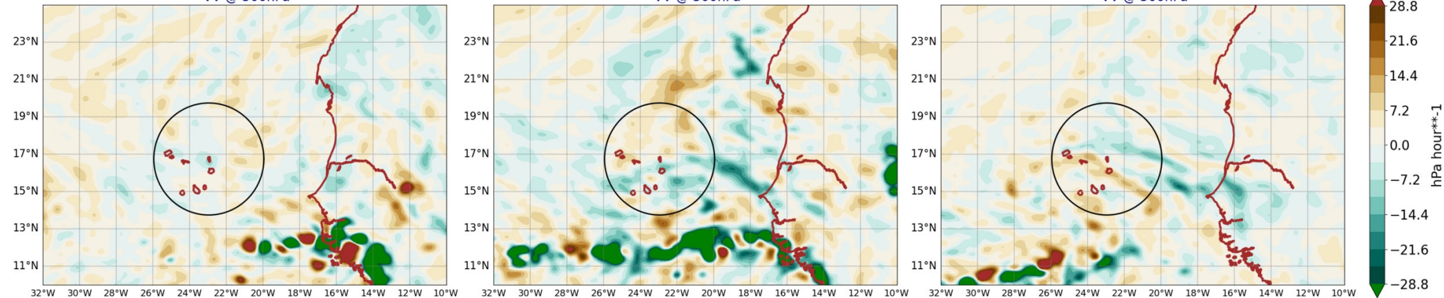
AROME25 20240810-12-UTC -ech(12h) VV @ 500hPa
