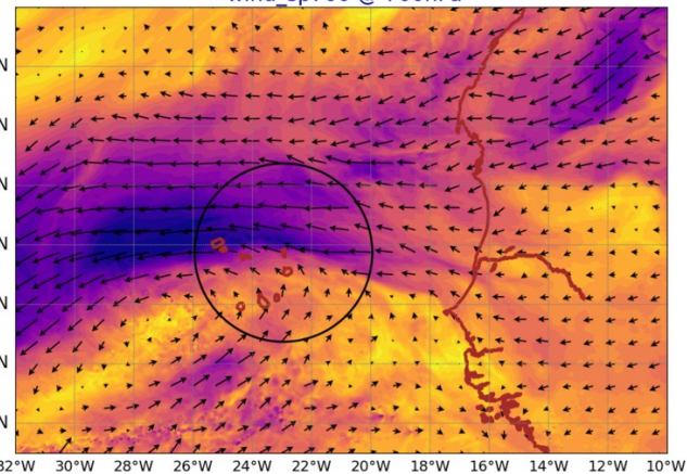
AROME25 20240812-12-UTC -ech(60h) wind_sp920 @ 920hPa
