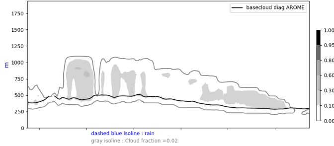
Cross section S/N @ -22W 20240810-12-UTC ech(12h)
