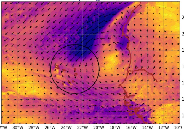
AROME25 20240810-12-UTC -ech(12h) wind_sp920 @ 920hPa
