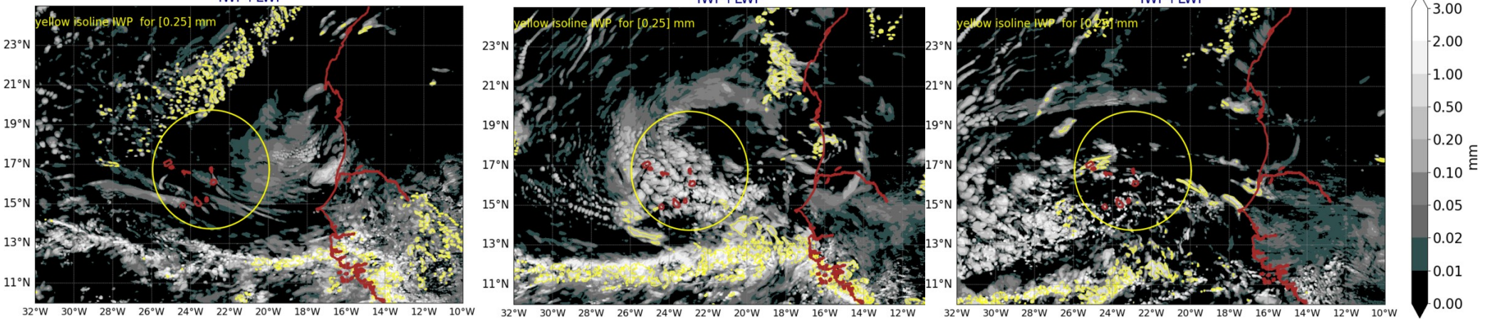
AROME25 20240810-12-UTC -ech(12h) IWP+LWP
