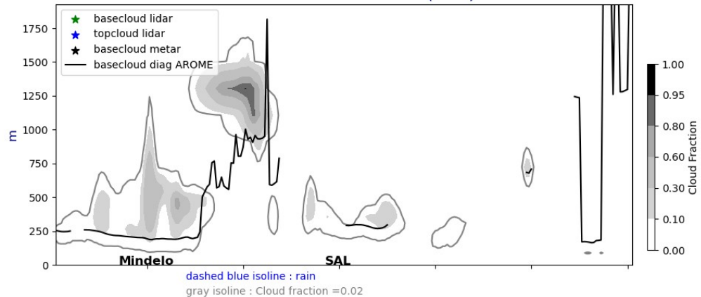
Cross section E/W @ 17.5N 20240812-12-UTC ech(60h)
