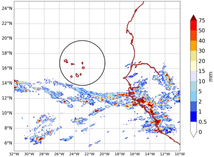
AROME25 20240810-15-UTC -ech(15h) RR cumulated over 6h
