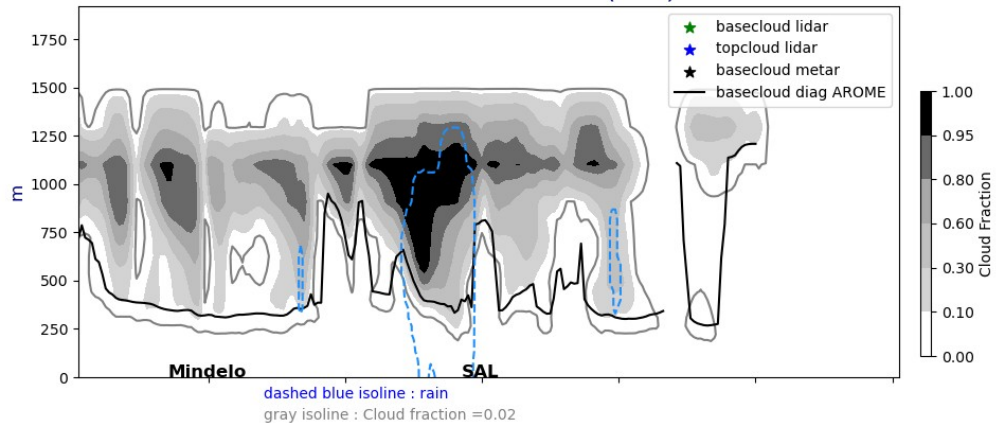
Cross section E/W @ 17.5N 20240811-12-UTC ech(36h)
