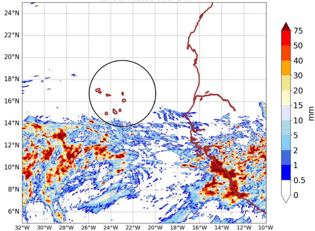
AROME25 20240810-00-UTC -ech(24h) RR cumulated over 24h
