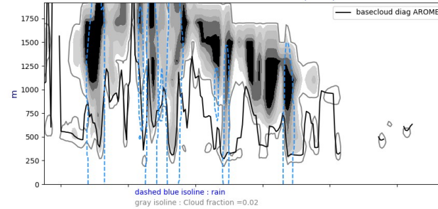
Cross section S/N @ -22W 20240811-12-UTC ech(36h)
