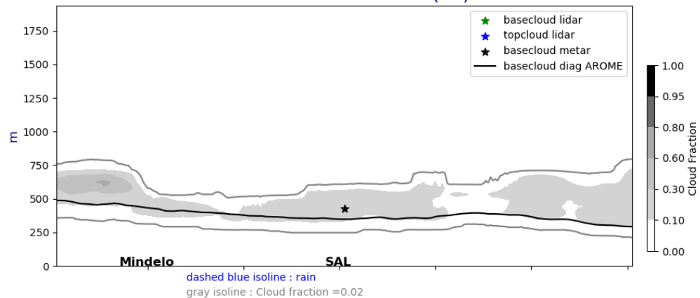
Cross section E/W @ 17.5N 20240810-01-UTC ech(1h)
