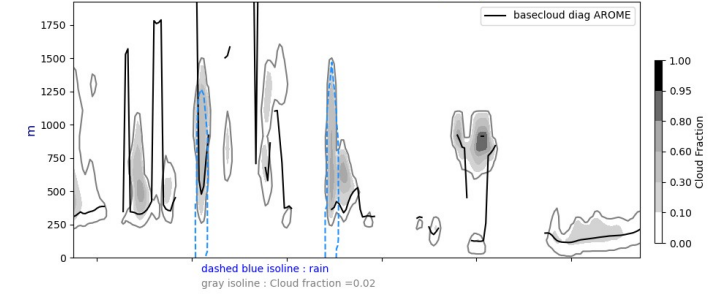
Cross section S/N @ -22W 20240812-12-UTC ech(60h)
