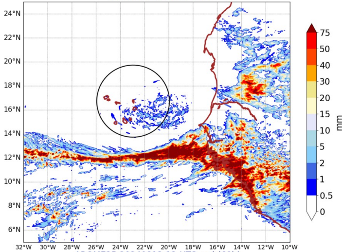
AROME25 20240812-12-UTC -ech(60h) RR cumulated over 24h
