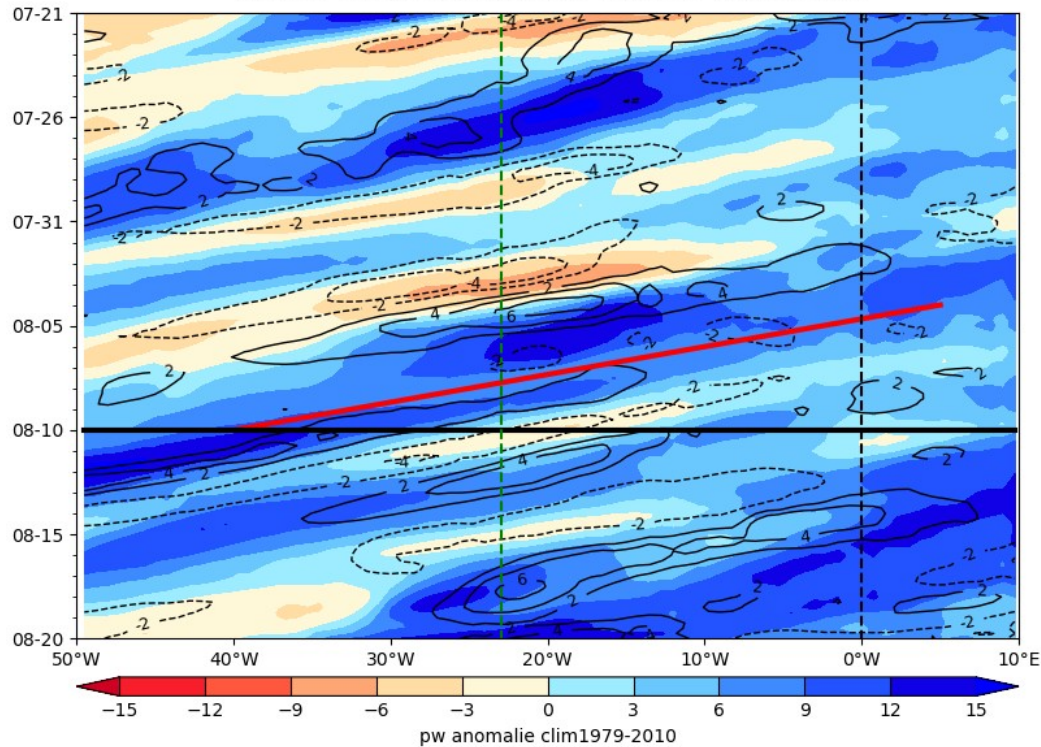
ECMWF PW (color) AND V at 925 hPa 2024-08-10
