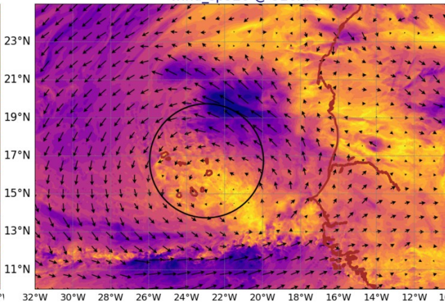
AROME25 20240811-12-UTC -ech(36h) wind_sp920 @ 920hPa
