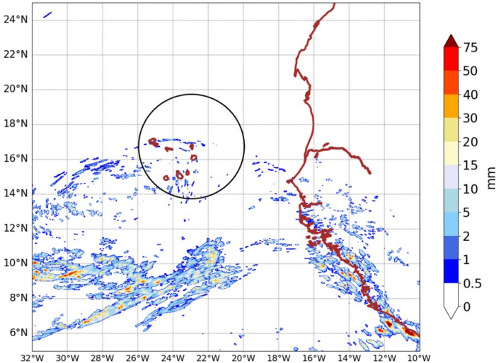
AROME25 20240812-15-UTC -ech(15h) RR cumulated over 6h
