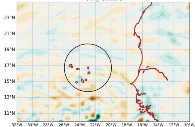
AROME25 20240812-12-UTC -ech(12h) VV @ 500hPa
