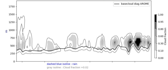
Cross section S/N @ -22W 20240814-12-UTC ech(60h)
