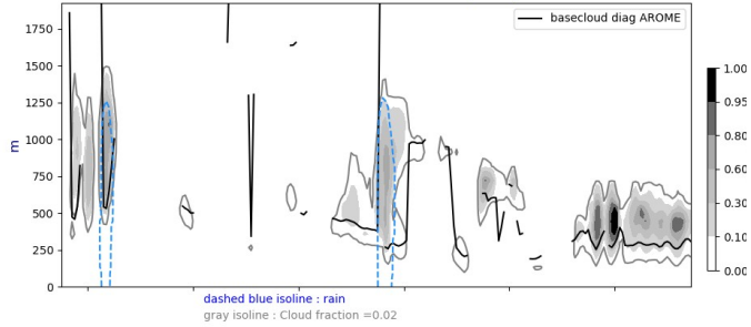
Cross section S/N @ -22W 20240812-12-UTC ech(12h)
