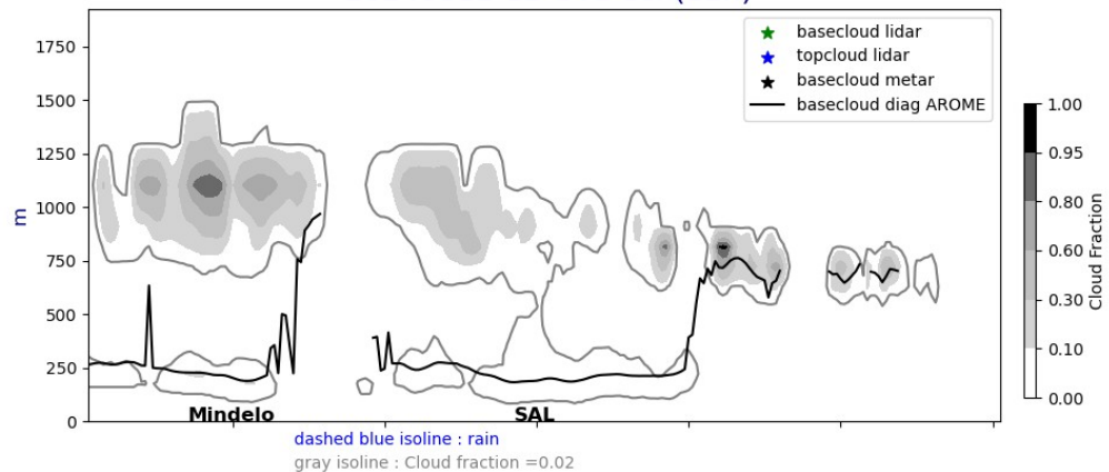
Cross section E/W @ 17.5N 20240812-12-UTC ech(12h)
