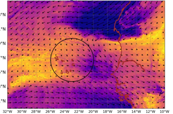
AROME25 20240814-12-UTC -ech(60h) wind_sp920 @ 920hPa
