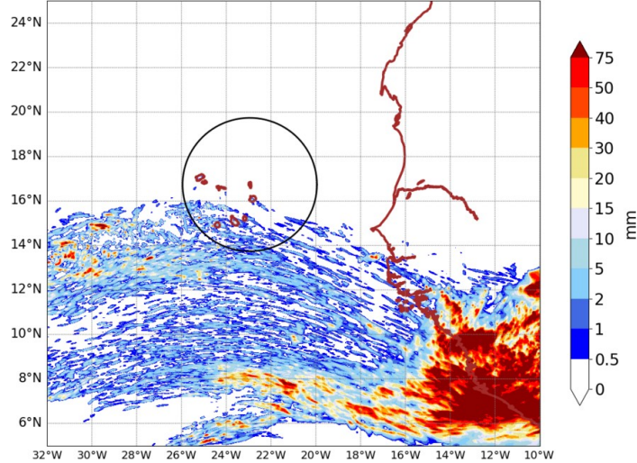
AROME25 20240814-12-UTC -ech(60h) RR cumulated over 24h
