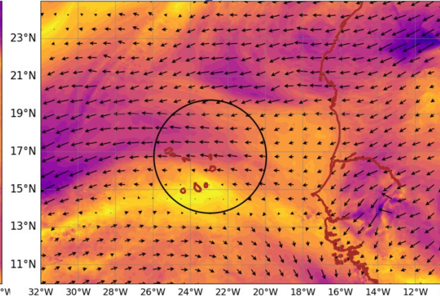
AROME25 20240813-12-UTC -ech(36h) wind_sp920 @ 920hPa
