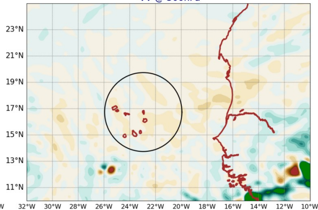
AROME25 20240814-12-UTC -ech(60h) VV @ 500hPa
