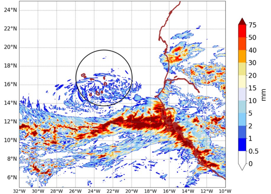
AROME25 20240812-00-UTC -ech(24h)
