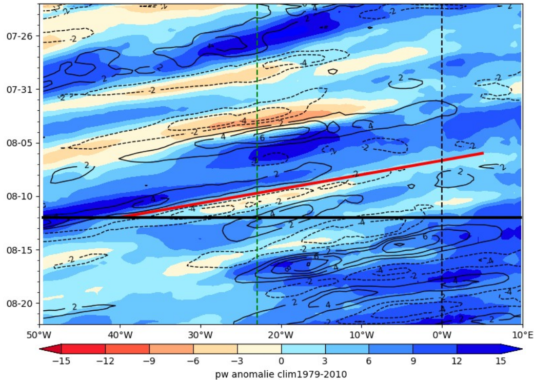
ECMWF PW (color) AND V at 925 hPa 2024-08-12
