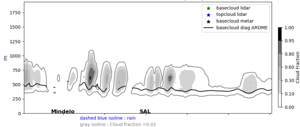
Cross section E/W @ 17.5N 20240814-12-UTC ech(60h)
