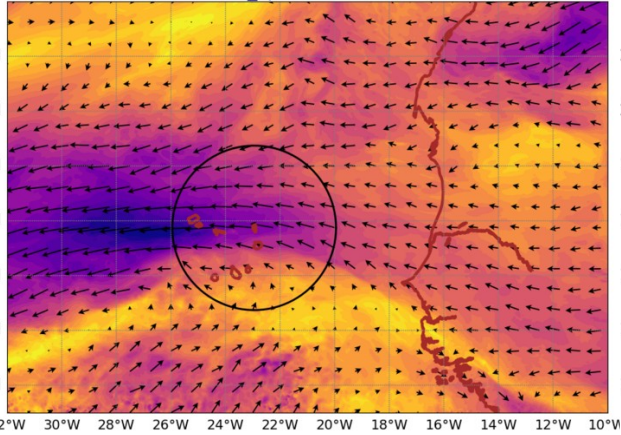
AROME25 20240812-12-UTC -ech(12h) wind_sp920 @ 920hPa
