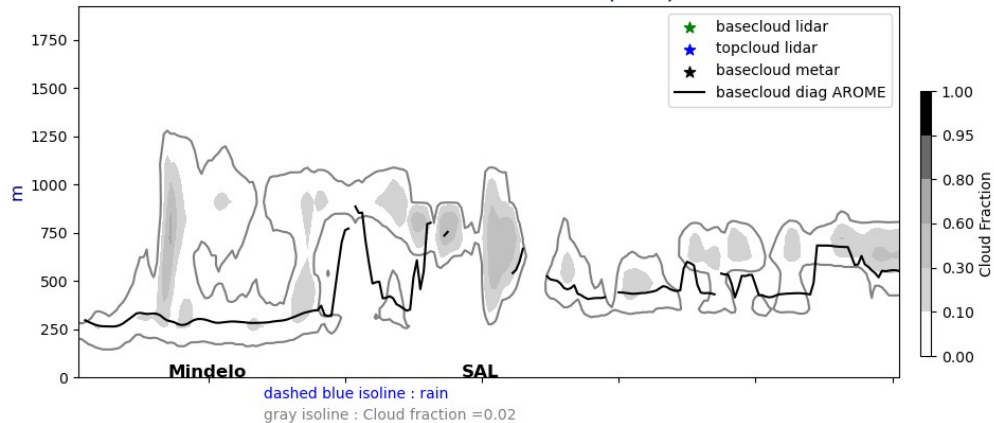
Cross section E/W @ 17.5N 20240813-12-UTC ech(36h)
