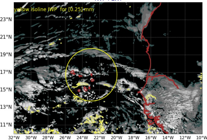
AROME25 20240812-12-UTC -ech(12h) IWP+LWP
