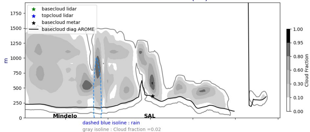
Cross section E/W @ 17.5N 20240812-01-UTC ech(1h)
