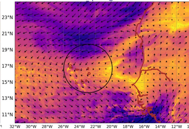
AROME25 20240815-12-UTC -ech(36h) wind_sp920 @ 920hPa
