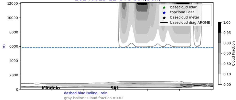
Cross section E/W @ 17.5N 20240815-12-UTC ech(36h)
