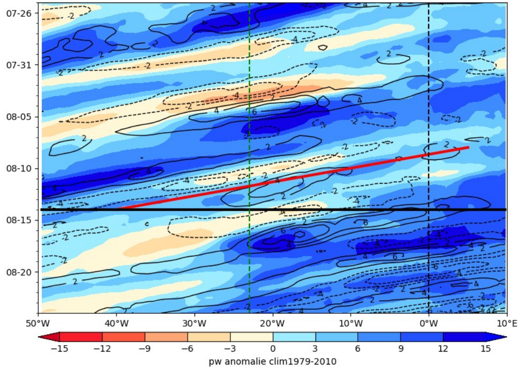
ECMWF PW (color) AND V at 925 hPa 2024-08-14
