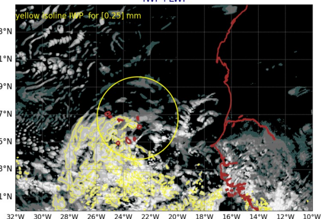
AROME25 20240816-12-UTC -ech(60h) IWP+LWP
