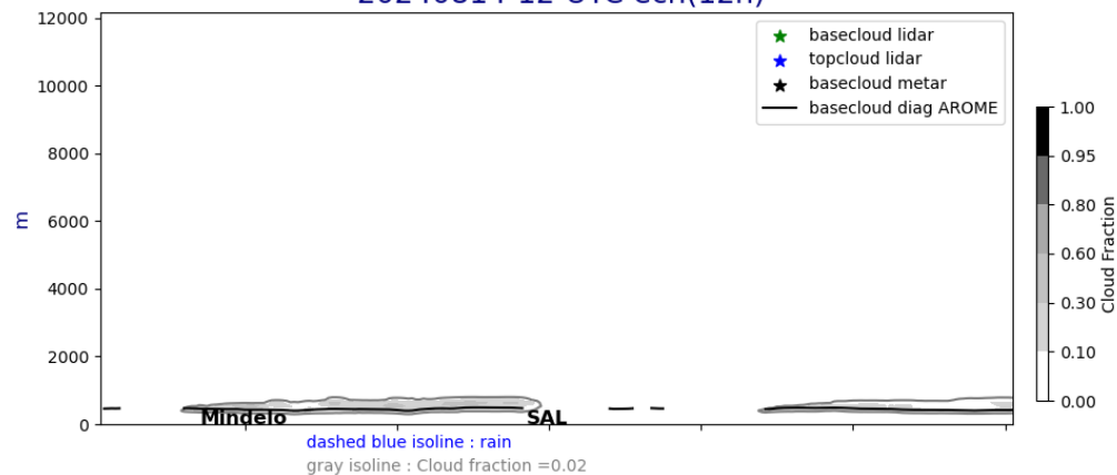
Cross section E/W @ 17.5N 20240814-12-UTC ech(12h)
