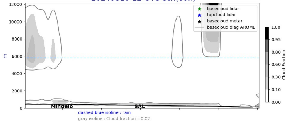
Cross section E/W @ 17.5N 20240816-12-UTC ech(60h)
