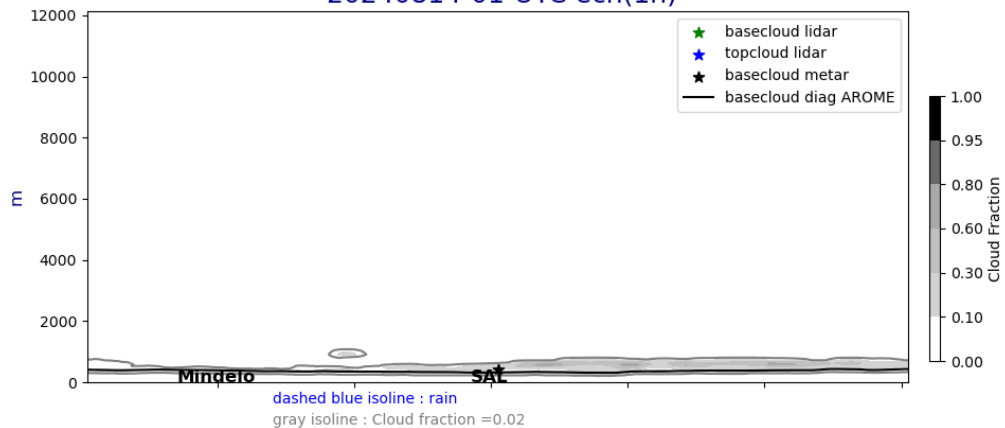
Cross section E/W @ 17.5N 20240814-01-UTC ech(1h)
