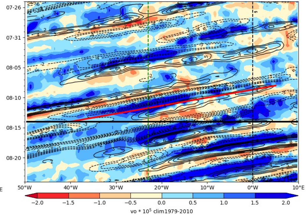
ECMWF Vorticity 850 hPa (color), V-700 hPa 2024-08-14
