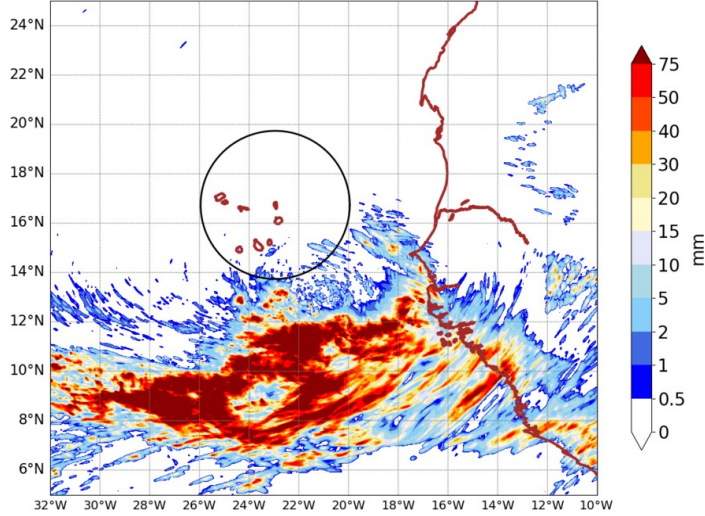
AROME25 20240816-12-UTC -ech(60h) RR cumulated over 24h
