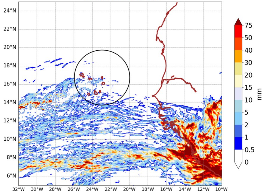
AROME25 20240814-00-UTC -ech(24h) RR cumulated over 24h
