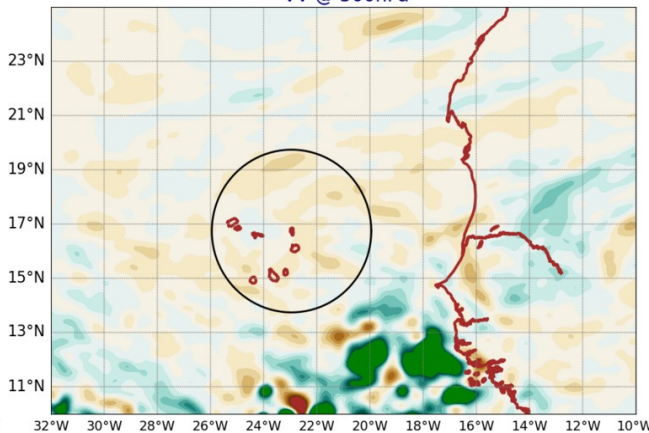
AROME25 20240815-12-UTC -ech(36h) VV @ 500hPa
