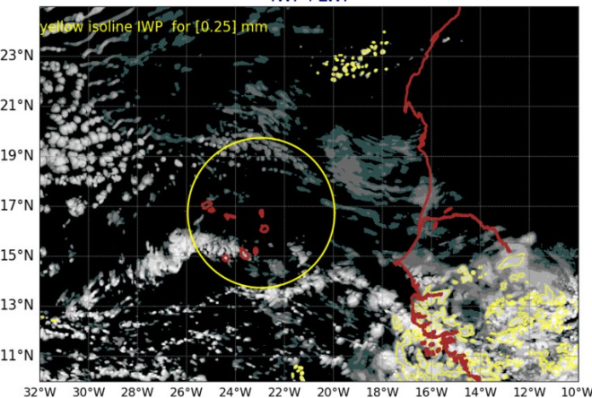
AROME25 20240814-12-UTC -ech(12h) IWP+LWP
