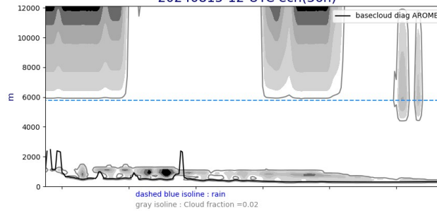
Cross section S/N @ -22W 20240815-12-UTC ech(36h)
