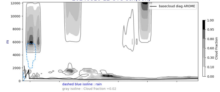
Cross section S/N @ -22W 20240816-12-UTC ech(60h)
