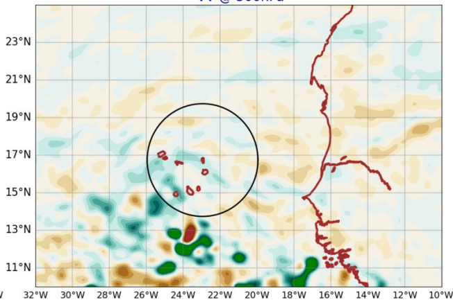
AROME25 20240816-12-UTC -ech(60h) VV @ 500hPa
