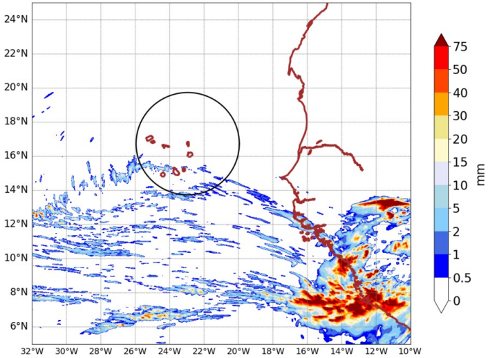
AROME25 20240814-15-UTC -ech(15h) RR cumulated over 6h
