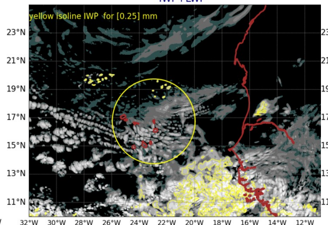
AROME25 20240815-12-UTC -ech(36h) IWP+LWP
