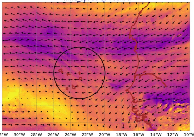
AROME25 20240814-12-UTC -ech(12h) wind_sp920 @ 920hPa
