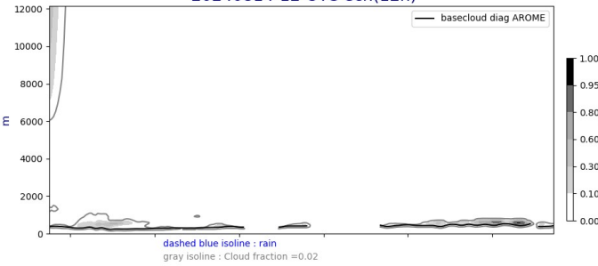
Cross section S/N @ -22W 20240814-12-UTC ech(12h)
