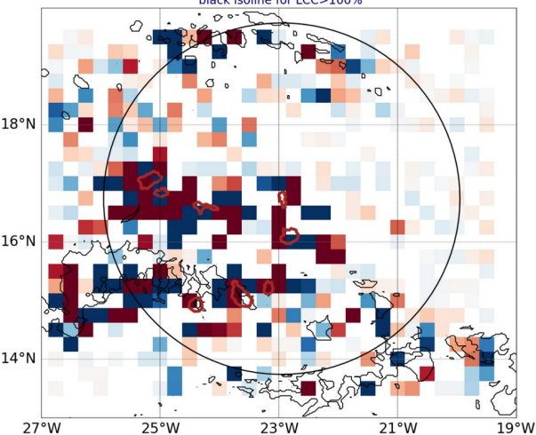
white box where subcloud and cloud layer have same sign of div
