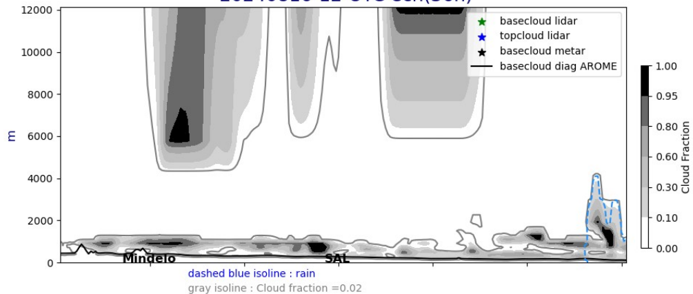
Cross section E/W @ 17.5N 20240816-12-UTC ech(36h)
