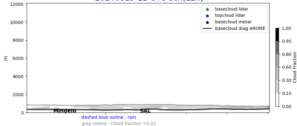
Cross section E/W @ 17.5N 20240815-12-UTC ech(12h)
