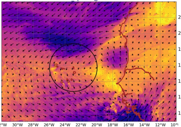
AROME25 20240815-12-UTC -ech(12h) wind_sp920 @ 920hPa
