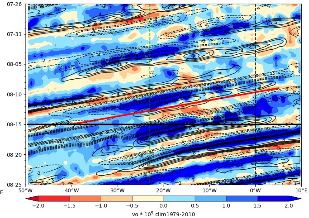
ECMWF Vorticity 850 hPa (color), V-700 hPa 2024-08-15
