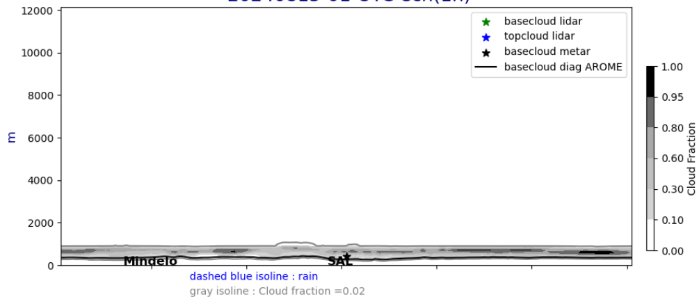
Cross section E/W @ 17.5N 20240815-01-UTC ech(1h)
