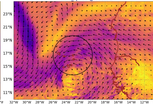
AROME25 20240816-12-UTC -ech(36h) wind_sp920 @ 920hPa
