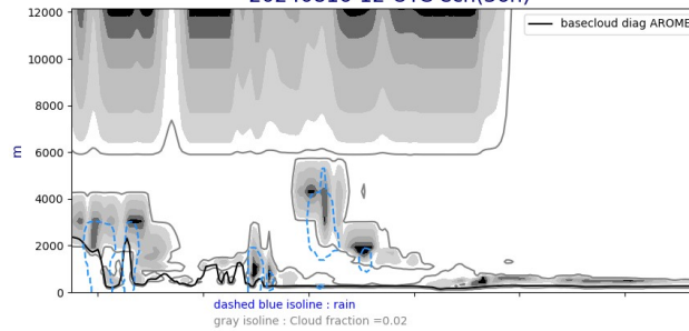
Cross section S/N @ -22W 20240816-12-UTC ech(36h)
