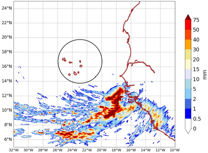
AROME25 20240815-15-UTC -ech(15h) RR cumulated over 6h
