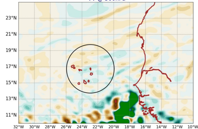
AROME25 20240815-12-UTC -ech(12h) VV @ 500hPa
