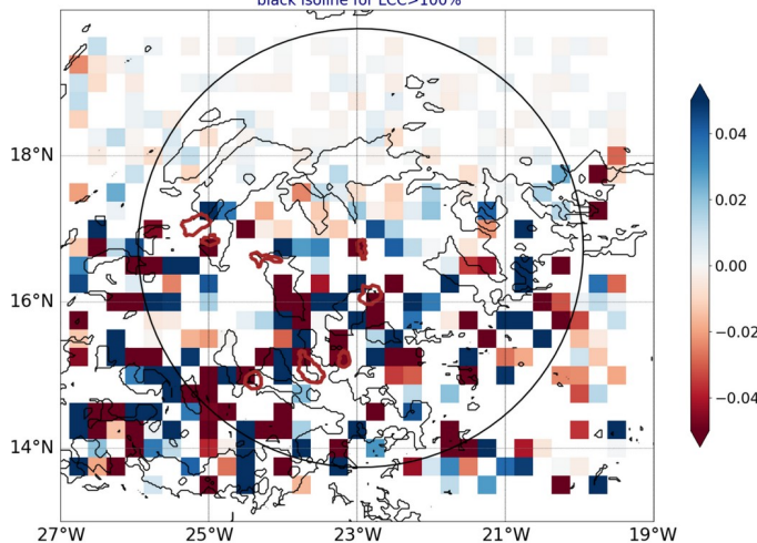
AROME25 regrid 0.25 20240816-12-UTC -ech(36h) blue for conv in subcloud layer black isoline for LCC>100%
