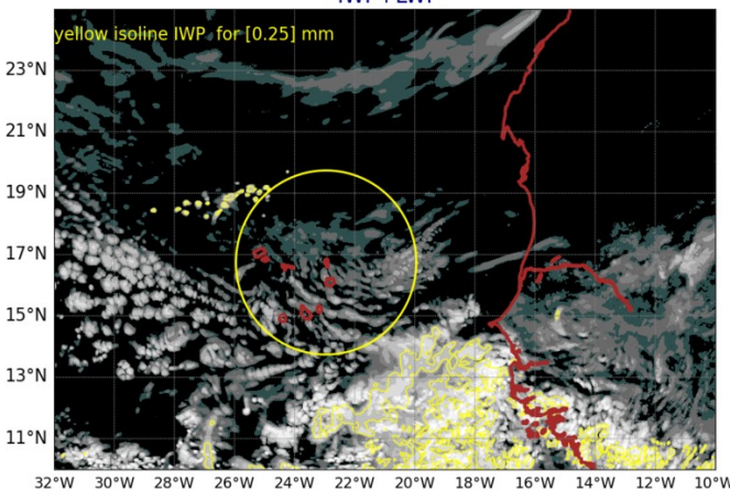
AROME25 20240815-12-UTC -ech(12h) IWP+LWP
