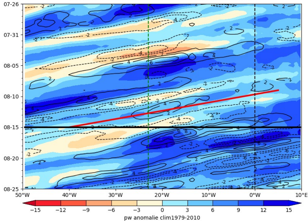
ECMWF PW (color) AND V at 925 hPa 2024-08-15
