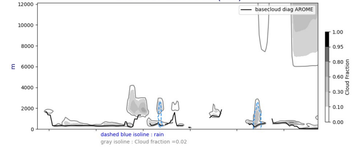
Cross section S/N @ -22W 20240817-12-UTC ech(60h)
