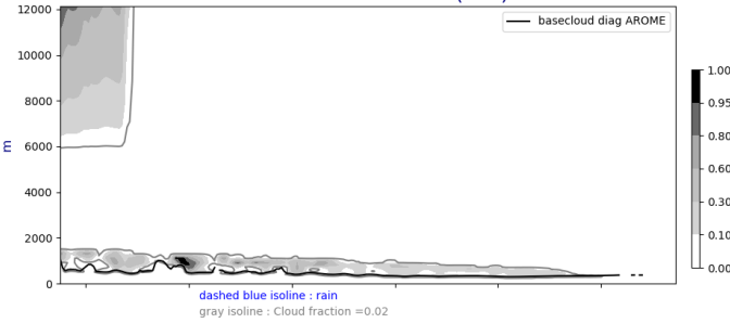
Cross section S/N @ -22W 20240815-12-UTC ech(12h)
