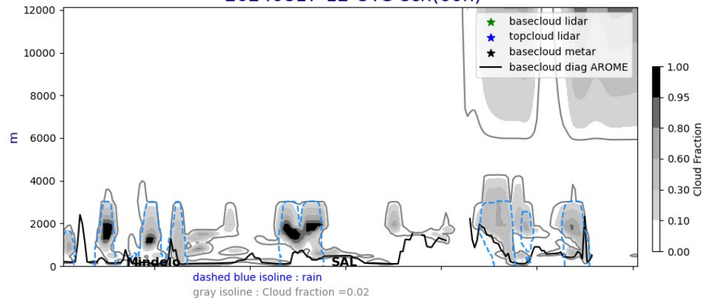
Cross section E/W @ 17.5N 20240817-12-UTC ech(60h)
