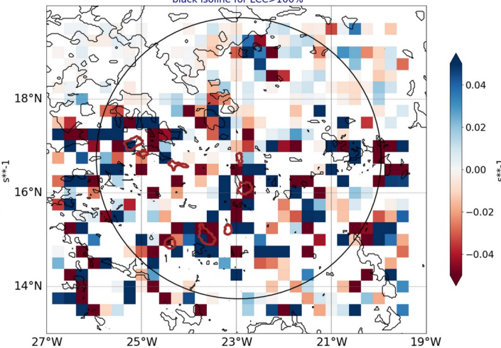
AROME25 regrid 0.25 20240817-12-UTC -ech(60h) blue for conv in subcloud layer black isoline for LCC>100%
