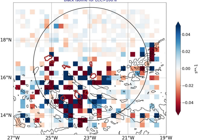
AROME25 regrid 0.25 20240815-12-UTC -ech(12h) blue for conv in subcloud layer black isoline for LCC>100%
