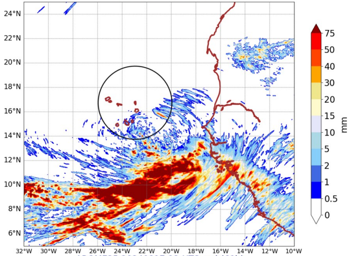
AROME25 20240817-12-UTC -ech(60h) RR cumulated over 24h
