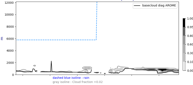
Cross section S/N @ -22W 20240816-12-UTC ech(12h)
