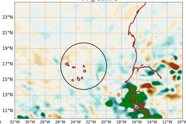
AROME25 20240818-12-UTC -ech(60h) VV @ 500hPa
