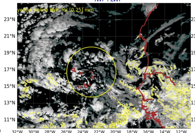
AROME25 20240817-12-UTC -ech(36h) IWP+LWP
