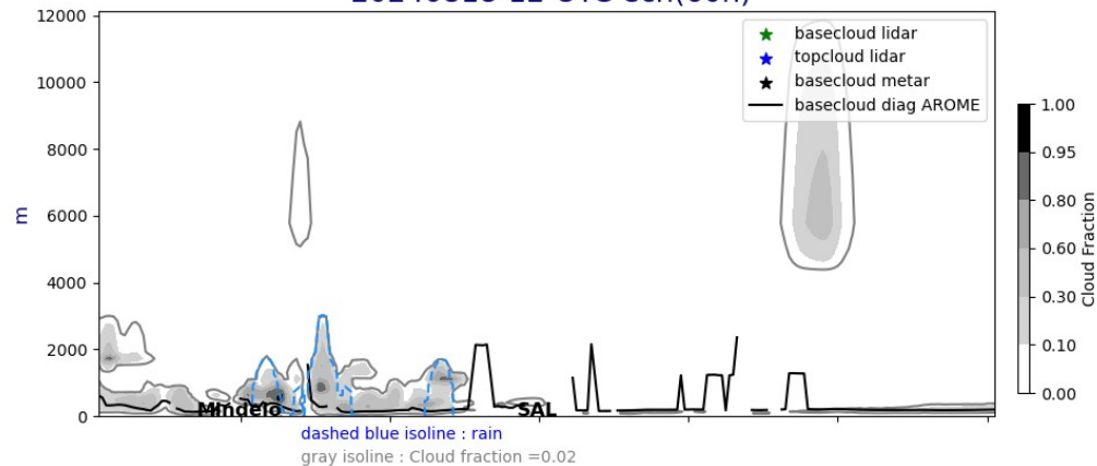
Cross section E/W @ 17.5N 20240818-12-UTC ech(60h)
