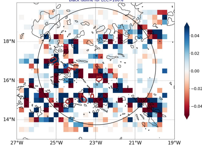
AROME25 regrid 0.25 20240817-12-UTC -ech(36h) blue for conv in subcloud layer black isoline for LCC>100%
