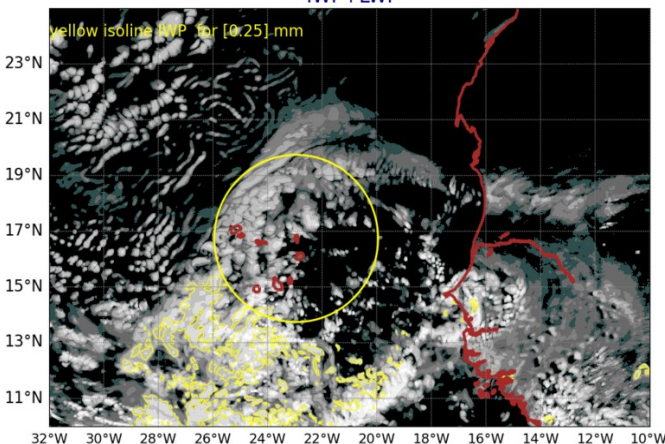
AROME25 20240816-12-UTC -ech(12h) IWP+LWP
