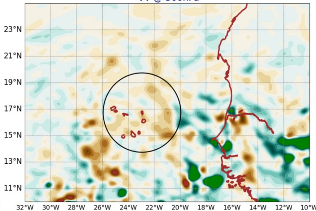
AROME25 20240817-12-UTC -ech(36h) VV @ 500hPa
