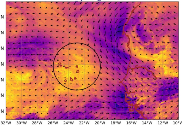
AROME25 20240818-12-UTC -ech(60h) wind_sp920 @ 920hPa
