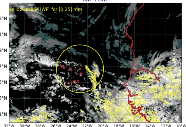
AROME25 20240818-12-UTC -ech(60h) IWP+LWP
