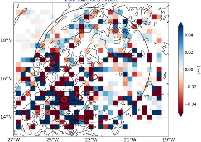
AROME25 regrid 0.25 20240816-12-UTC -ech(12h) blue for conv in subcloud layer black isoline for LCC>100%
