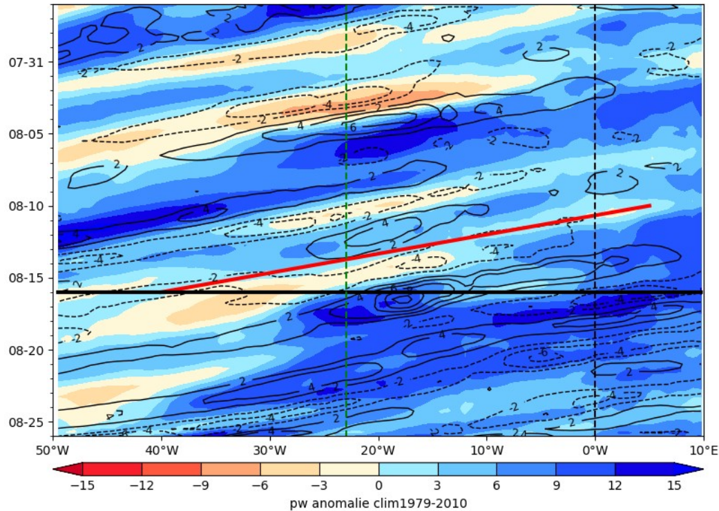
ECMWF PW (color) AND V at 925 hPa 2024-08-16
