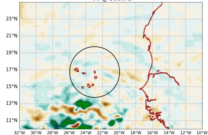
AROME25 20240816-12-UTC -ech(12h) VV @ 500hPa
