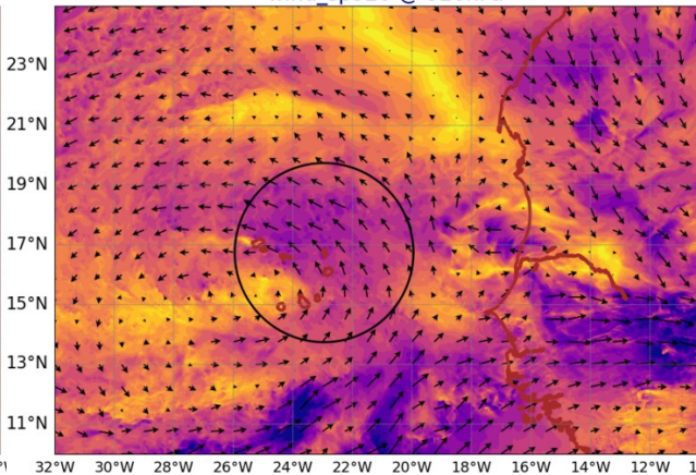
AROME25 20240817-12-UTC -ech(36h) wind_sp920 @ 920hPa
