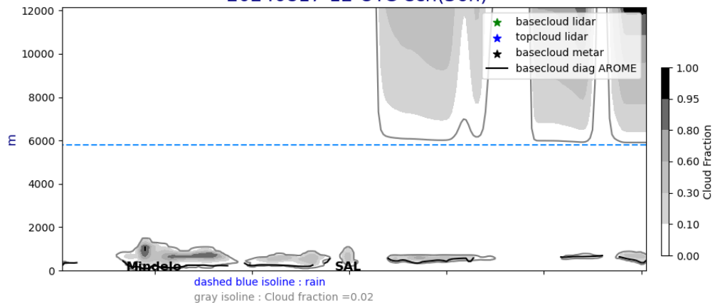
Cross section E/W @ 17.5N 20240817-12-UTC ech(36h)
