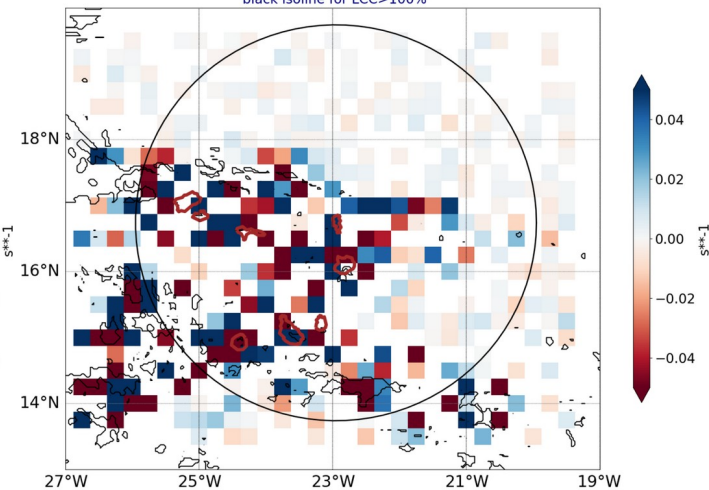
AROME25 regrid 0.25 20240818-12-UTC -ech(60h) blue for conv in subcloud layer black isoline for LCC>100%
