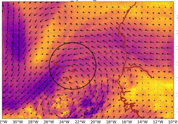
AROME25 20240816-12-UTC -ech(12h) wind_sp920 @ 920hPa
