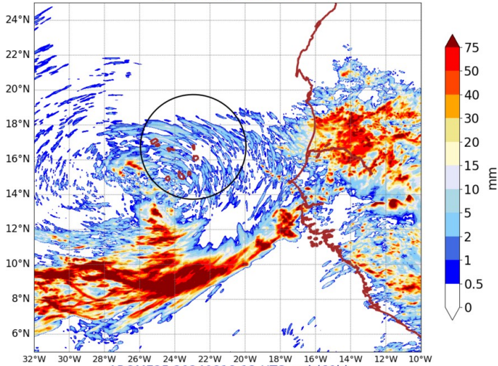
AROME25 20240818-12-UTC -ech(60h) RR cumulated over 24h
