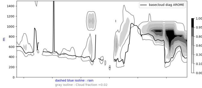
Cross section S/N @ -22W 20240816-12-UTC ech(12h)
