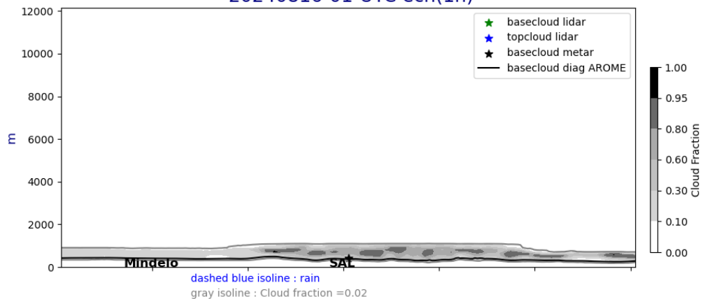
Cross section E/W @ 17.5N 20240816-01-UTC ech(1h)
