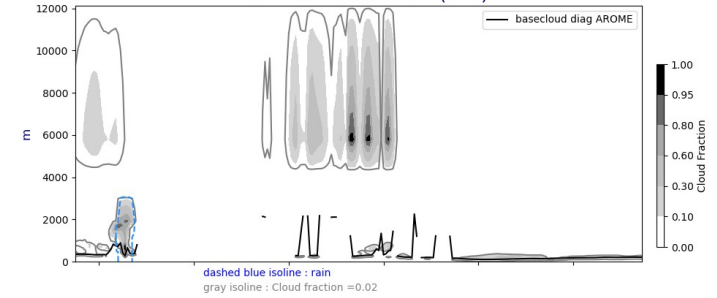
Cross section S/N @ -22W 20240818-12-UTC ech(60h)
