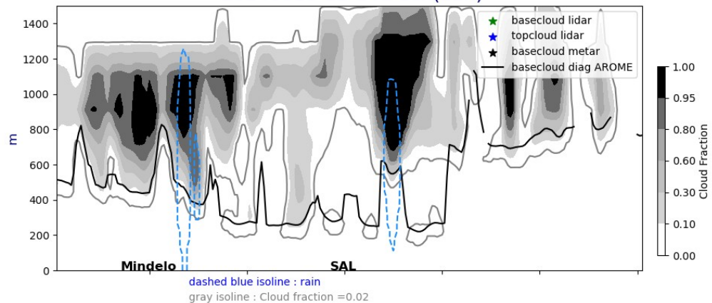
Cross section E/W @ 17.5N 20240816-12-UTC ech(12h)
