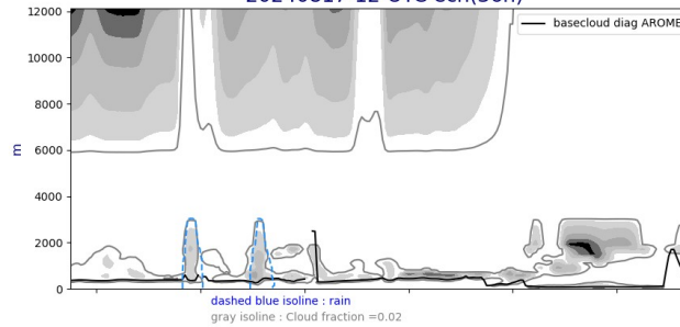
Cross section S/N @ -22W 20240817-12-UTC ech(36h)
