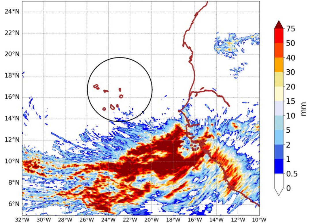
AROME25 20240816-00-UTC -ech(24h)
