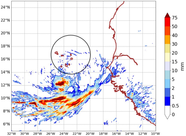
AROME25 20240816-15-UTC -ech(15h) RR cumulated over 6h
