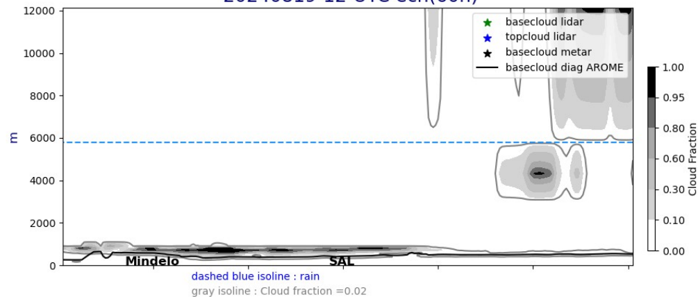
Cross section E/W @ 17.5N 20240819-12-UTC ech(60h)
