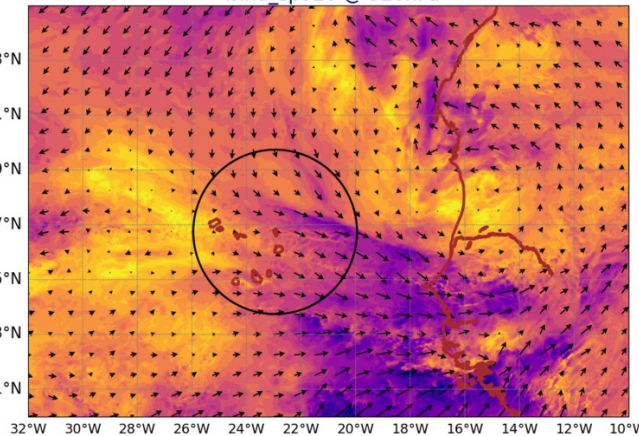
AROME25 20240819-12-UTC -ech(60h) wind_sp920 @ 920hPa
