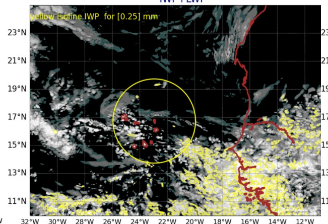
AROME25 20240818-12-UTC -ech(36h) IWP+LWP
