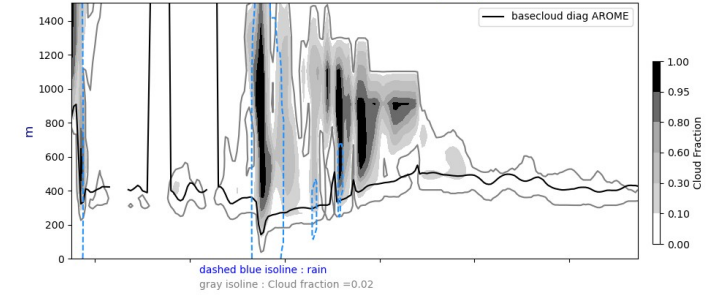
Cross section S/N @ -22W 20240819-12-UTC ech(60h)
