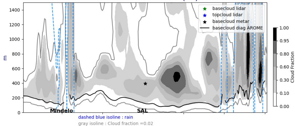
Cross section E/W @ 17.5N 20240817-01-UTC ech(1h)
