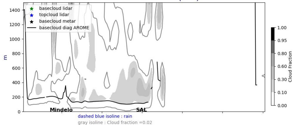
Cross section E/W @ 17.5N 20240817-12-UTC ech(12h)
