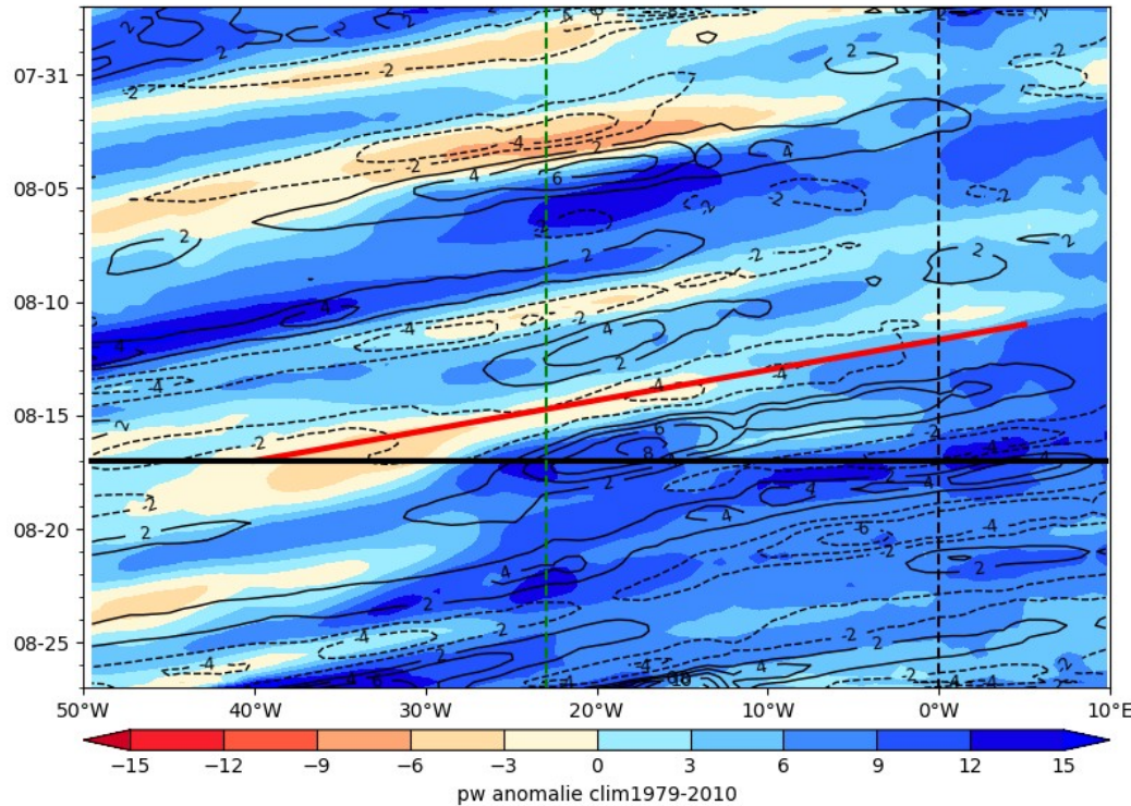
ECMWF PW (color) AND V at 925 hPa 2024-08-17
