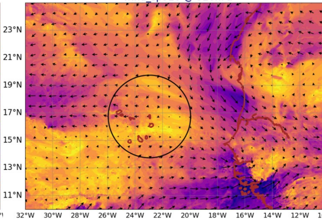
AROME25 20240818-12-UTC -ech(36h) wind_sp920 @ 920hPa
