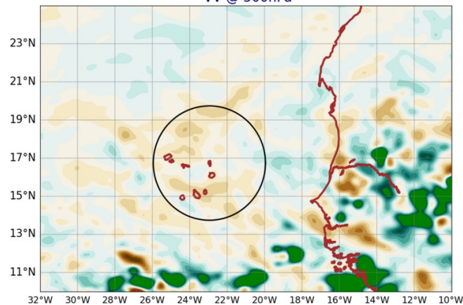
AROME25 20240817-12-UTC -ech(12h) VV @ 500hPa
