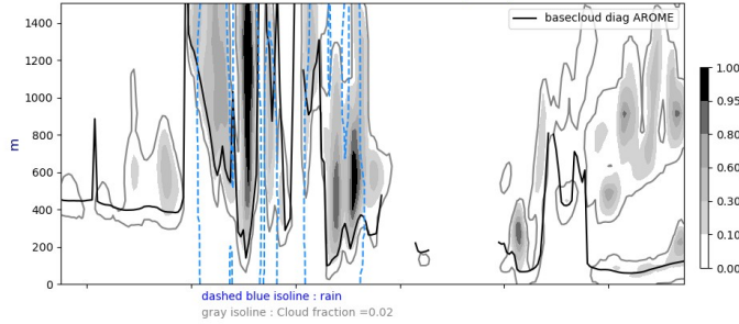
Cross section S/N @ -22W 20240817-12-UTC ech(12h)
