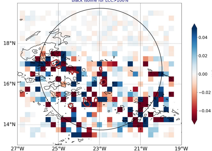
AROME25 regrid 0.25 20240818-12-UTC -ech(36h) blue for conv in subcloud layer black isoline for LCC>100%
