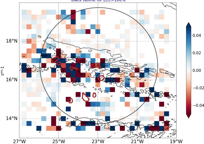
AROME25 regrid 0.25 20240819-12-UTC -ech(60h) blue for conv in subcloud layer black isoline for LCC>100%
