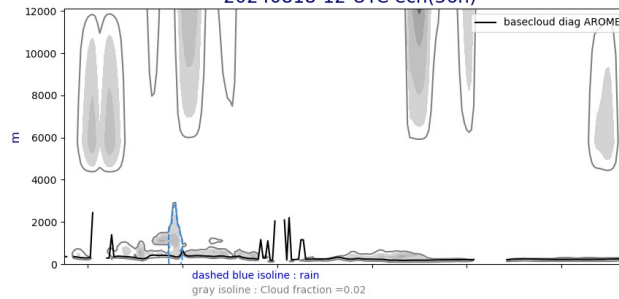
Cross section S/N @ -22W 20240818-12-UTC ech(36h)
