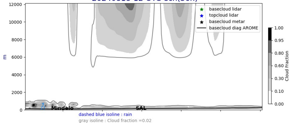
Cross section E/W @ 17.5N 20240818-12-UTC ech(36h)
