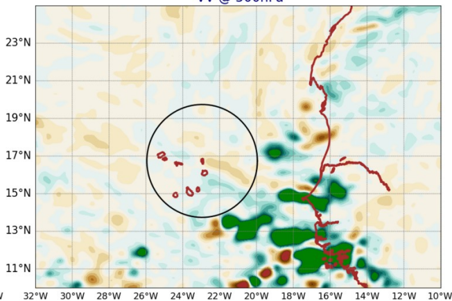
AROME25 20240819-12-UTC -ech(60h) VV @ 500hPa
