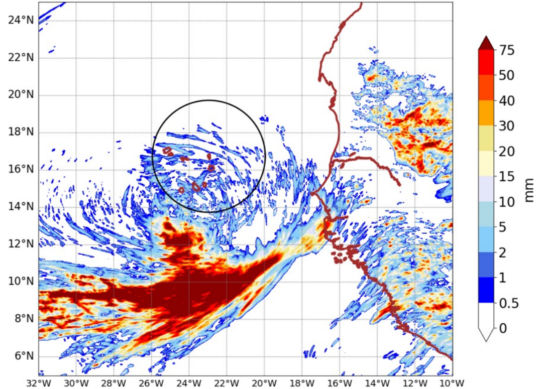
AROME25 20240817-00-UTC -ech(24h)
