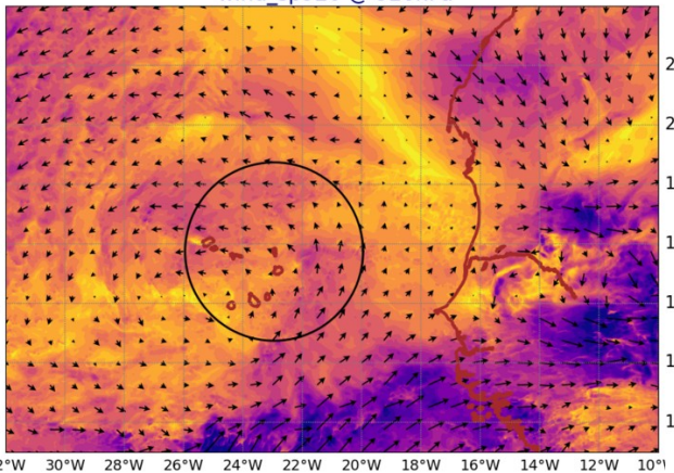
AROME25 20240817-12-UTC -ech(12h) wind_sp920 @ 920hPa
