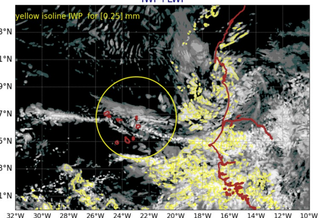
AROME25 20240819-12-UTC -ech(60h) IWP+LWP
