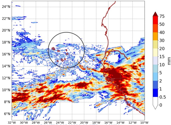
AROME25 20240819-12-UTC -ech(60h) RR cumulated over 24h
