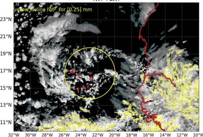
AROME25 20240817-12-UTC -ech(12h) IWP+LWP
