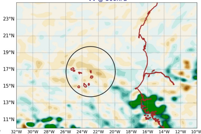
AROME25 20240818-12-UTC -ech(36h) VV @ 500hPa
