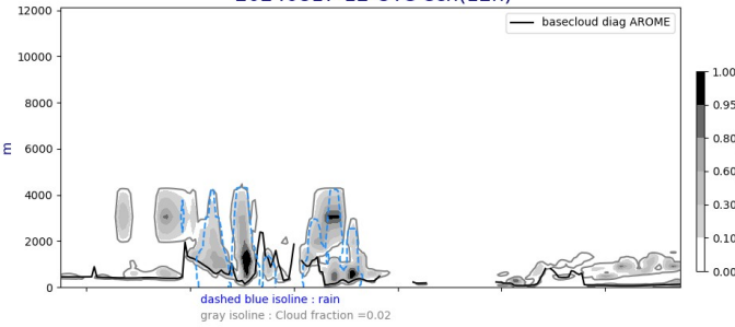
Cross section S/N @ -22W 20240817-12-UTC ech(12h)
