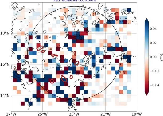
AROME25 regrid 0.25 20240817-12-UTC -ech(12h) blue for conv in subcloud layer black isoline for LCC>100%
