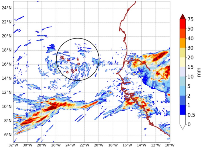
AROME25 20240817-15-UTC -ech(15h) RR cumulated over 6h
