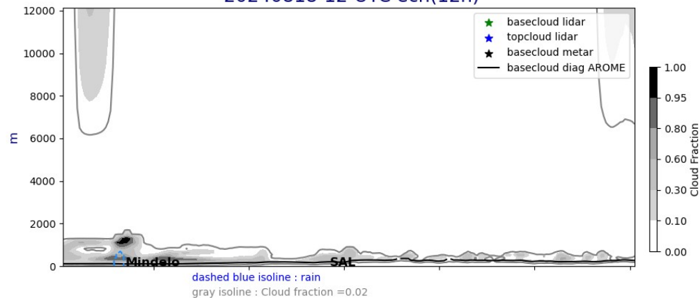
Cross section E/W @ 17.5N 20240818-12-UTC ech(12h)
