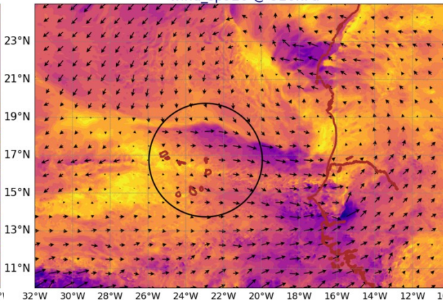
AROME25 20240819-12-UTC -ech(36h) wind_sp920 @ 920hPa
