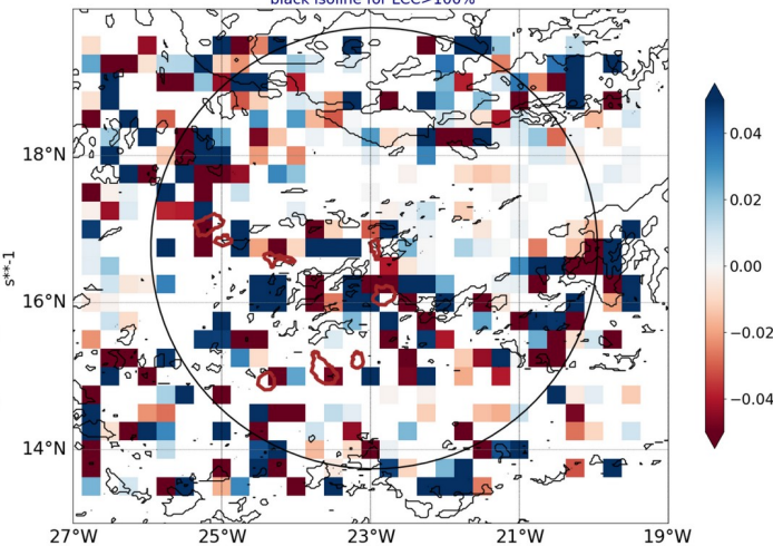
AROME25 regrid 0.25 20240820-12-UTC -ech(60h) blue for conv in subcloud layer black isoline for LCC>100%
