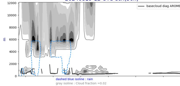
Cross section S/N @ -22W 20240819-12-UTC ech(36h)
