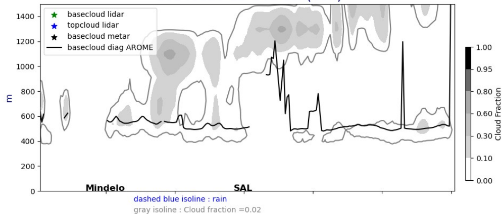
Cross section E/W @ 17.5N 20240820-12-UTC ech(60h)
