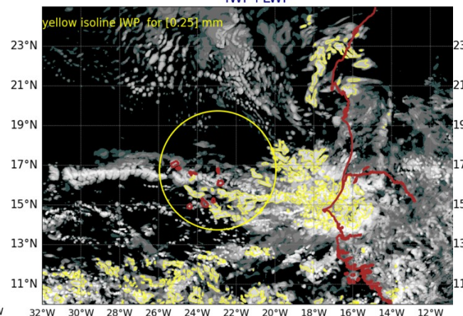
AROME25 20240819-12-UTC -ech(36h) IWP+LWP
