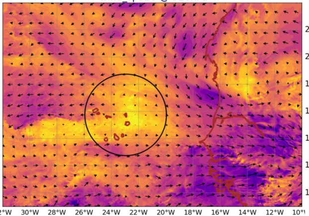
AROME25 20240818-12-UTC -ech(12h) wind_sp920 @ 920hPa
