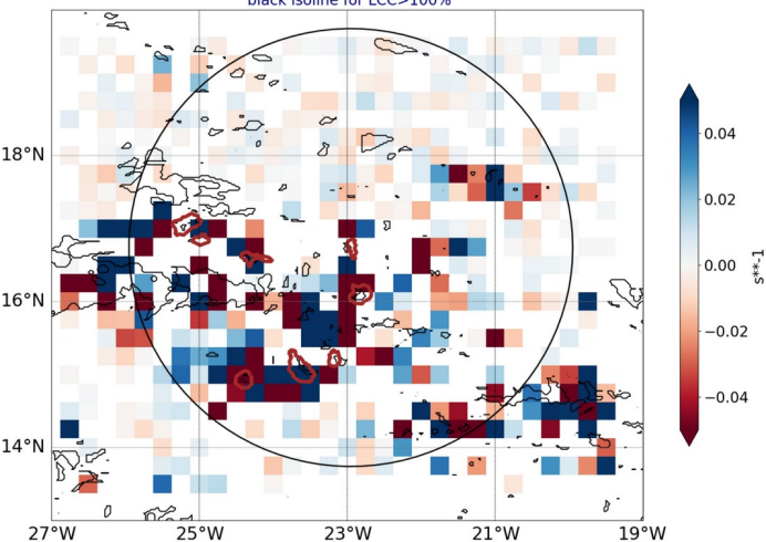
AROME25 regrid 0.25 20240818-12-UTC -ech(12h) blue for conv in subcloud layer black isoline for LCC>100%
