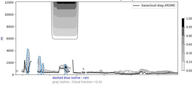
Cross section S/N @ -22W 20240818-12-UTC ech(12h)
