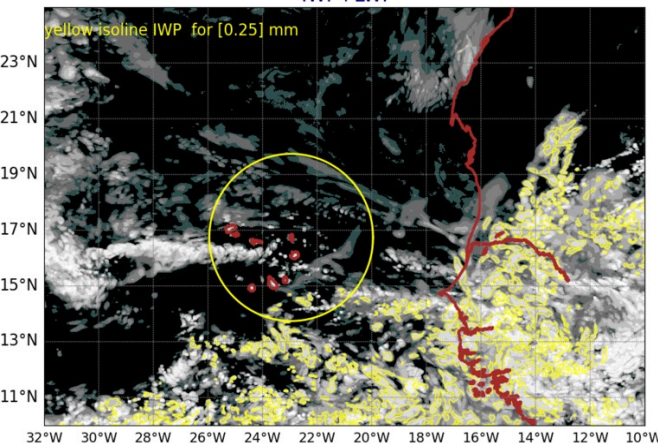
AROME25 20240818-12-UTC -ech(12h) IWP+LWP
