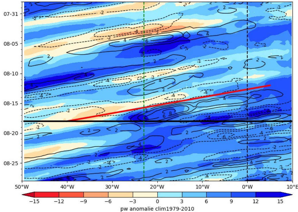
ECMWF PW (color) AND V at 925 hPa 2024-08-18
