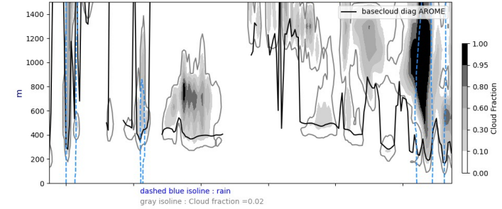
Cross section S/N @ -22W 20240820-12-UTC ech(60h)
