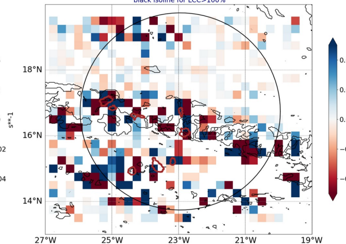
AROME25 regrid 0.25 20240819-12-UTC -ech(36h) blue for conv in subcloud layer black isoline for LCC>100%
