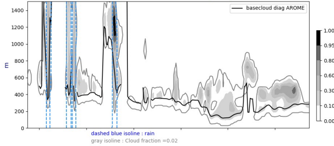
Cross section S/N @ -22W 20240818-12-UTC ech(12h)
