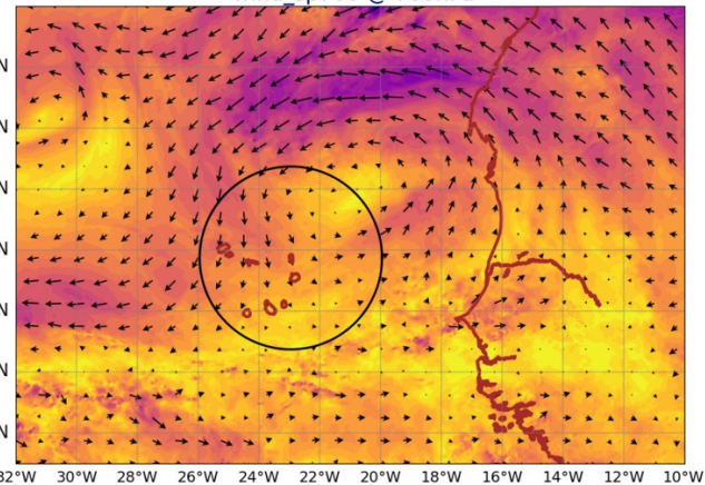
AROME25 20240820-12-UTC -ech(60h) wind_sp920 @ 920hPa
