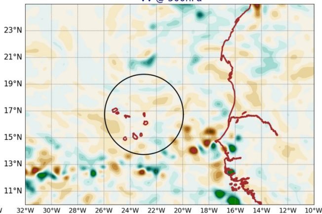
AROME25 20240820-12-UTC -ech(60h) VV @ 500hPa
