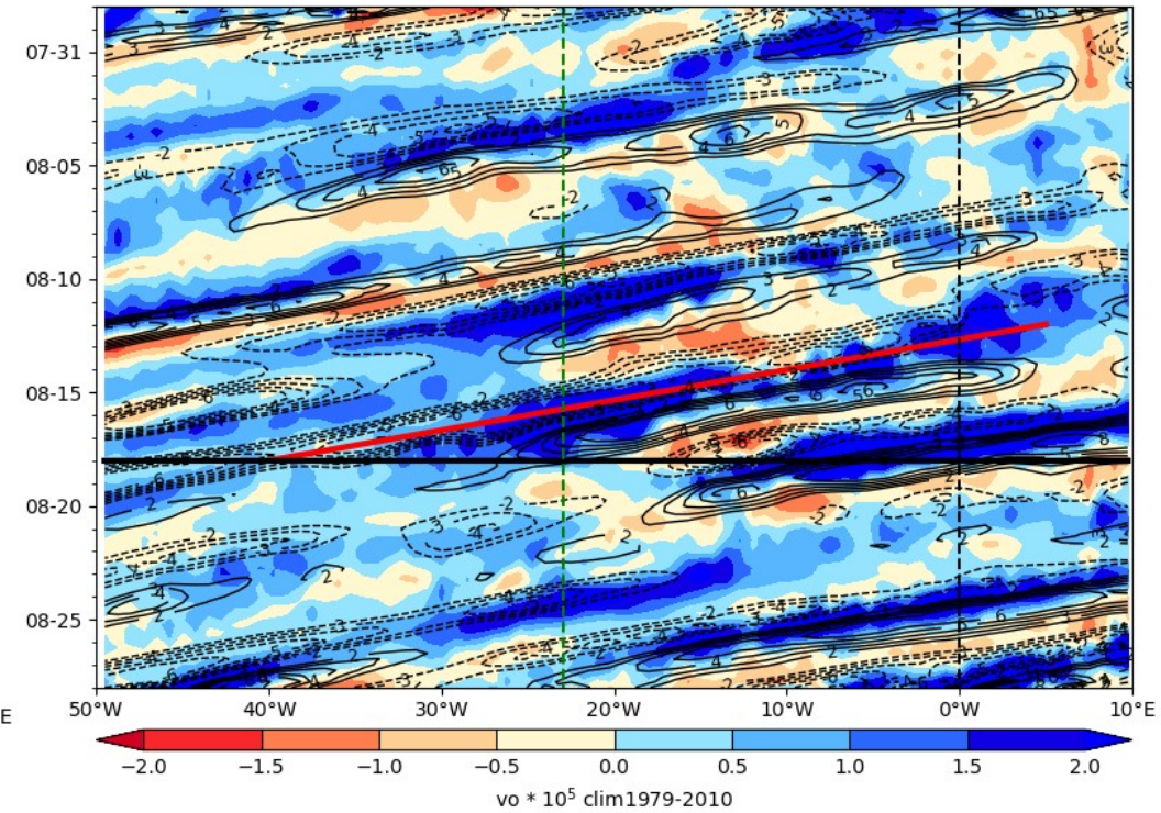
ECMWF Vorticity 850 hPa (color), V-700 hPa 2024-08-18
