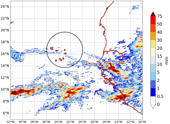
AROME25 20240818-15-UTC -ech(15h) RR cumulated over 6h
