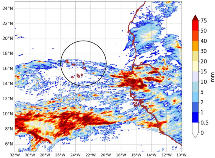
AROME25 20240820-12-UTC -ech(60h) RR cumulated over 24h
