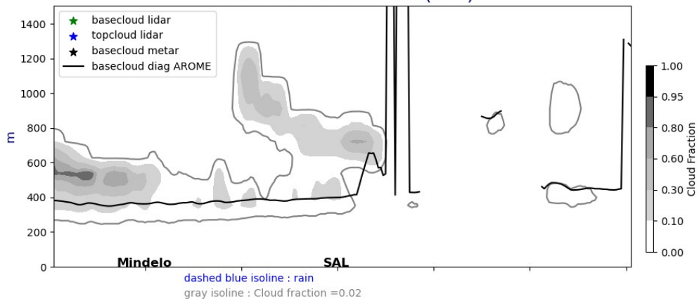
Cross section E/W @ 17.5N 20240819-12-UTC ech(36h)
