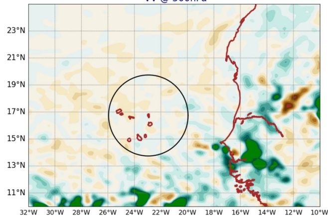
AROME25 20240818-12-UTC -ech(12h) VV @ 500hPa
