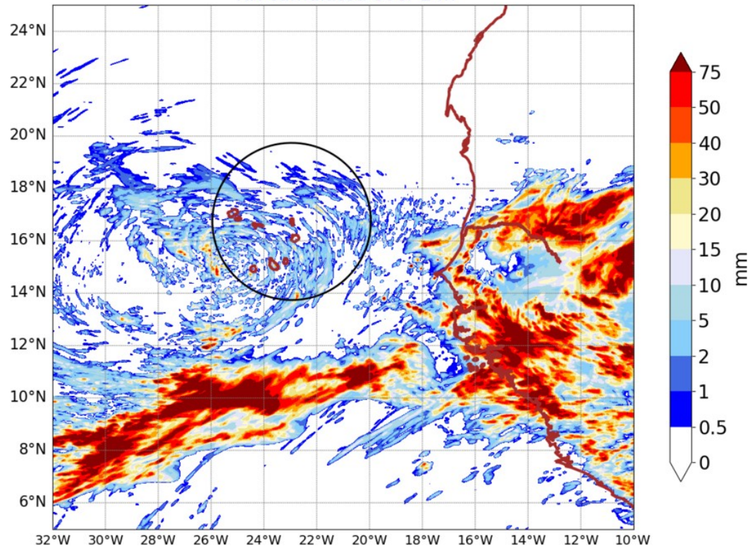
AROME25 20240818-00-UTC -ech(24h) RR cumulated over 24h
