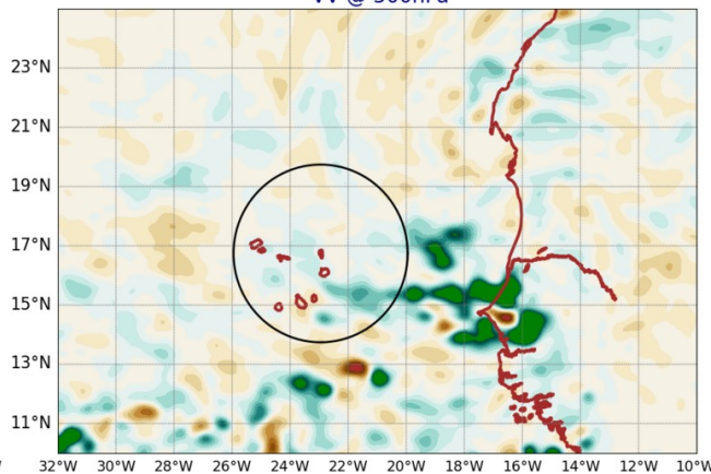
AROME25 20240819-12-UTC -ech(36h) VV @ 500hPa
