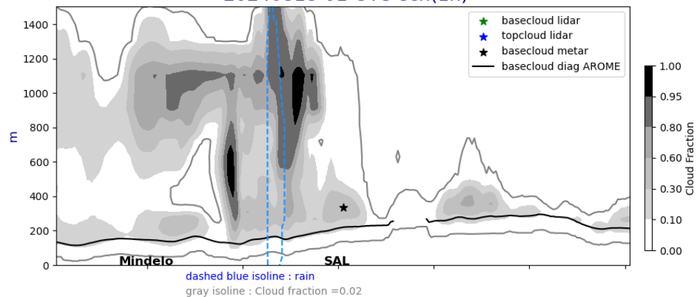
Cross section E/W @ 17.5N 20240818-01-UTC ech(1h)
