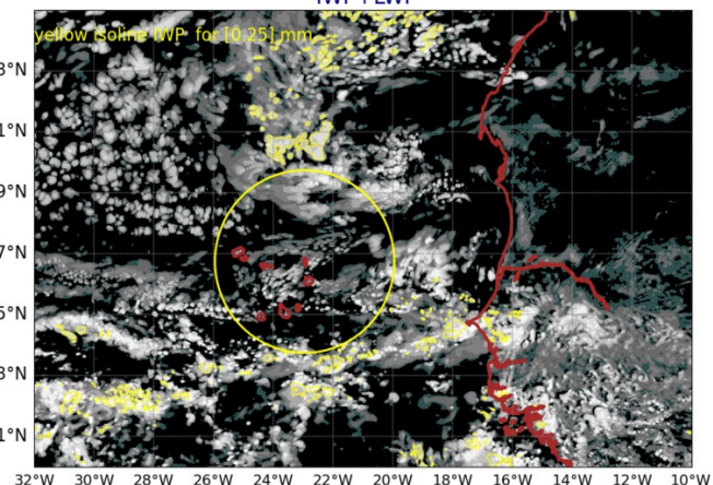
AROME25 20240820-12-UTC -ech(60h) IWP+LWP
