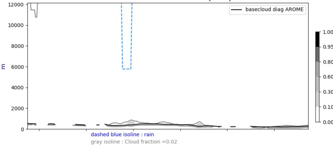
Cross section S/N @ -22W 20240823-12-UTC ech(12h)
