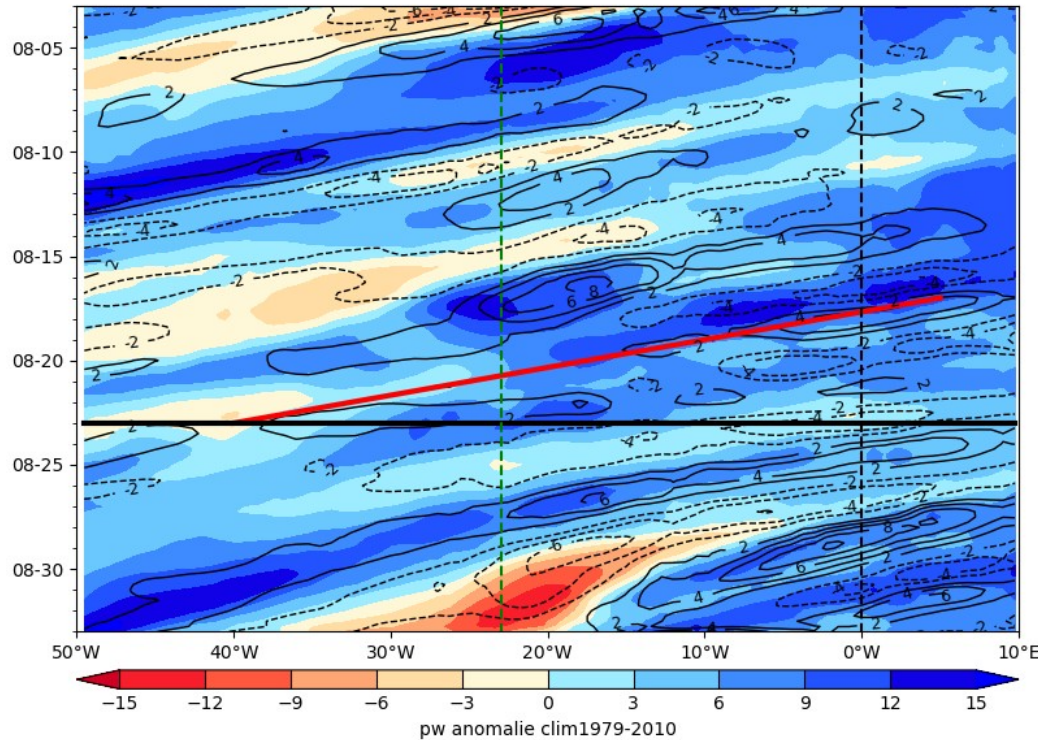
ECMWF PW (color) AND V at 925 hPa 2024-08-23
