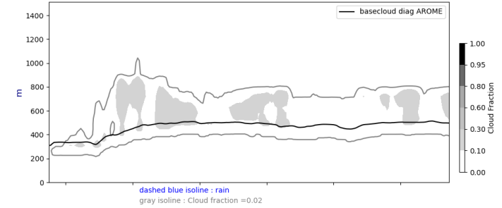
Cross section S/N @ -22W 20240825-12-UTC ech(60h)
