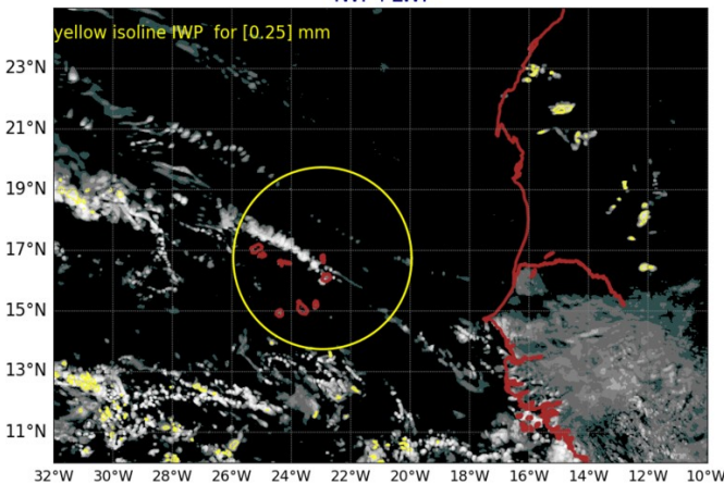
AROME25 20240823-12-UTC -ech(12h) IWP+LWP
