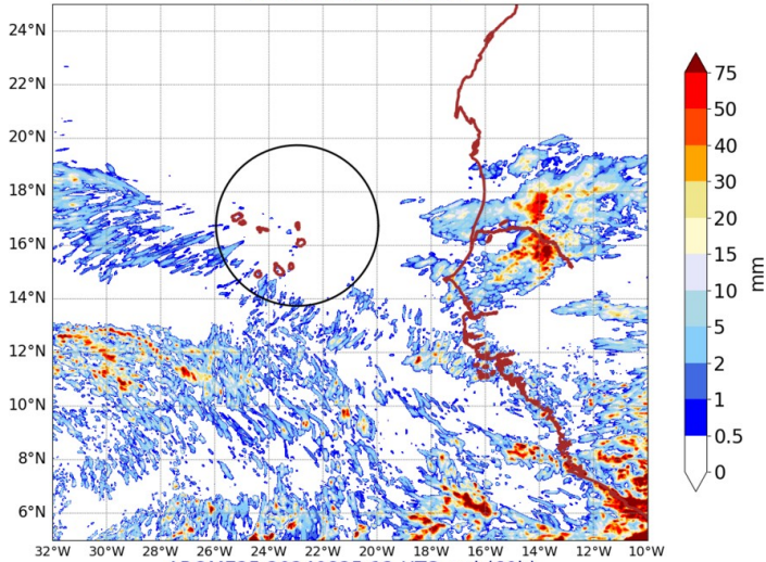
AROME25 20240825-12-UTC -ech(60h) RR cumulated over 24h
