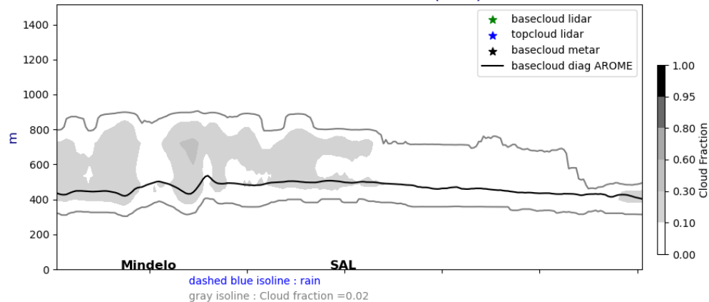
Cross section E/W @ 17.5N 20240825-12-UTC ech(60h)
