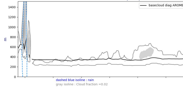
Cross section S/N @ -22W 20240824-12-UTC ech(36h)
