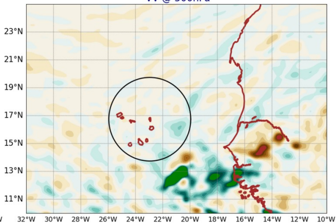
AROME25 20240825-12-UTC -ech(60h) VV @ 500hPa
