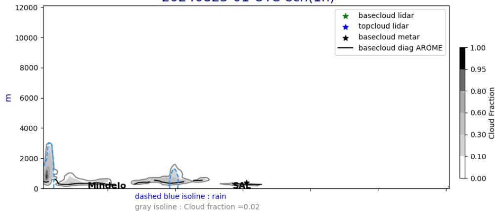
Cross section E/W @ 17.5N 20240823-01-UTC ech(1h)
