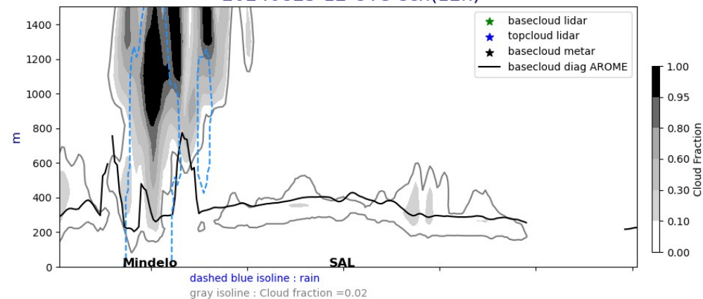
Cross section E/W @ 17.5N 20240823-12-UTC ech(12h)
