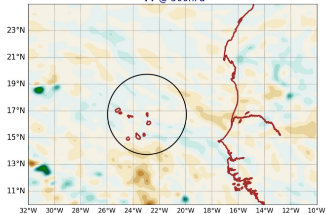
AROME25 20240823-12-UTC -ech(12h) VV @ 500hPa
