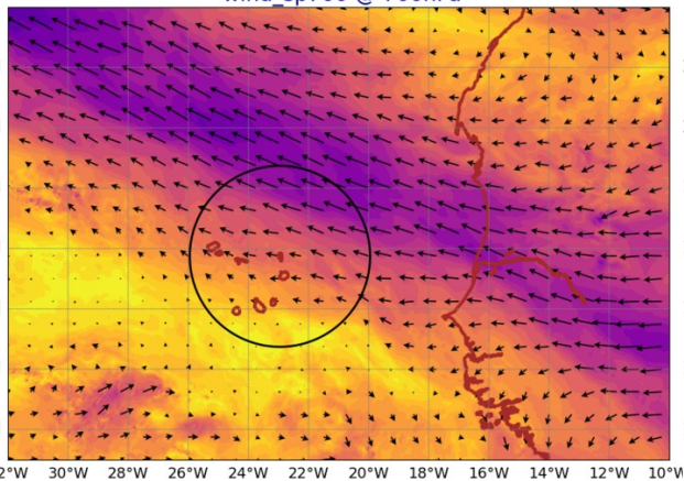
AROME25 20240823-12-UTC -ech(12h) wind_sp920 @ 920hPa
