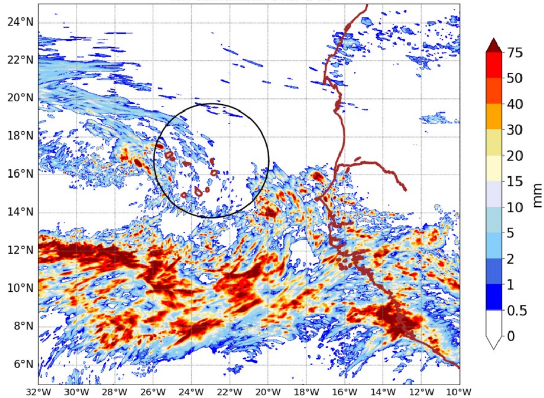
AROME25 20240823-00-UTC -ech(24h) RR cumulated over 24h
