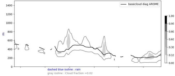
Cross section S/N @ -22W 20240823-12-UTC ech(12h)
