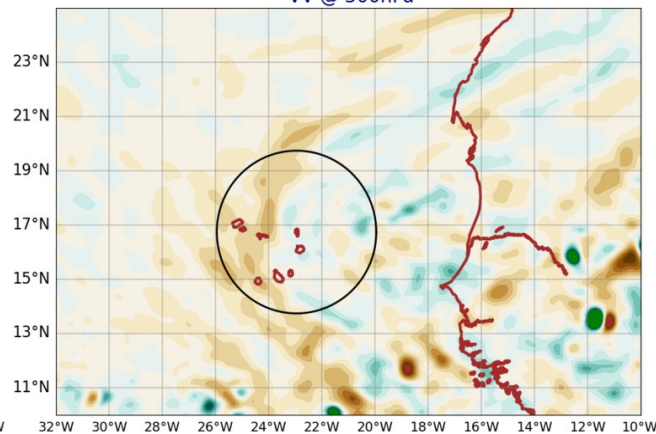
AROME25 20240824-12-UTC -ech(36h) VV @ 500hPa
