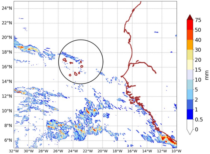
AROME25 20240823-15-UTC -ech(15h) RR cumulated over 6h
