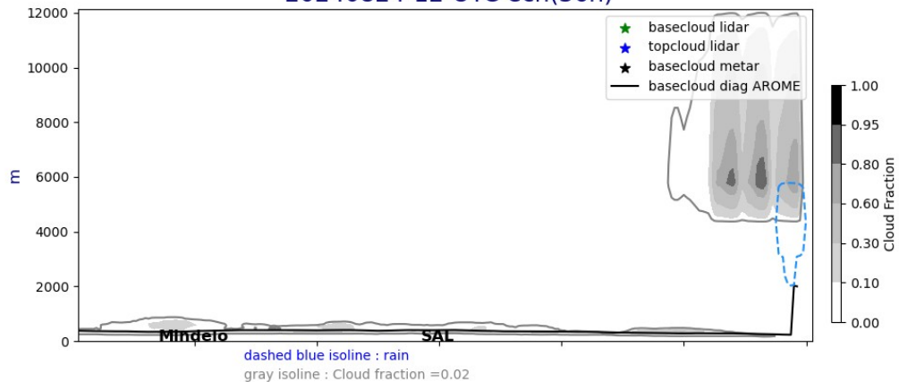
Cross section E/W @ 17.5N 20240824-12-UTC ech(36h)
