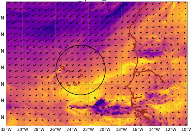
AROME25 20240825-12-UTC -ech(60h) wind_sp920 @ 920hPa
