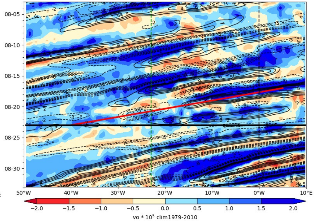
ECMWF Vorticity 850 hPa (color), V-700 hPa 2024-08-23
