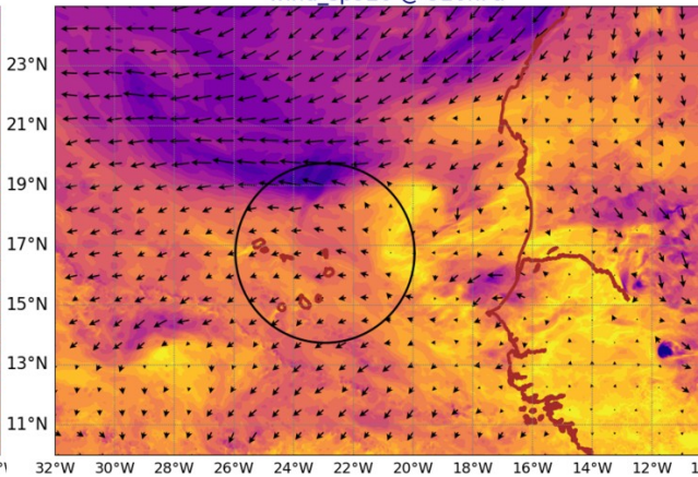
AROME25 20240824-12-UTC -ech(36h) wind_sp920 @ 920hPa
