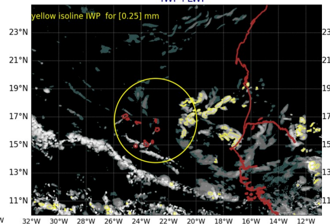
AROME25 20240824-12-UTC -ech(36h) IWP+LWP
