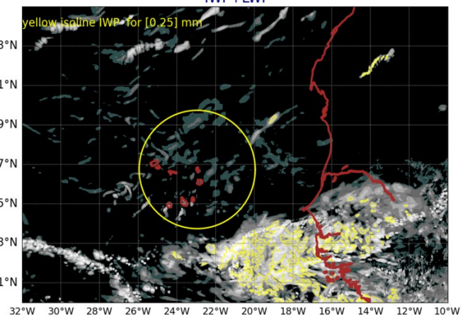
AROME25 20240825-12-UTC -ech(60h) IWP+LWP
