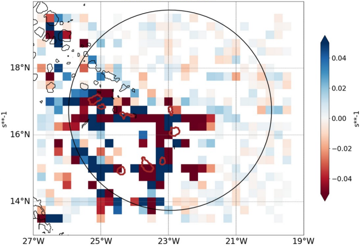
AROME25 regrid 0.25 20240829-12-UTC -ech(60h) blue for conv in subcloud layer black isoline for LCC>100%
