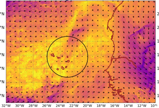
AROME25 20240827-12-UTC -ech(12h) wind_sp920 @ 920hPa
