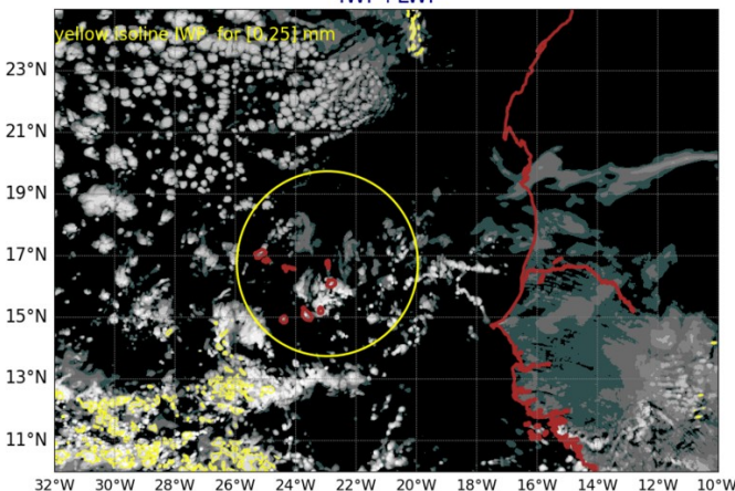
AROME25 20240827-12-UTC -ech(12h) IWP+LWP
