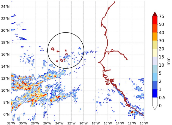
AROME25 20240827-15-UTC -ech(15h) RR cumulated over 6h
