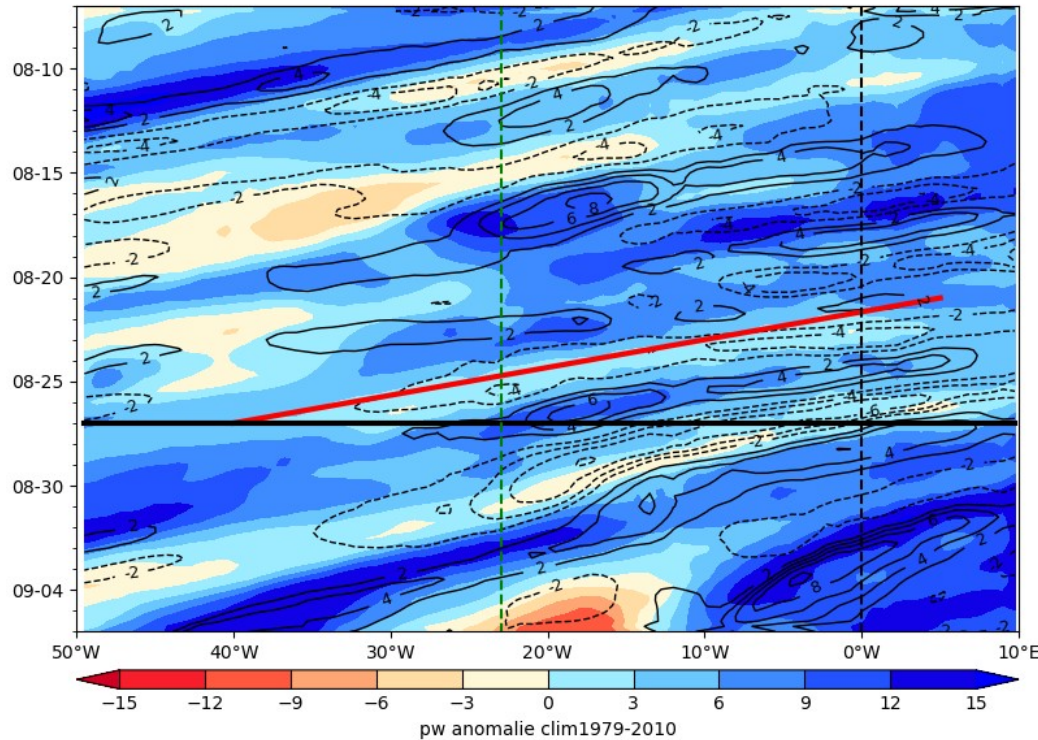
ECMWF PW (color) AND V at 925 hPa 2024-08-27
