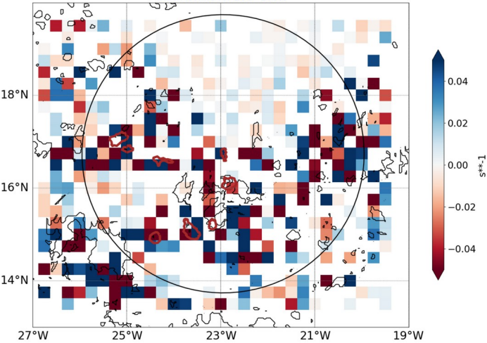
AROME25 regrid 0.25 20240827-12-UTC -ech(12h) blue for conv in subcloud layer black isoline for LCC>100%
