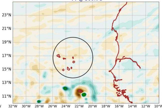
AROME25 20240829-12-UTC -ech(60h) VV @ 500hPa
