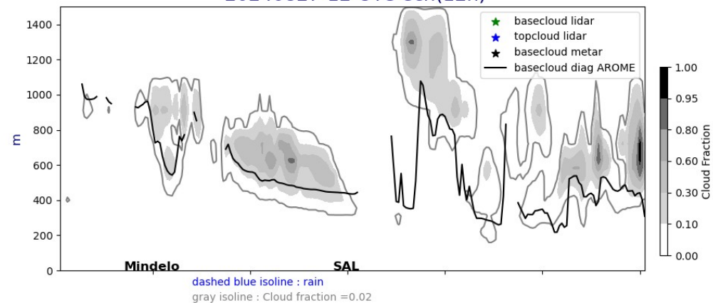
Cross section E/W @ 17.5N 20240827-12-UTC ech(12h)
