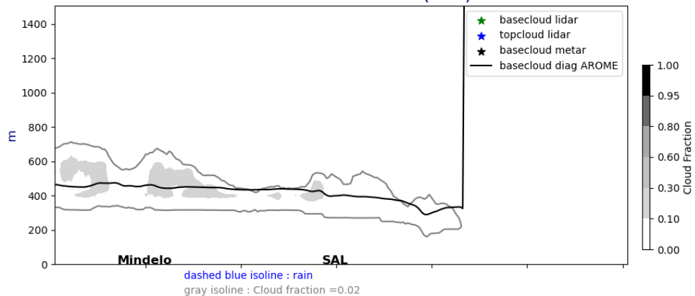
Cross section E/W @ 17.5N 20240828-12-UTC ech(36h)
