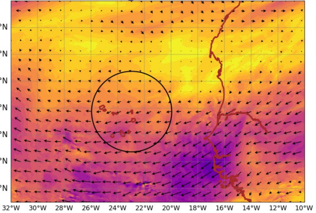
AROME25 20240829-12-UTC -ech(60h) wind_sp920 @ 920hPa
