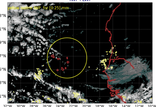
AROME25 20240829-12-UTC -ech(60h) IWP+LWP
