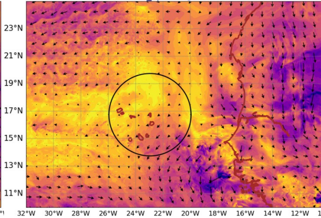
AROME25 20240828-12-UTC -ech(36h) wind_sp920 @ 920hPa
