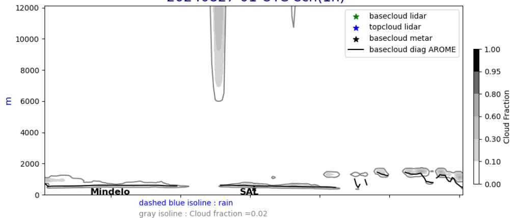
Cross section E/W @ 17.5N 20240827-01-UTC ech(1h)
