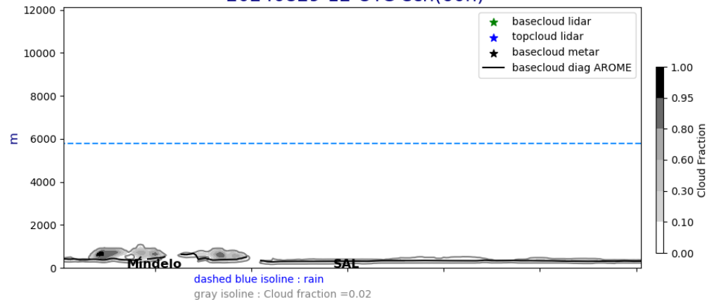
Cross section E/W @ 17.5N 20240829-12-UTC ech(60h)
