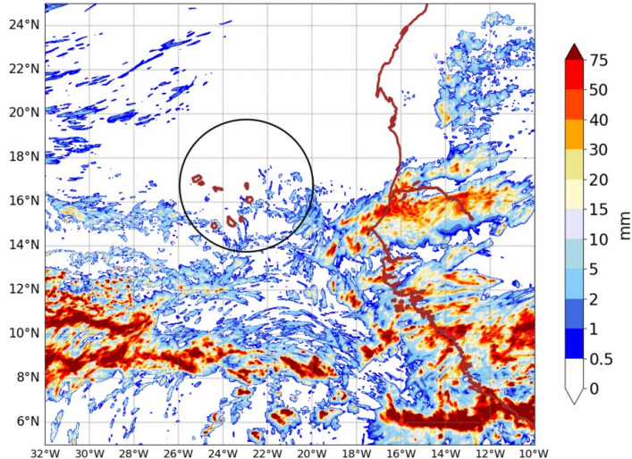
AROME25 20240829-12-UTC -ech(60h) RR cumulated over 24h
