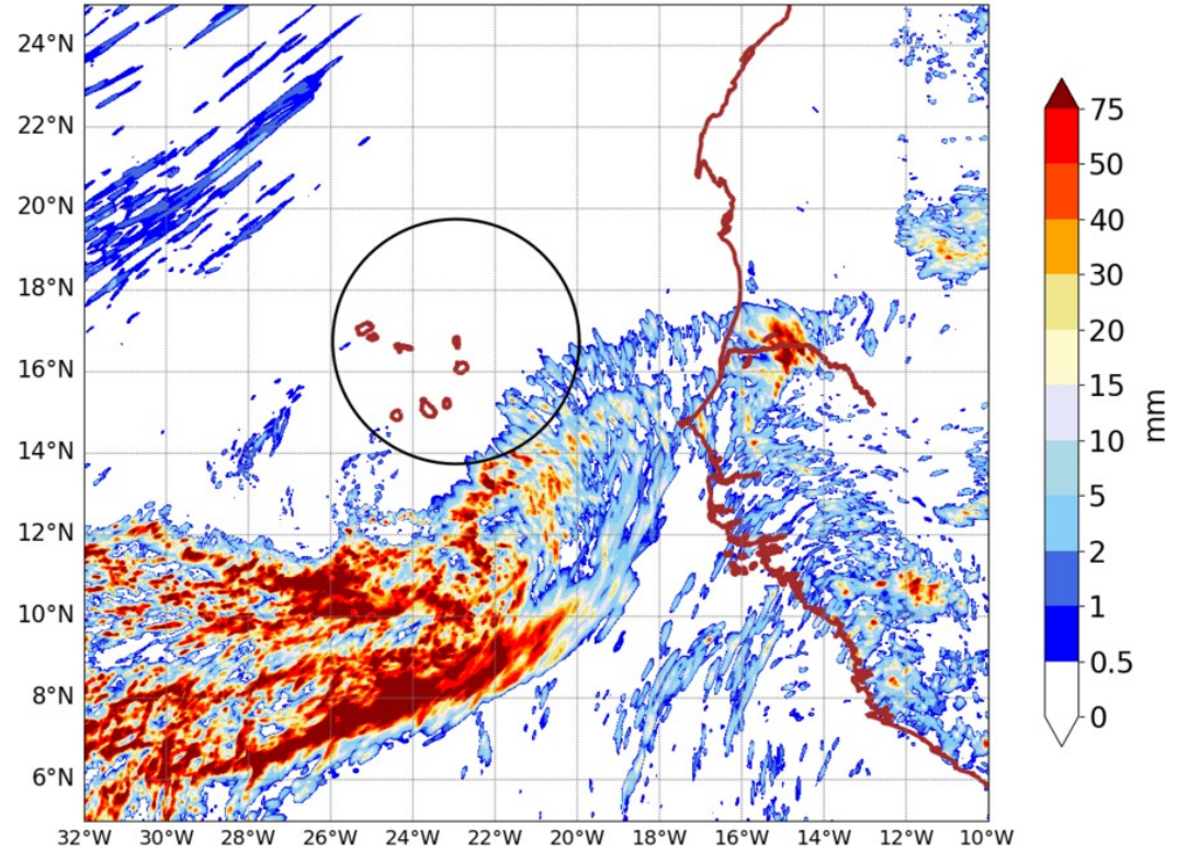
AROME25 20240827-00-UTC -ech(24h)
