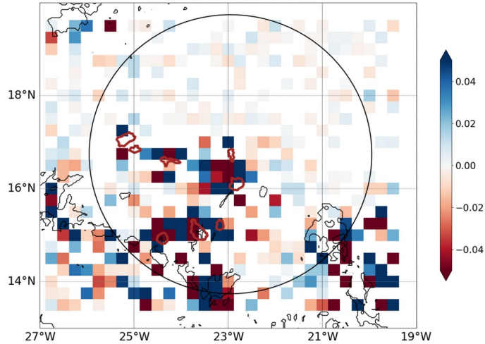
AROME25 regrid 0.25 20240828-12-UTC -ech(36h) blue for conv in subcloud layer black isoline for LCC>100%
