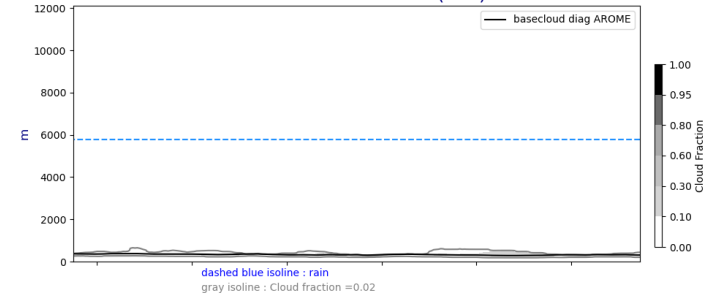
Cross section S/N @ -22W 20240829-12-UTC ech(60h)
