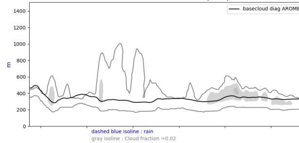
Cross section S/N @ -22W 20240828-12-UTC ech(36h)
