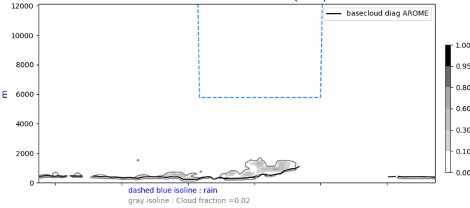
Cross section S/N @ -22W 20240827-12-UTC ech(12h)
