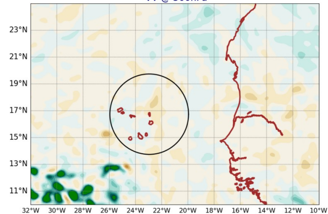
AROME25 20240827-12-UTC -ech(12h) VV @ 500hPa
