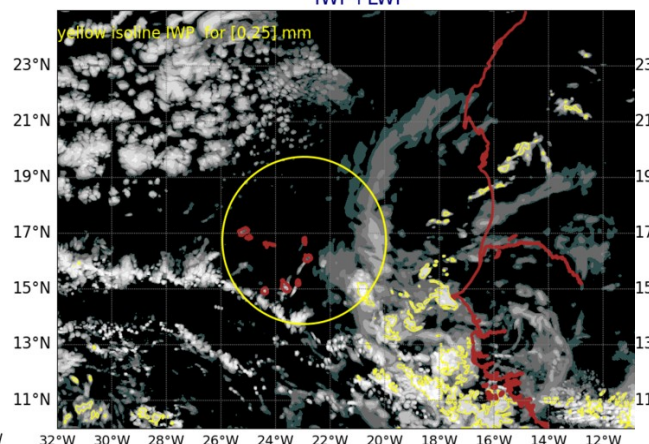
AROME25 20240828-12-UTC -ech(36h) IWP+LWP
