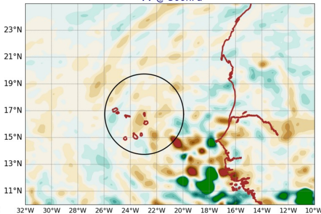
AROME25 20240828-12-UTC -ech(36h) VV @ 500hPa
