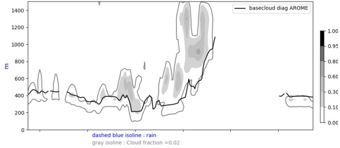
Cross section S/N @ -22W 20240827-12-UTC ech(12h)
