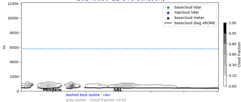
Cross section E/W @ 17.5N 20240830-12-UTC ech(60h)
