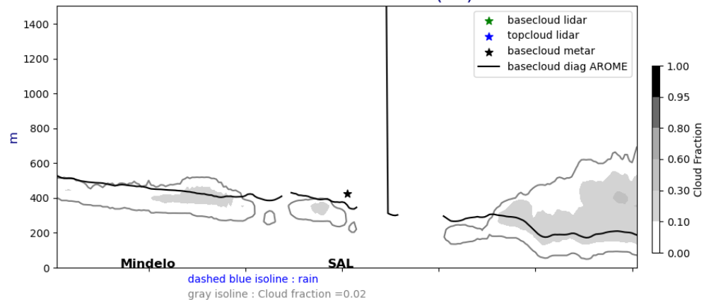
Cross section E/W @ 17.5N 20240828-01-UTC ech(1h)
