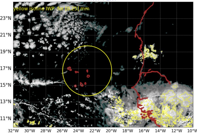
AROME25 20240828-12-UTC -ech(12h) IWP+LWP
