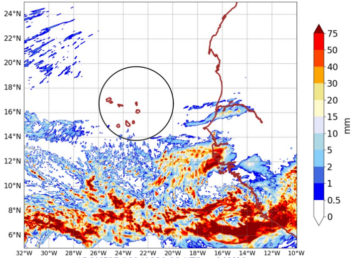
AROME25 20240830-12-UTC -ech(60h) RR cumulated over 24h
