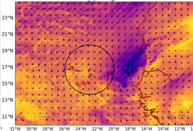
AROME25 20240829-12-UTC -ech(36h) wind_sp920 @ 920hPa
