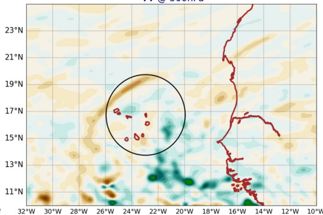
AROME25 20240829-12-UTC -ech(36h) VV @ 500hPa
