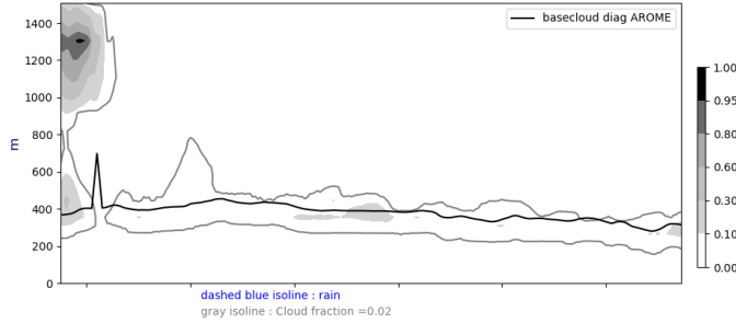
Cross section S/N @ -22W 20240828-12-UTC ech(12h)
