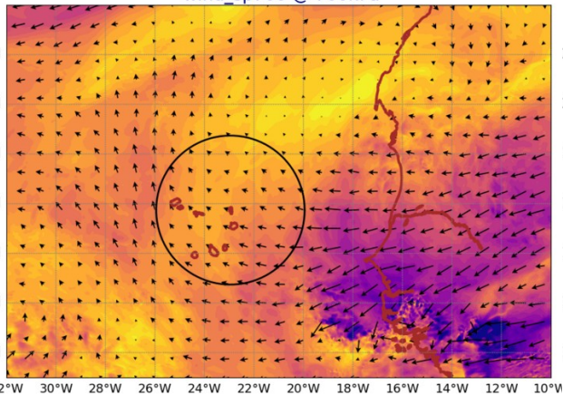
AROME25 20240828-12-UTC -ech(12h) wind_sp920 @ 920hPa
