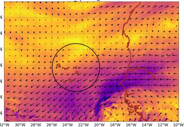
AROME25 20240830-12-UTC -ech(60h) wind_sp920 @ 920hPa
