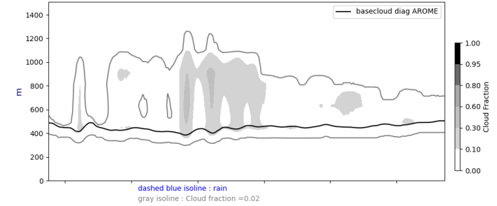
Cross section S/N @ -22W 20240830-12-UTC ech(60h)
