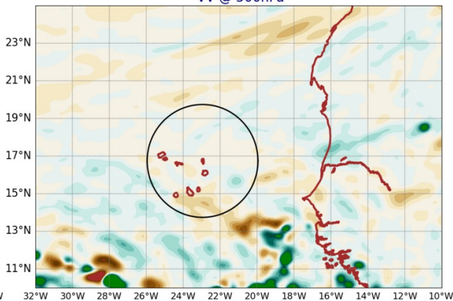
AROME25 20240830-12-UTC -ech(60h) VV @ 500hPa
