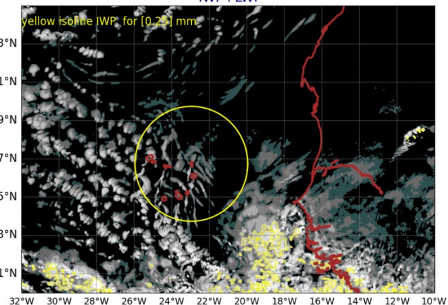
AROME25 20240830-12-UTC -ech(60h) IWP+LWP
