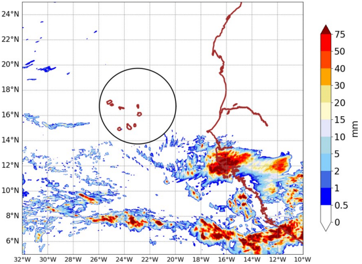
AROME25 20240828-15-UTC -ech(15h) RR cumulated over 6h
