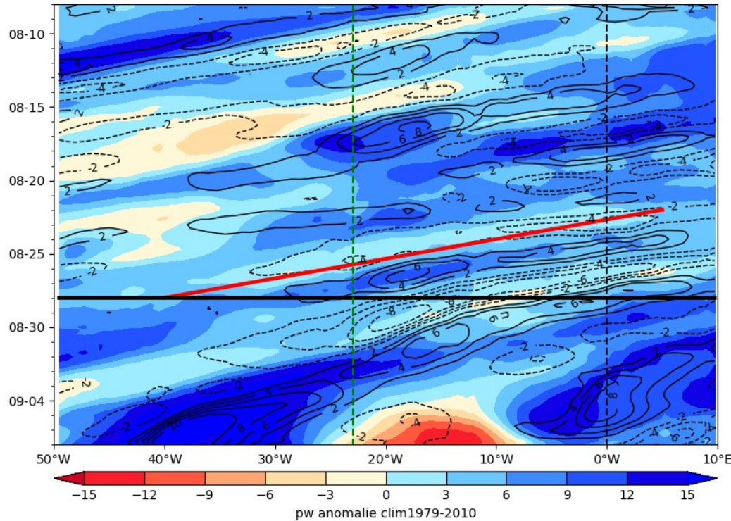
ECMWF PW (color) AND V at 925 hPa 2024-08-28
