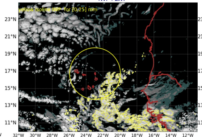
AROME25 20240829-12-UTC -ech(36h) IWP+LWP
