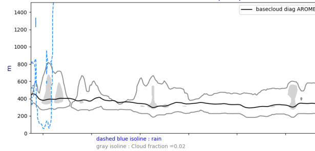
Cross section S/N @ -22W 20240829-12-UTC ech(36h)
