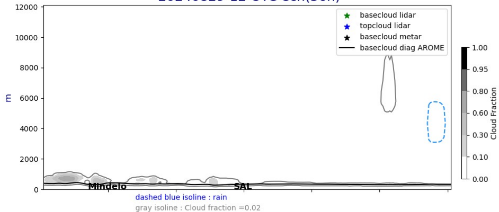
Cross section E/W @ 17.5N 20240829-12-UTC ech(36h)
