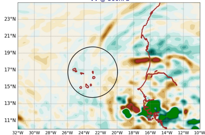
AROME25 20240828-12-UTC -ech(12h) VV @ 500hPa
