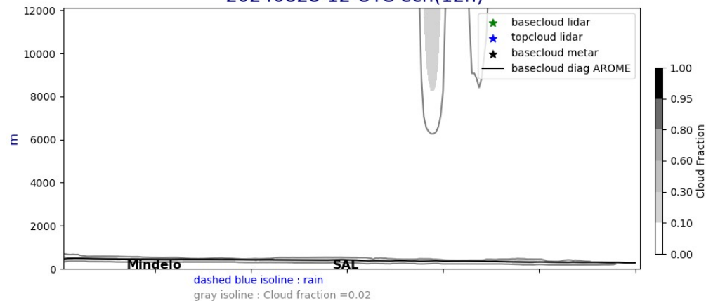
Cross section E/W @ 17.5N 20240828-12-UTC ech(12h)
