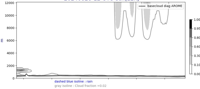
Cross section S/N @ -22W 20240828-12-UTC ech(12h)
