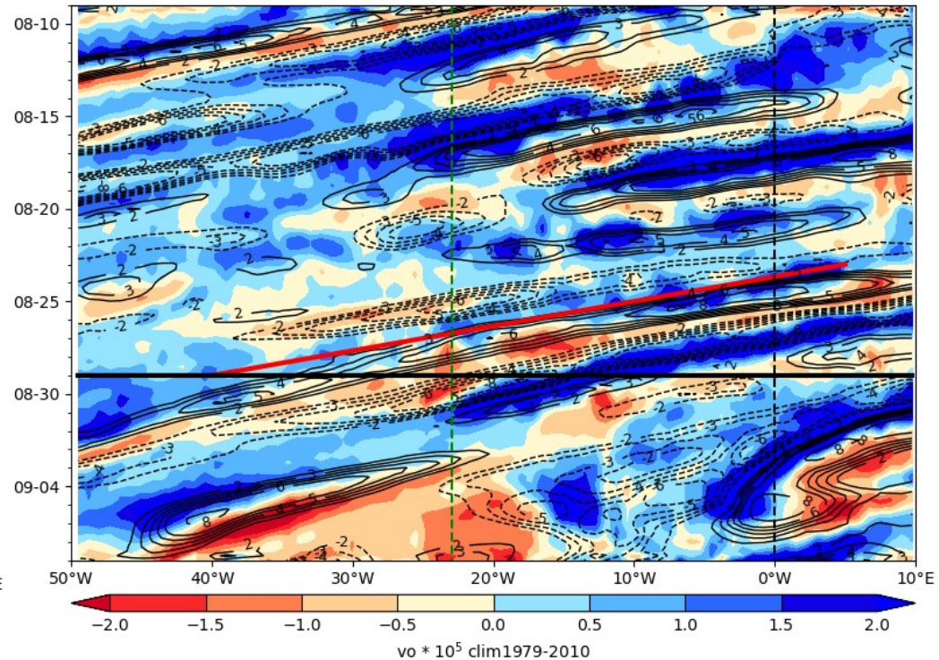
ECMWF Vorticity 850 hPa (color), V-700 hPa 2024-08-29
