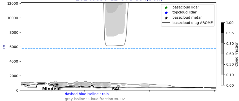
Cross section E/W @ 17.5N 20240830-12-UTC ech(36h)
