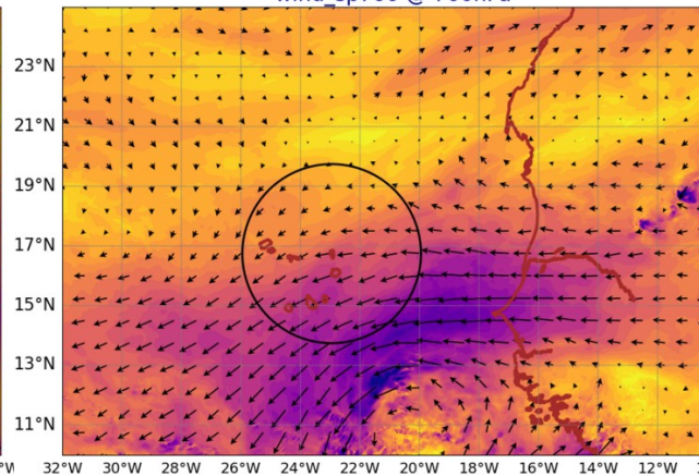
AROME25 20240830-12-UTC -ech(36h) wind_sp920 @ 920hPa
