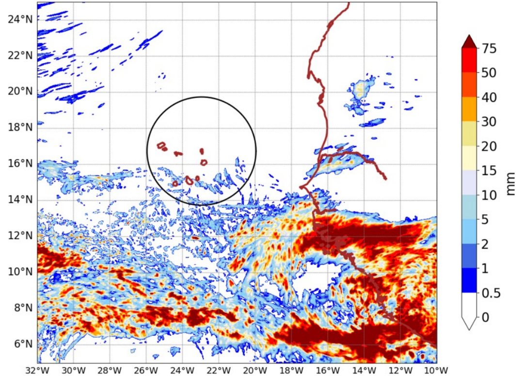
AROME25 20240829-00-UTC -ech(24h)
