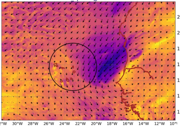
AROME25 20240829-12-UTC -ech(12h) wind_sp920 @ 920hPa
