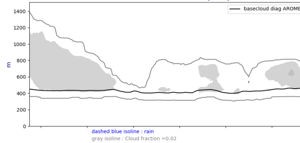
Cross section S/N @ -22W 20240830-12-UTC ech(36h)
