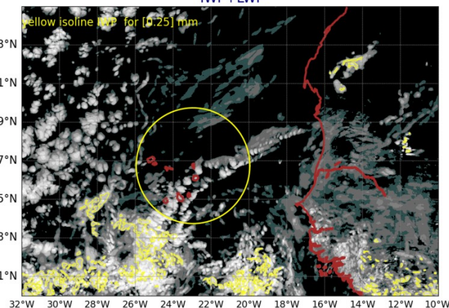
AROME25 20240831-12-UTC -ech(60h) IWP+LWP
