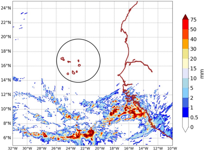
AROME25 20240829-15-UTC -ech(15h) RR cumulated over 6h
