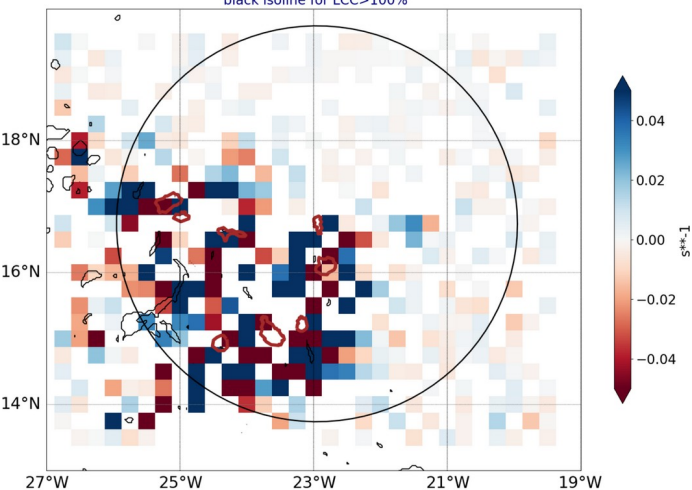
AROME25 regrid 0.25 20240829-12-UTC -ech(12h) blue for conv in subcloud layer black isoline for LCC>100%
