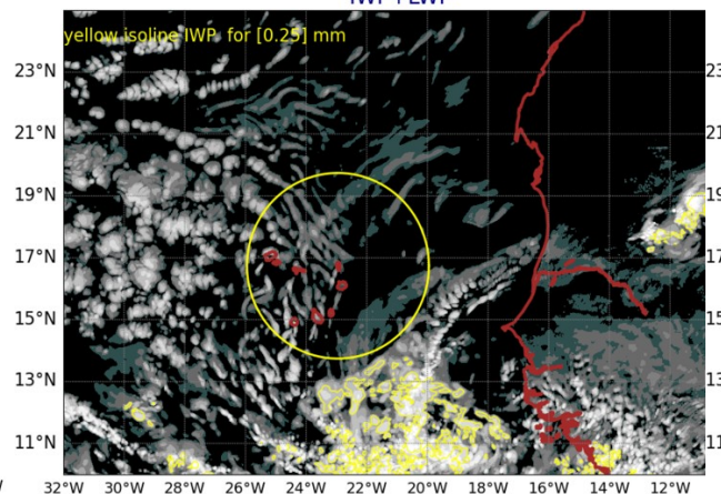
AROME25 20240830-12-UTC -ech(36h) IWP+LWP
