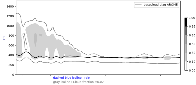
Cross section S/N @ -22W 20240829-12-UTC ech(12h)
