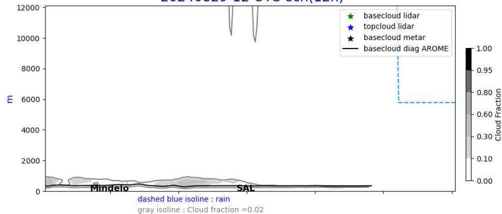
Cross section E/W @ 17.5N 20240829-12-UTC ech(12h)
