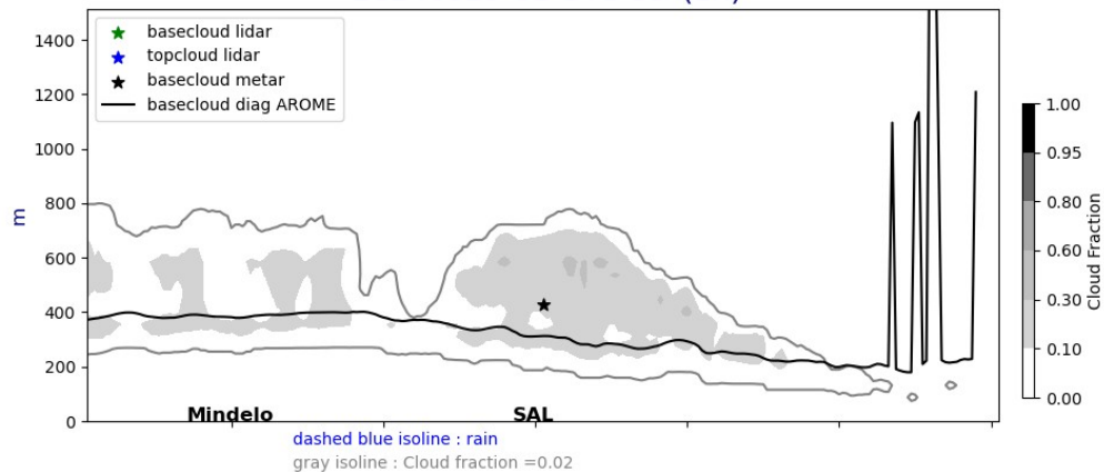
Cross section E/W @ 17.5N 20240829-01-UTC ech(1h)
