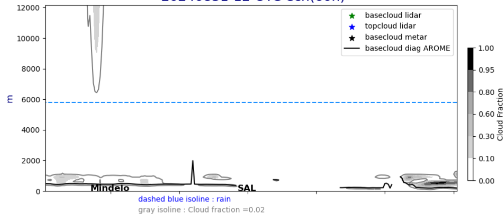
Cross section E/W @ 17.5N 20240831-12-UTC ech(60h)
