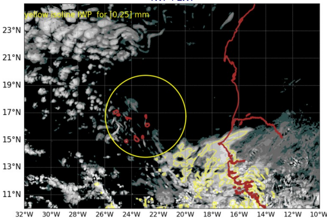
AROME25 20240829-12-UTC -ech(12h) IWP+LWP
