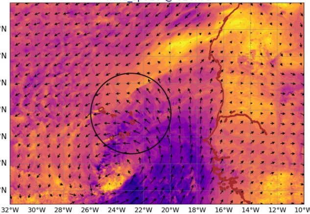
AROME25 20240831-12-UTC -ech(60h) wind_sp920 @ 920hPa
