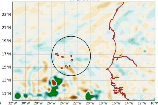
AROME25 20240831-12-UTC -ech(60h) VV @ 500hPa
