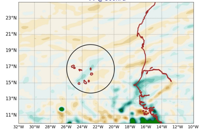
AROME25 20240829-12-UTC -ech(12h) VV @ 500hPa
