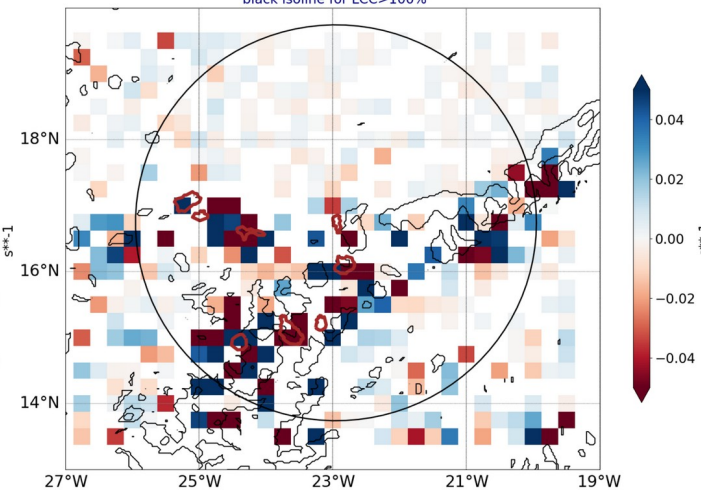
AROME25 regrid 0.25 20240831-12-UTC -ech(60h) blue for conv in subcloud layer black isoline for LCC>100%
