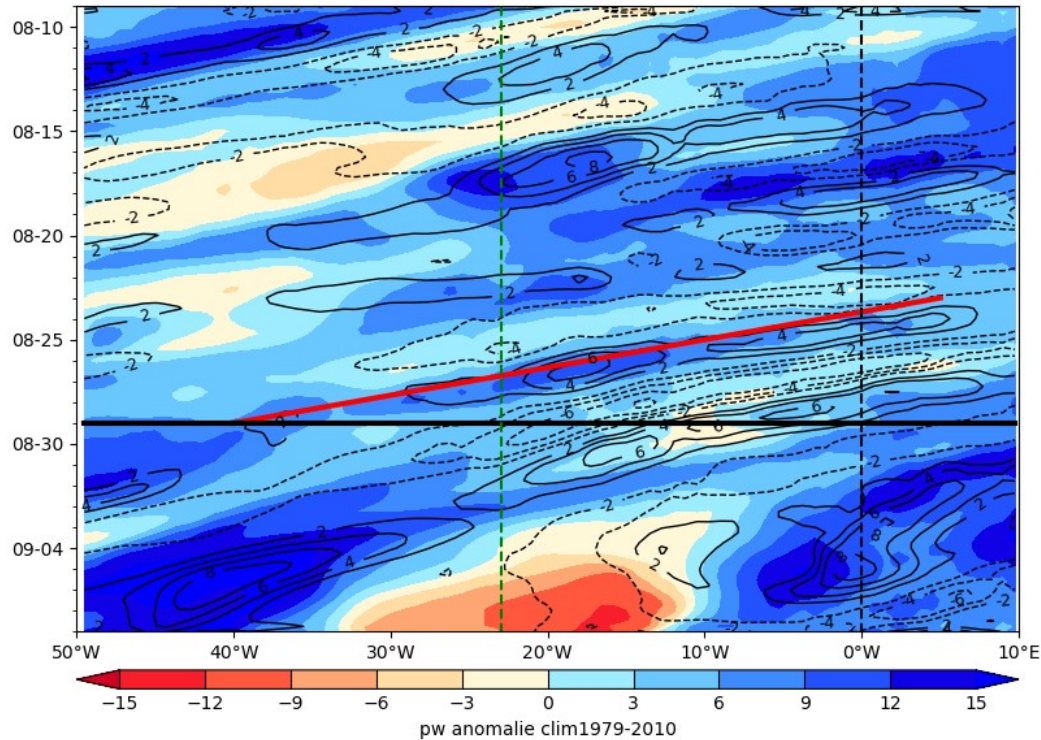
ECMWF PW (color) AND V at 925 hPa 2024-08-29
