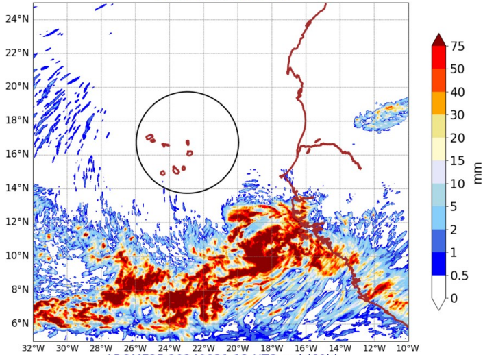
AROME25 20240831-12-UTC -ech(60h) RR cumulated over 24h
