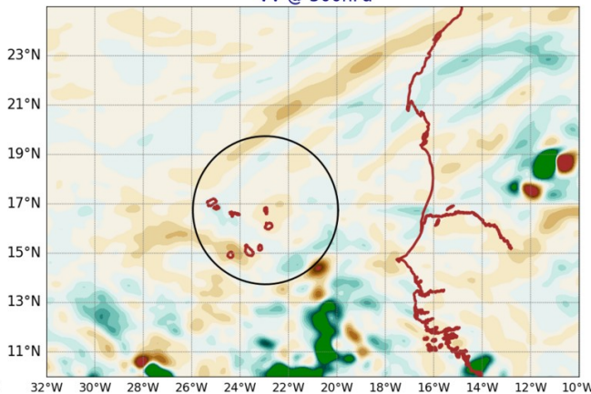
AROME25 20240830-12-UTC -ech(36h) VV @ 500hPa
