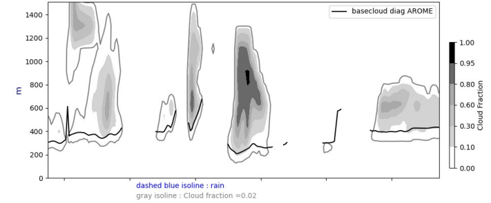
Cross section S/N @ -22W 20240831-12-UTC ech(60h)
