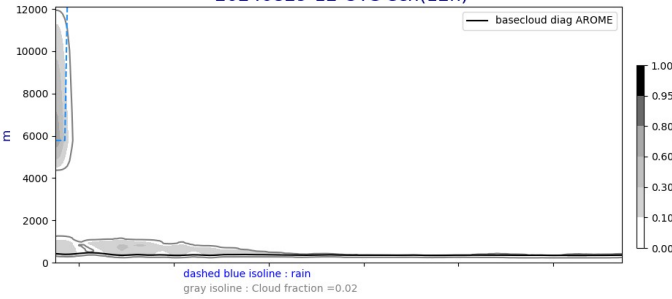
Cross section S/N @ -22W 20240829-12-UTC ech(12h)
