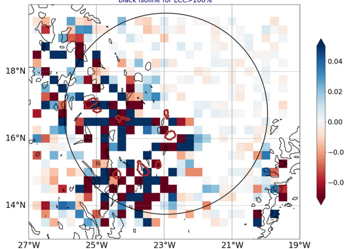
AROME25 regrid 0.25 20240830-12-UTC -ech(36h) blue for conv in subcloud layer black isoline for LCC>100%
