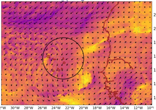
AROME25 20240830-12-UTC -ech(12h) wind_sp920 @ 920hPa
