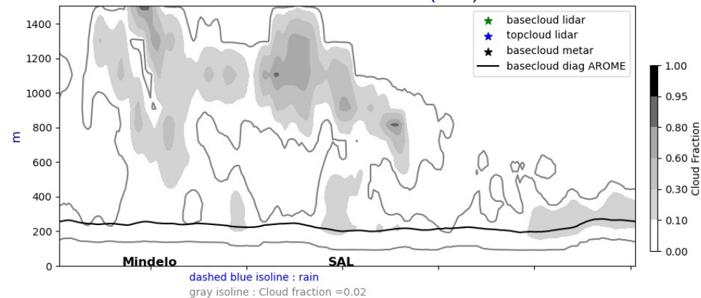
Cross section E/W @ 17.5N 20240901-12-UTC ech(60h)
