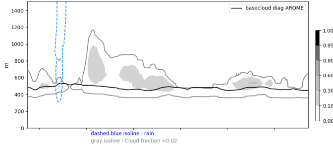
Cross section S/N @ -22W 20240830-12-UTC ech(12h)
