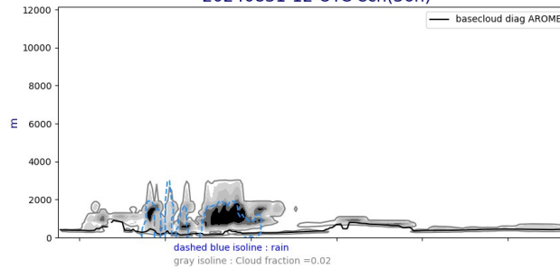
Cross section S/N @ -22W 20240831-12-UTC ech(36h)
