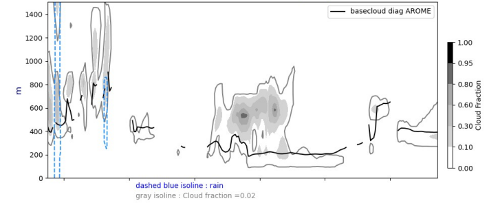
Cross section S/N @ -22W 20240901-12-UTC ech(60h)
