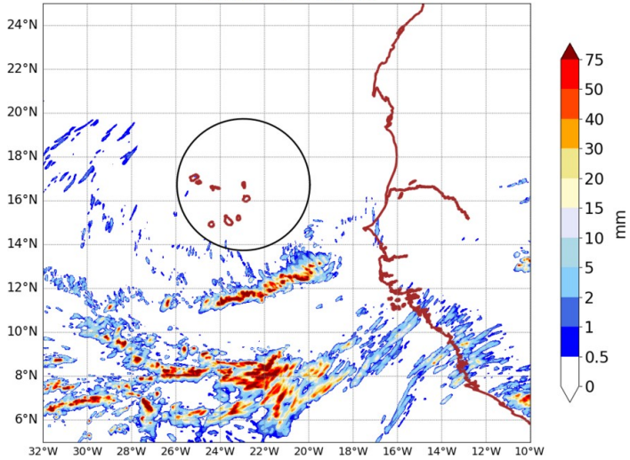
AROME25 20240830-15-UTC -ech(15h) RR cumulated over 6h
