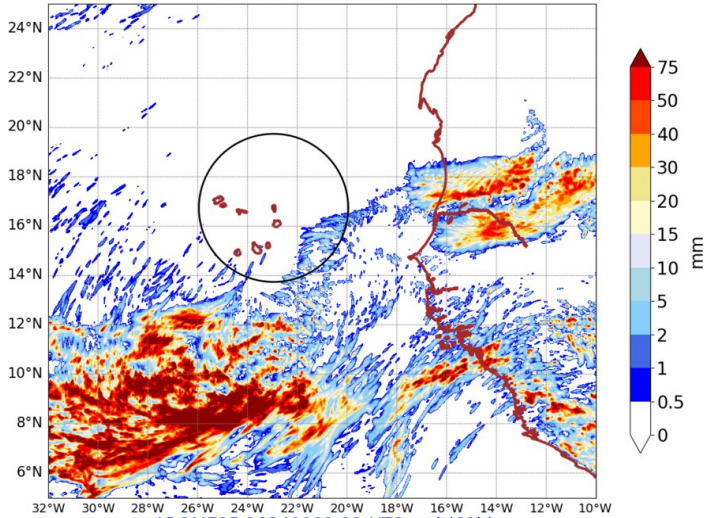
AROME25 20240901-12-UTC -ech(60h) RR cumulated over 24h
