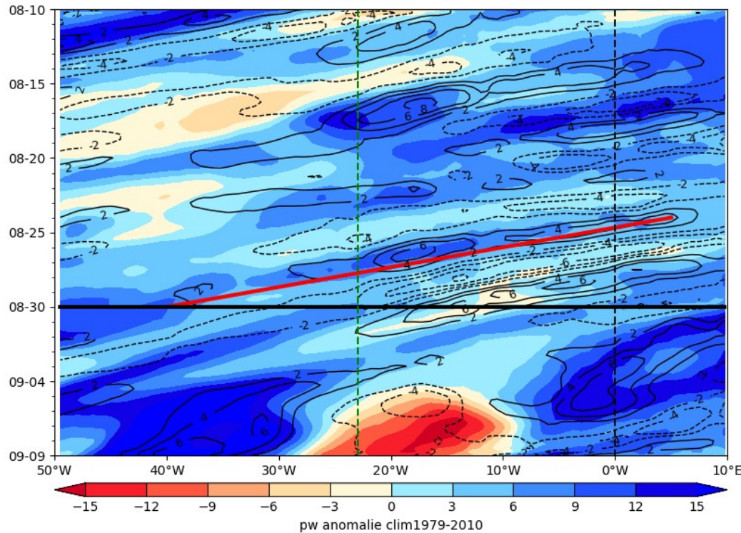
ECMWF PW (color) AND V at 925 hPa 2024-08-30
