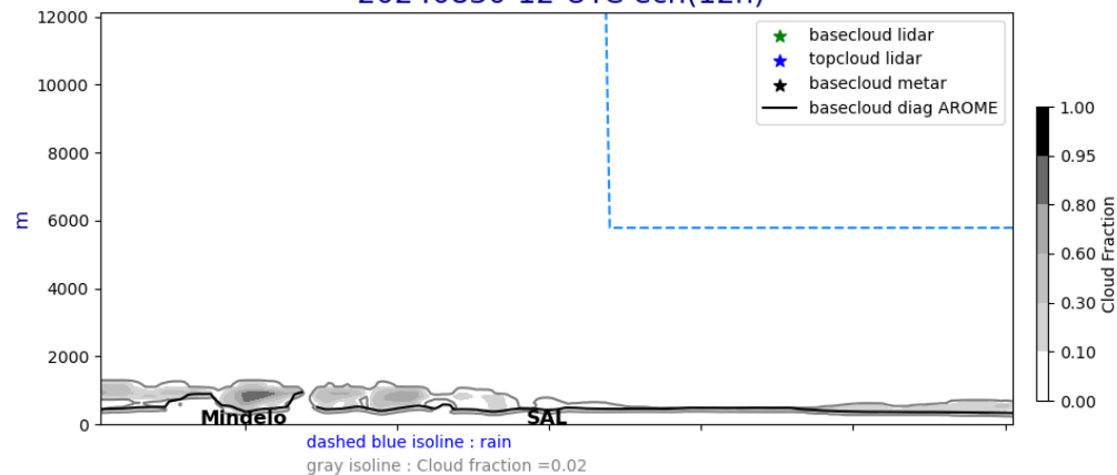
Cross section E/W @ 17.5N 20240830-12-UTC ech(12h)
