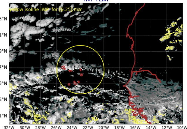
AROME25 20240901-12-UTC -ech(60h) IWP+LWP
