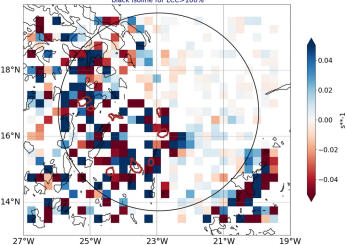
AROME25 regrid 0.25 20240830-12-UTC -ech(12h) blue for conv in subcloud layer black isoline for LCC>100%
