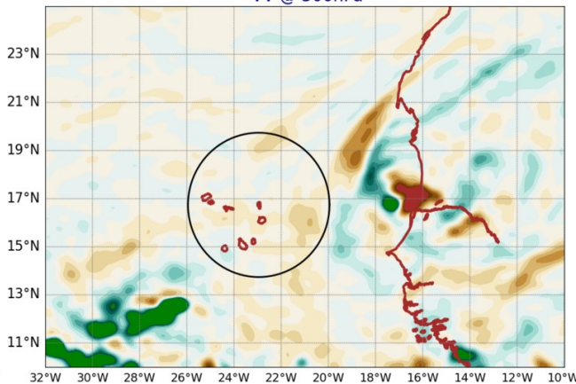
AROME25 20240831-12-UTC -ech(36h) VV @ 500hPa
