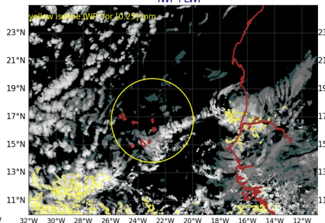
AROME25 20240831-12-UTC -ech(36h) IWP+LWP
