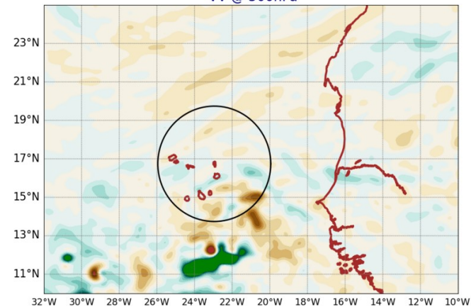
AROME25 20240830-12-UTC -ech(12h) VV @ 500hPa
