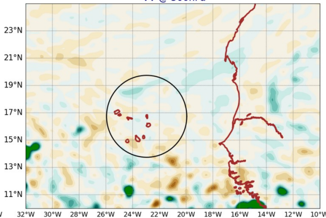
AROME25 20240901-12-UTC -ech(60h) VV @ 500hPa
