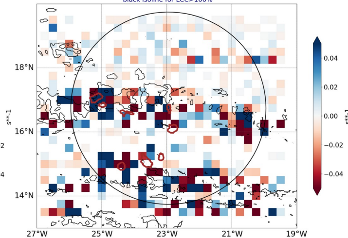
AROME25 regrid 0.25 20240901-12-UTC -ech(60h) blue for conv in subcloud layer black isoline for LCC>100%
