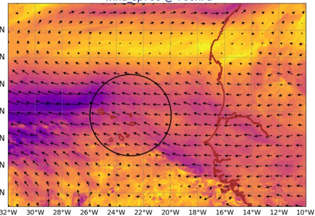
AROME25 20240901-12-UTC -ech(60h) wind_sp920 @ 920hPa
