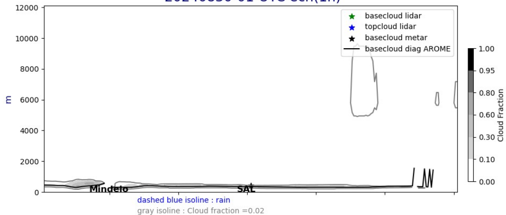
Cross section E/W @ 17.5N 20240830-01-UTC ech(1h)
