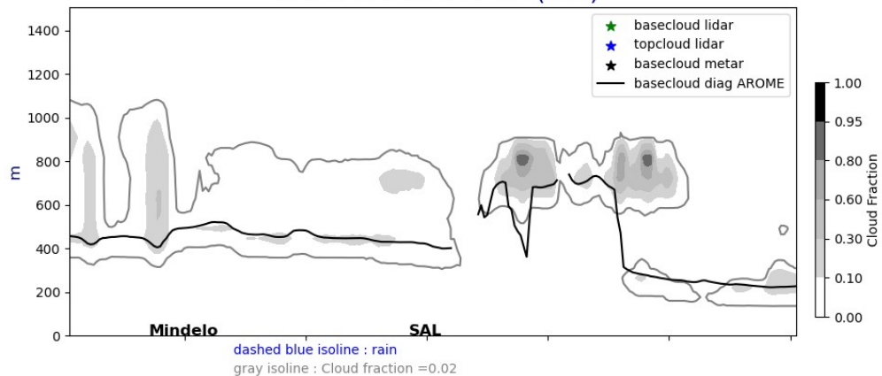
Cross section E/W @ 17.5N 20240831-12-UTC ech(36h)
