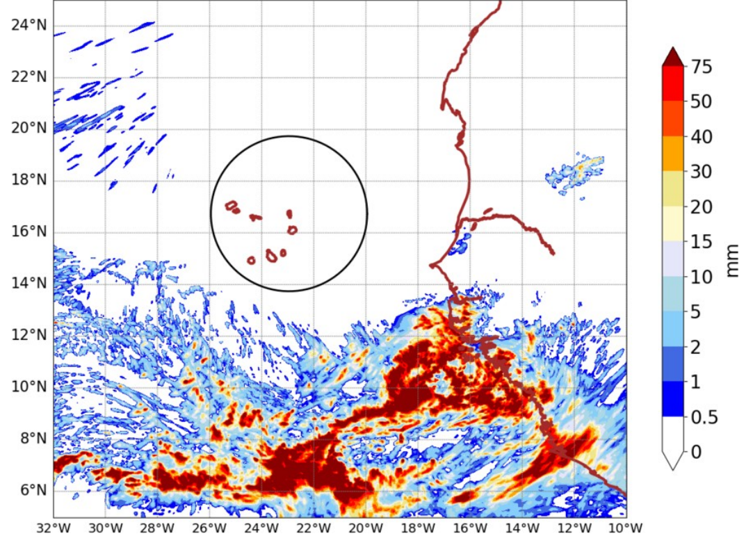
AROME25 20240830-00-UTC -ech(24h)
