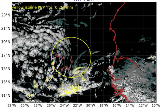
AROME25 20240830-12-UTC -ech(12h) IWP+LWP
