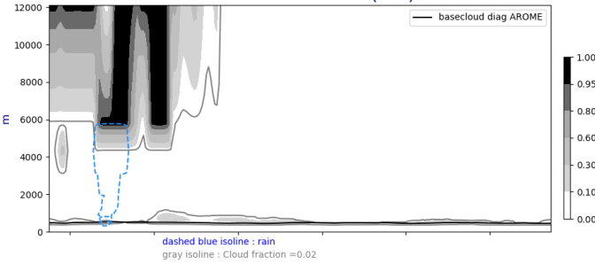
Cross section S/N @ -22W 20240830-12-UTC ech(12h)
