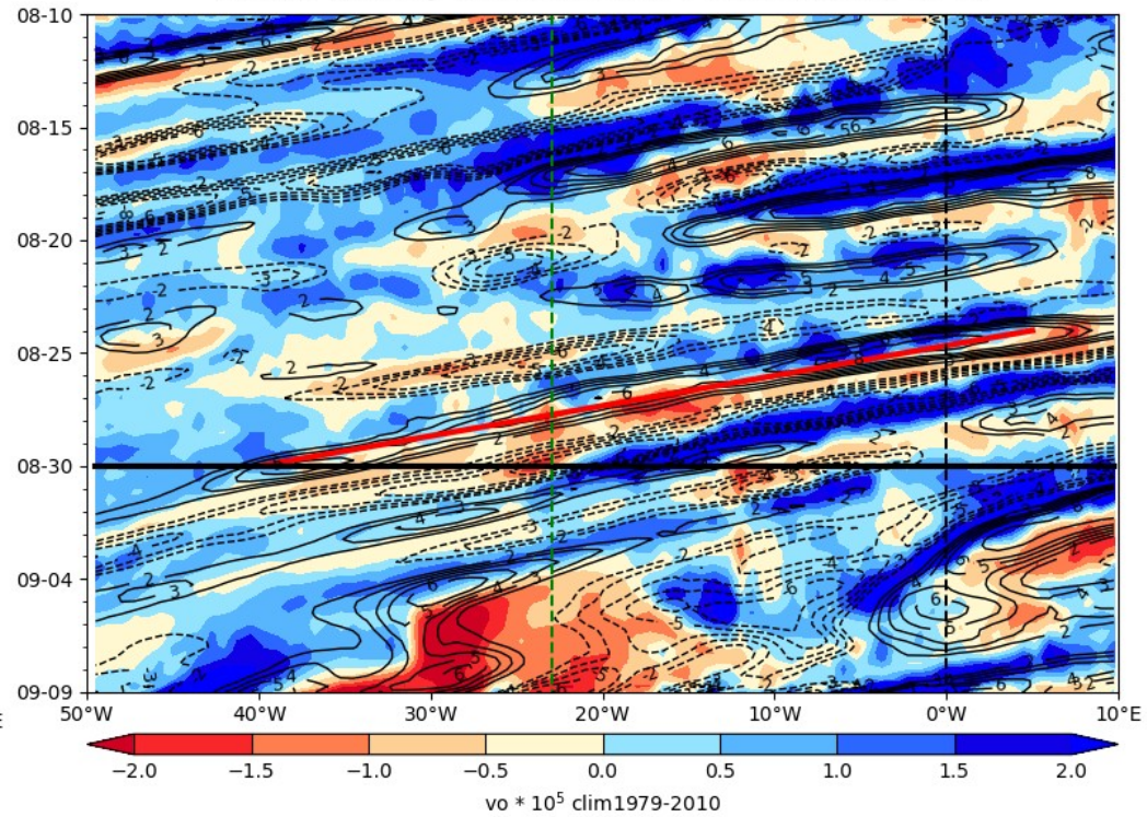
ECMWF Vorticity 850 hPa (color), V-700 hPa 2024-08-30
