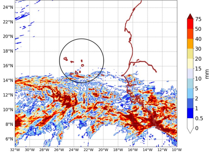
AROME25 20240902-12-UTC -ech(60h) RR cumulated over 24h
