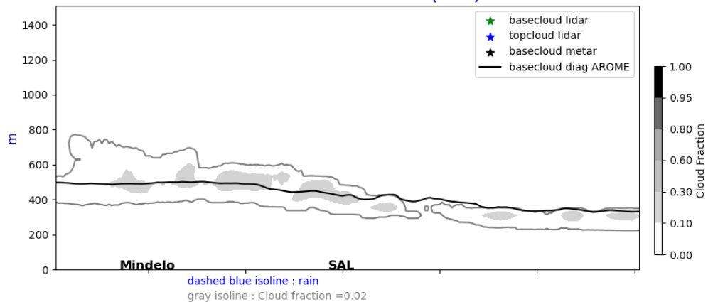
Cross section E/W @ 17.5N 20240901-12-UTC ech(36h)
