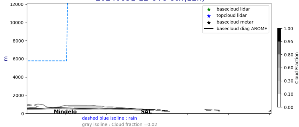
Cross section E/W @ 17.5N 20240831-12-UTC ech(12h)
