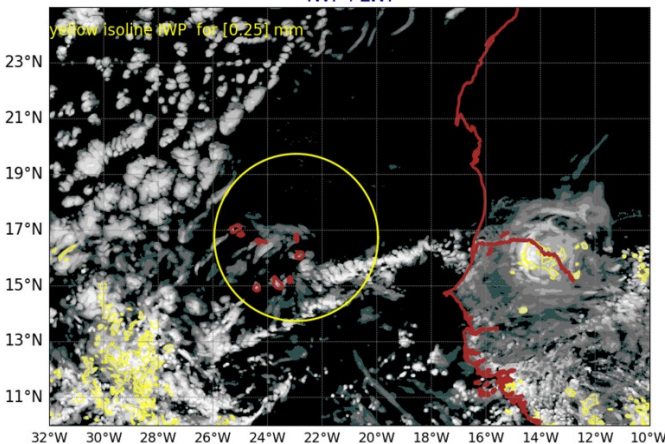
AROME25 20240831-12-UTC -ech(12h) IWP+LWP
