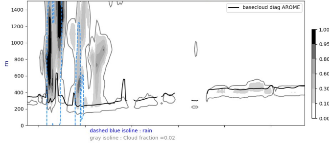
Cross section S/N @ -22W 20240831-12-UTC ech(12h)
