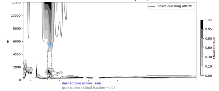
Cross section S/N @ -22W 20240902-12-UTC ech(60h)
