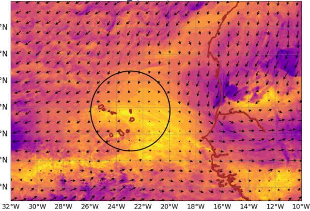
AROME25 20240902-12-UTC -ech(60h) wind_sp920 @ 920hPa
