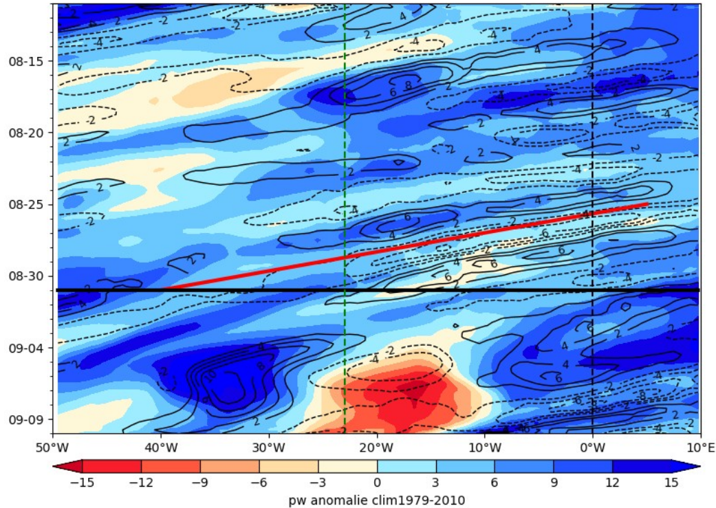
ECMWF PW (color) AND V at 925 hPa 2024-08-31
