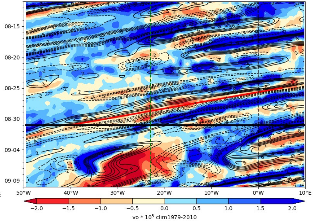
ECMWF Vorticity 850 hPa (color), V-700 hPa 2024-08-31
