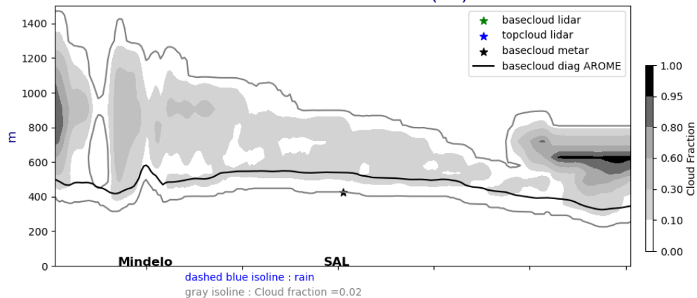
Cross section E/W @ 17.5N 20240831-01-UTC ech(1h)
