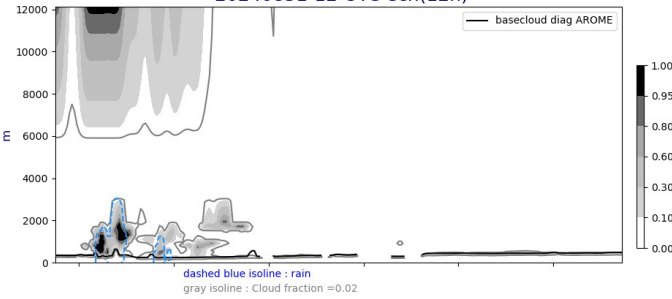
Cross section S/N @ -22W 20240831-12-UTC ech(12h)
