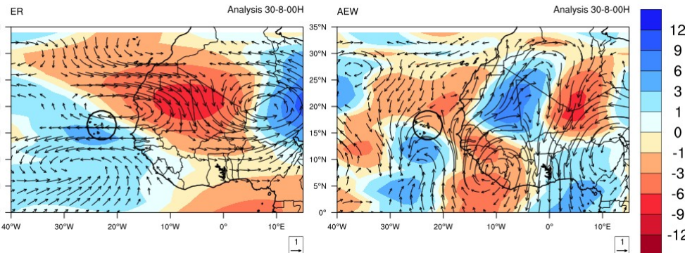
PW and 850hPa wind anomalies
