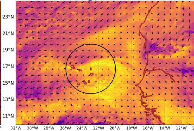
AROME25 20240901-12-UTC -ech(36h) wind_sp920 @ 920hPa
