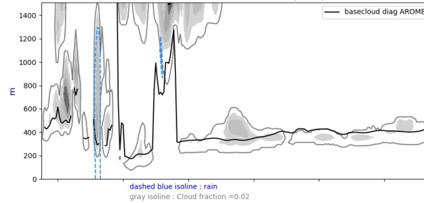
Cross section S/N @ -22W 20240901-12-UTC ech(36h)
