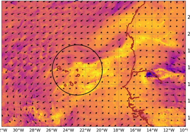
AROME25 20240831-12-UTC -ech(12h) wind_sp920 @ 920hPa
