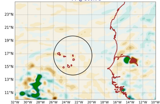
AROME25 20240831-12-UTC -ech(12h) VV @ 500hPa
