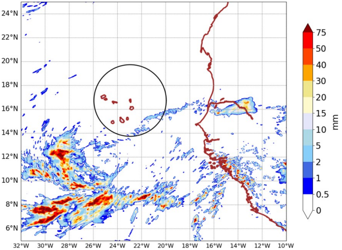
AROME25 20240831-15-UTC -ech(15h) RR cumulated over 6h
