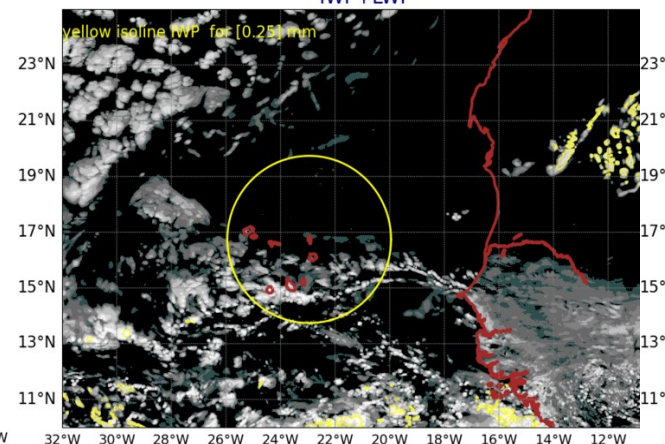
AROME25 20240901-12-UTC -ech(36h) IWP+LWP
