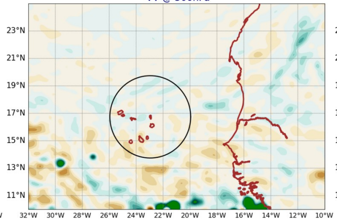
AROME25 20240901-12-UTC -ech(36h) VV @ 500hPa
