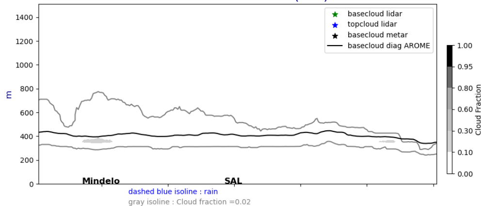
Cross section E/W @ 17.5N 20240902-12-UTC ech(60h)
