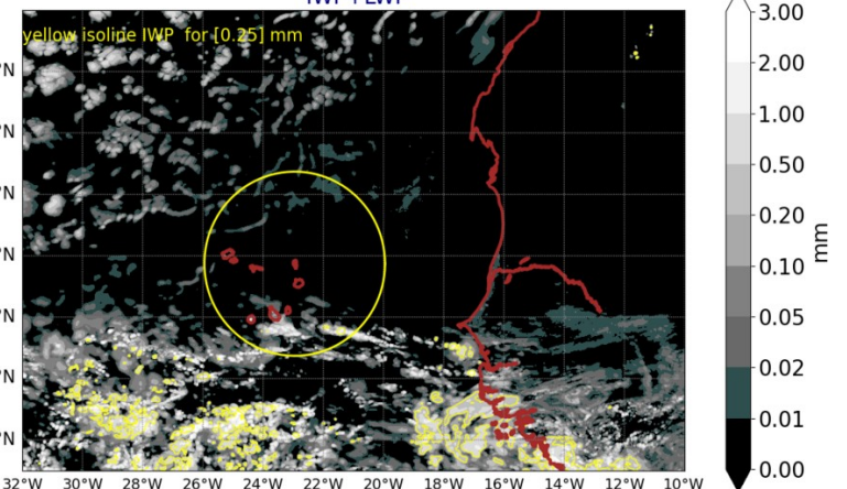
AROME25 20240902-12-UTC -ech(60h) IWP+LWP
