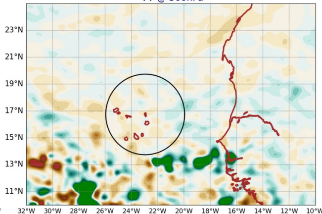
AROME25 20240902-12-UTC -ech(36h) VV @ 500hPa
