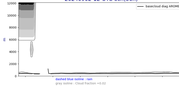
Cross section S/N @ -22W 20240902-12-UTC ech(36h)
