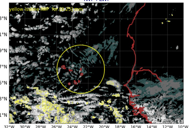
AROME25 20240903-12-UTC -ech(60h) IWP+LWP
