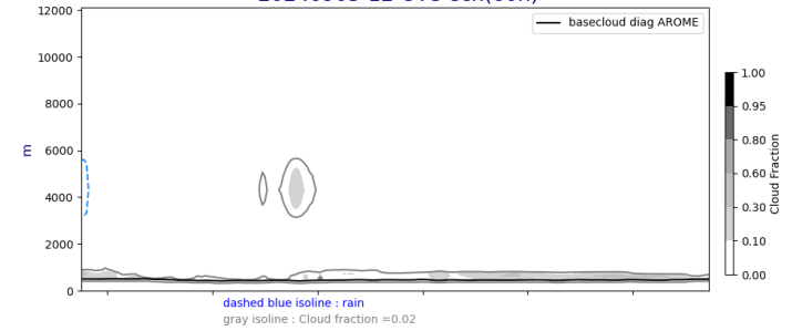
Cross section S/N @ -22W 20240903-12-UTC ech(60h)
