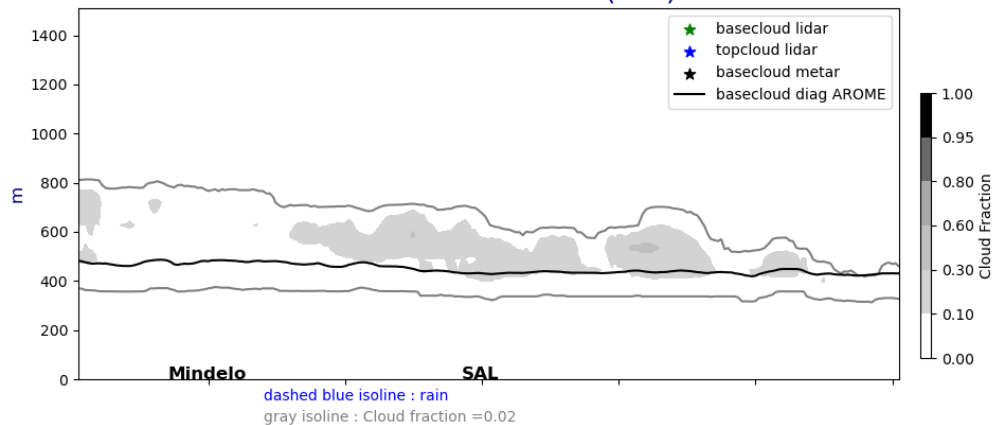
Cross section E/W @ 17.5N 20240902-12-UTC ech(36h)
