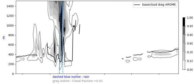
Cross section S/N @ -22W 20240901-12-UTC ech(12h)
