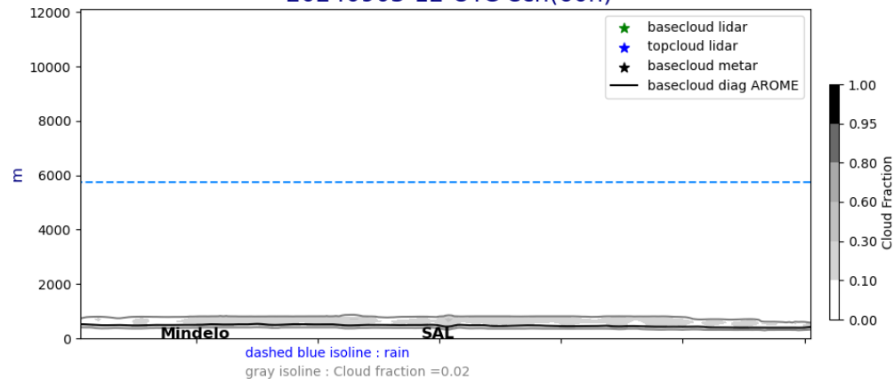
Cross section E/W @ 17.5N 20240903-12-UTC ech(60h)
