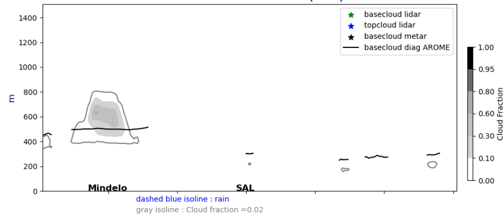
Cross section E/W @ 17.5N 20240901-12-UTC ech(12h)
