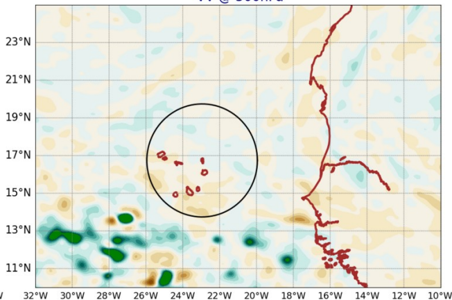
AROME25 20240903-12-UTC -ech(60h) VV @ 500hPa
