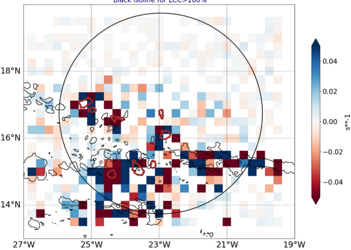
AROME25 regrid 0.25 20240901-12-UTC -ech(12h) blue for conv in subcloud layer black isoline for LCC>100%
