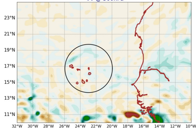
AROME25 20240901-12-UTC -ech(12h) VV @ 500hPa
