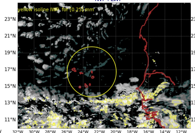
AROME25 20240902-12-UTC -ech(36h) IWP+LWP
