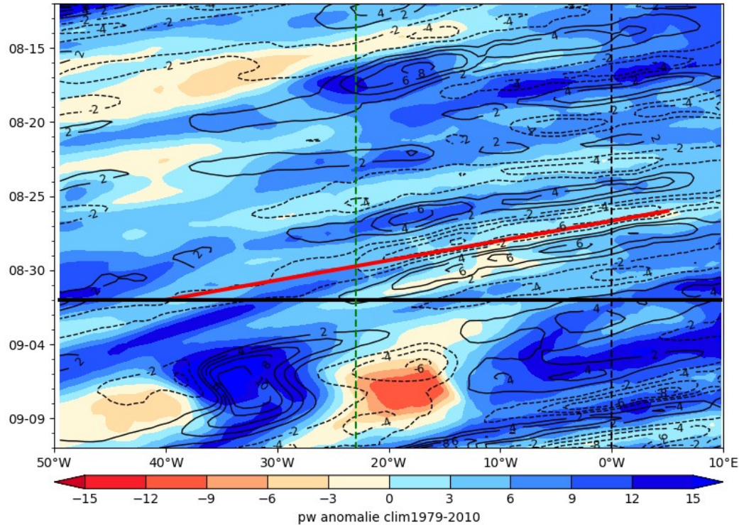
ECMWF PW (color) AND V at 925 hPa 2024-09-01
