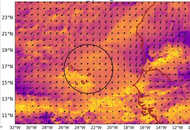
AROME25 20240902-12-UTC -ech(36h) wind_sp920 @ 920hPa
