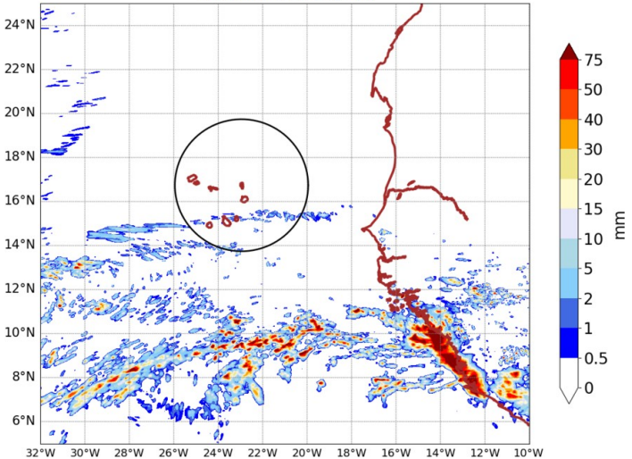
AROME25 20240901-15-UTC -ech(15h) RR cumulated over 6h
