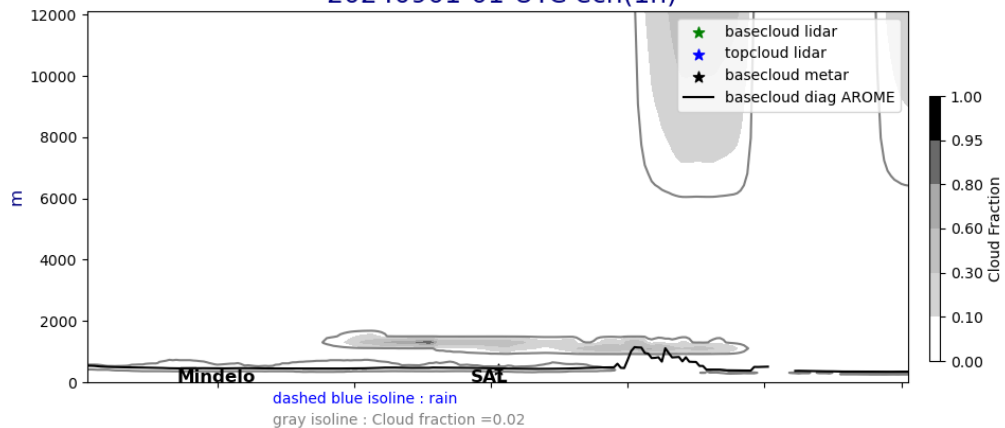
Cross section E/W @ 17.5N 20240901-01-UTC ech(1h)
