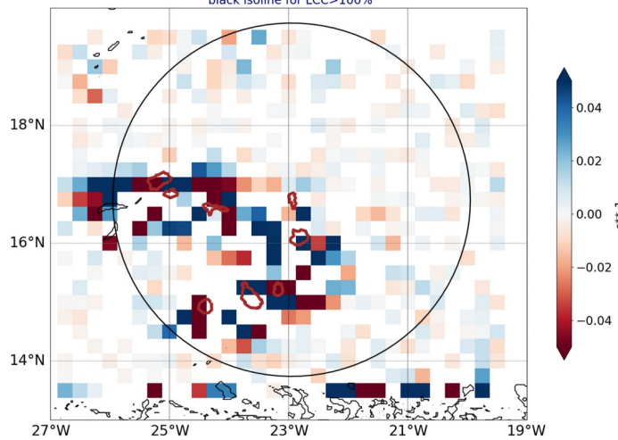
AROME25 regrid 0.25 20240902-12-UTC -ech(36h) blue for conv in subcloud layer black isoline for LCC>100%
