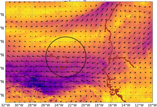
AROME25 20240903-12-UTC -ech(60h) wind_sp920 @ 920hPa
