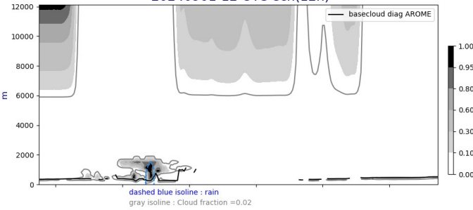
Cross section S/N @ -22W 20240901-12-UTC ech(12h)
