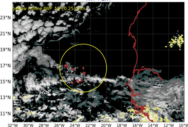
AROME25 20240901-12-UTC -ech(12h) IWP+LWP
