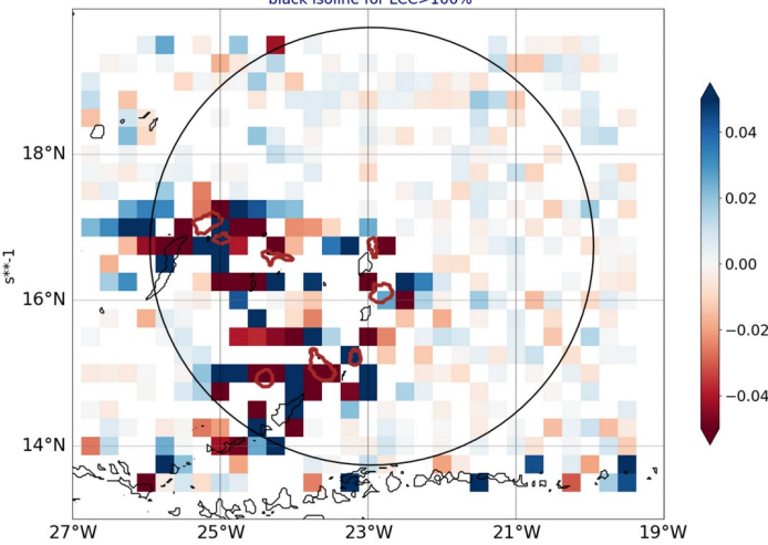
AROME25 regrid 0.25 20240903-12-UTC -ech(60h) blue for conv in subcloud layer black isoline for LCC>100%
