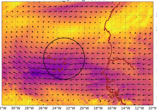
AROME25 20240901-12-UTC -ech(12h) wind_sp920 @ 920hPa
