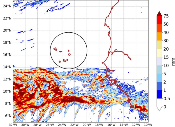
AROME25 20240903-12-UTC -ech(60h) RR cumulated over 24h
