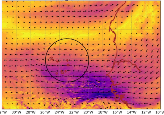
AROME25 20240902-12-UTC -ech(12h) wind_sp920 @ 920hPa
