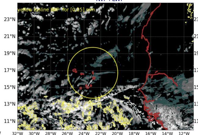
AROME25 20240903-12-UTC -ech(36h) IWP+LWP
