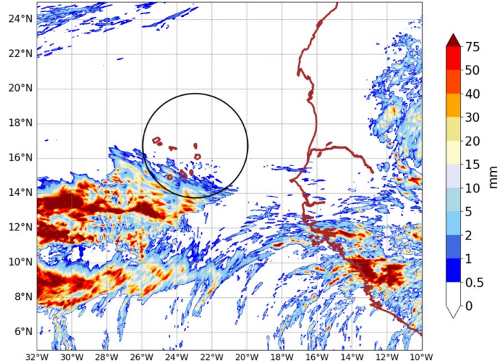
AROME25 20240904-12-UTC -ech(60h) RR cumulated over 24h
