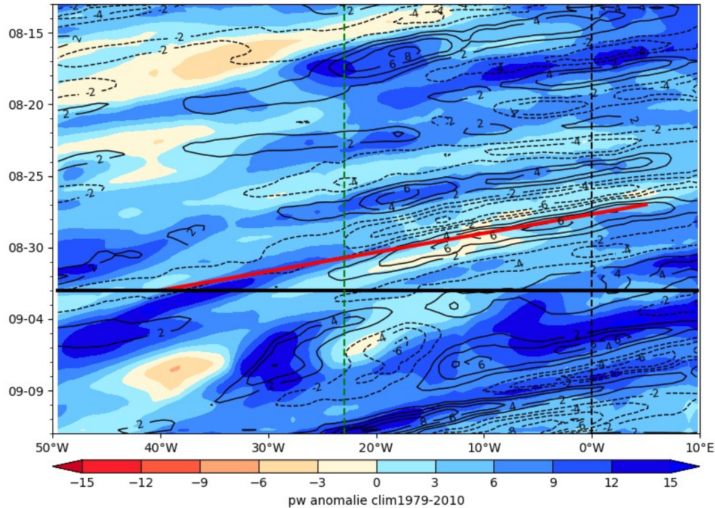
ECMWF PW (color) AND V at 925 hPa 2024-09-02
