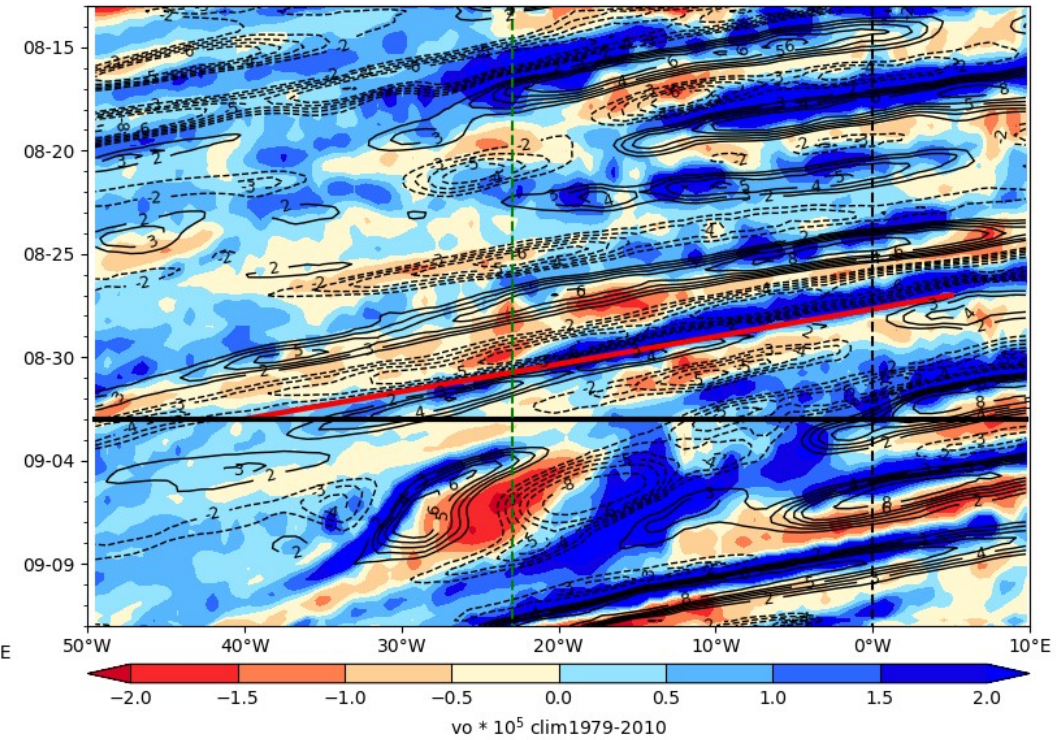
ECMWF Vorticity 850 hPa (color), V-700 hPa 2024-09-02
