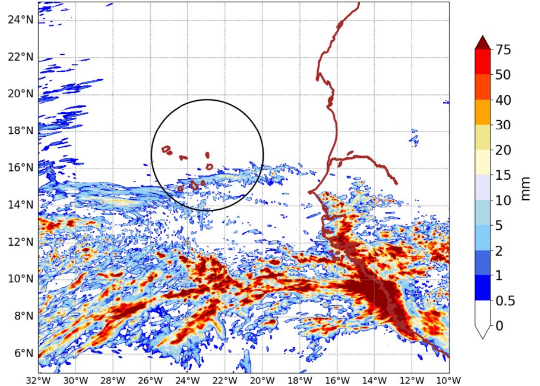
AROME25 20240902-00-UTC -ech(24h)
