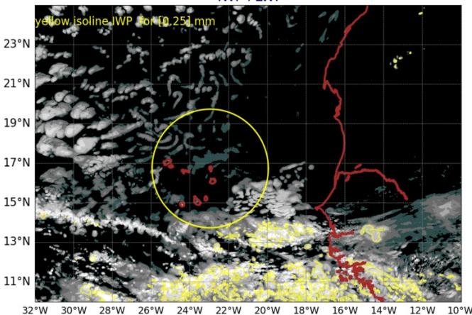
AROME25 20240902-12-UTC -ech(12h) IWP+LWP
