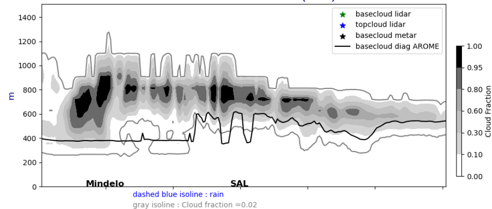
Cross section E/W @ 17.5N 20240904-12-UTC ech(60h)
