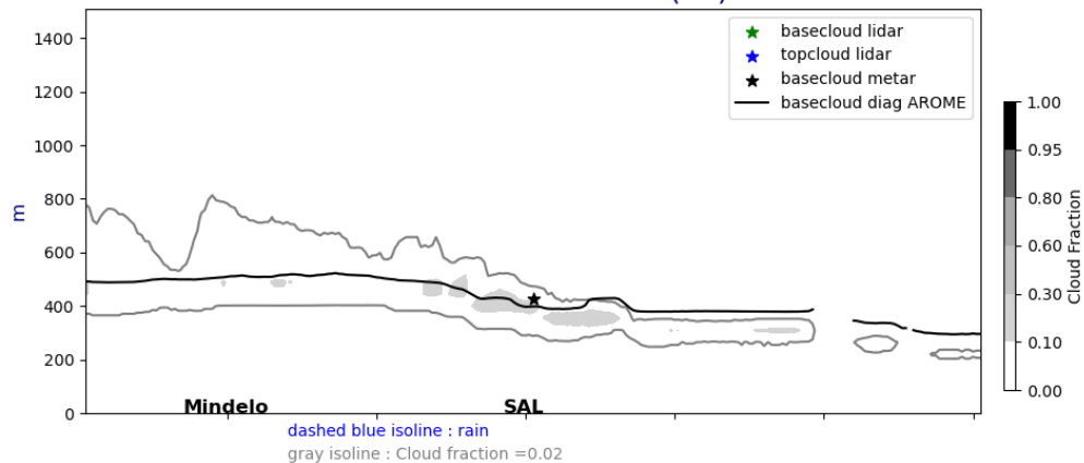
Cross section E/W @ 17.5N 20240902-01-UTC ech(1h)
