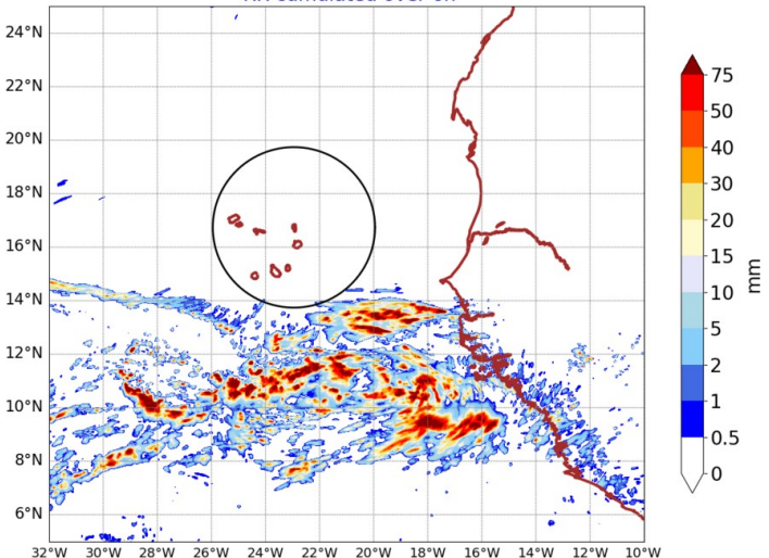
AROME25 20240902-15-UTC -ech(15h) RR cumulated over 6h
