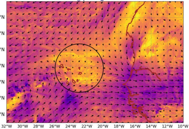
AROME25 20240904-12-UTC -ech(60h) wind_sp920 @ 920hPa
