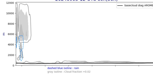
Cross section S/N @ -22W 20240903-12-UTC ech(36h)
