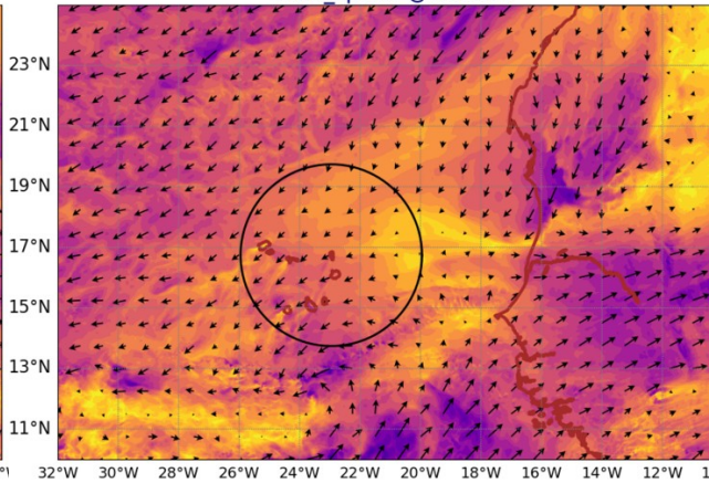
AROME25 20240903-12-UTC -ech(36h) wind_sp920 @ 920hPa
