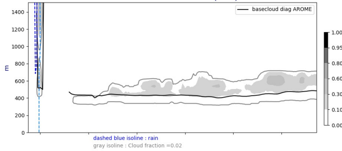
Cross section S/N @ -22W 20240902-12-UTC ech(12h)
