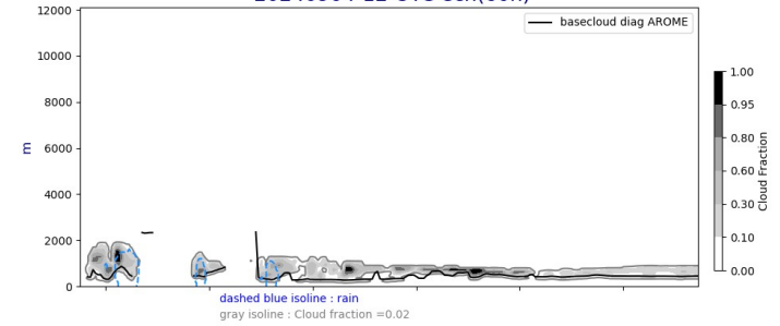
Cross section S/N @ -22W 20240904-12-UTC ech(60h)
