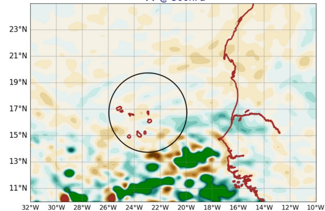
AROME25 20240902-12-UTC -ech(12h) VV @ 500hPa
