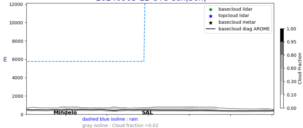
Cross section E/W @ 17.5N 20240903-12-UTC ech(36h)
