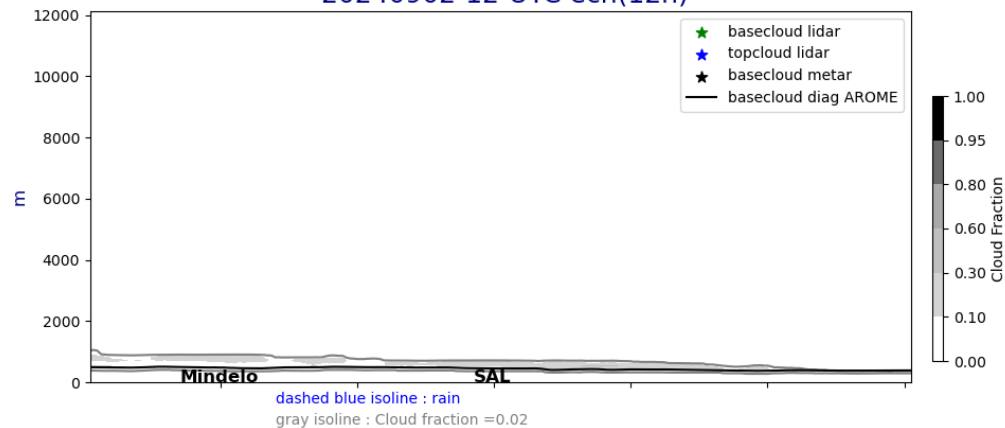
Cross section E/W @ 17.5N 20240902-12-UTC ech(12h)
