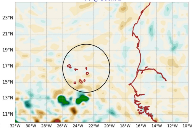
AROME25 20240903-12-UTC -ech(36h) VV @ 500hPa
