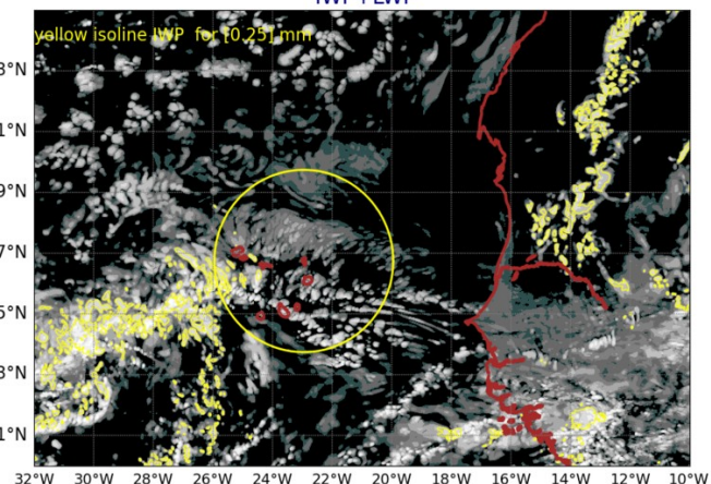
AROME25 20240904-12-UTC -ech(60h) IWP+LWP
