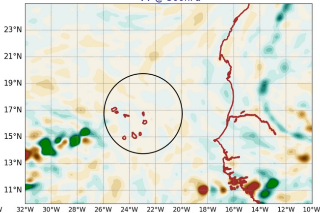
AROME25 20240904-12-UTC -ech(60h) VV @ 500hPa
