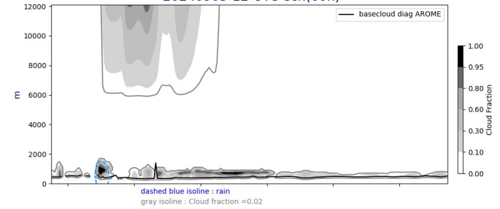
Cross section S/N @ -22W 20240905-12-UTC ech(60h)
