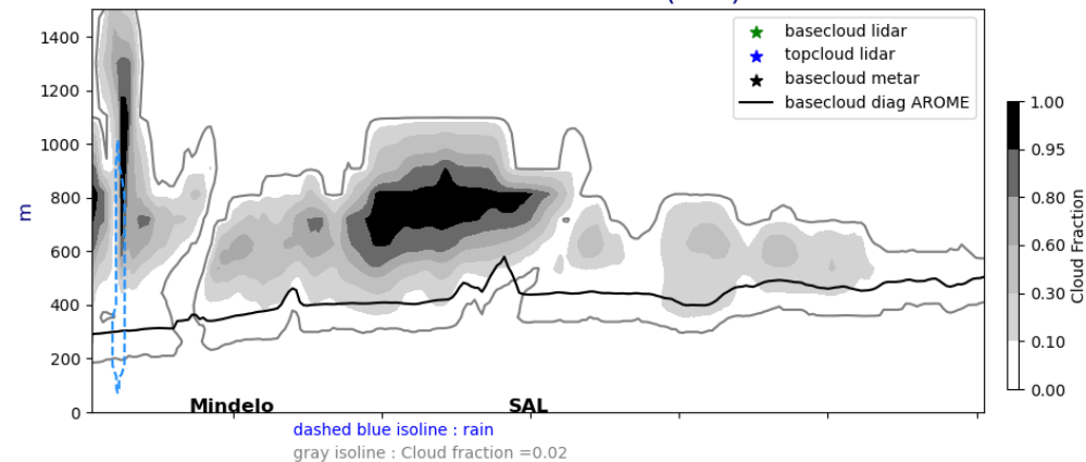
Cross section E/W @ 17.5N 20240905-12-UTC ech(60h)
