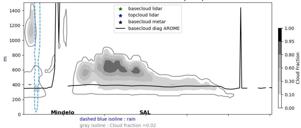
Cross section E/W @ 17.5N 20240904-12-UTC ech(36h)
