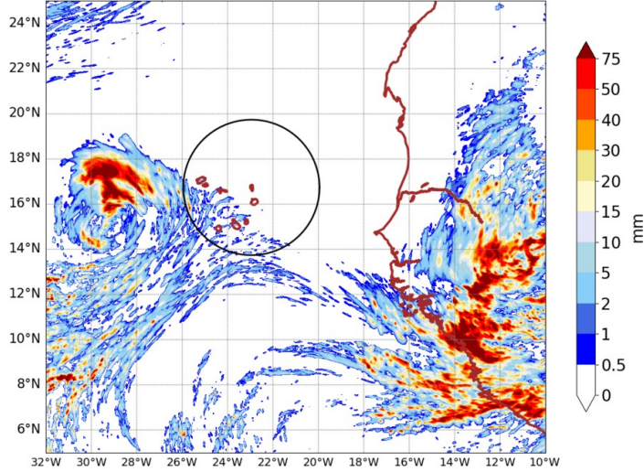
AROME25 20240905-12-UTC -ech(60h) RR cumulated over 24h
