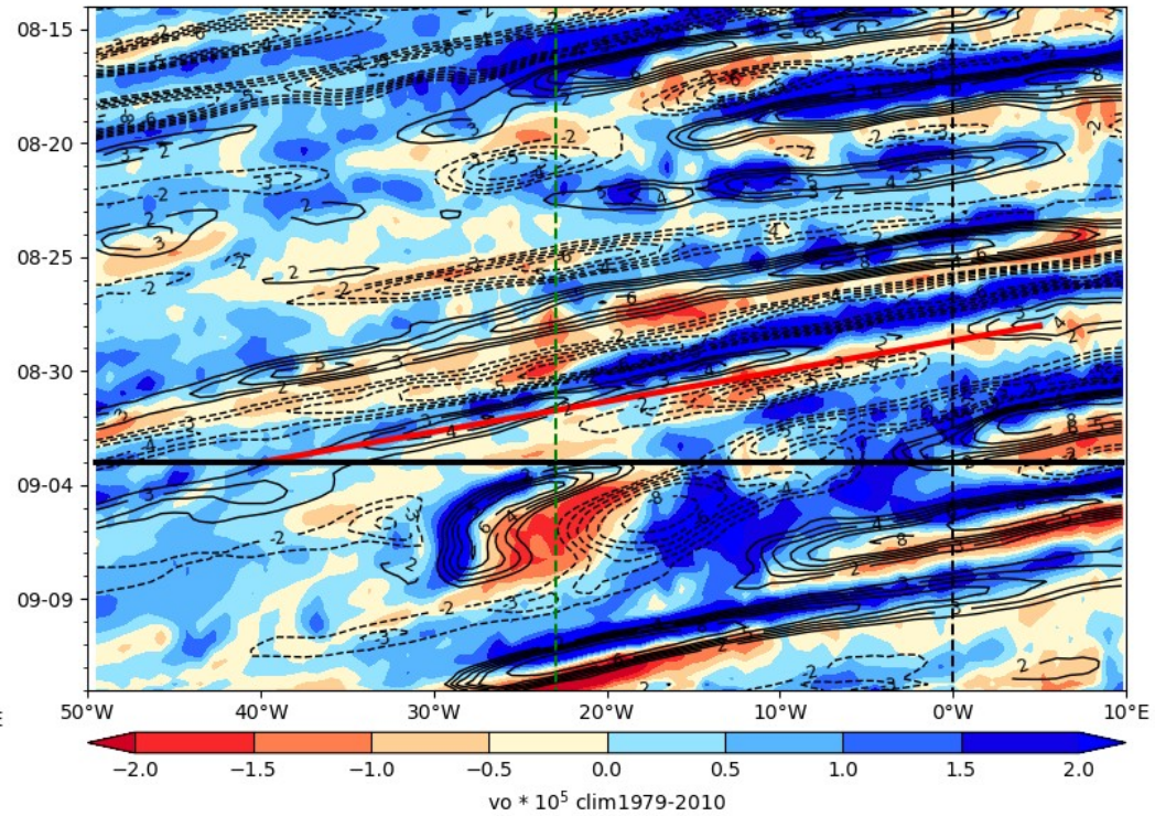
ECMWF Vorticity 850 hPa (color), V-700 hPa 2024-09-03
