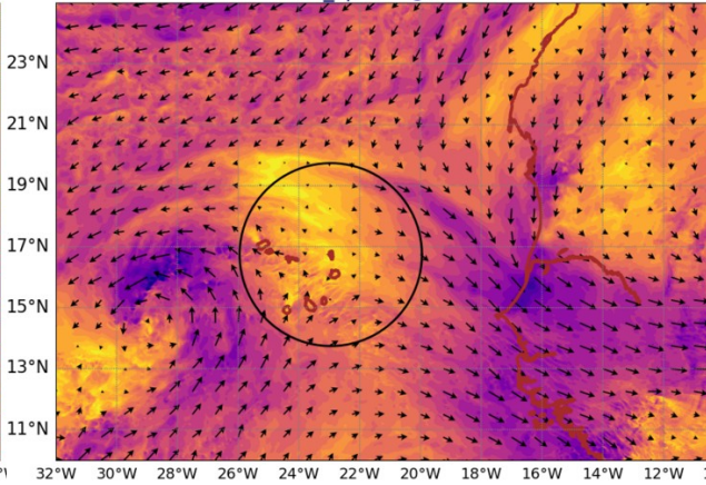
AROME25 20240904-12-UTC -ech(36h) wind_sp920 @ 920hPa
