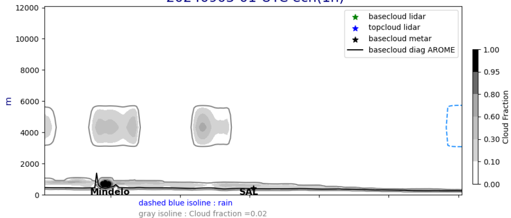
Cross section E/W @ 17.5N 20240903-01-UTC ech(1h)
