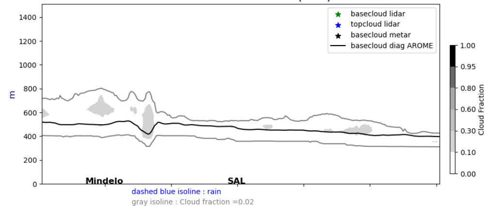
Cross section E/W @ 17.5N 20240903-12-UTC ech(12h)
