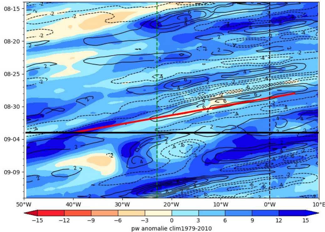
ECMWF PW (color) AND V at 925 hPa 2024-09-03
