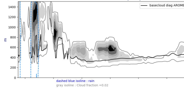
Cross section S/N @ -22W 20240904-12-UTC ech(36h)
