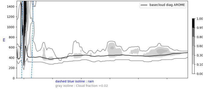
Cross section S/N @ -22W 20240903-12-UTC ech(12h)
