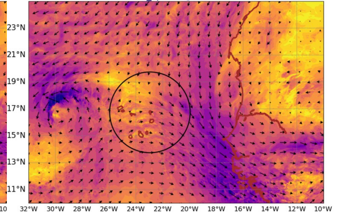
AROME25 20240905-12-UTC -ech(60h) wind_sp920 @ 920hPa
