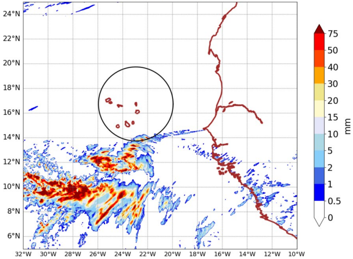
AROME25 20240903-15-UTC -ech(15h) RR cumulated over 6h
