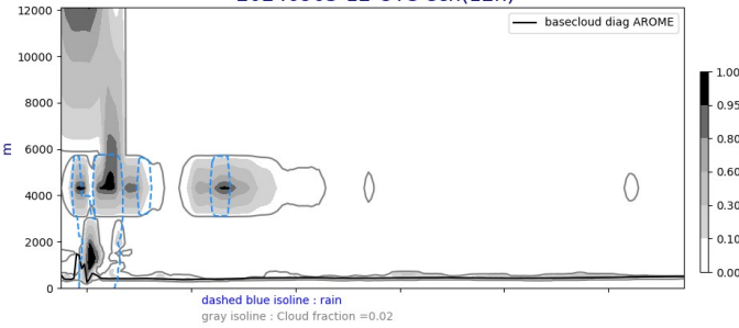
Cross section S/N @ -22W 20240903-12-UTC ech(12h)
