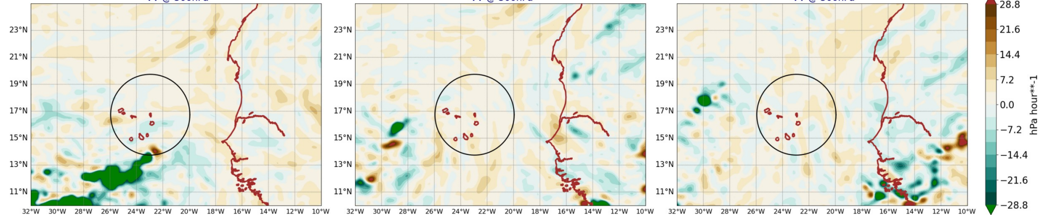
AROME25 20240903-12-UTC -ech(12h) VV @ 500hPa
