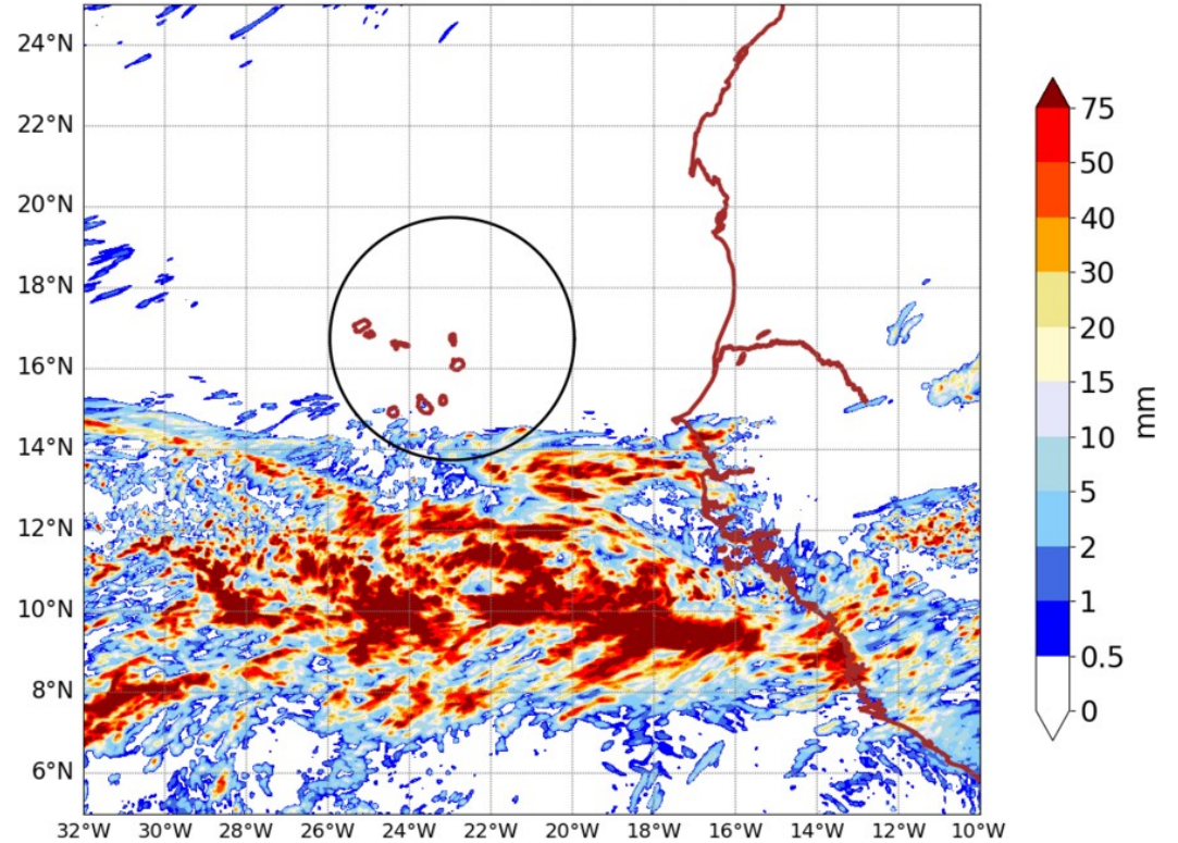
AROME25 20240903-00-UTC -ech(24h)
