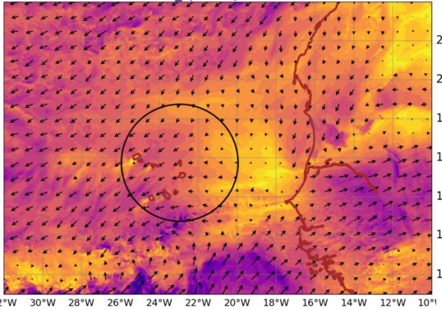
AROME25 20240903-12-UTC -ech(12h) wind_sp920 @ 920hPa
