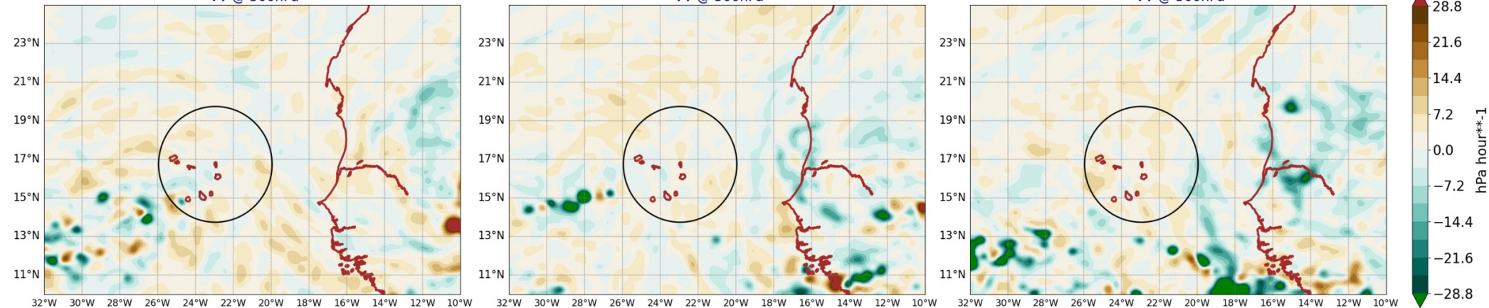
AROME25 20240904-12-UTC -ech(12h) VV @ 500hPa
