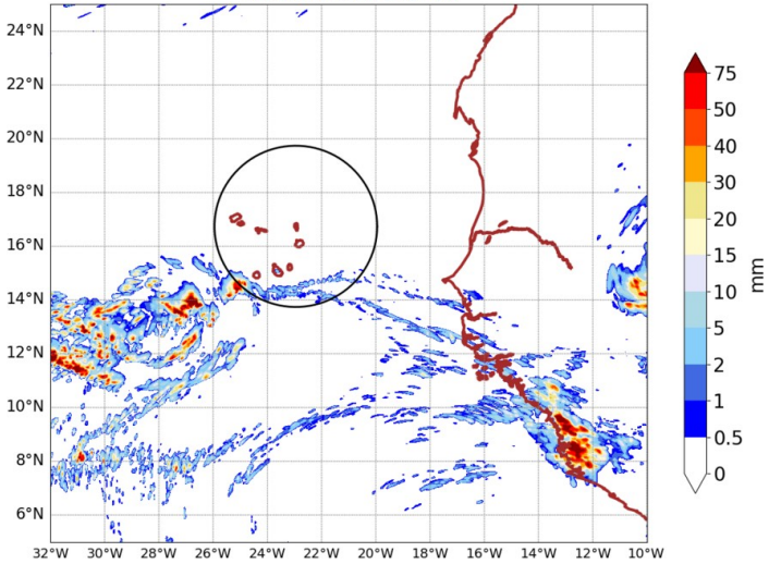
AROME25 20240904-15-UTC -ech(15h) RR cumulated over 6h
