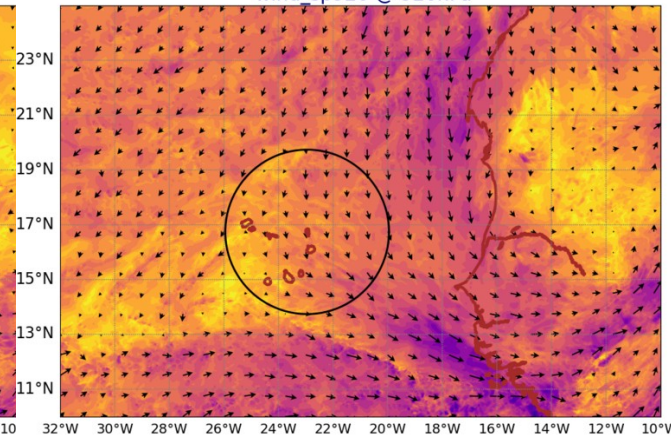
AROME25 20240906-12-UTC -ech(60h) wind_sp920 @ 920hPa
