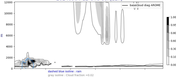
Cross section S/N @ -22W 20240904-12-UTC ech(12h)
