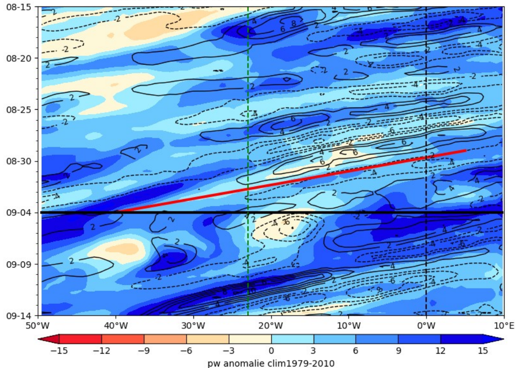
ECMWF PW (color) AND V at 925 hPa 2024-09-04
