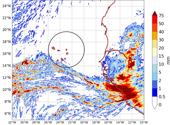
AROME25 20240906-12-UTC -ech(60h) RR cumulated over 24h
