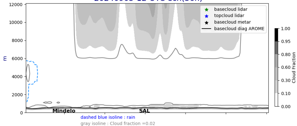
Cross section E/W @ 17.5N 20240905-12-UTC ech(36h)
