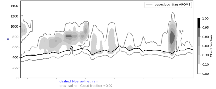
Cross section S/N @ -22W 20240906-12-UTC ech(60h)
