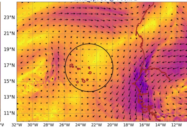
AROME25 20240905-12-UTC -ech(36h) wind_sp920 @ 920hPa
