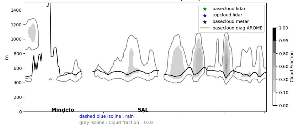
Cross section E/W @ 17.5N 20240906-12-UTC ech(60h)
