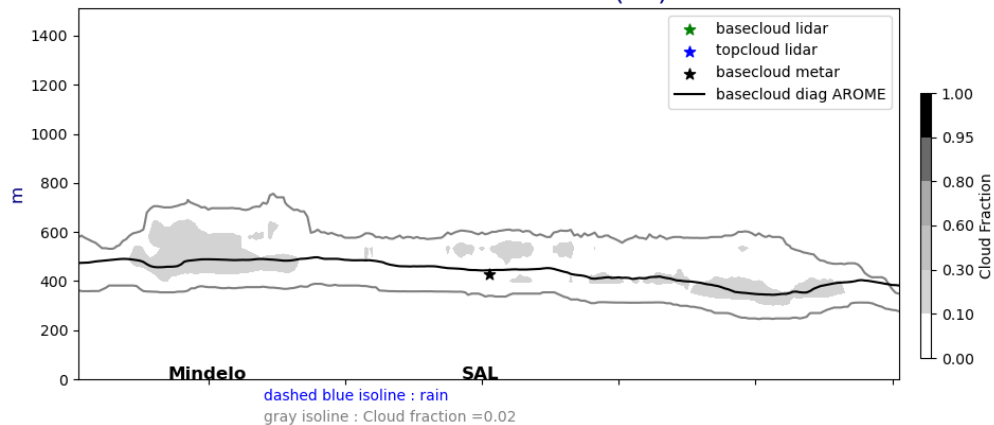
Cross section E/W @ 17.5N 20240904-01-UTC ech(1h)
