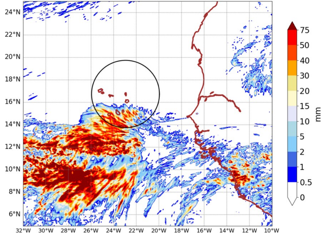
AROME25 20240904-00-UTC -ech(24h)
