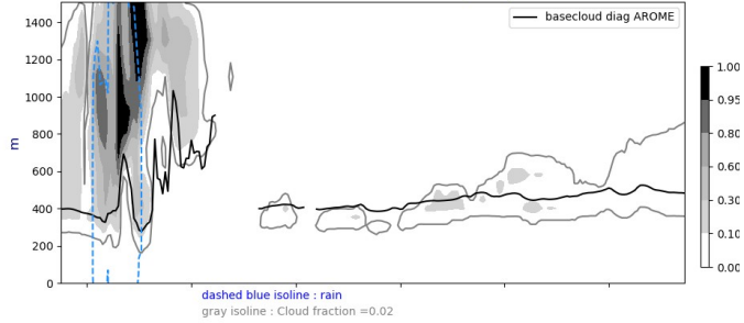
Cross section S/N @ -22W 20240904-12-UTC ech(12h)
