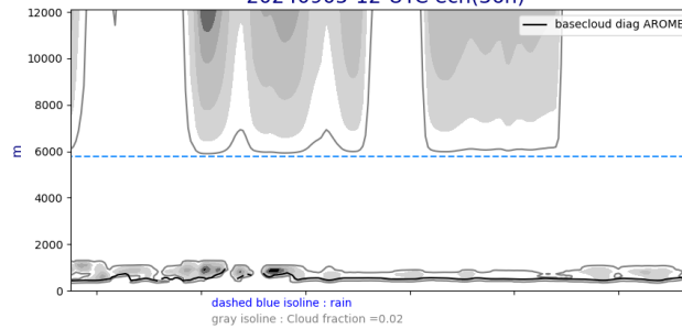
Cross section S/N @ -22W 20240905-12-UTC ech(36h)
