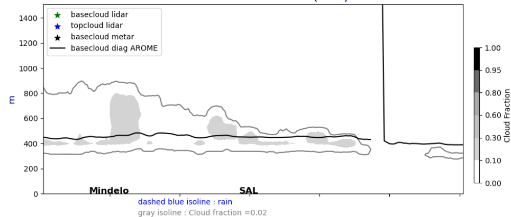
Cross section E/W @ 17.5N 20240904-12-UTC ech(12h)
