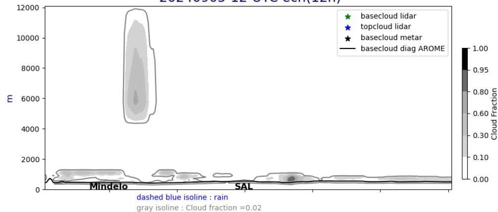
Cross section E/W @ 17.5N 20240905-12-UTC ech(12h)
