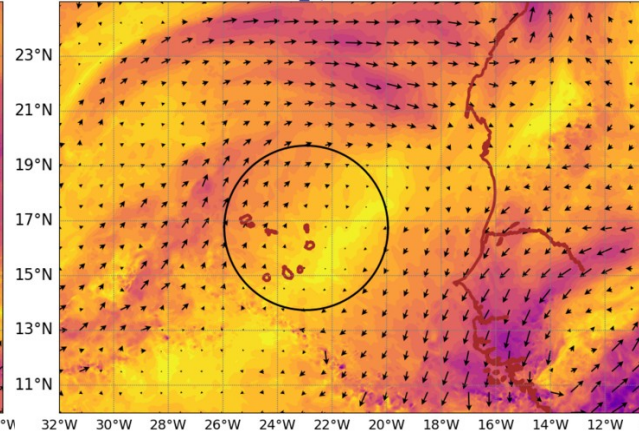
AROME25 20240906-12-UTC -ech(36h) wind_sp920 @ 920hPa
