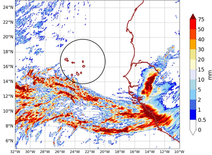
AROME25 20240907-12-UTC -ech(60h) RR cumulated over 24h
