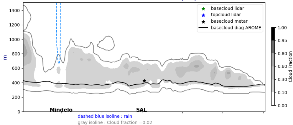
Cross section E/W @ 17.5N 20240905-01-UTC ech(1h)
