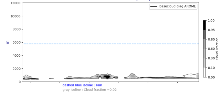
Cross section S/N @ -22W 20240907-12-UTC ech(60h)
