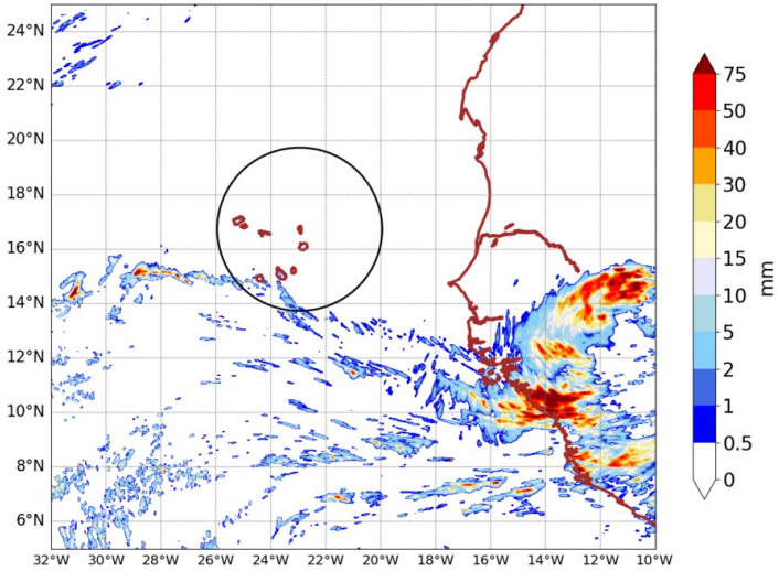
AROME25 20240905-15-UTC -ech(15h) RR cumulated over 6h
