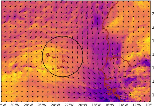
AROME25 20240905-12-UTC -ech(12h) wind_sp920 @ 920hPa
