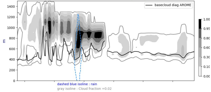
Cross section S/N @ -22W 20240905-12-UTC ech(12h)
