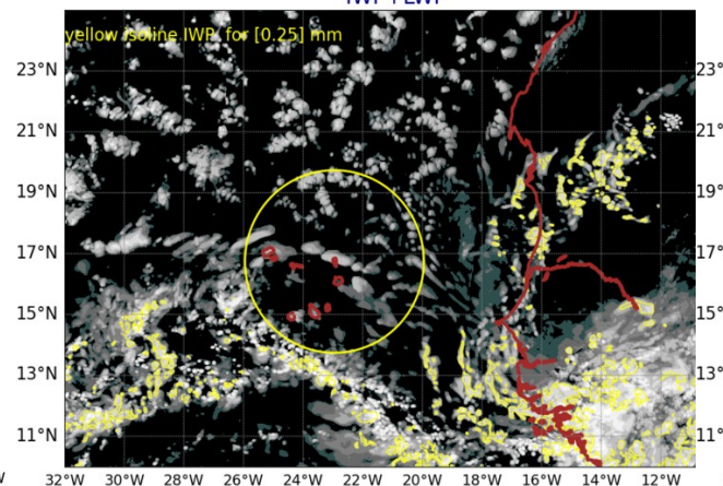
AROME25 20240906-12-UTC -ech(36h) IWP+LWP
