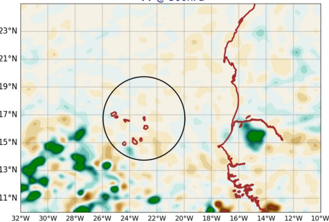
AROME25 20240907-12-UTC -ech(60h) VV @ 500hPa
