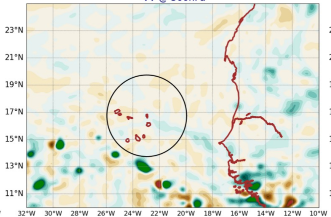
AROME25 20240906-12-UTC -ech(36h) VV @ 500hPa
