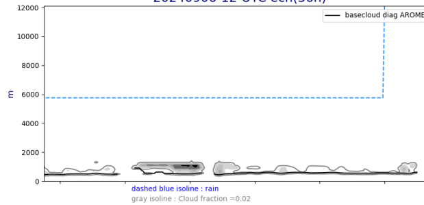
Cross section S/N @ -22W 20240906-12-UTC ech(36h)
