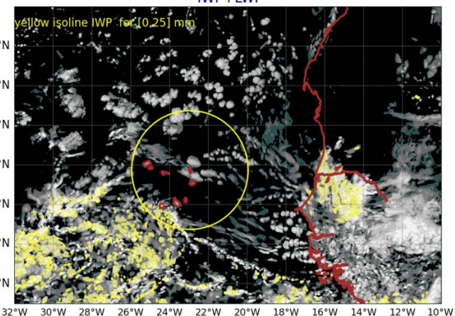
AROME25 20240907-12-UTC -ech(60h) IWP+LWP
