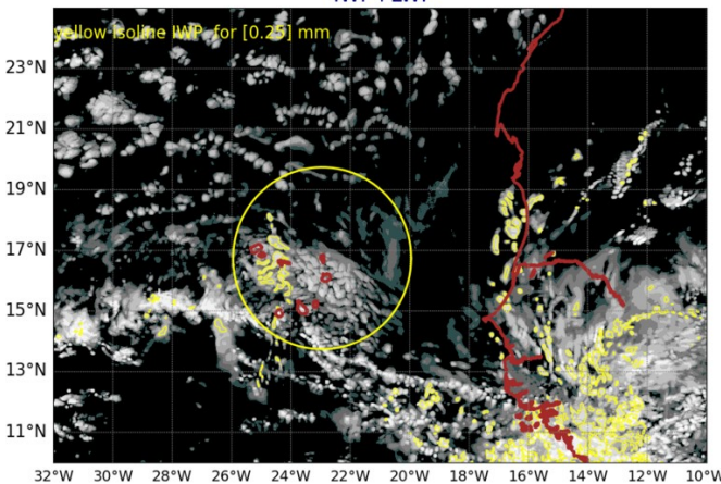
AROME25 20240905-12-UTC -ech(12h) IWP+LWP
