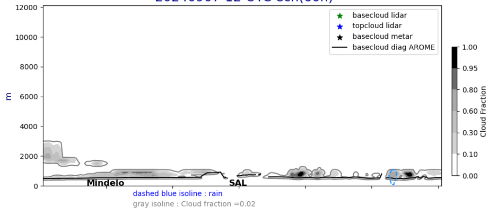
Cross section E/W @ 17.5N 20240907-12-UTC ech(60h)
