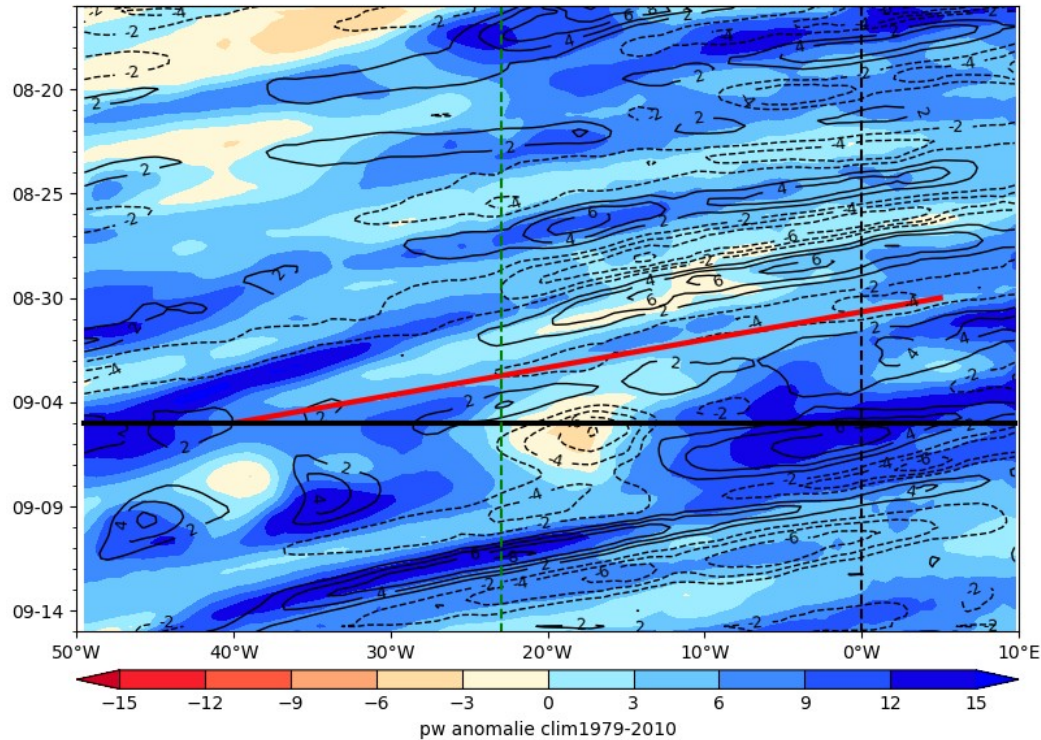
ECMWF PW (color) AND V at 925 hPa 2024-09-05
