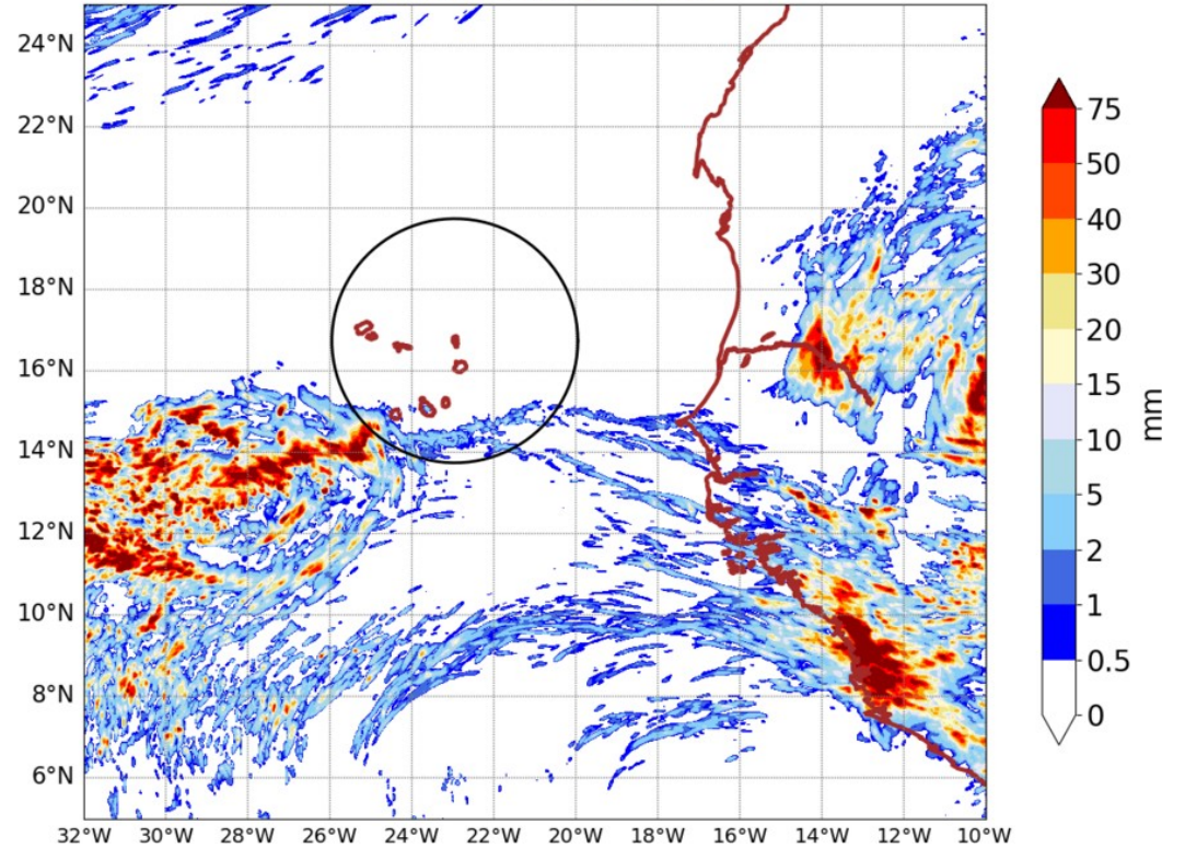
AROME25 20240905-00-UTC -ech(24h)
