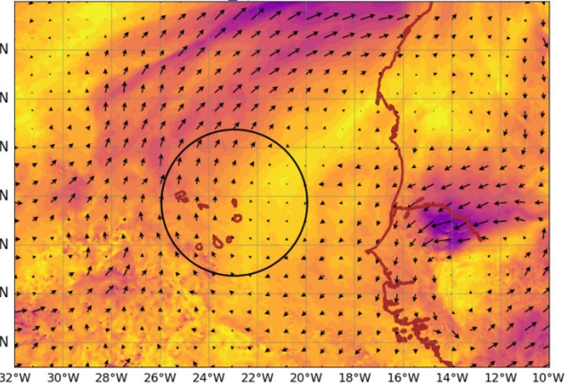
AROME25 20240907-12-UTC -ech(60h) wind_sp920 @ 920hPa
