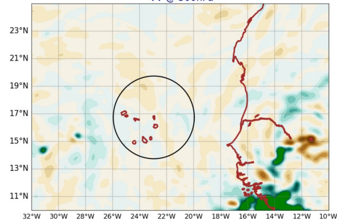
AROME25 20240905-12-UTC -ech(12h) VV @ 500hPa
