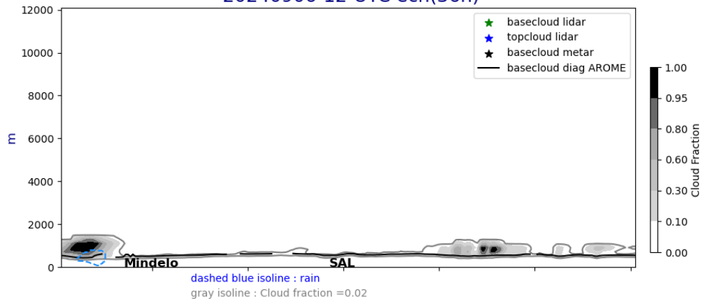
Cross section E/W @ 17.5N 20240906-12-UTC ech(36h)
