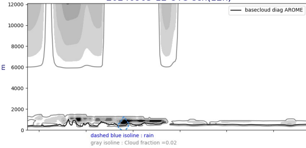
Cross section S/N @ -22W 20240905-12-UTC ech(12h)
