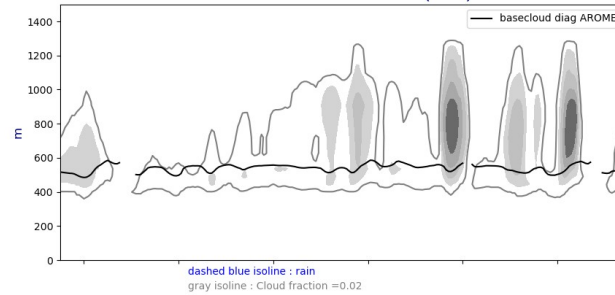
Cross section S/N @ -22W 20240908-12-UTC ech(36h)
