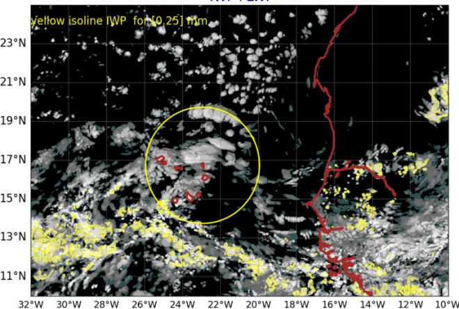
AROME25 20240907-12-UTC -ech(12h) IWP+LWP
