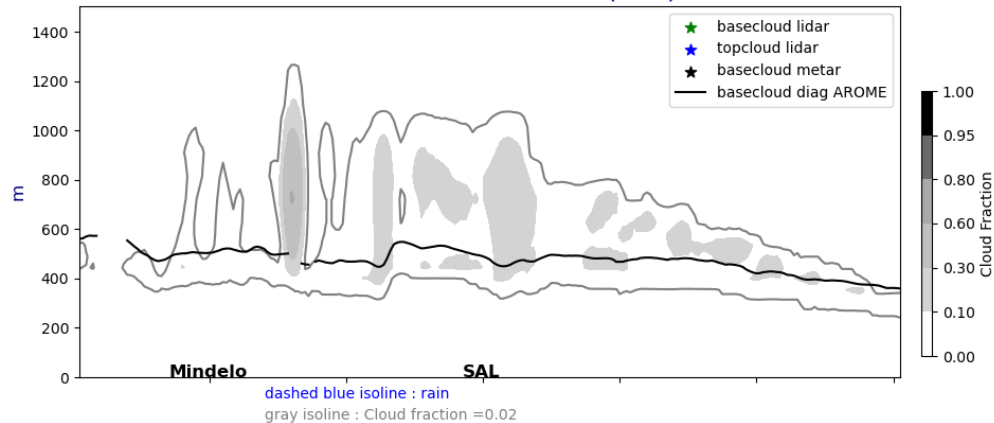
Cross section E/W @ 17.5N 20240909-12-UTC ech(60h)
