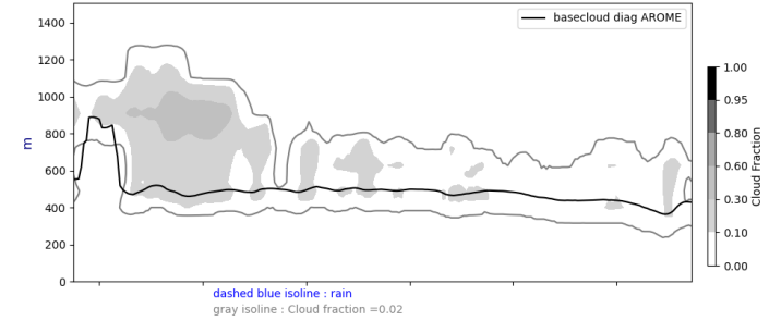
Cross section S/N @ -22W 20240909-12-UTC ech(60h)
