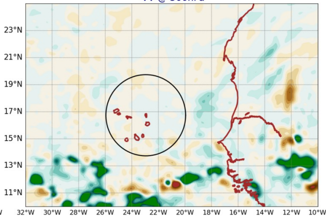
AROME25 20240909-12-UTC -ech(60h) VV @ 500hPa
