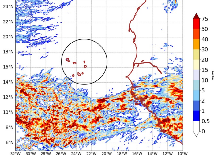
AROME25 20240909-12-UTC -ech(60h) RR cumulated over 24h
