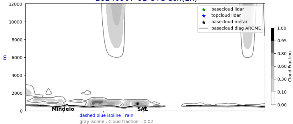
Cross section E/W @ 17.5N 20240907-01-UTC ech(1h)
