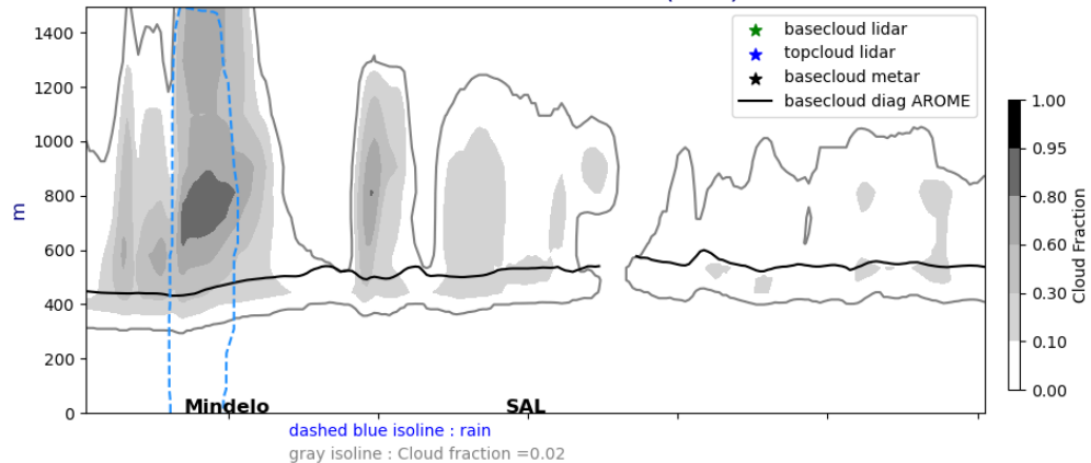
Cross section E/W @ 17.5N 20240908-12-UTC ech(36h)
