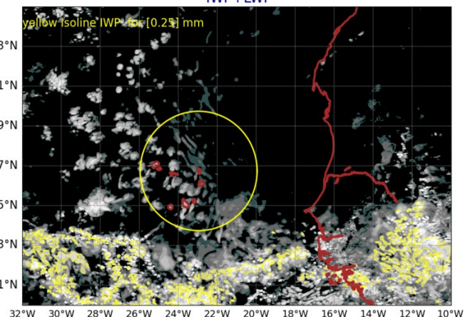
AROME25 20240909-12-UTC -ech(60h) IWP+LWP
