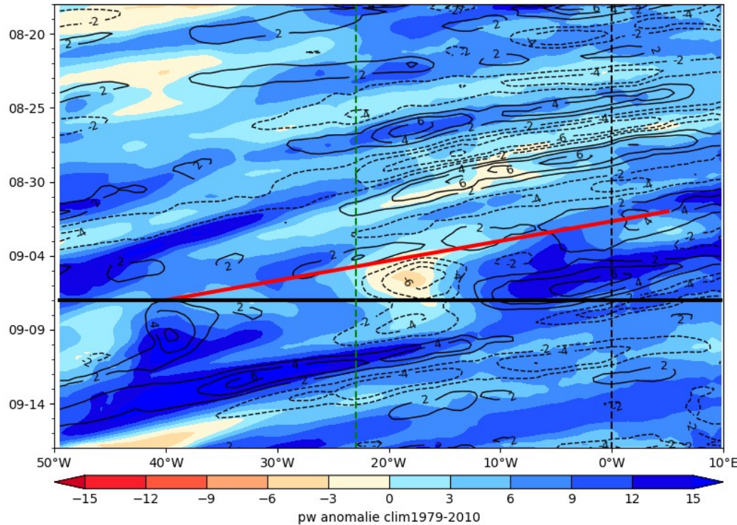
ECMWF PW (color) AND V at 925 hPa 2024-09-07
