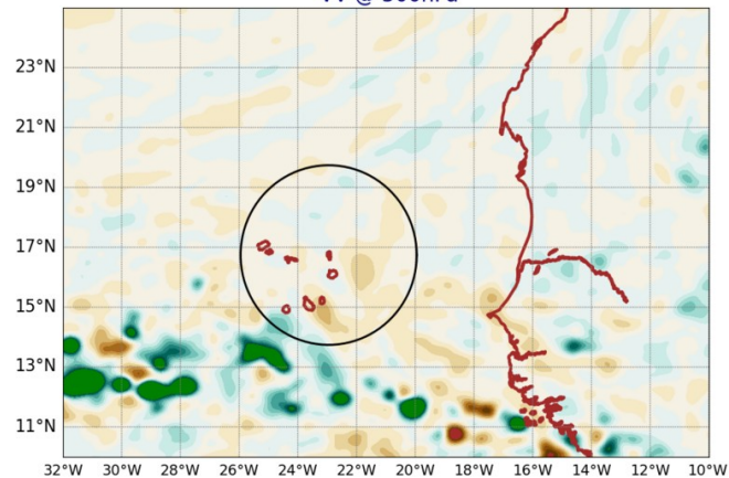
AROME25 20240907-12-UTC -ech(12h) VV @ 500hPa
