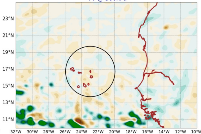
AROME25 20240908-12-UTC -ech(36h) VV @ 500hPa
