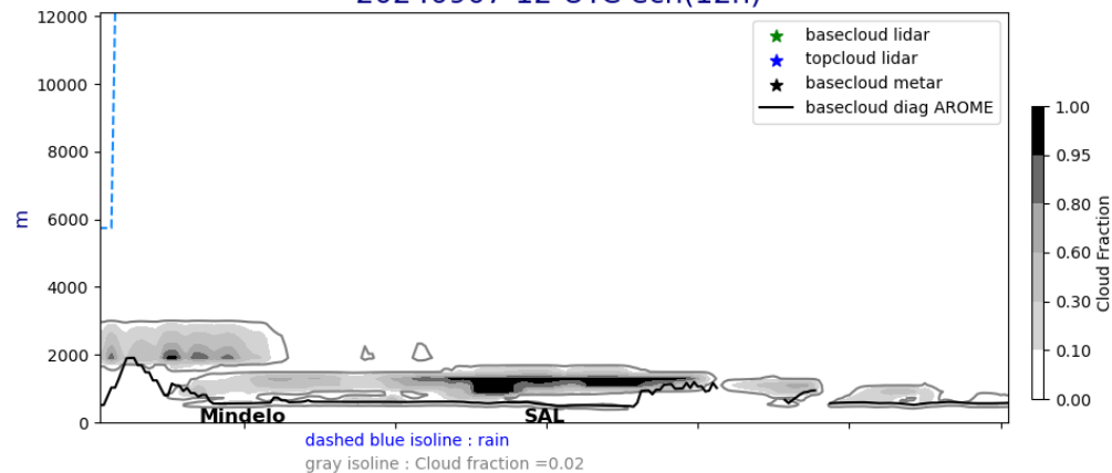
Cross section E/W @ 17.5N 20240907-12-UTC ech(12h)
