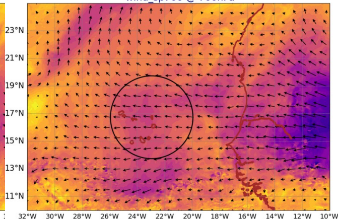
AROME25 20240909-12-UTC -ech(60h) wind_sp920 @ 920hPa
