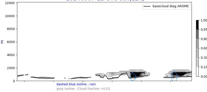
Cross section S/N @ -22W 20240907-12-UTC ech(12h)
