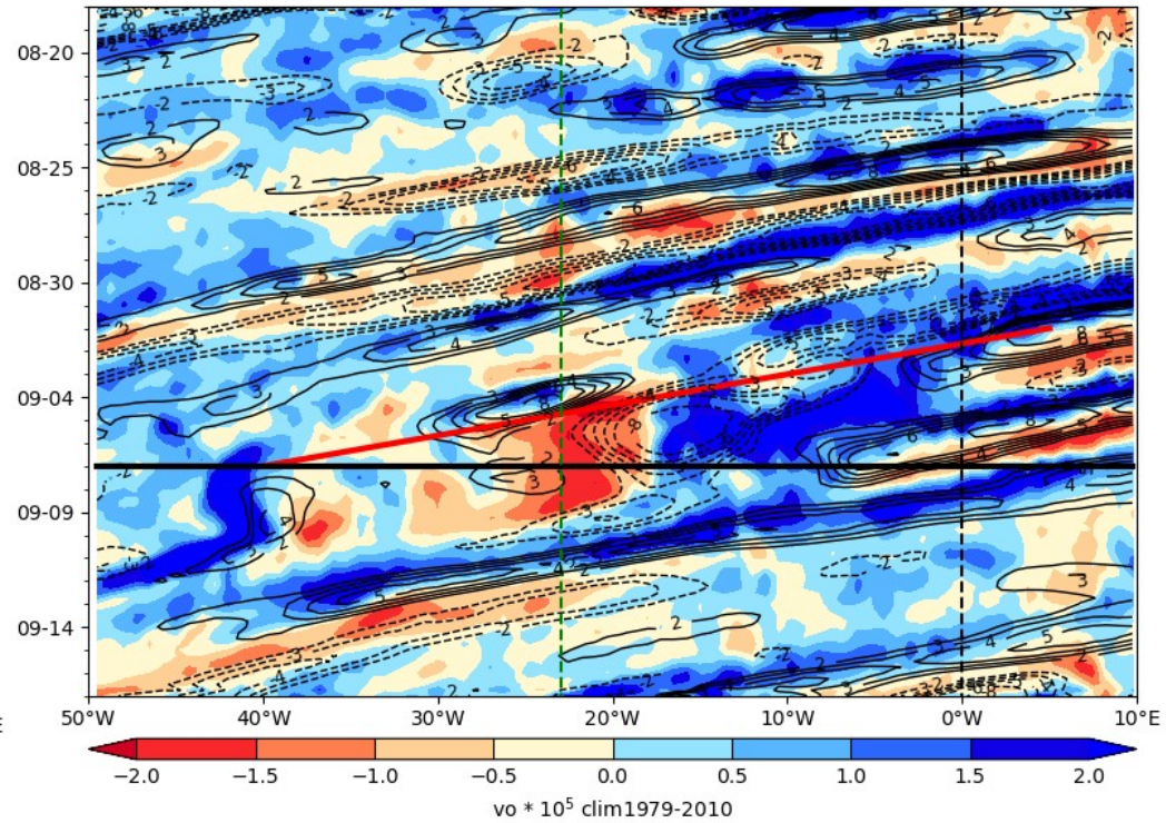
ECMWF Vorticity 850 hPa (color), V-700 hPa 2024-09-07
