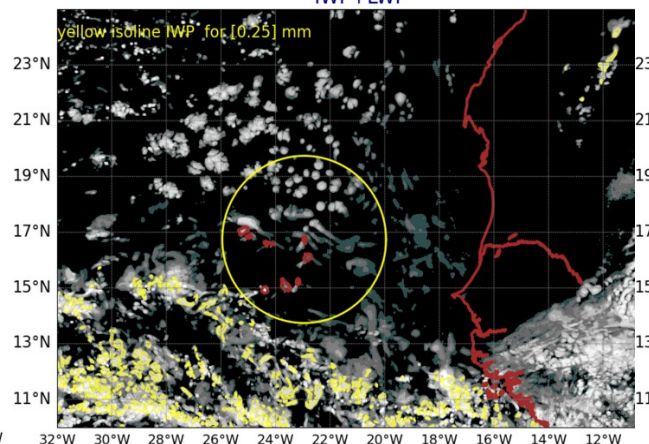
AROME25 20240908-12-UTC -ech(36h) IWP+LWP
