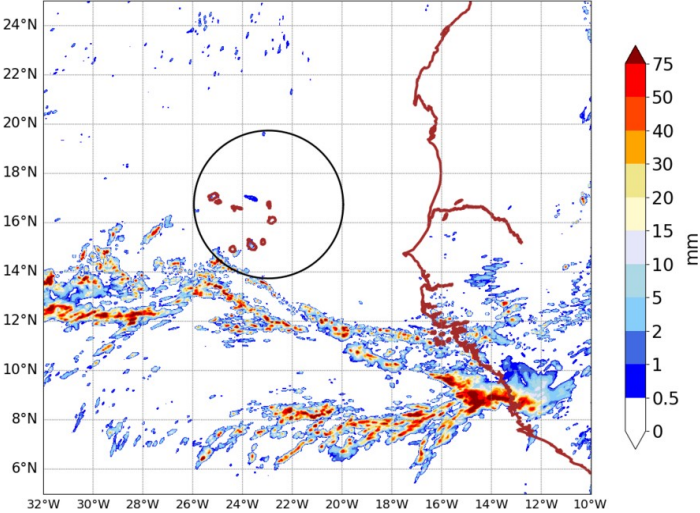
AROME25 20240907-15-UTC -ech(15h) RR cumulated over 6h
