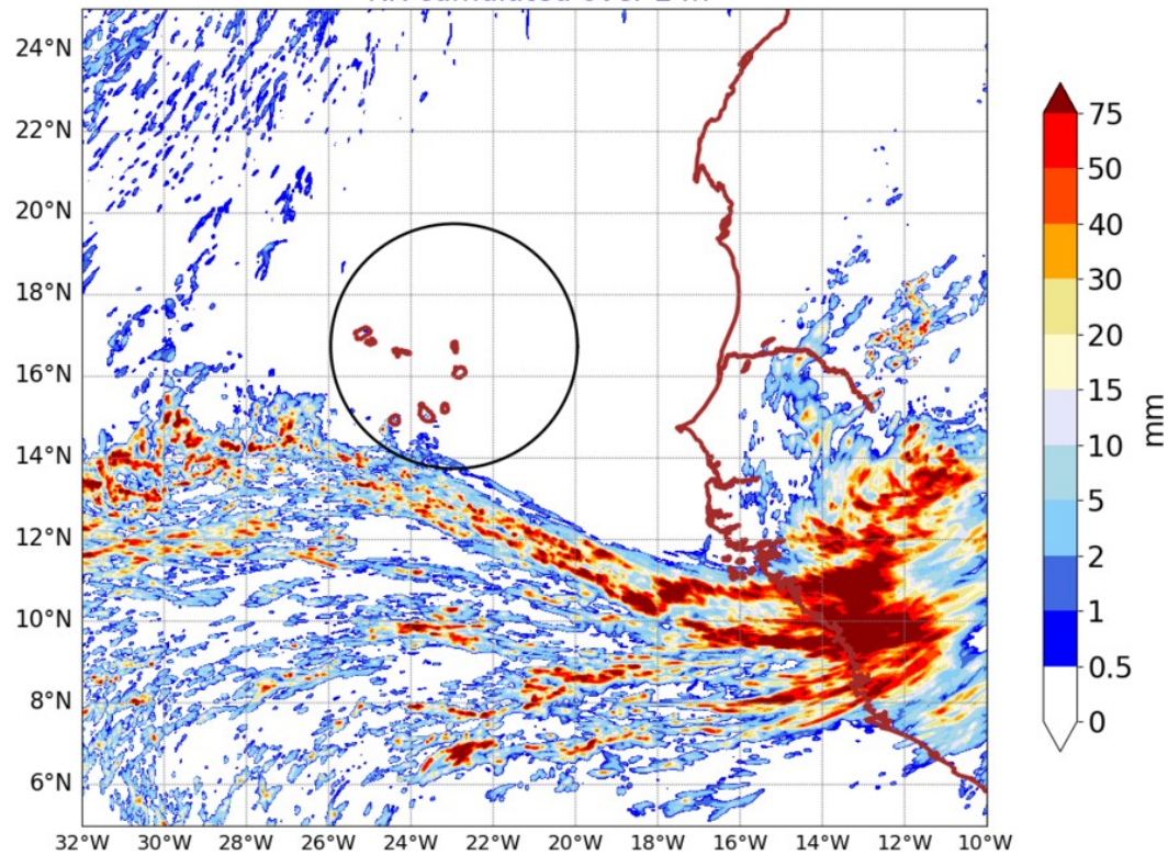
AROME25 20240907-00-UTC -ech(24h)
