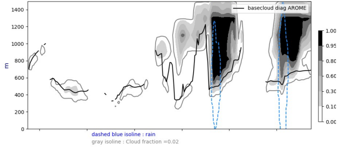
Cross section S/N @ -22W 20240907-12-UTC ech(12h)
