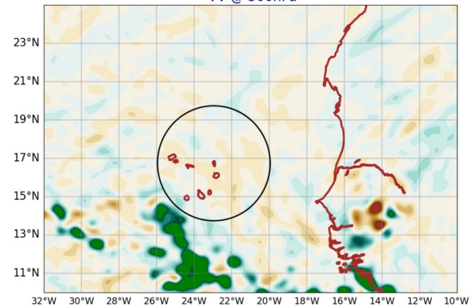
AROME25 20240908-12-UTC -ech(12h) VV @ 500hPa
