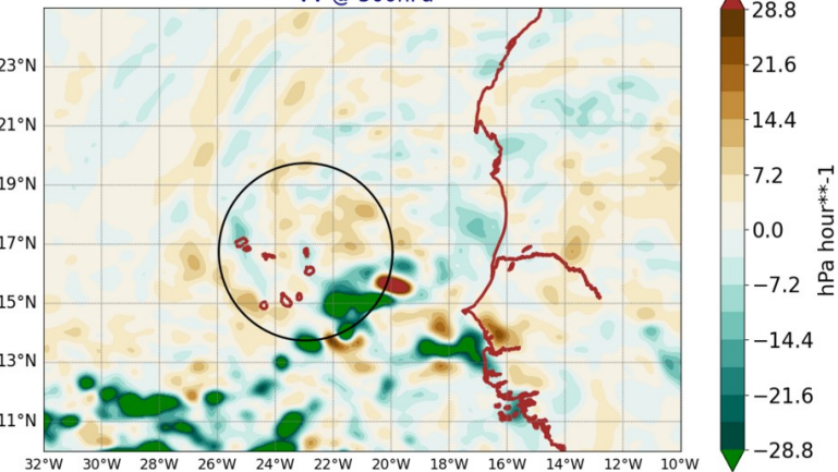
AROME25 20240910-12-UTC -ech(60h) VV @ 500hPa
