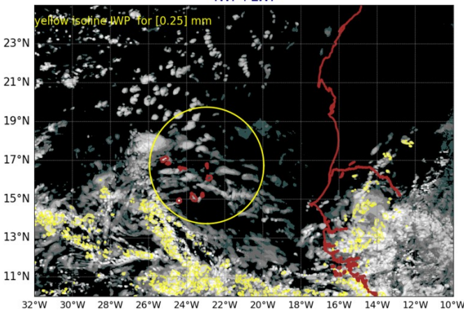
AROME25 20240908-12-UTC -ech(12h) IWP+LWP
