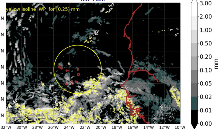
AROME25 20240910-12-UTC -ech(60h) IWP+LWP
