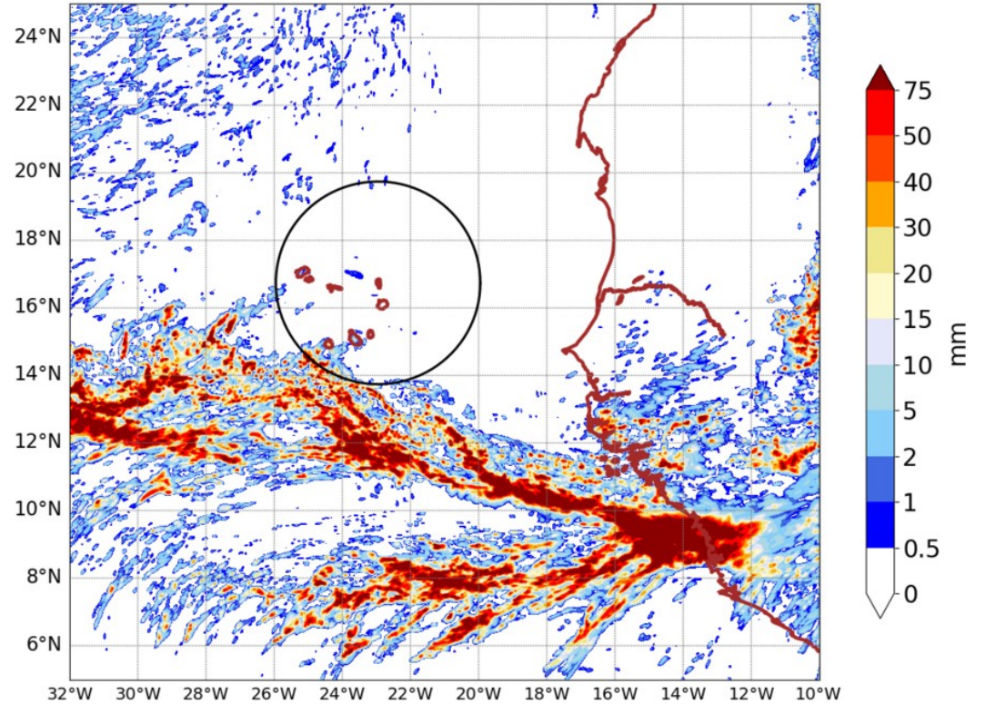
AROME25 20240908-00-UTC -ech(24h)
