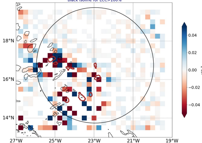
AROME25 regrid 0.25 20240909-12-UTC -ech(36h) blue for conv in subcloud layer black isoline for LCC>100%
