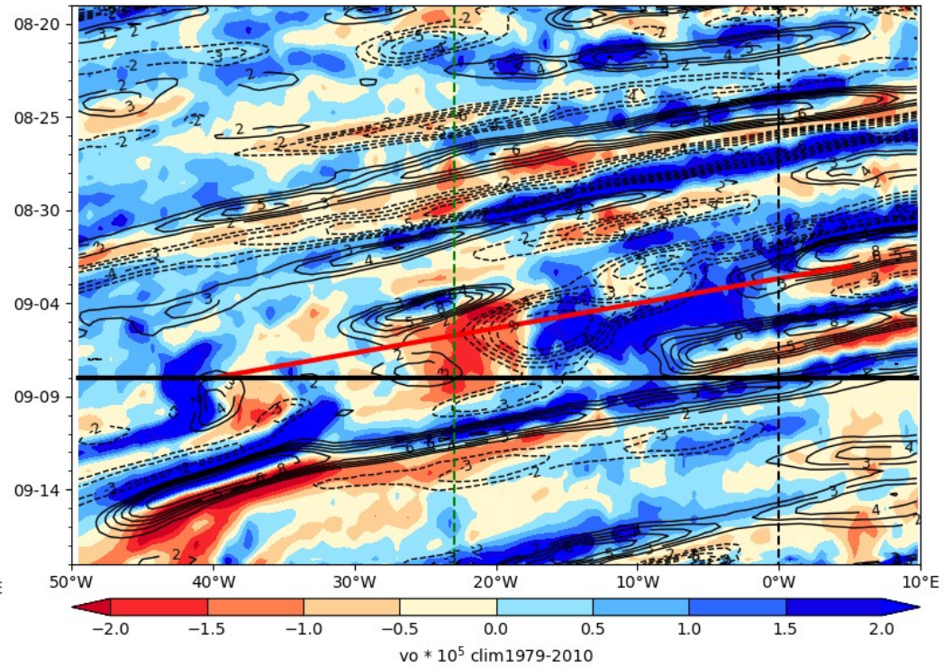
ECMWF Vorticity 850 hPa (color), V-700 hPa 2024-09-08
