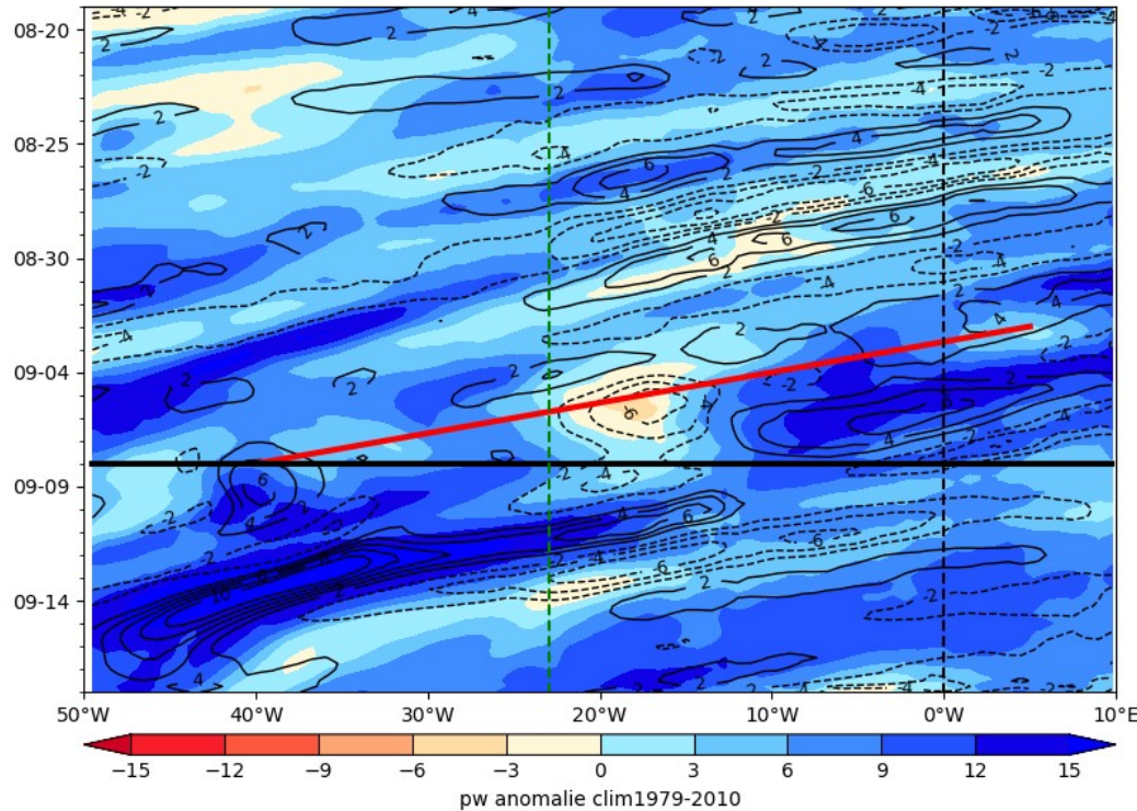
ECMWF PW (color) AND V at 925 hPa 2024-09-08
