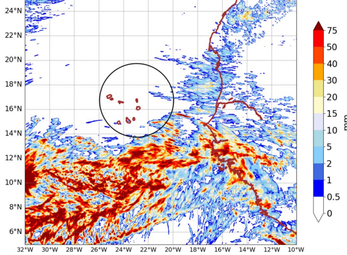
AROME25 20240910-12-UTC -ech(60h) RR cumulated over 24h
