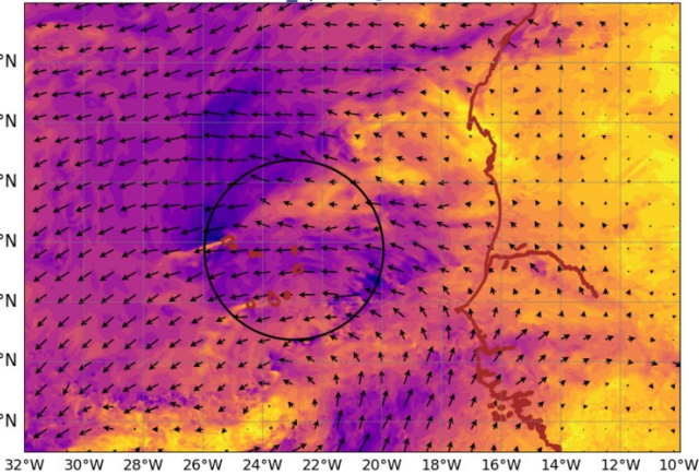
AROME25 20240910-12-UTC -ech(60h) wind_sp920 @ 920hPa
