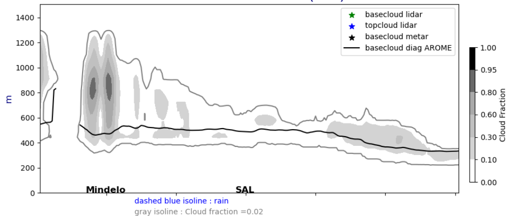
Cross section E/W @ 17.5N 20240909-12-UTC ech(36h)
