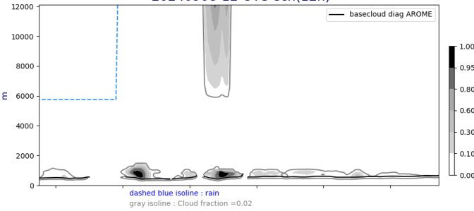
Cross section S/N @ -22W 20240908-12-UTC ech(12h)
