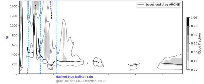
Cross section S/N @ -22W 20240910-12-UTC ech(60h)
