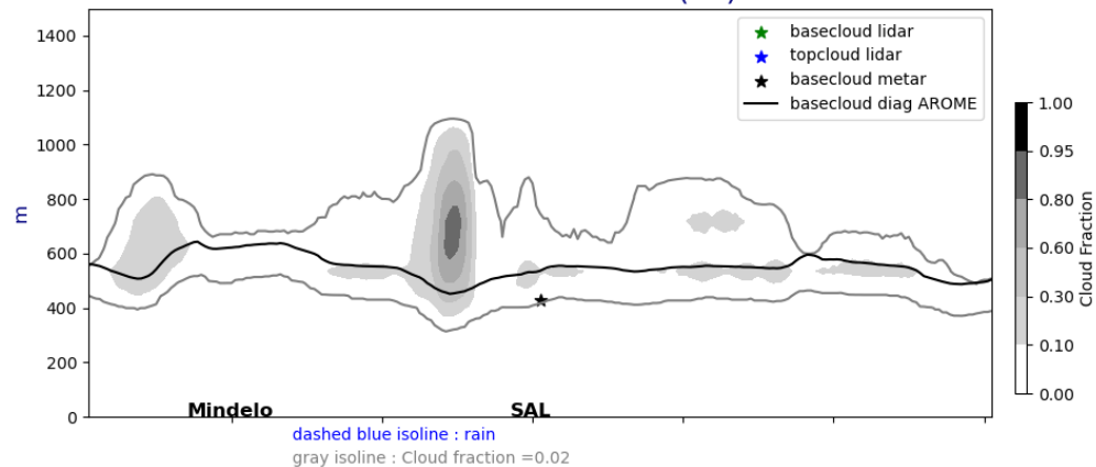
Cross section E/W @ 17.5N 20240908-01-UTC ech(1h)
