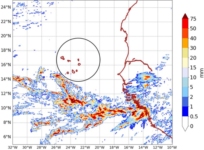
AROME25 20240908-15-UTC -ech(15h) RR cumulated over 6h
