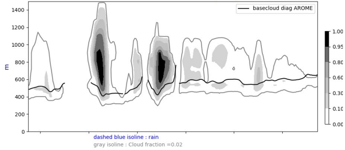
Cross section S/N @ -22W 20240908-12-UTC ech(12h)
