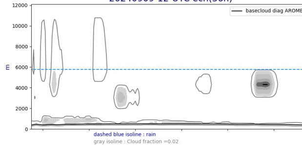
Cross section S/N @ -22W 20240909-12-UTC ech(36h)
