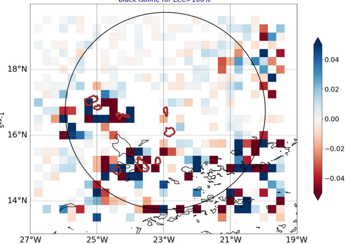
AROME25 regrid 0.25 20240910-12-UTC -ech(60h) blue for conv in subcloud layer black isoline for LCC>100%
