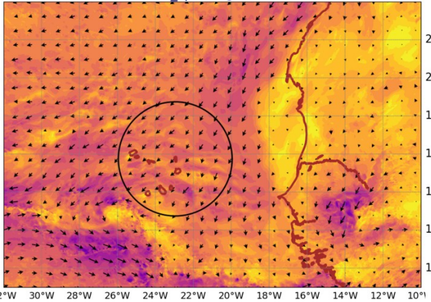
AROME25 20240908-12-UTC -ech(12h) wind_sp920 @ 920hPa
