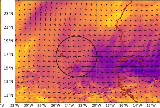
AROME25 20240909-12-UTC -ech(36h) wind_sp920 @ 920hPa
