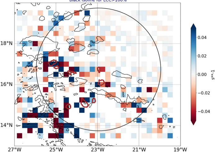
AROME25 regrid 0.25 20240908-12-UTC -ech(12h) blue for conv in subcloud layer black isoline for LCC>100%
