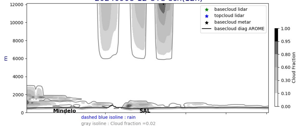
Cross section E/W @ 17.5N 20240908-12-UTC ech(12h)
