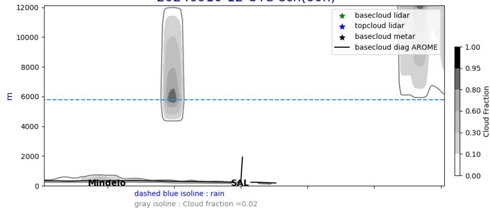
Cross section E/W @ 17.5N 20240910-12-UTC ech(60h)
