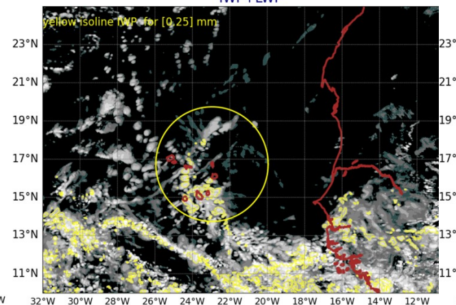
AROME25 20240909-12-UTC -ech(36h) IWP+LWP
