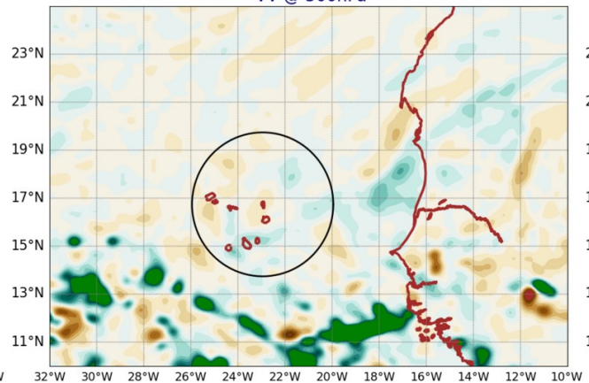
AROME25 20240909-12-UTC -ech(36h) VV @ 500hPa
