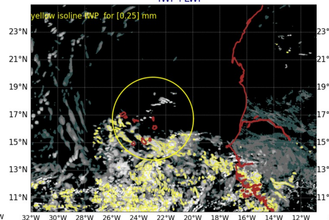
AROME25 20240910-12-UTC -ech(36h) IWP+LWP
