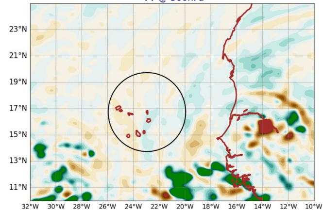
AROME25 20240909-12-UTC -ech(12h) VV @ 500hPa
