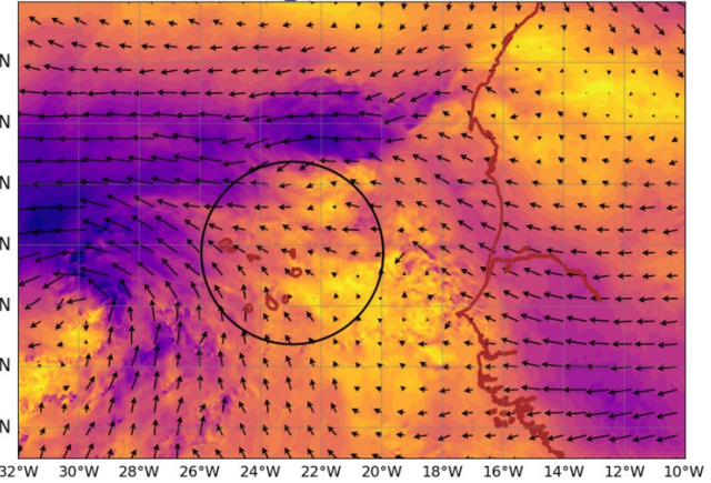
AROME25 20240911-12-UTC -ech(60h) wind_sp920 @ 920hPa
