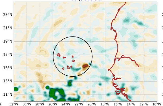
AROME25 20240910-12-UTC -ech(36h) VV @ 500hPa
