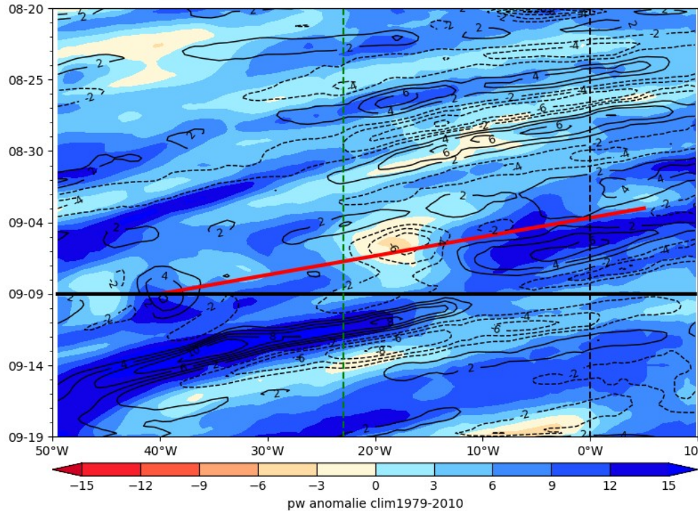
ECMWF PW (color) AND V at 925 hPa 2024-09-09
