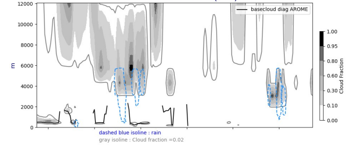
Cross section S/N @ -22W 20240911-12-UTC ech(60h)
