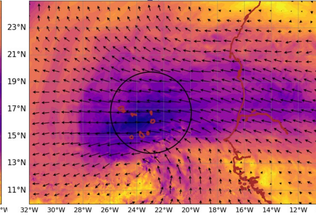
AROME25 20240910-12-UTC -ech(36h) wind_sp920 @ 920hPa
