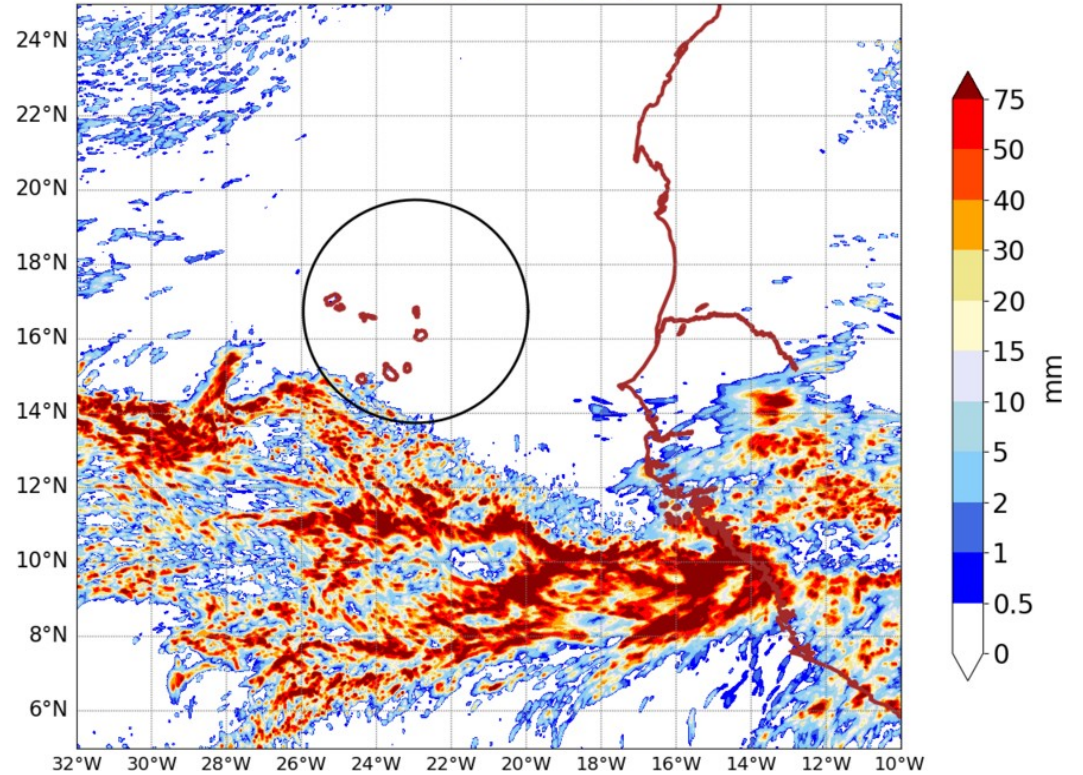
AROME25 20240909-00-UTC -ech(24h)
