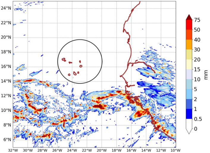
AROME25 20240909-15-UTC -ech(15h) RR cumulated over 6h
