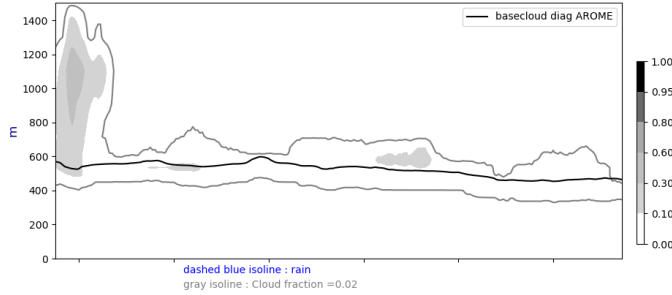
Cross section S/N @ -22W 20240909-12-UTC ech(12h)
