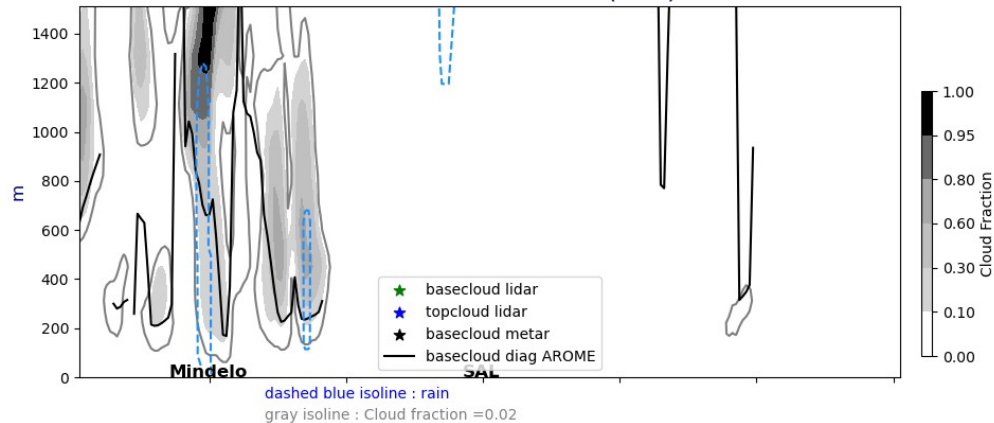
Cross section E/W @ 17.5N 20240911-12-UTC ech(60h)
