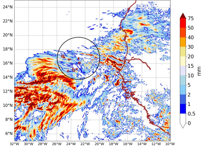
AROME25 20240911-12-UTC -ech(60h) RR cumulated over 24h
