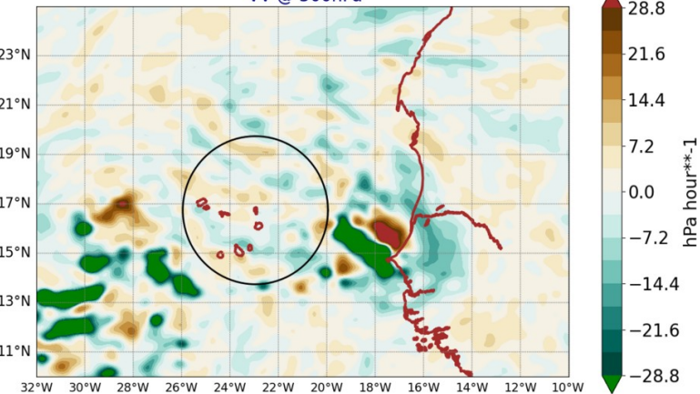
AROME25 20240911-12-UTC -ech(60h) VV @ 500hPa
