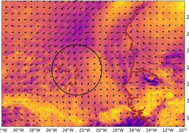
AROME25 20240909-12-UTC -ech(12h) wind_sp920 @ 920hPa
