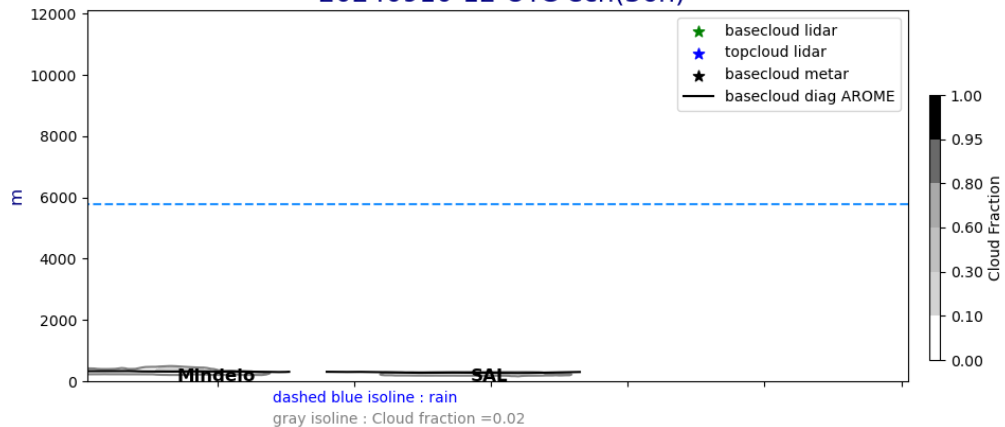
Cross section E/W @ 17.5N 20240910-12-UTC ech(36h)
