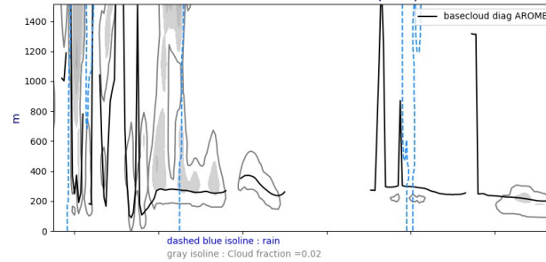
Cross section S/N @ -22W 20240910-12-UTC ech(36h)
