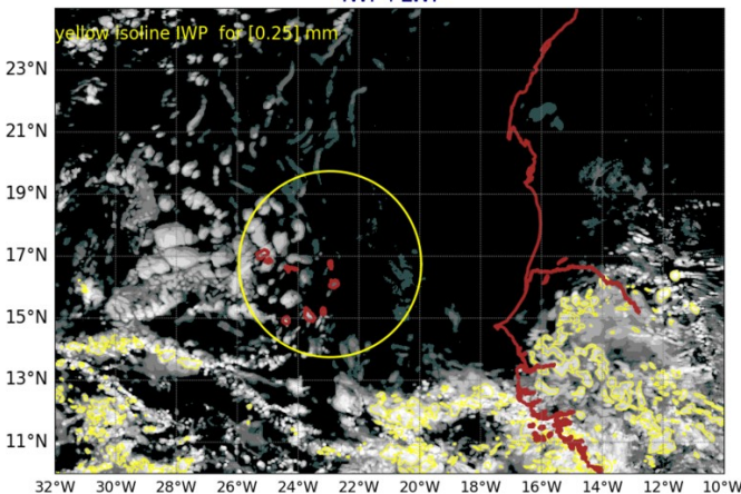
AROME25 20240909-12-UTC -ech(12h) IWP+LWP
