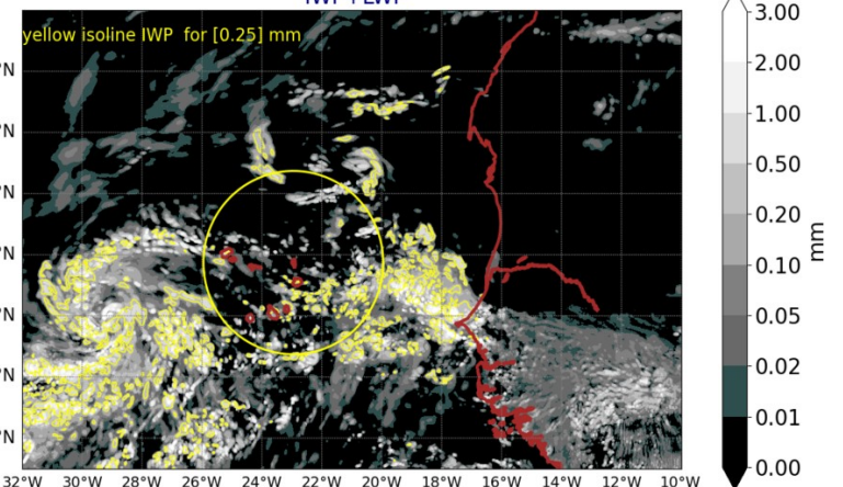
AROME25 20240911-12-UTC -ech(60h) IWP+LWP
