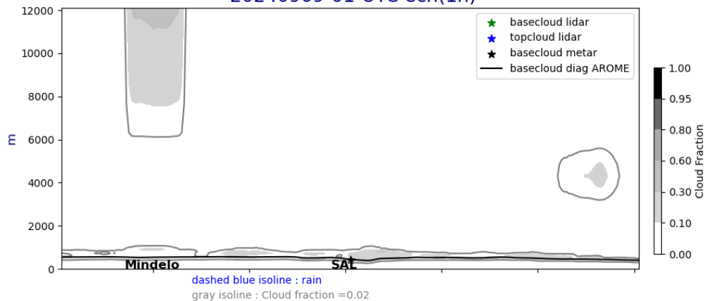
Cross section E/W @ 17.5N 20240909-01-UTC ech(1h)
