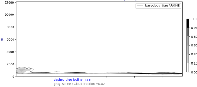
Cross section S/N @ -22W 20240909-12-UTC ech(12h)
