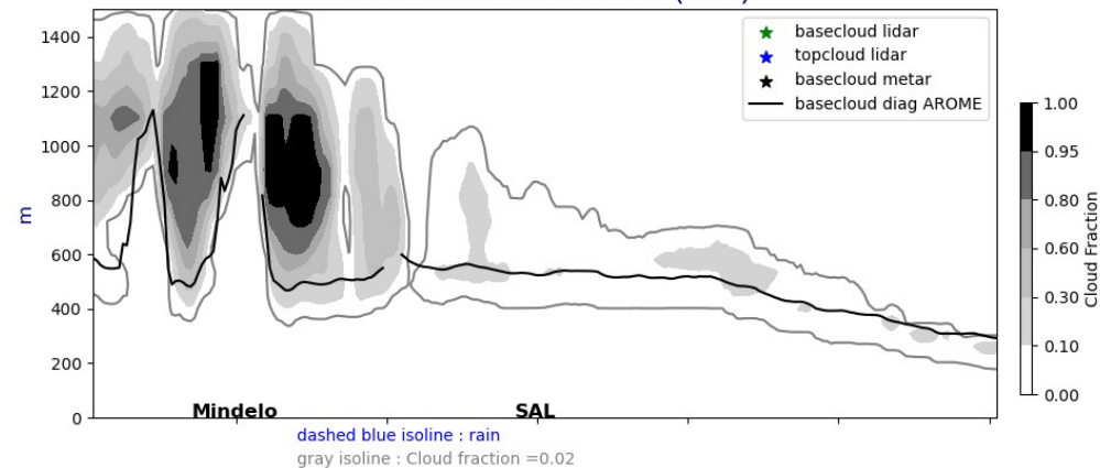
Cross section E/W @ 17.5N 20240909-12-UTC ech(12h)
