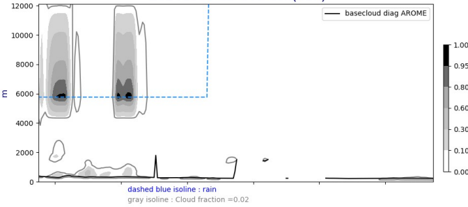
Cross section S/N @ -22W 20240910-12-UTC ech(12h)
