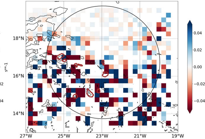
AROME25 regrid 0.25 20240911-12-UTC -ech(36h) blue for conv in subcloud layer black isoline for LCC>100%
