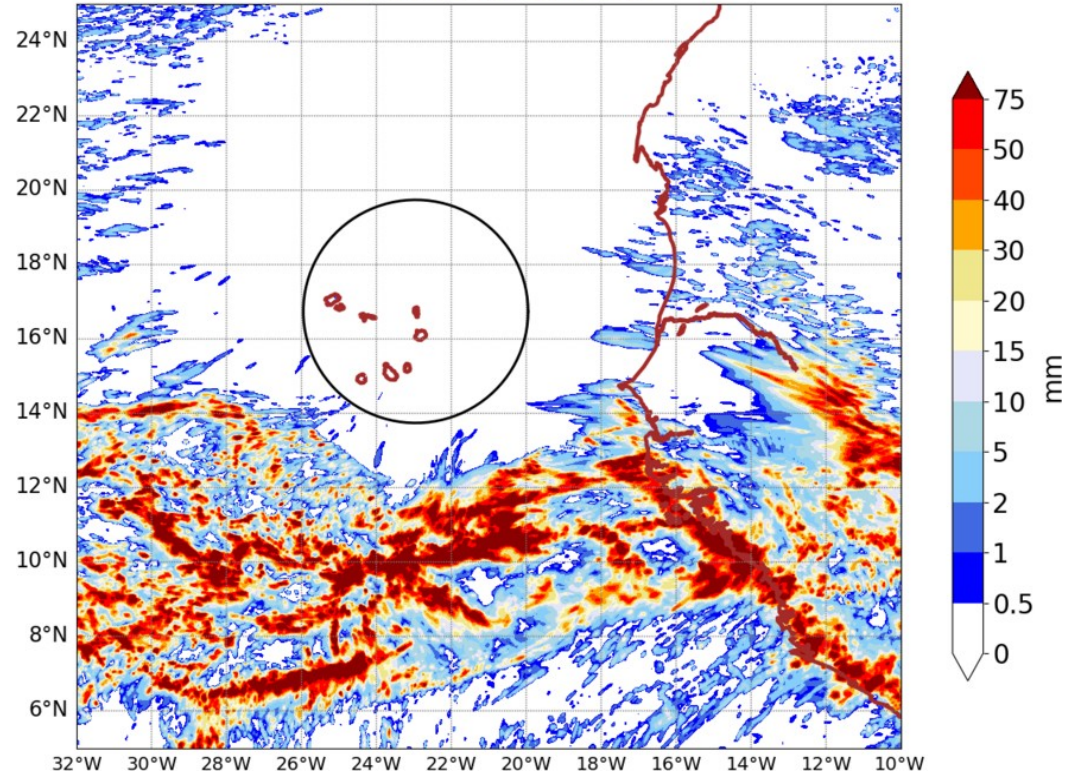
AROME25 20240910-00-UTC -ech(24h)
