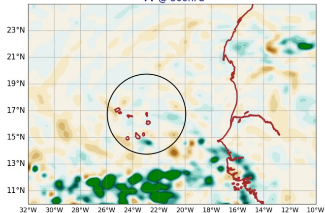
AROME25 20240910-12-UTC -ech(12h) VV @ 500hPa
