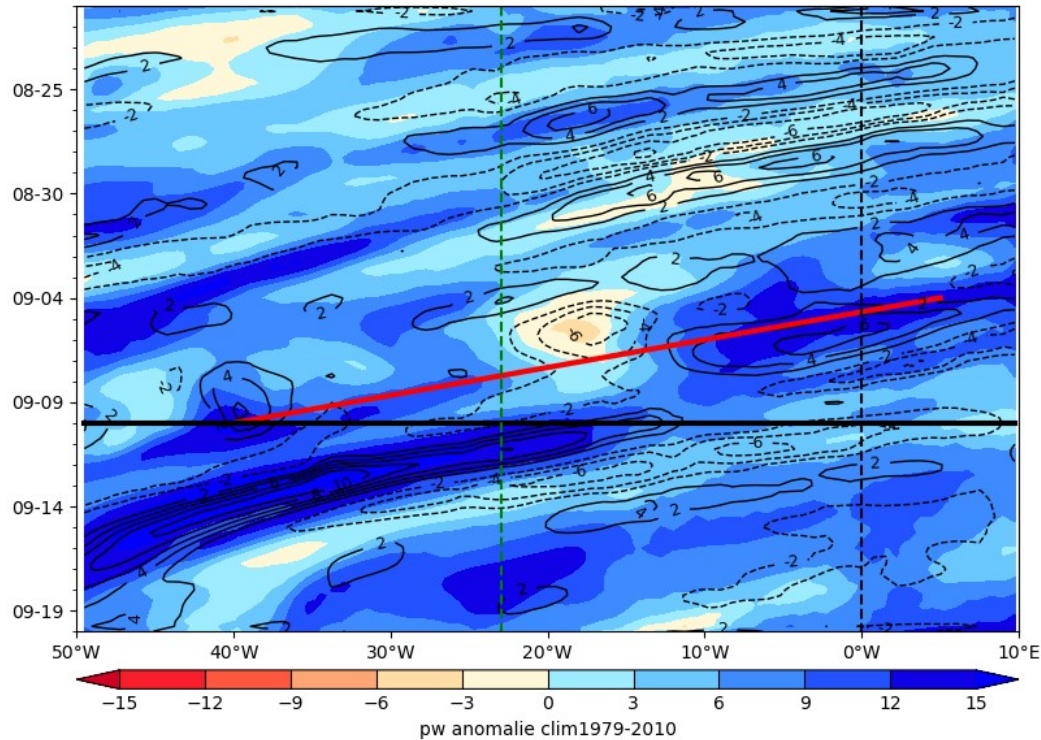
ECMWF PW (color) AND V at 925 hPa 2024-09-10
