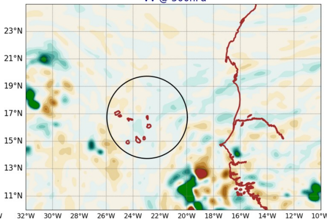
AROME25 20240912-12-UTC -ech(60h) VV @ 500hPa
