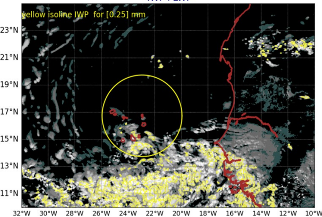
AROME25 20240910-12-UTC -ech(12h) IWP+LWP
