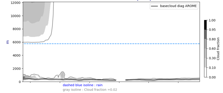
Cross section S/N @ -22W 20240912-12-UTC ech(60h)
