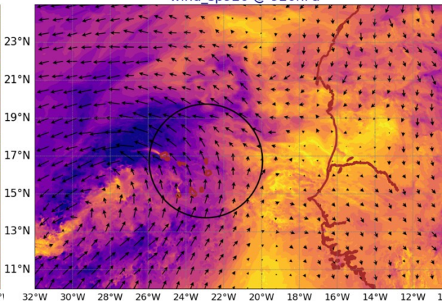
AROME25 20240911-12-UTC -ech(36h) wind_sp920 @ 920hPa
