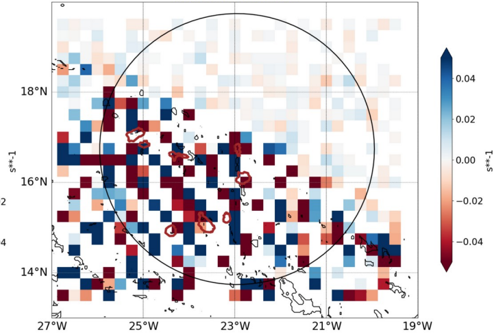
AROME25 regrid 0.25 20240912-12-UTC -ech(60h) blue for conv in subcloud layer black isoline for LCC>100%
