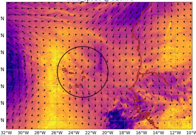
AROME25 20240912-12-UTC -ech(60h) wind_sp920 @ 920hPa
