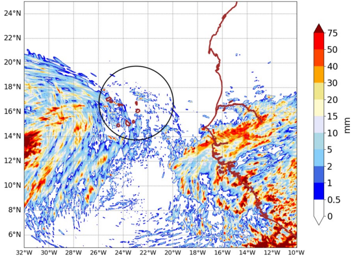
AROME25 20240912-12-UTC -ech(60h) RR cumulated over 24h
