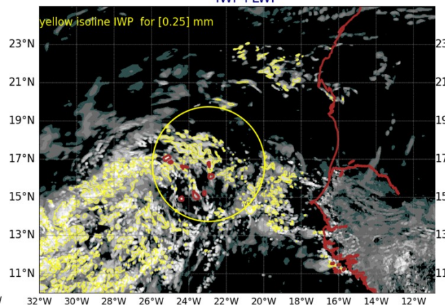
AROME25 20240911-12-UTC -ech(36h) IWP+LWP
