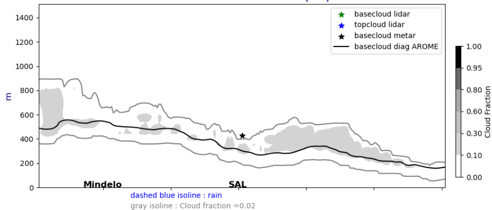
Cross section E/W @ 17.5N 20240910-01-UTC ech(1h)
