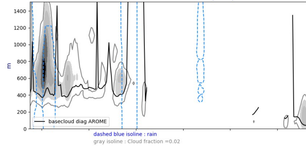
Cross section S/N @ -22W 20240911-12-UTC ech(36h)
