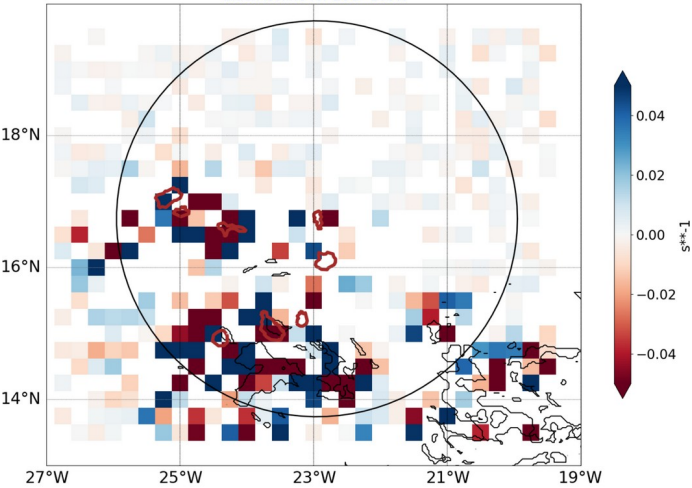
AROME25 regrid 0.25 20240910-12-UTC -ech(12h) blue for conv in subcloud layer black isoline for LCC>100%
