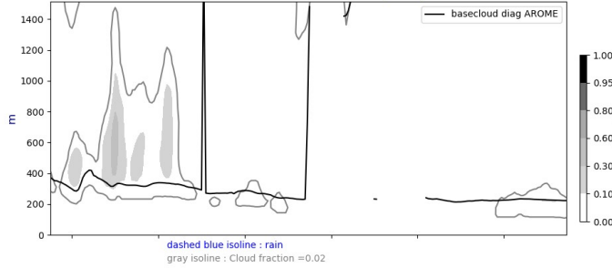
Cross section S/N @ -22W 20240910-12-UTC ech(12h)
