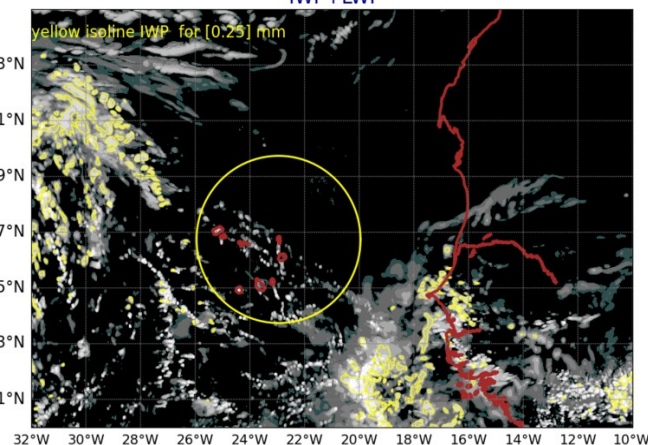
AROME25 20240912-12-UTC -ech(60h) IWP+LWP
