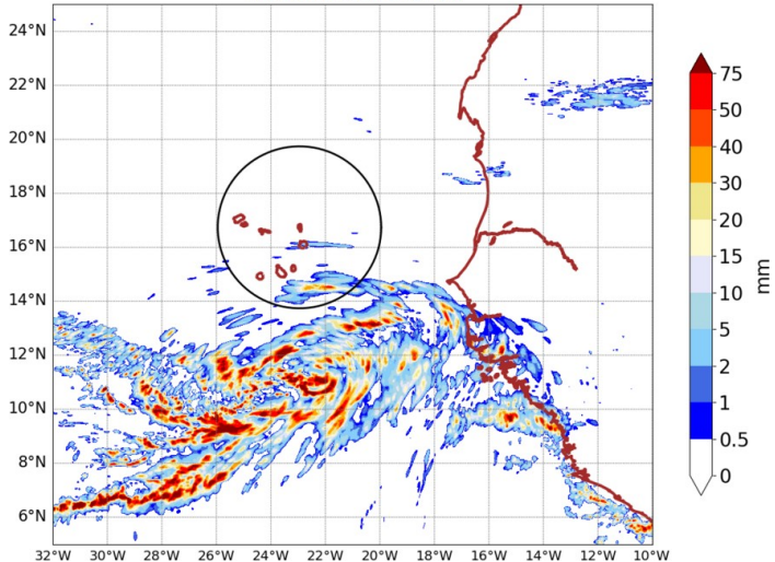
AROME25 20240910-15-UTC -ech(15h) RR cumulated over 6h
