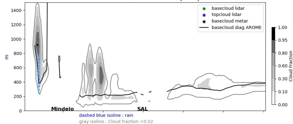
Cross section E/W @ 17.5N 20240912-12-UTC ech(60h)
