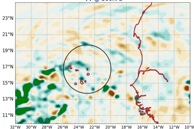
AROME25 20240911-12-UTC -ech(36h) VV @ 500hPa
