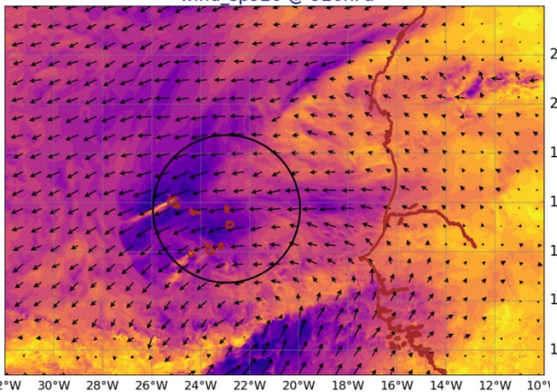
AROME25 20240910-12-UTC -ech(12h) wind_sp920 @ 920hPa
