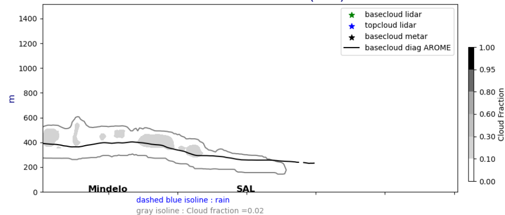
Cross section E/W @ 17.5N 20240910-12-UTC ech(12h)
