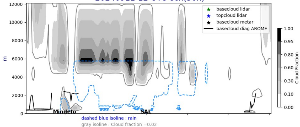
Cross section E/W @ 17.5N 20240911-12-UTC ech(36h)
