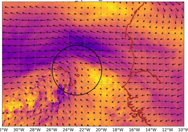
AROME25 20240911-12-UTC -ech(12h) wind_sp920 @ 920hPa
