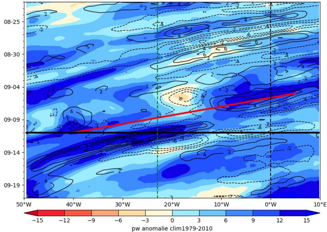
ECMWF PW (color) AND V at 925 hPa 2024-09-11
