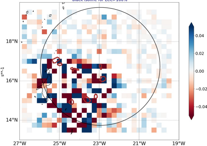
AROME25 regrid 0.25 20240913-12-UTC -ech(60h) blue for conv in subcloud layer black isoline for LCC>100%
