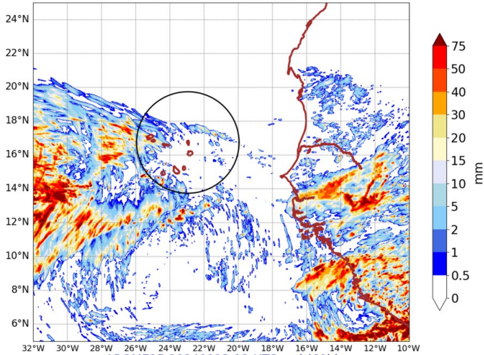
AROME25 20240913-12-UTC -ech(60h) RR cumulated over 24h
