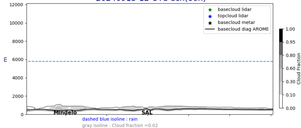
Cross section E/W @ 17.5N 20240913-12-UTC ech(60h)
