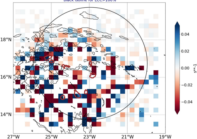
AROME25 regrid 0.25 20240911-12-UTC -ech(12h) blue for conv in subcloud layer black isoline for LCC>100%
