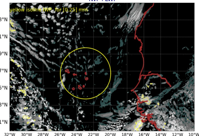
AROME25 20240913-12-UTC -ech(60h) IWP+LWP
