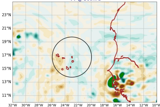
AROME25 20240912-12-UTC -ech(36h) VV @ 500hPa
