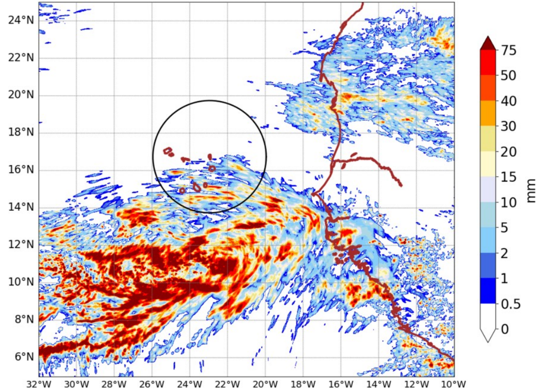
AROME25 20240911-00-UTC -ech(24h)
