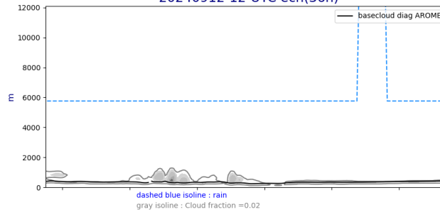
Cross section S/N @ -22W 20240912-12-UTC ech(36h)
