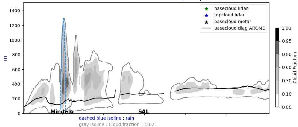
Cross section E/W @ 17.5N 20240912-12-UTC ech(36h)
