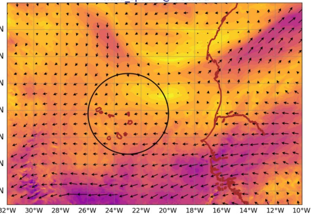
AROME25 20240913-12-UTC -ech(60h) wind_sp920 @ 920hPa
