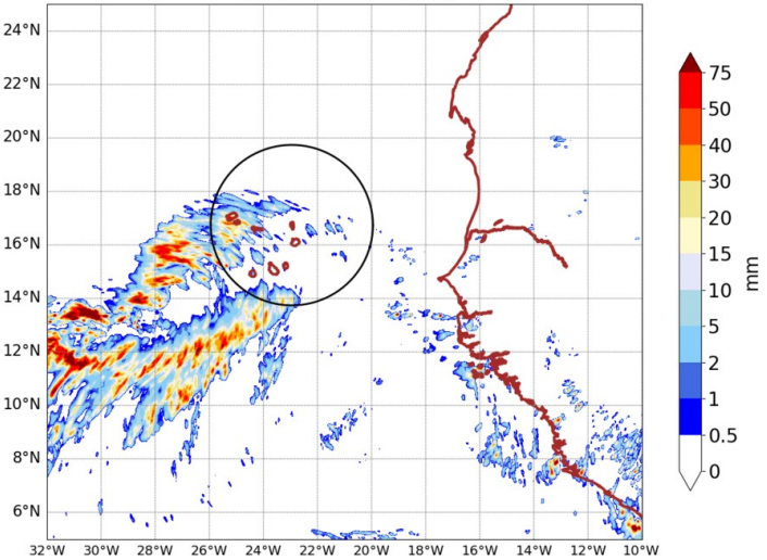
AROME25 20240911-15-UTC -ech(15h) RR cumulated over 6h
