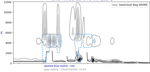
Cross section S/N @ -22W 20240911-12-UTC ech(12h)
