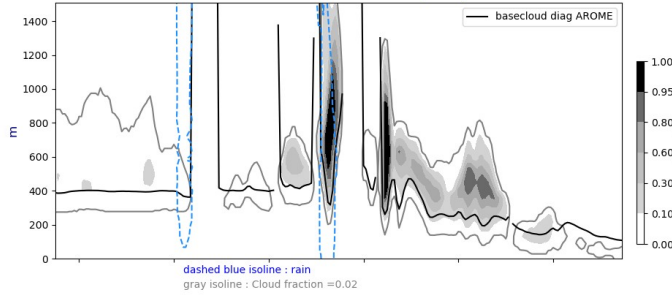
Cross section S/N @ -22W 20240911-12-UTC ech(12h)
