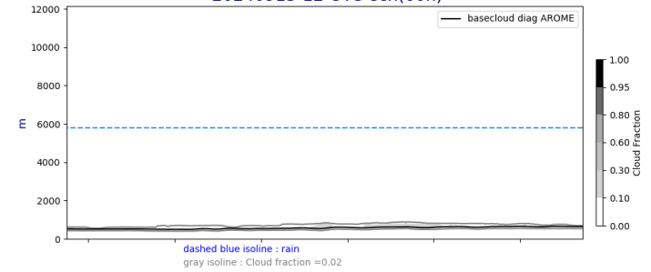
Cross section S/N @ -22W 20240913-12-UTC ech(60h)
