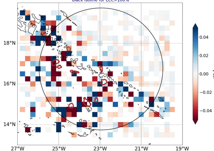
AROME25 regrid 0.25 20240912-12-UTC -ech(36h) blue for conv in subcloud layer black isoline for LCC>100%
