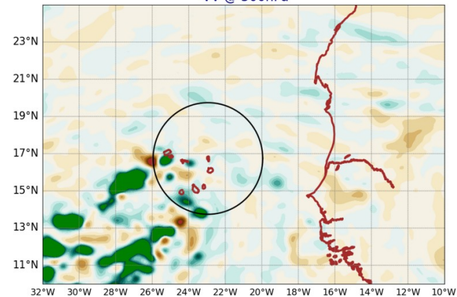
AROME25 20240911-12-UTC -ech(12h) VV @ 500hPa
