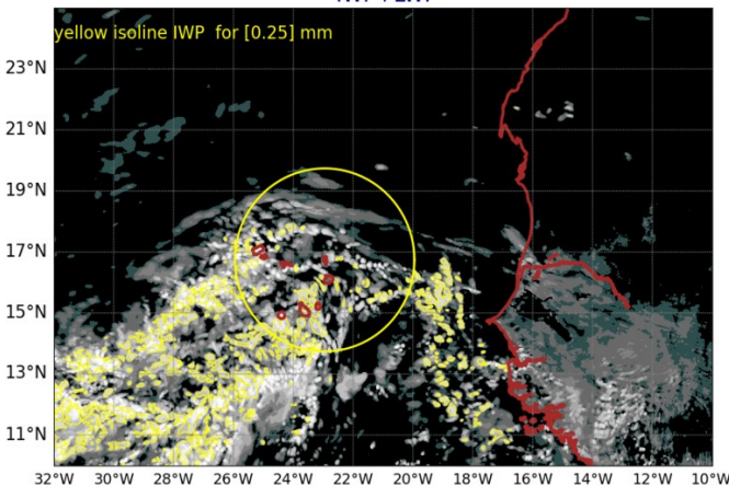
AROME25 20240911-12-UTC -ech(12h) IWP+LWP
