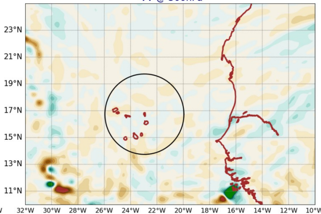
AROME25 20240913-12-UTC -ech(60h) VV @ 500hPa
