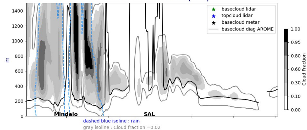
Cross section E/W @ 17.5N 20240911-12-UTC ech(12h)
