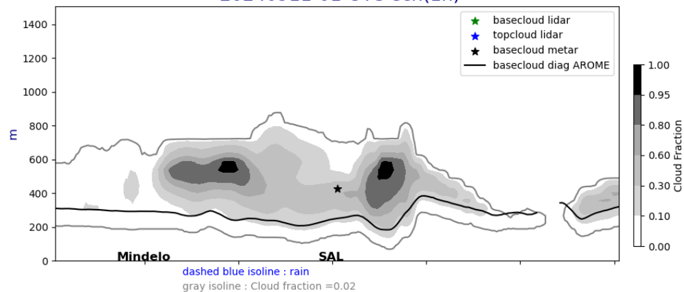
Cross section E/W @ 17.5N 20240911-01-UTC ech(1h)
