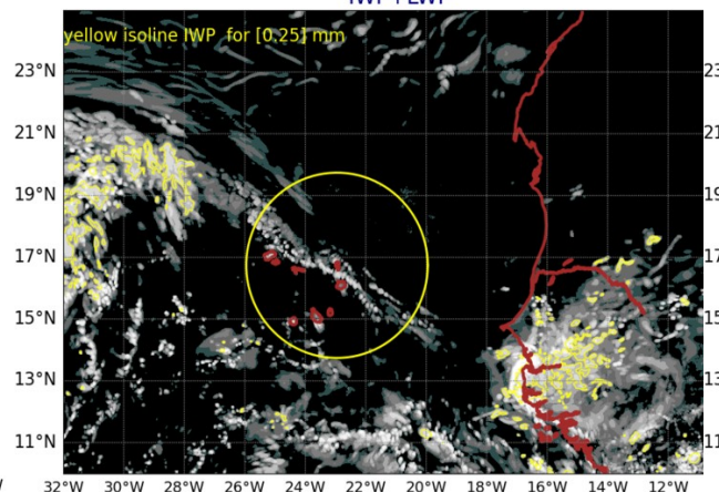
AROME25 20240912-12-UTC -ech(36h) IWP+LWP
