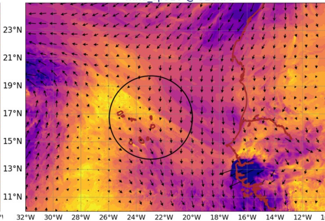
AROME25 20240912-12-UTC -ech(36h) wind_sp920 @ 920hPa
