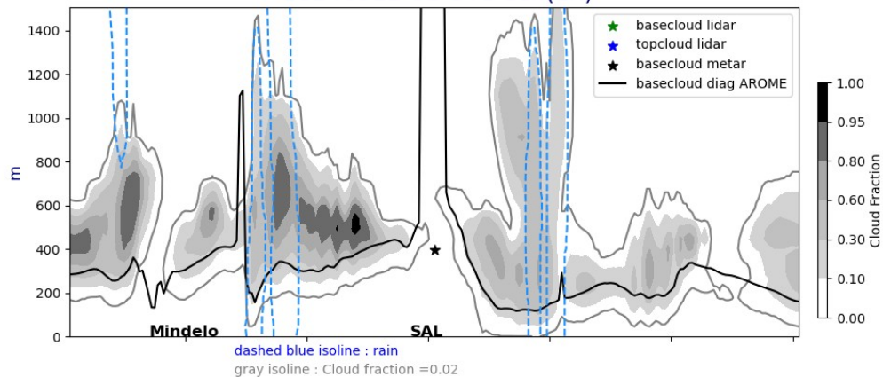
Cross section E/W @ 17.5N 20240912-01-UTC ech(1h)
