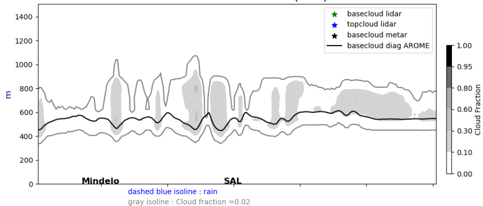
Cross section E/W @ 17.5N 20240913-12-UTC ech(36h)
