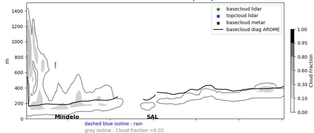
Cross section E/W @ 17.5N 20240912-12-UTC ech(12h)
