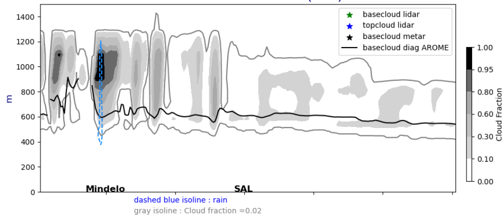
Cross section E/W @ 17.5N 20240914-12-UTC ech(60h)
