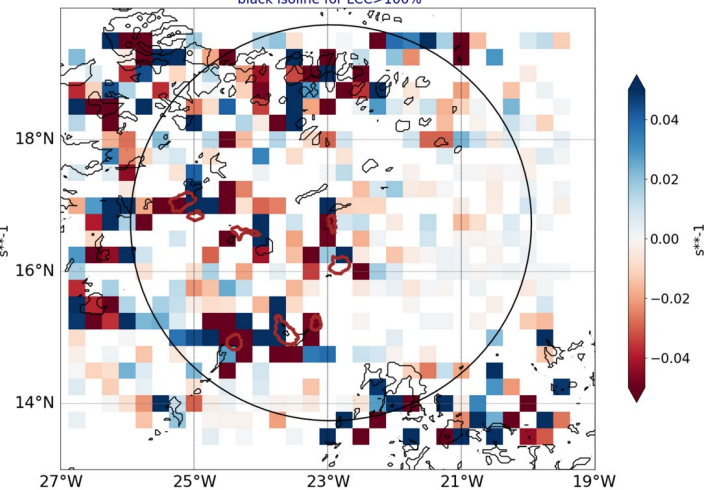
AROME25 regrid 0.25 20240915-12-UTC -ech(60h) blue for conv in subcloud layer black isoline for LCC>100%
