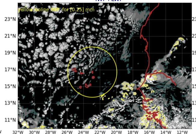
AROME25 20240914-12-UTC -ech(36h) IWP+LWP
