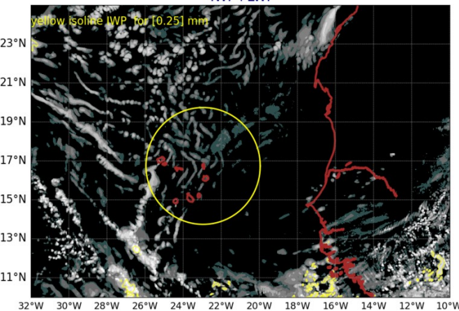
AROME25 20240913-12-UTC -ech(12h) IWP+LWP
