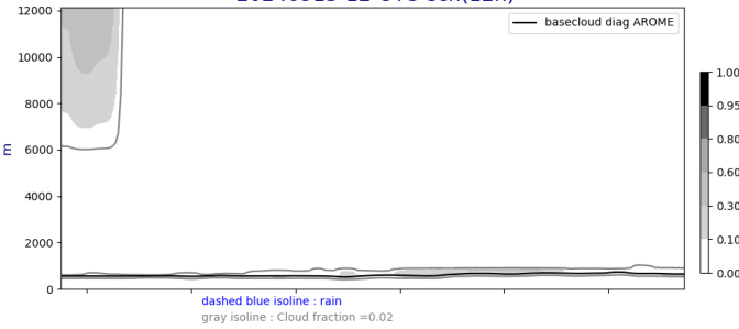
Cross section S/N @ -22W 20240913-12-UTC ech(12h)
