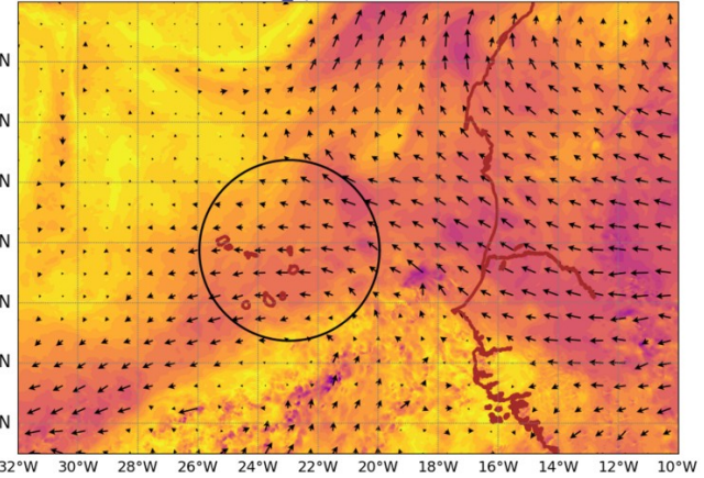
AROME25 20240915-12-UTC -ech(60h) wind_sp920 @ 920hPa
