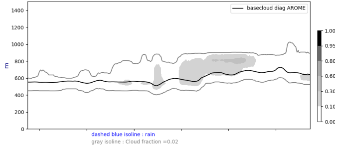
Cross section S/N @ -22W 20240913-12-UTC ech(12h)
