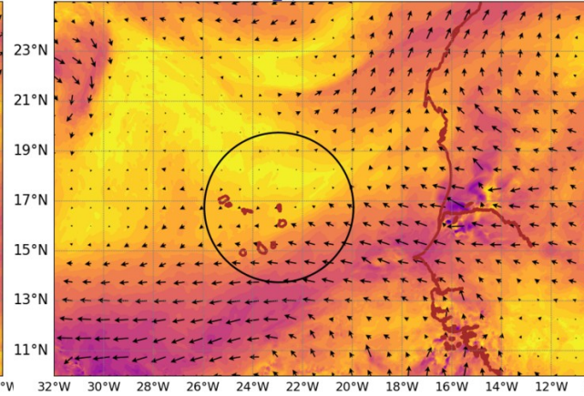
AROME25 20240914-12-UTC -ech(36h) wind_sp920 @ 920hPa
