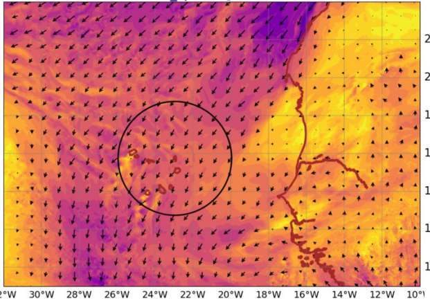
AROME25 20240913-12-UTC -ech(12h) wind_sp920 @ 920hPa
