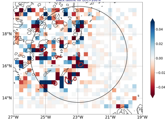
AROME25 regrid 0.25 20240914-12-UTC -ech(36h) blue for conv in subcloud layer black isoline for LCC>100%
