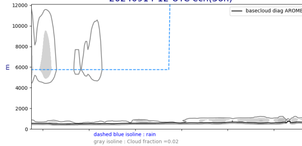
Cross section S/N @ -22W 20240914-12-UTC ech(36h)
