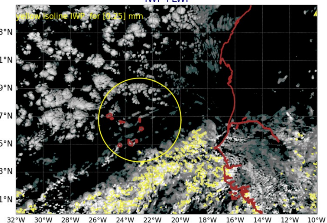
AROME25 20240915-12-UTC -ech(60h) IWP+LWP
