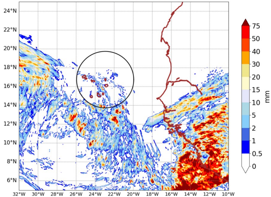
AROME25 20240913-00-UTC -ech(24h) RR cumulated over 24h
