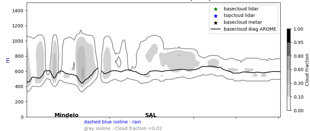
Cross section E/W @ 17.5N 20240913-12-UTC ech(12h)
