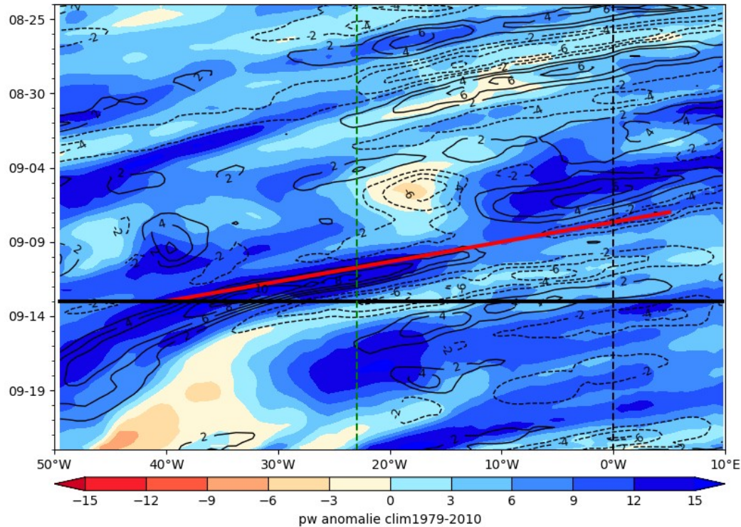
ECMWF PW (color) AND V at 925 hPa 2024-09-13
