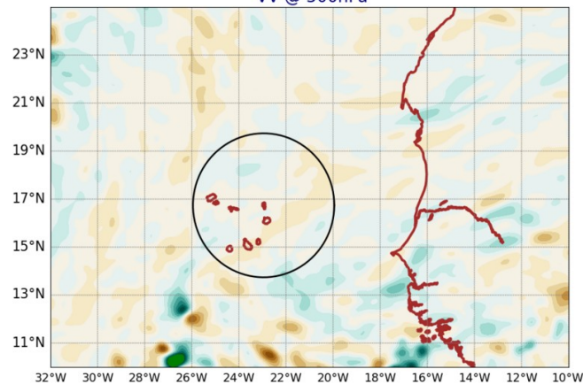
AROME25 20240913-12-UTC -ech(12h) VV @ 500hPa
