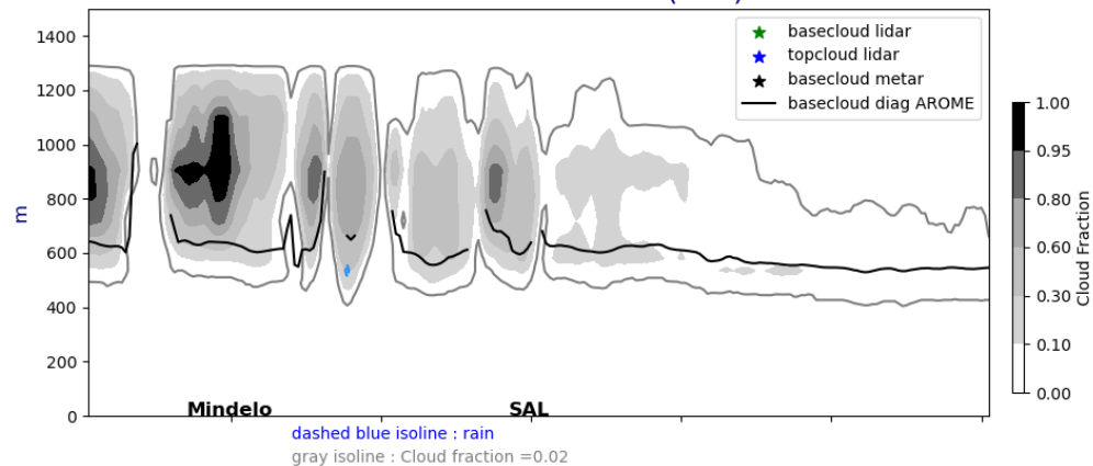
Cross section E/W @ 17.5N 20240914-12-UTC ech(36h)
