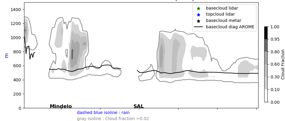
Cross section E/W @ 17.5N 20240915-12-UTC ech(60h)
