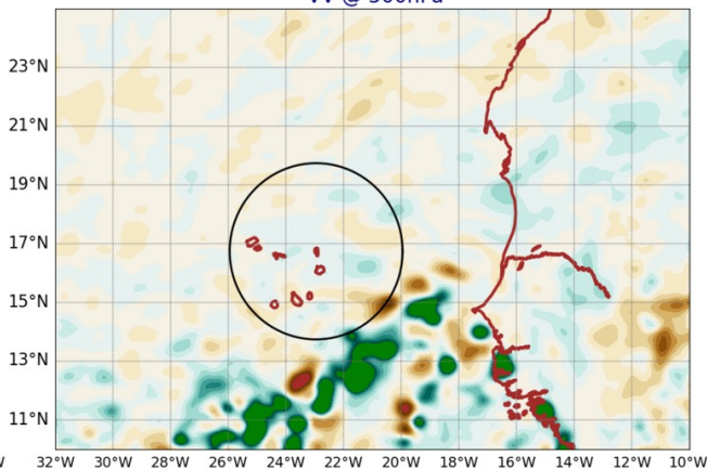
AROME25 20240915-12-UTC -ech(60h) VV @ 500hPa
