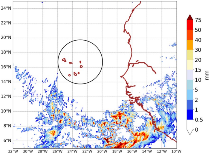
AROME25 20240913-15-UTC -ech(15h) RR cumulated over 6h
