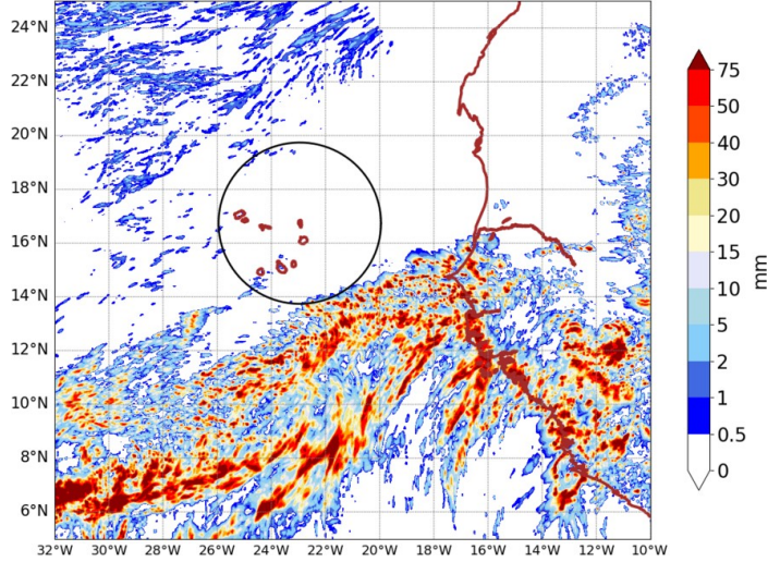
AROME25 20240915-12-UTC -ech(60h) RR cumulated over 24h
