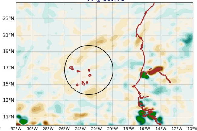
AROME25 20240914-12-UTC -ech(36h) VV @ 500hPa
