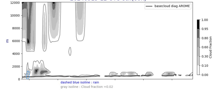
Cross section S/N @ -22W 20240915-12-UTC ech(60h)
