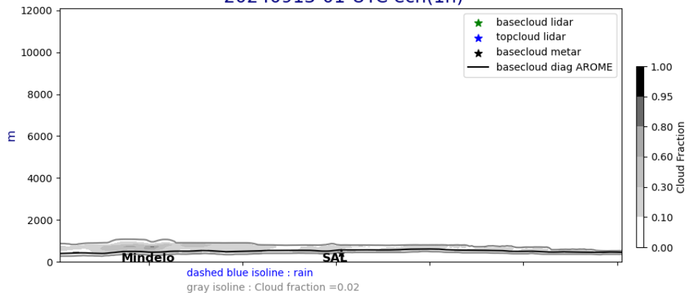
Cross section E/W @ 17.5N 20240913-01-UTC ech(1h)
