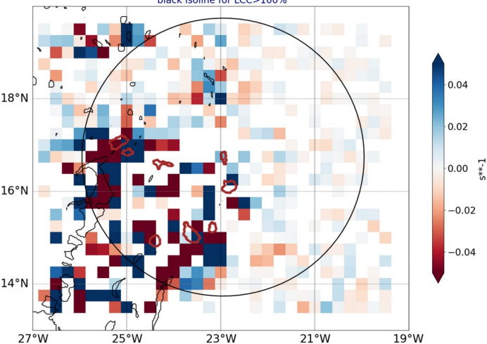
AROME25 regrid 0.25 20240913-12-UTC -ech(12h) blue for conv in subcloud layer black isoline for LCC>100%
