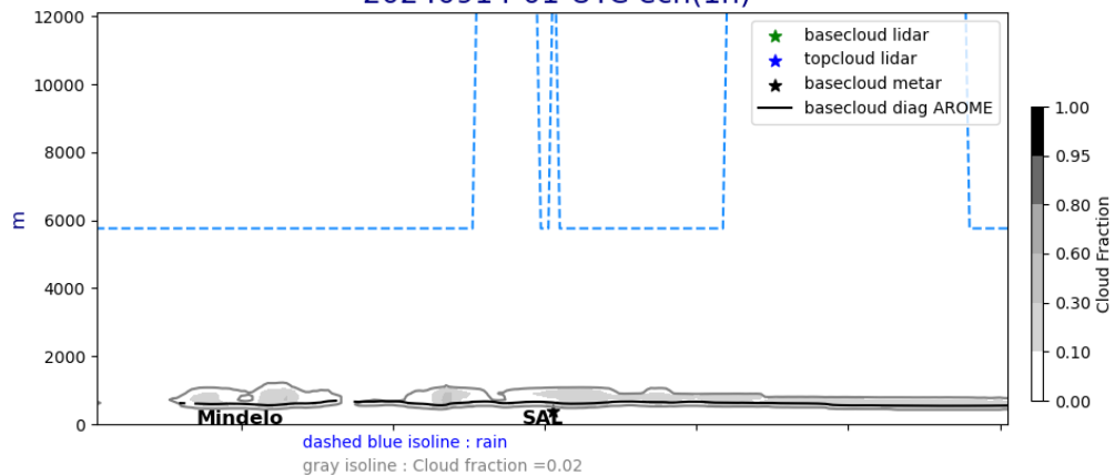
Cross section E/W @ 17.5N 20240914-01-UTC ech(1h)
