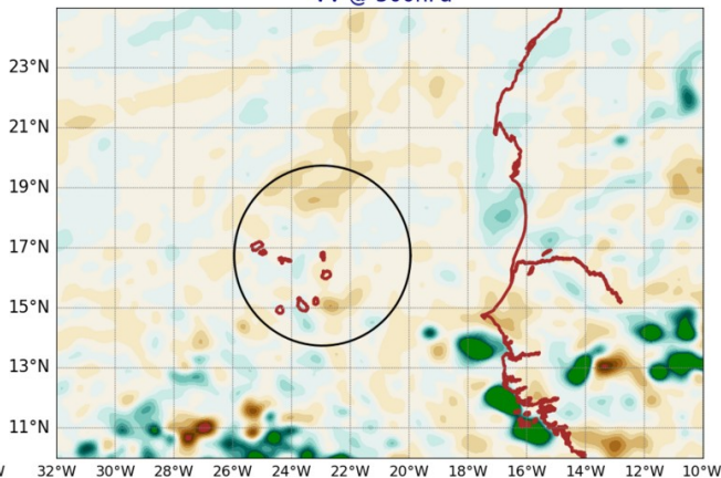
AROME25 20240916-12-UTC -ech(60h) VV @ 500hPa
