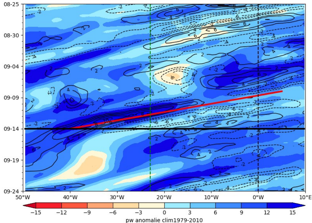
ECMWF PW (color) AND V at 925 hPa 2024-09-14
