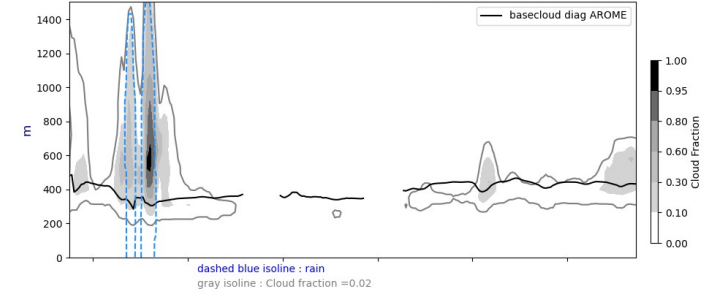
Cross section S/N @ -22W 20240916-12-UTC ech(60h)
