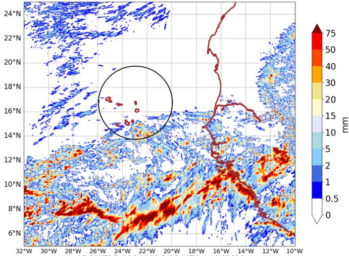
AROME25 20240916-12-UTC -ech(60h) RR cumulated over 24h
