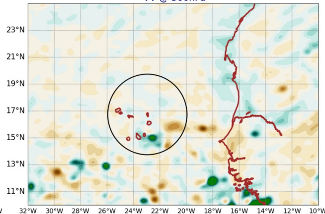
AROME25 20240915-12-UTC -ech(36h) VV @ 500hPa
