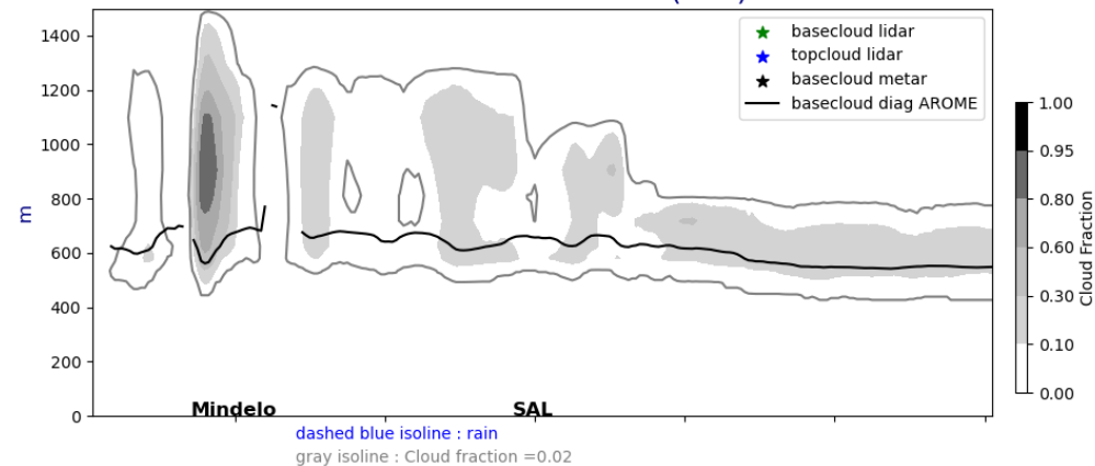
Cross section E/W @ 17.5N 20240914-12-UTC ech(12h)
