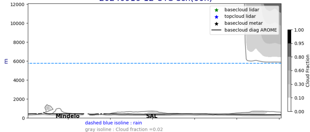
Cross section E/W @ 17.5N 20240916-12-UTC ech(60h)
