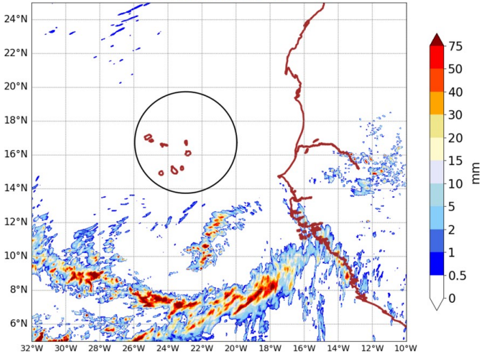
AROME25 20240914-15-UTC -ech(15h) RR cumulated over 6h
