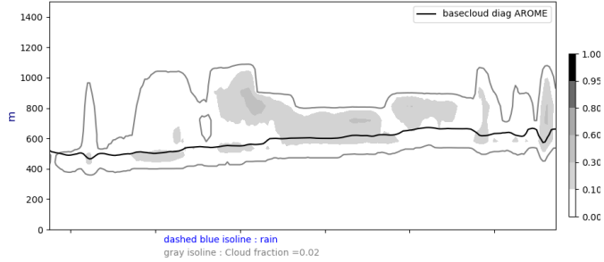
Cross section S/N @ -22W 20240914-12-UTC ech(12h)
