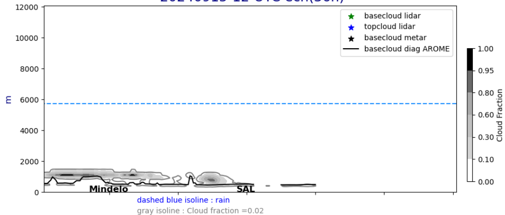
Cross section E/W @ 17.5N 20240915-12-UTC ech(36h)
