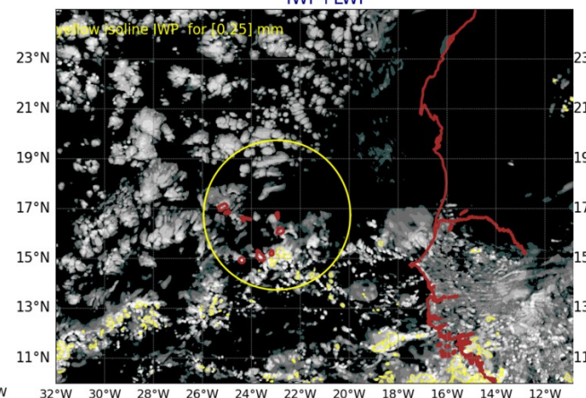
AROME25 20240915-12-UTC -ech(36h) IWP+LWP
