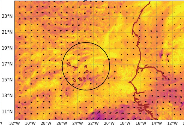
AROME25 20240915-12-UTC -ech(36h) wind_sp920 @ 920hPa
