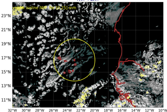
AROME25 20240914-12-UTC -ech(12h) IWP+LWP
