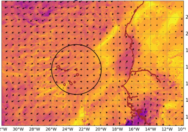
AROME25 20240914-12-UTC -ech(12h) wind_sp920 @ 920hPa
