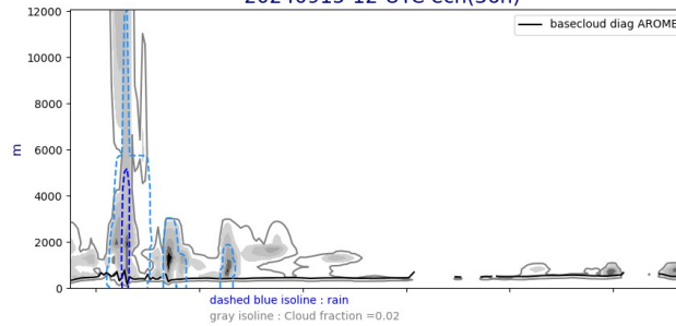
Cross section S/N @ -22W 20240915-12-UTC ech(36h)
