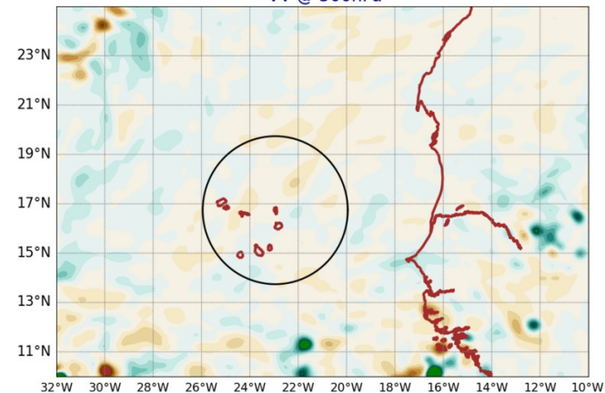
AROME25 20240914-12-UTC -ech(12h) VV @ 500hPa
