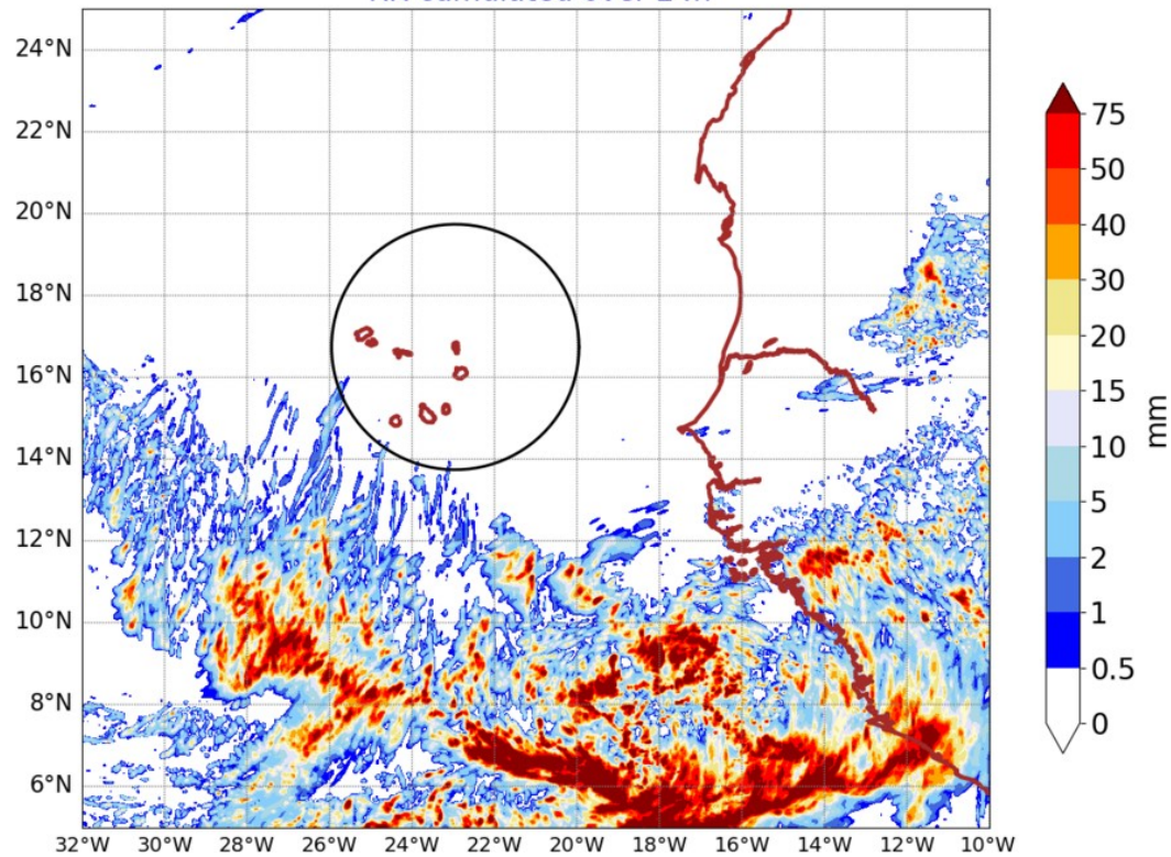
AROME25 20240914-00-UTC -ech(24h) RR cumulated over 24h
