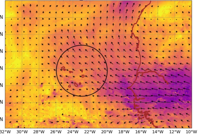
AROME25 20240916-12-UTC -ech(60h) wind_sp920 @ 920hPa
