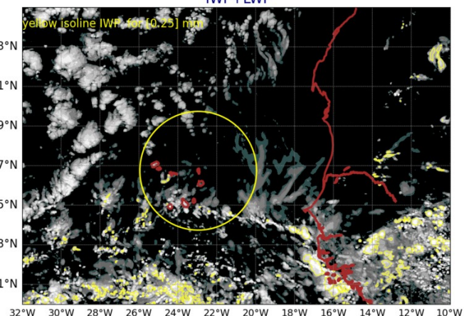
AROME25 20240916-12-UTC -ech(60h) IWP+LWP
