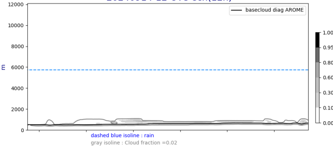
Cross section S/N @ -22W 20240914-12-UTC ech(12h)
