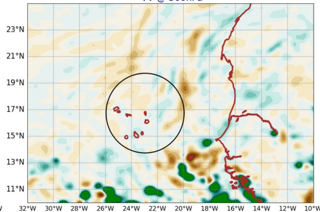
AROME25 20240916-12-UTC -ech(36h) VV @ 500hPa
