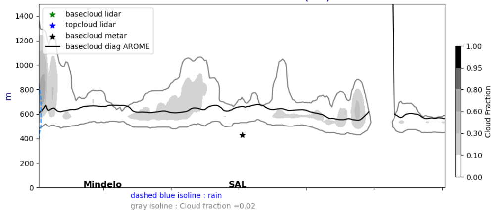
Cross section E/W @ 17.5N 20240915-01-UTC ech(1h)
