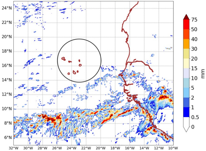
AROME25 20240915-15-UTC -ech(15h) RR cumulated over 6h
