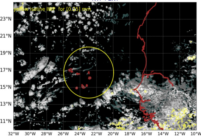
AROME25 20240915-12-UTC -ech(12h) IWP+LWP
