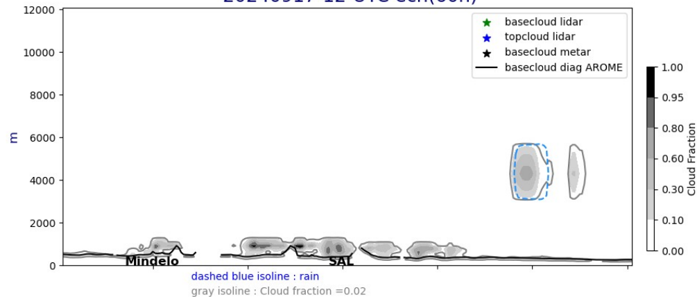
Cross section E/W @ 17.5N 20240917-12-UTC ech(60h)
