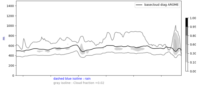
Cross section S/N @ -22W 20240915-12-UTC ech(12h)
