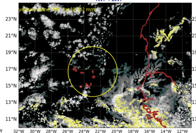
AROME25 20240916-12-UTC -ech(36h) IWP+LWP
