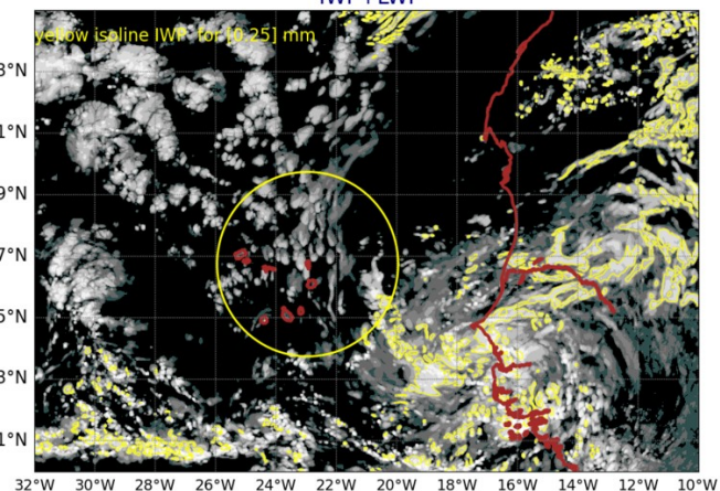
AROME25 20240917-12-UTC -ech(60h) IWP+LWP
