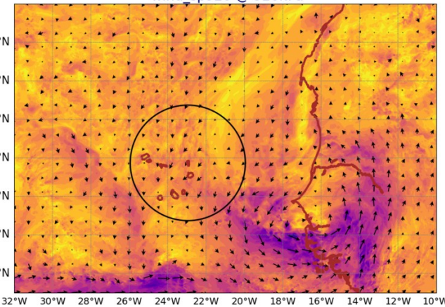
AROME25 20240917-12-UTC -ech(60h) wind_sp920 @ 920hPa
