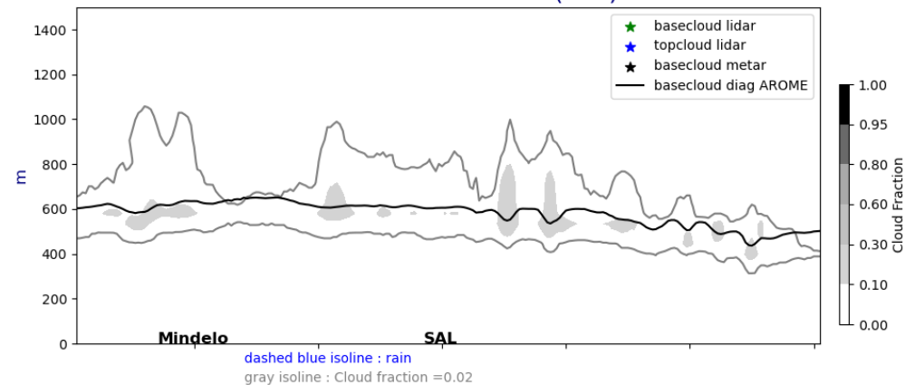
Cross section E/W @ 17.5N 20240915-12-UTC ech(12h)
