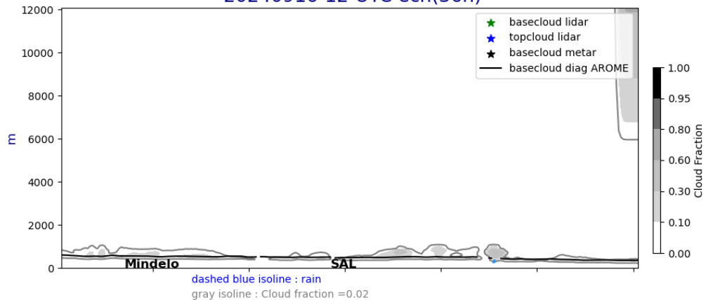
Cross section E/W @ 17.5N 20240916-12-UTC ech(36h)
