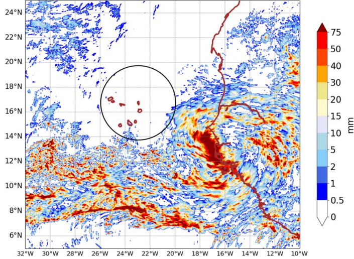
AROME25 20240917-12-UTC -ech(60h) RR cumulated over 24h
