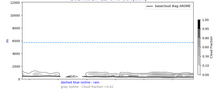
Cross section S/N @ -22W 20240917-12-UTC ech(60h)
