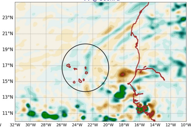
AROME25 20240917-12-UTC -ech(60h) VV @ 500hPa
