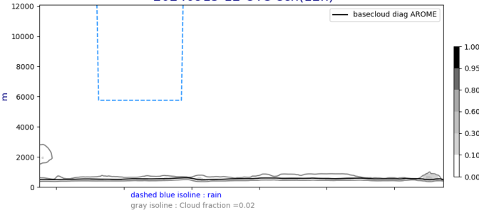
Cross section S/N @ -22W 20240915-12-UTC ech(12h)
