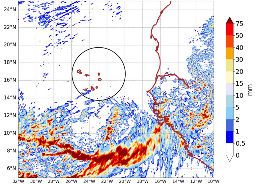
AROME25 20240915-00-UTC -ech(24h)
