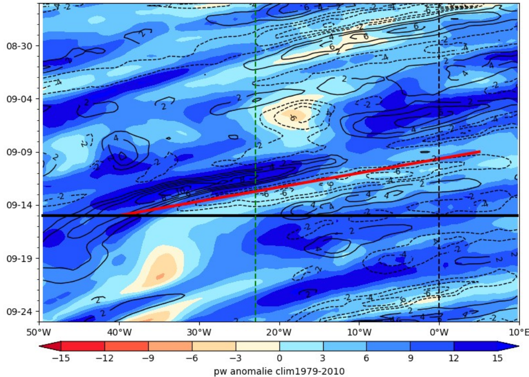
ECMWF PW (color) AND V at 925 hPa 2024-09-15
