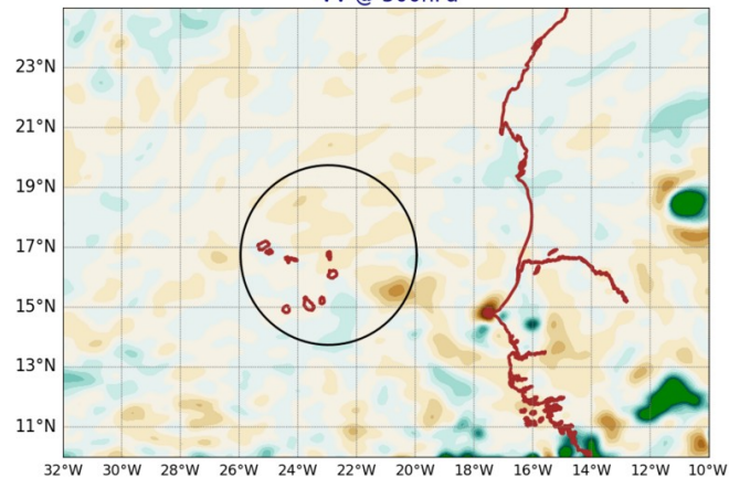
AROME25 20240915-12-UTC -ech(12h) VV @ 500hPa
