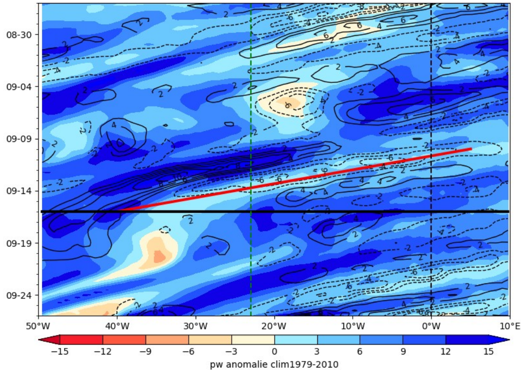
ECMWF PW (color) AND V at 925 hPa 2024-09-16
