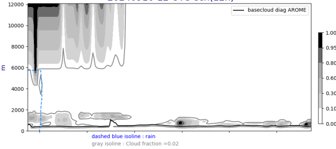
Cross section S/N @ -22W 20240916-12-UTC ech(12h)
