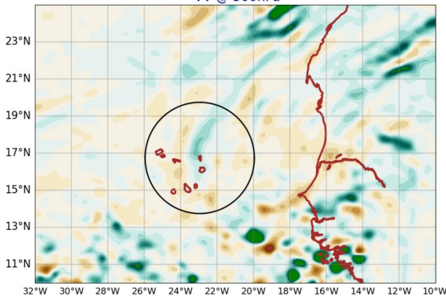
AROME25 20240917-12-UTC -ech(36h) VV @ 500hPa
