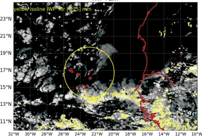
AROME25 20240916-12-UTC -ech(12h) IWP+LWP
