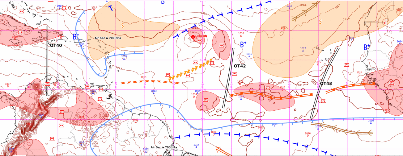
ANASYG du Lun. 16/09/2024 - 00 UTC
