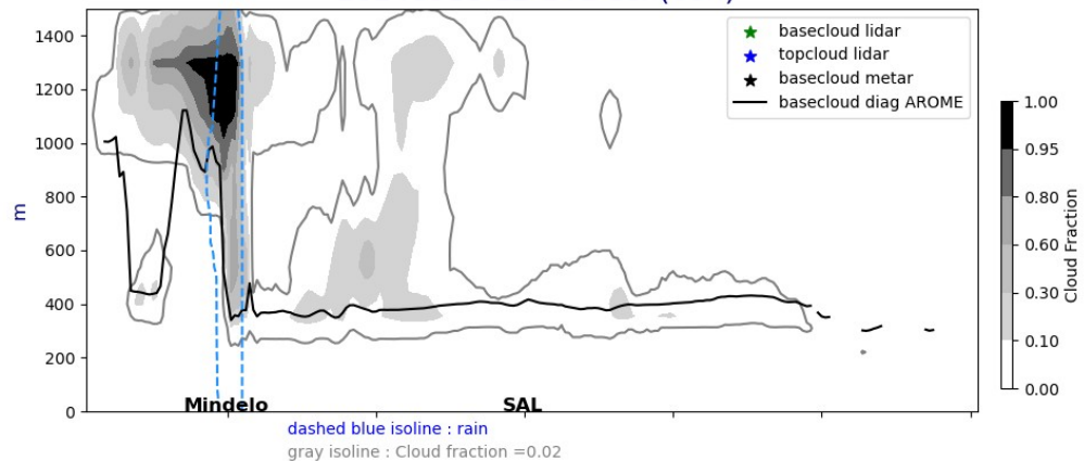
Cross section E/W @ 17.5N 20240918-12-UTC ech(60h)
