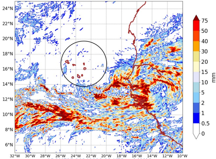
AROME25 20240918-12-UTC -ech(60h) RR cumulated over 24h
