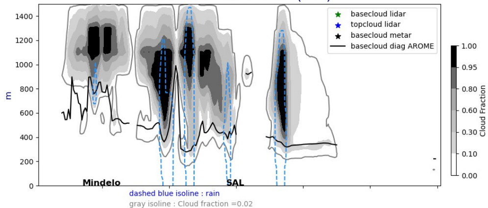
Cross section E/W @ 17.5N 20240917-12-UTC ech(36h)
