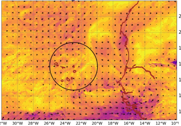
AROME25 20240916-12-UTC -ech(12h) wind_sp920 @ 920hPa
