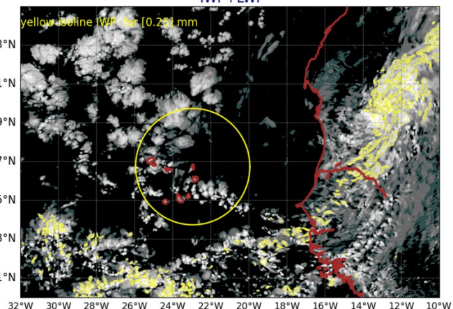
AROME25 20240918-12-UTC -ech(60h) IWP+LWP
