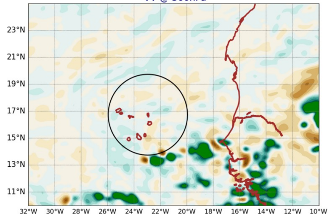
AROME25 20240916-12-UTC -ech(12h) VV @ 500hPa
