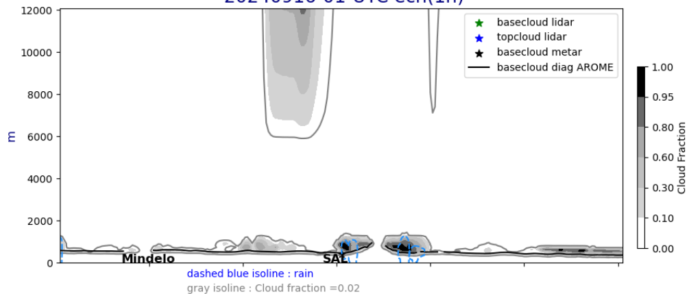
Cross section E/W @ 17.5N 20240916-01-UTC ech(1h)
