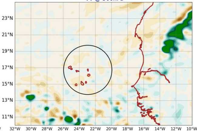
AROME25 20240918-12-UTC -ech(60h) VV @ 500hPa
