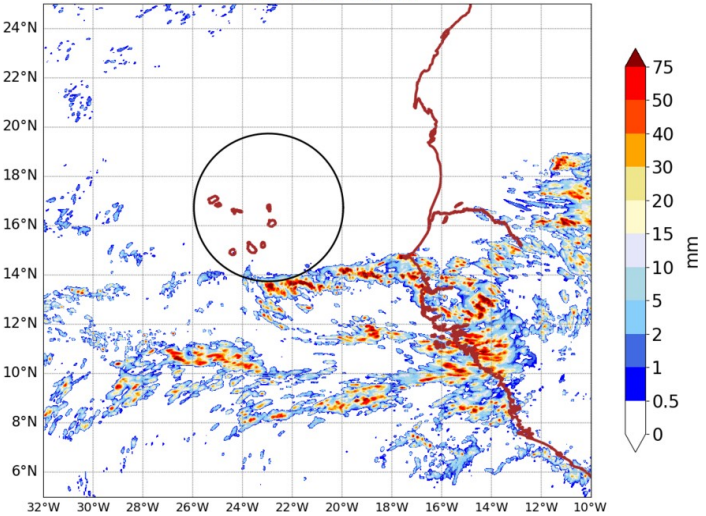
AROME25 20240916-15-UTC -ech(15h) RR cumulated over 6h
