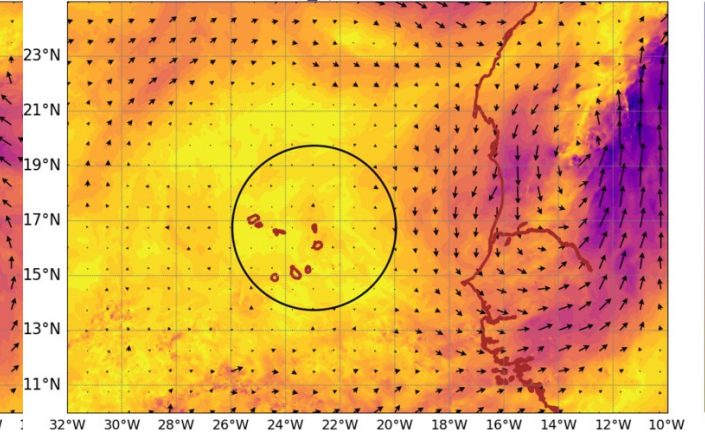
AROME25 20240918-12-UTC -ech(60h) wind_sp920 @ 920hPa
