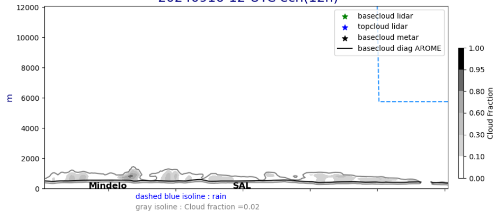
Cross section E/W @ 17.5N 20240916-12-UTC ech(12h)
