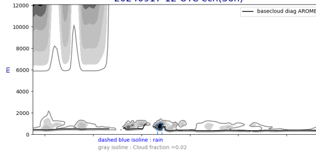
Cross section S/N @ -22W 20240917-12-UTC ech(36h)
