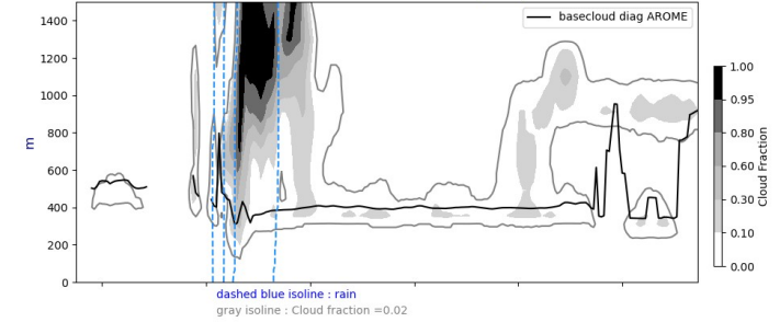
Cross section S/N @ -22W 20240918-12-UTC ech(60h)
