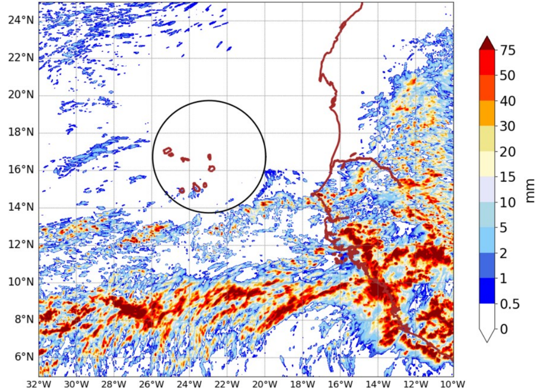
AROME25 20240916-00-UTC -ech(24h)
