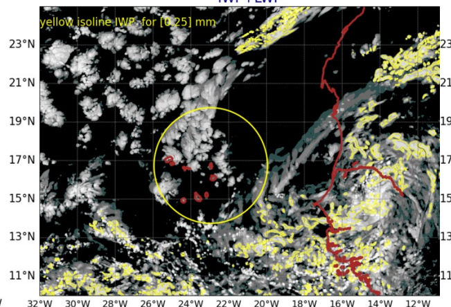
AROME25 20240917-12-UTC -ech(36h) IWP+LWP
