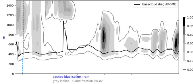
Cross section S/N @ -22W 20240916-12-UTC ech(12h)
