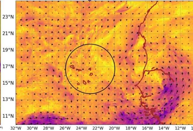
AROME25 20240917-12-UTC -ech(36h) wind_sp920 @ 920hPa
