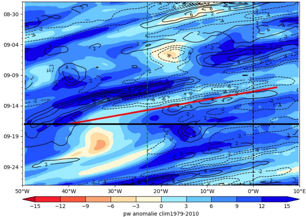
ECMWF PW (color) AND V at 925 hPa 2024-09-17
