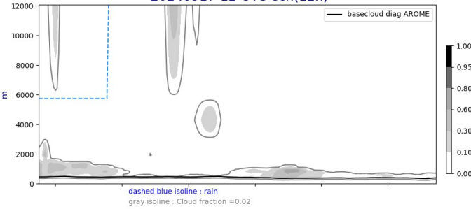
Cross section S/N @ -22W 20240917-12-UTC ech(12h)
