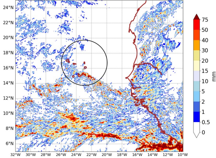
AROME25 20240919-12-UTC -ech(60h) RR cumulated over 24h
