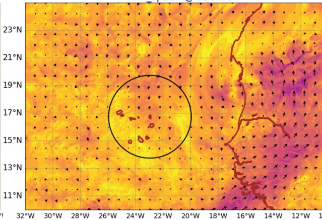
AROME25 20240918-12-UTC -ech(36h) wind_sp920 @ 920hPa
