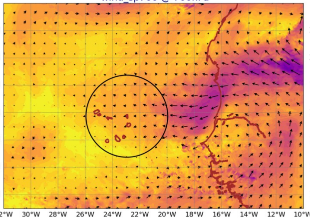
AROME25 20240917-12-UTC -ech(12h) wind_sp920 @ 920hPa
