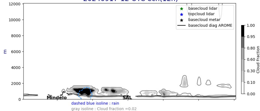
Cross section E/W @ 17.5N 20240917-12-UTC ech(12h)
