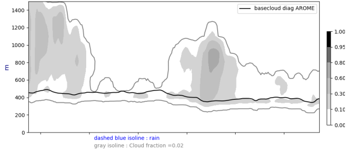
Cross section S/N @ -22W 20240917-12-UTC ech(12h)
