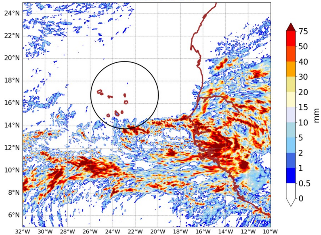
AROME25 20240917-00-UTC -ech(24h)
