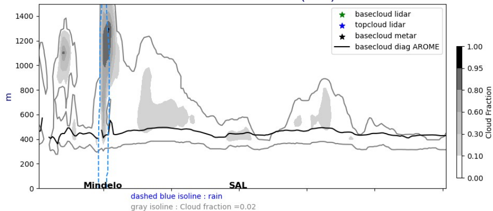
Cross section E/W @ 17.5N 20240918-12-UTC ech(36h)
