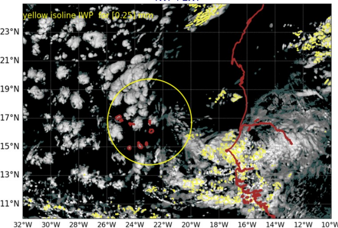
AROME25 20240917-12-UTC -ech(12h) IWP+LWP
