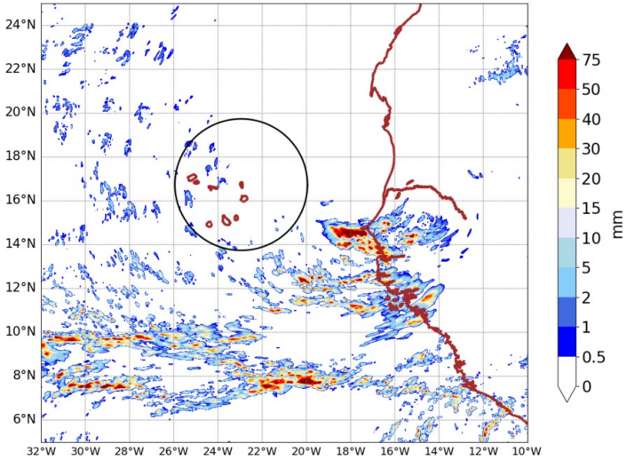
AROME25 20240917-15-UTC -ech(15h) RR cumulated over 6h
