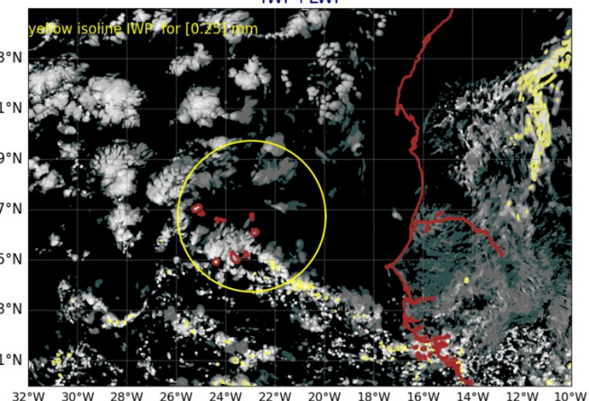
AROME25 20240919-12-UTC -ech(60h) IWP+LWP
