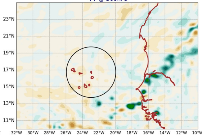
AROME25 20240918-12-UTC -ech(36h) VV @ 500hPa
