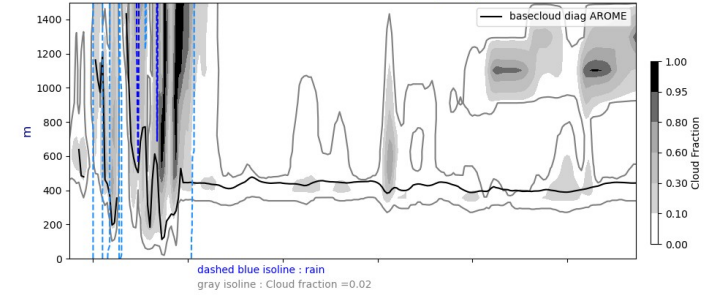
Cross section S/N @ -22W 20240919-12-UTC ech(60h)
