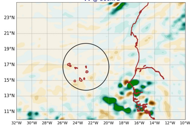
AROME25 20240917-12-UTC -ech(12h) VV @ 500hPa
