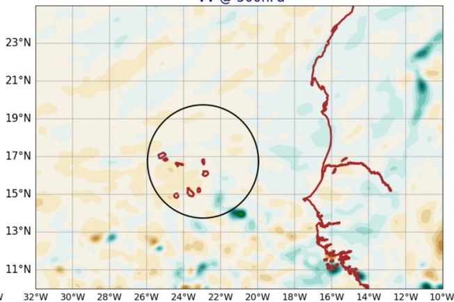
AROME25 20240919-12-UTC -ech(60h) VV @ 500hPa
