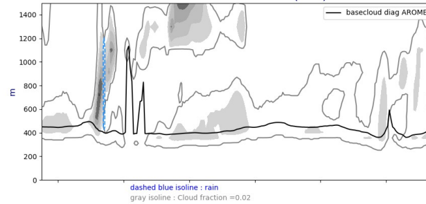
Cross section S/N @ -22W 20240918-12-UTC ech(36h)
