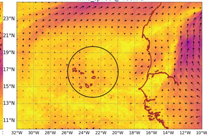
AROME25 20240919-12-UTC -ech(60h) wind_sp920 @ 920hPa
