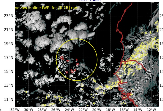
AROME25 20240918-12-UTC -ech(36h) IWP+LWP
