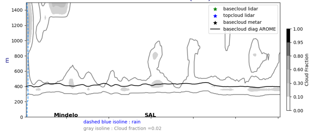
Cross section E/W @ 17.5N 20240919-12-UTC ech(60h)
