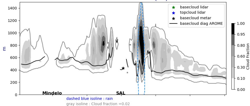
Cross section E/W @ 17.5N 20240917-01-UTC ech(1h)
